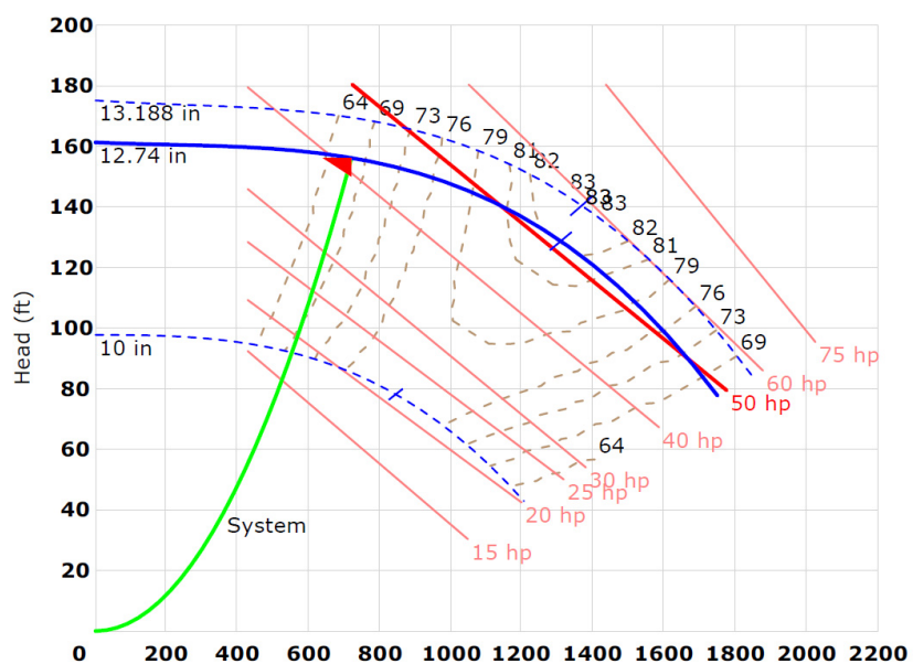
Figure 4. Single Speed Pump Curve
