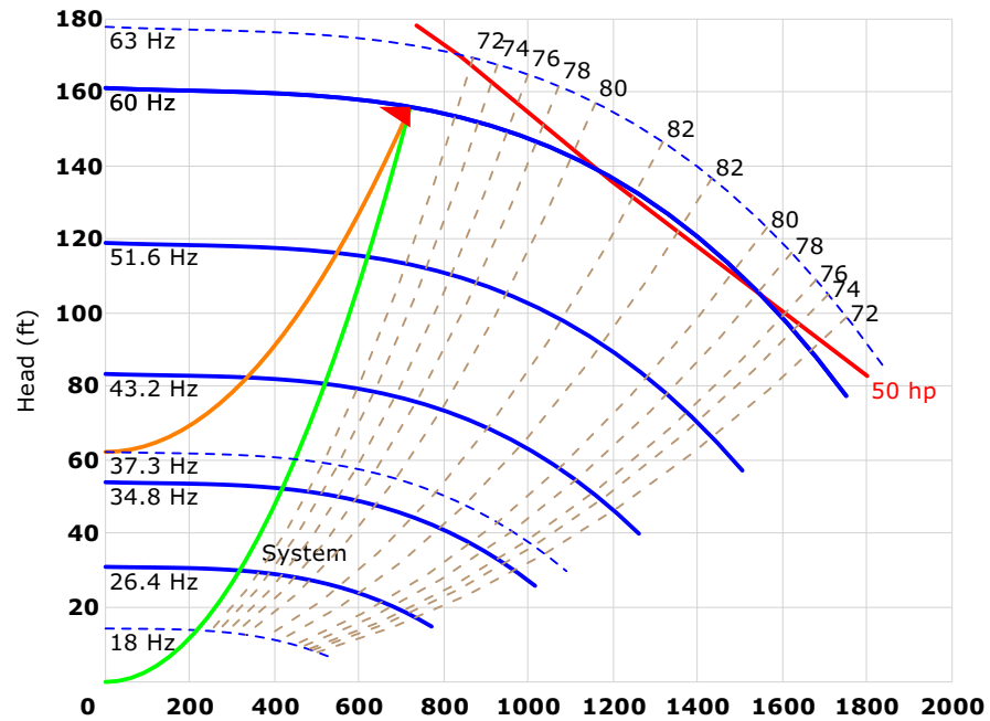
Figure 5. Multi Speed Pump Curve
