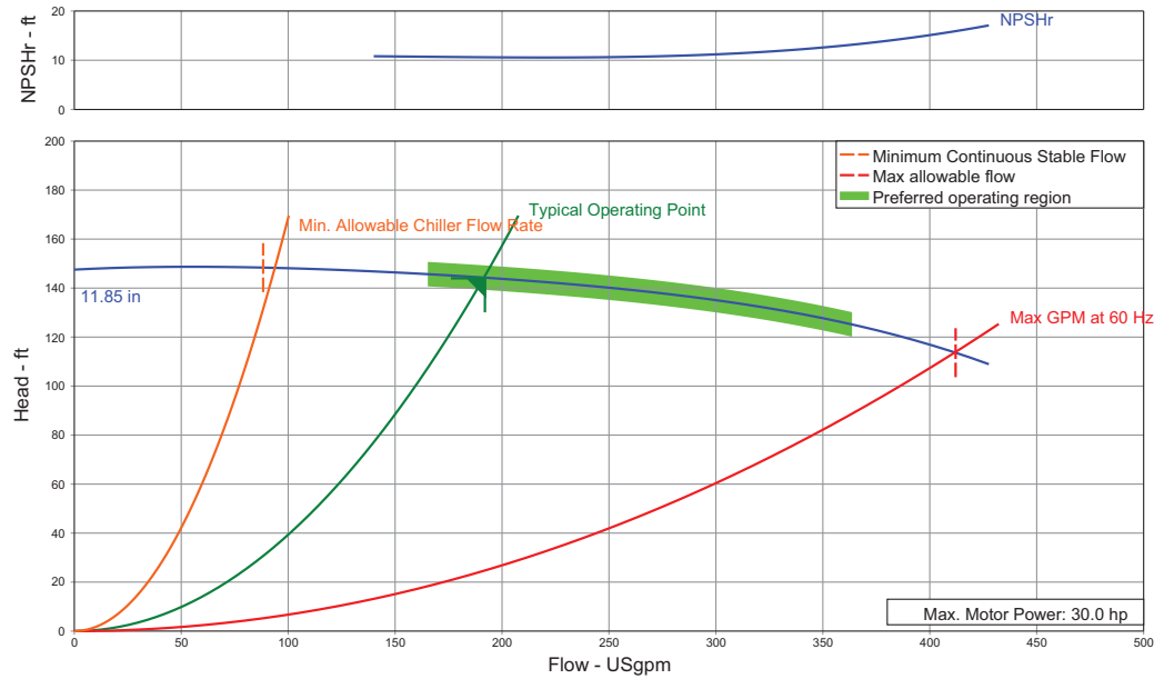
Single Speed Pump Curve
