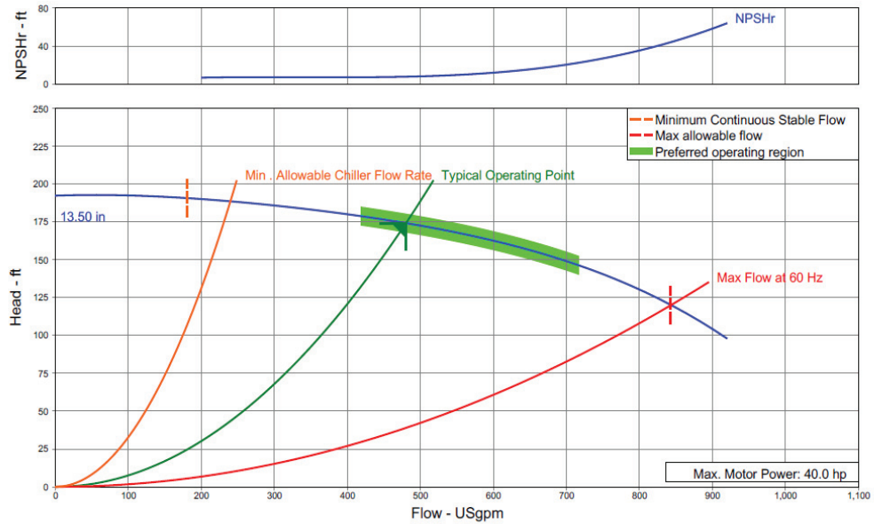
F0 and F1 Style ACSA Chillers - Single Speed Pump Curve
