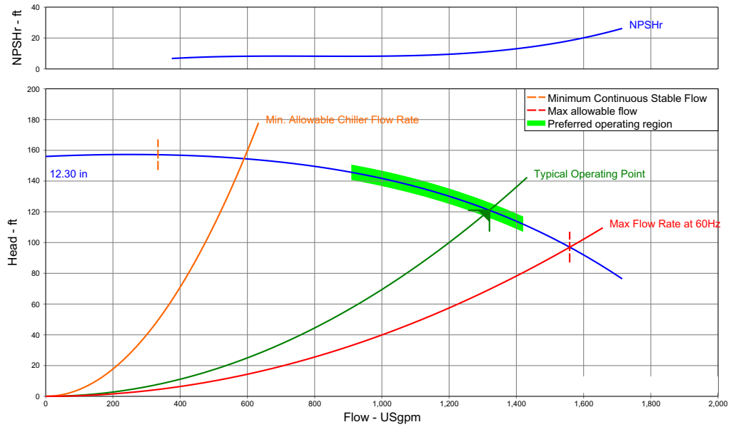
Figure 11. Multi Speed Pump Curve
