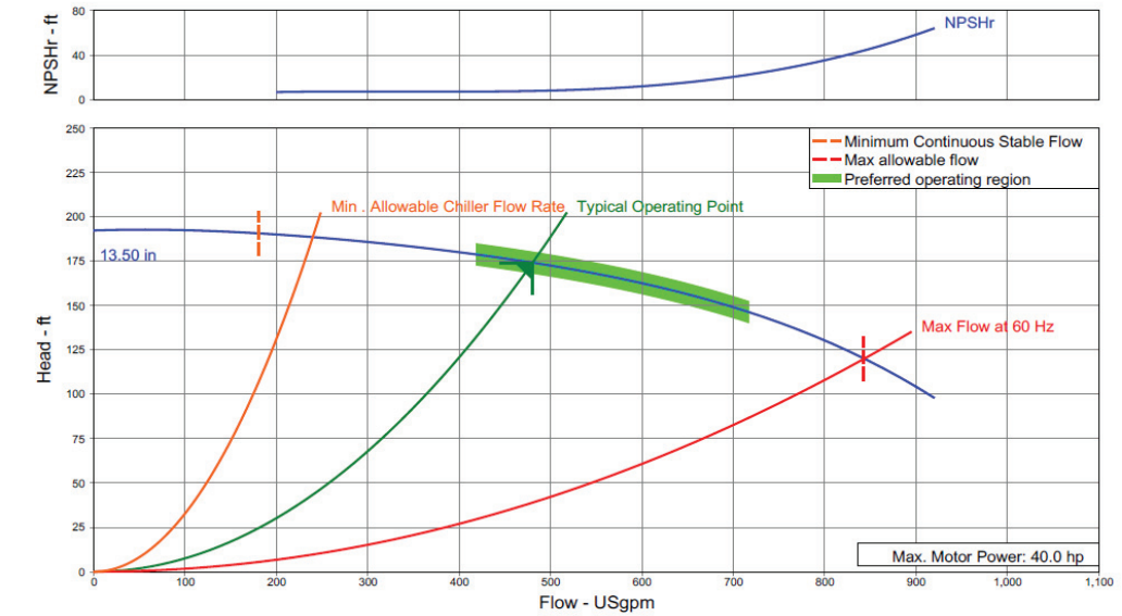
Single Speed Pump Curve
