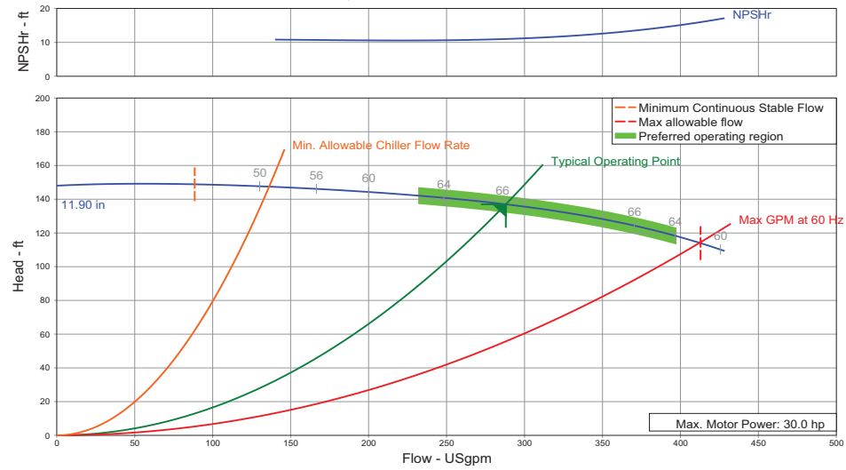
Single Speed Pump Curve
