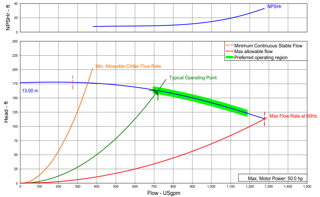
Multi Speed Pump Curve
