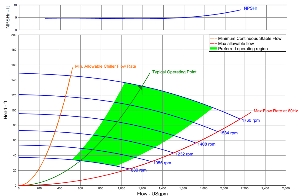
Figure 9. Multi Speed Pump Curve
