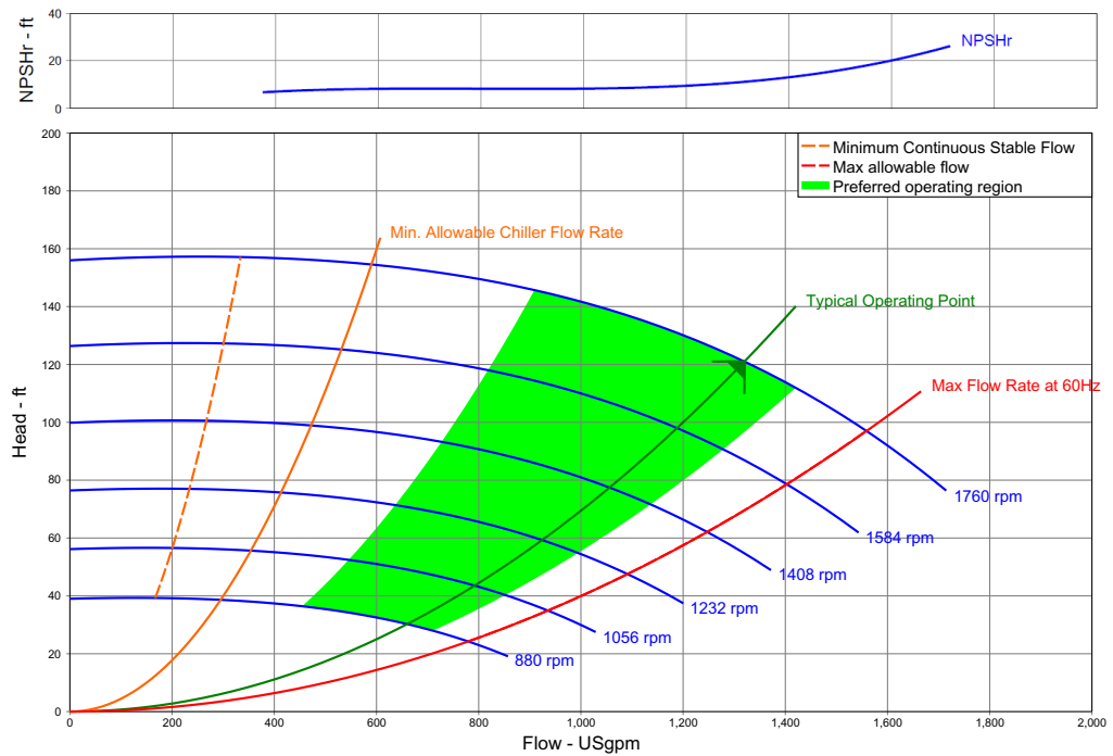
Figure 11. Multi Speed Pump Curve
