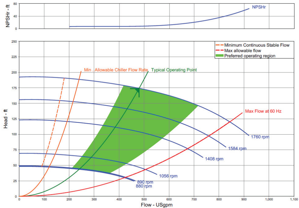
F0 and F1 Style ACSA Chillers - Multi Speed Pump Curve
