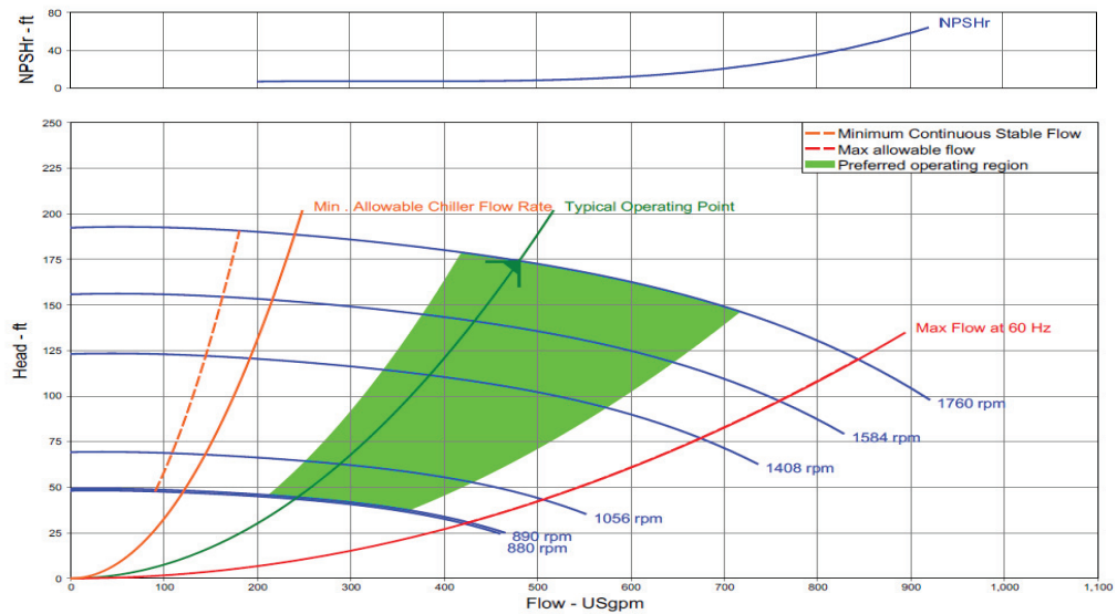
Multi-Speed Pump Curve
