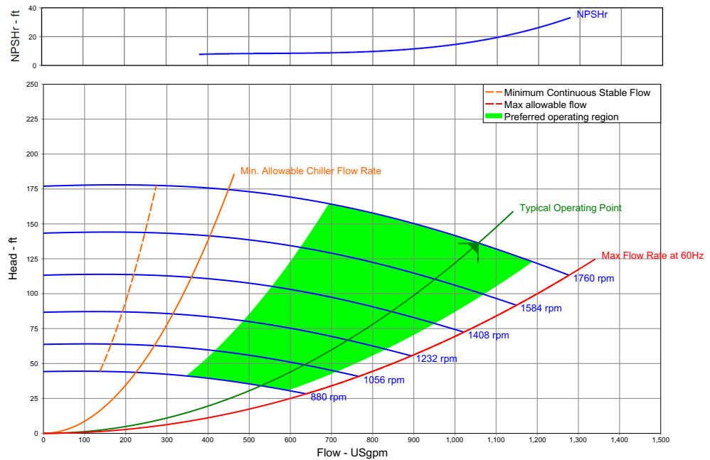
Figure 7. Multi Speed Pump Curve
