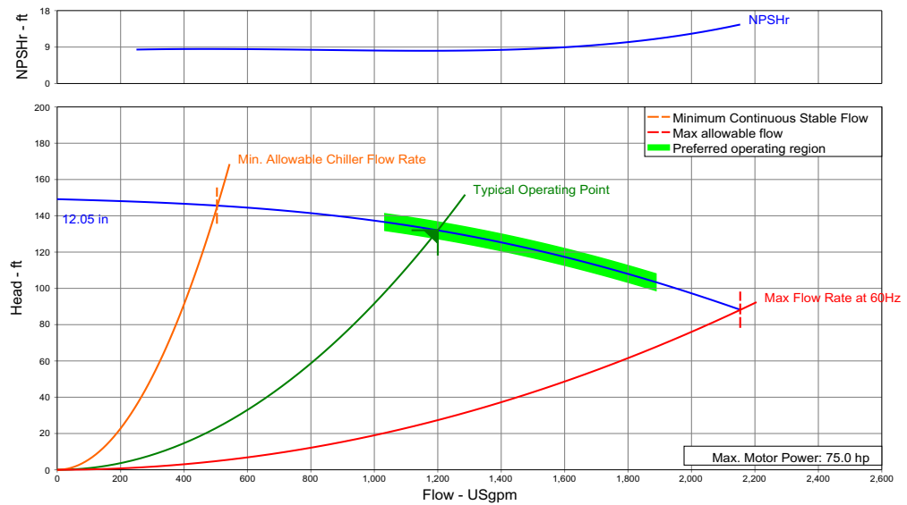
Figure 9. Multi Speed Pump Curve
