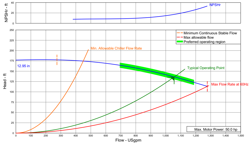
Figure 7. Multi Speed Pump Curve
