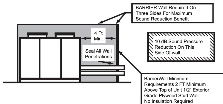
Figure 3. Minimum wall requirements
