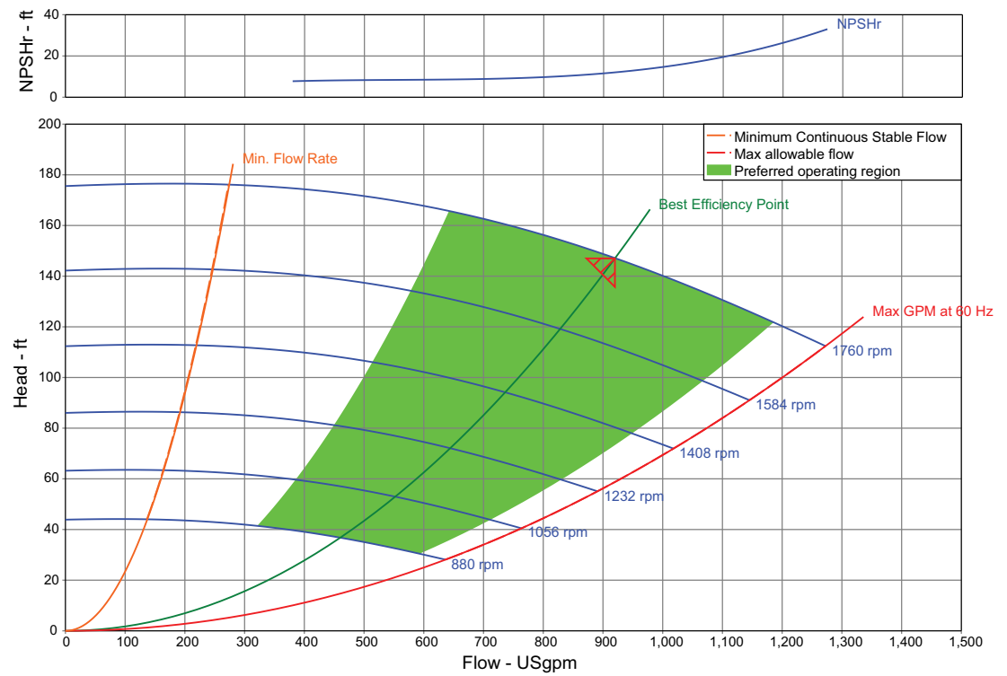
Figure 43. 300 to 440 Ton ACRC (F0) multi speed pump curve
