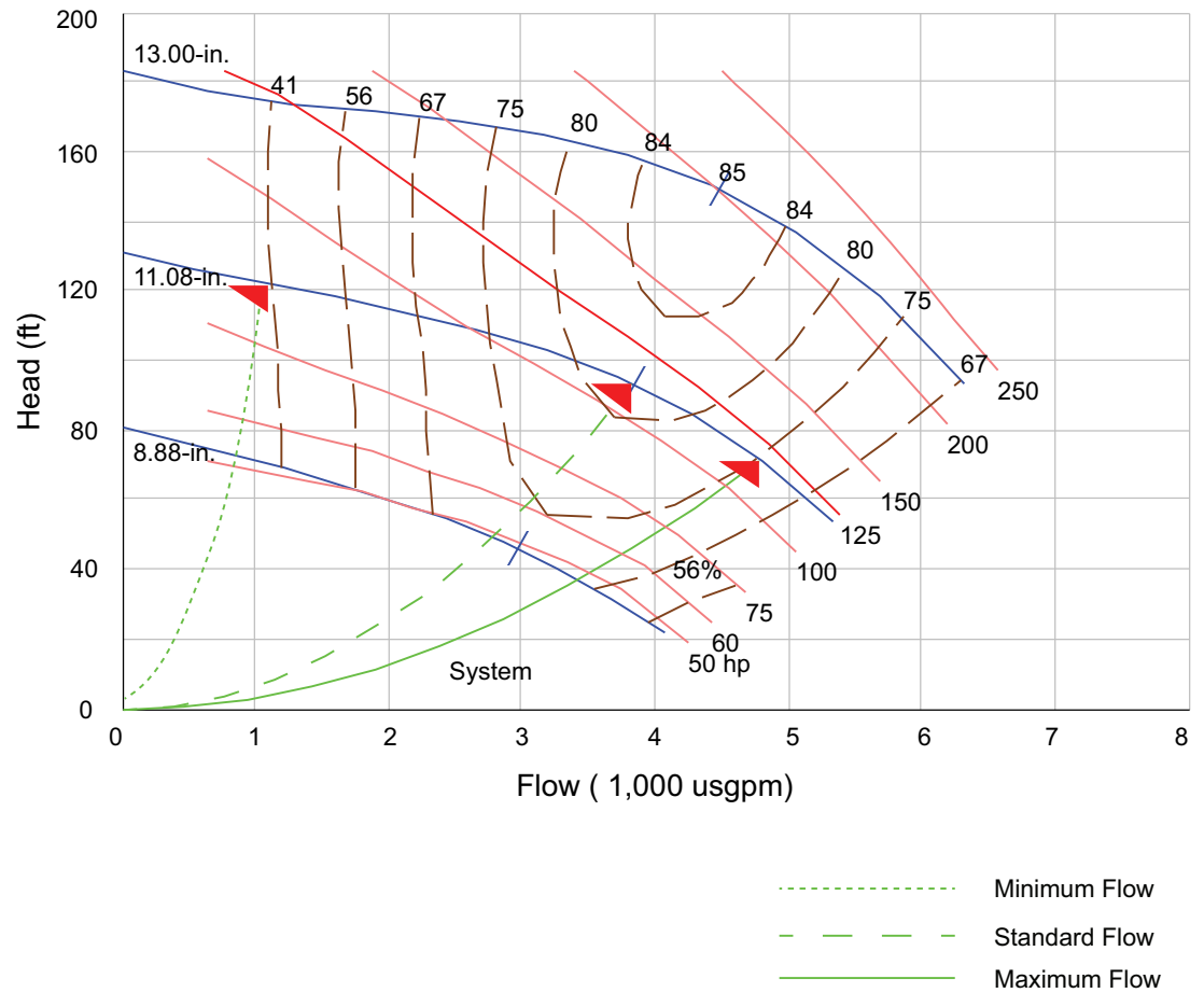
Figure 26. RSPC0125F2 pump curve
