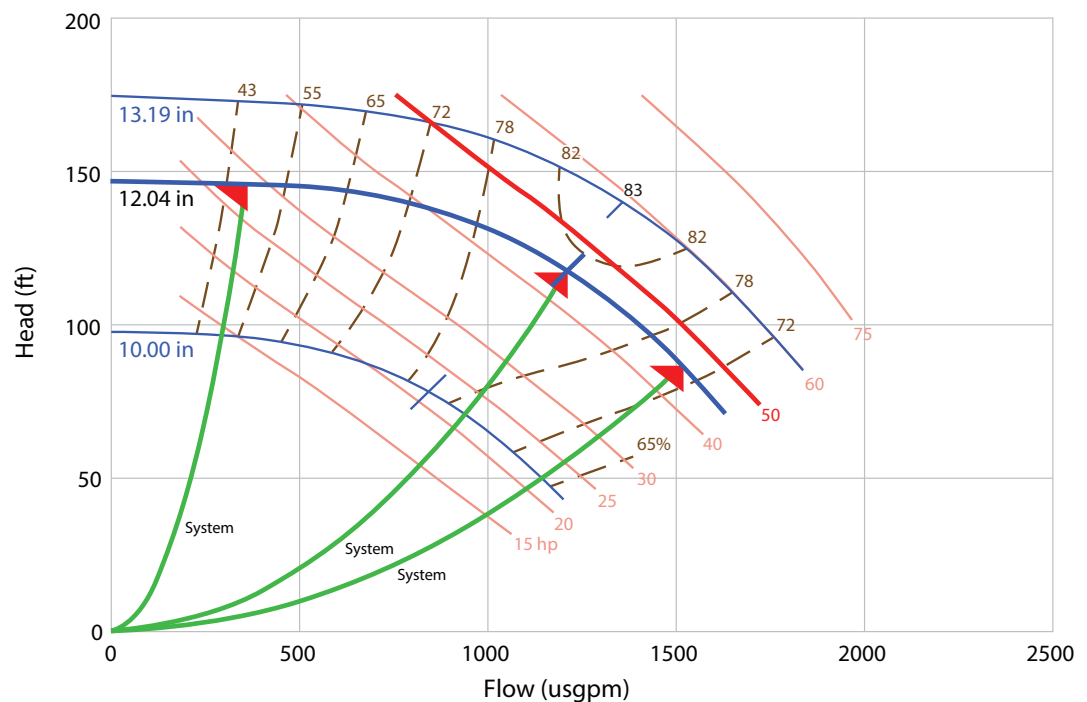
Figure 39. 300/400 ton RTAC (F2 to F3) pump curve
