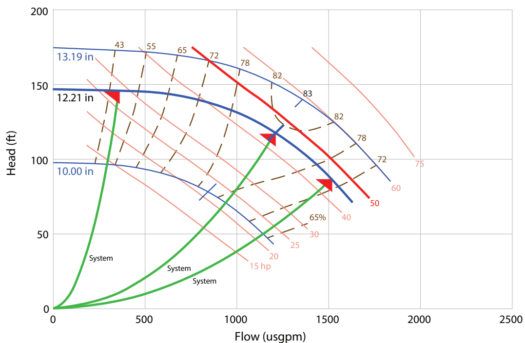
Figure 44. 500 ton RTAC (F0) pump curve
