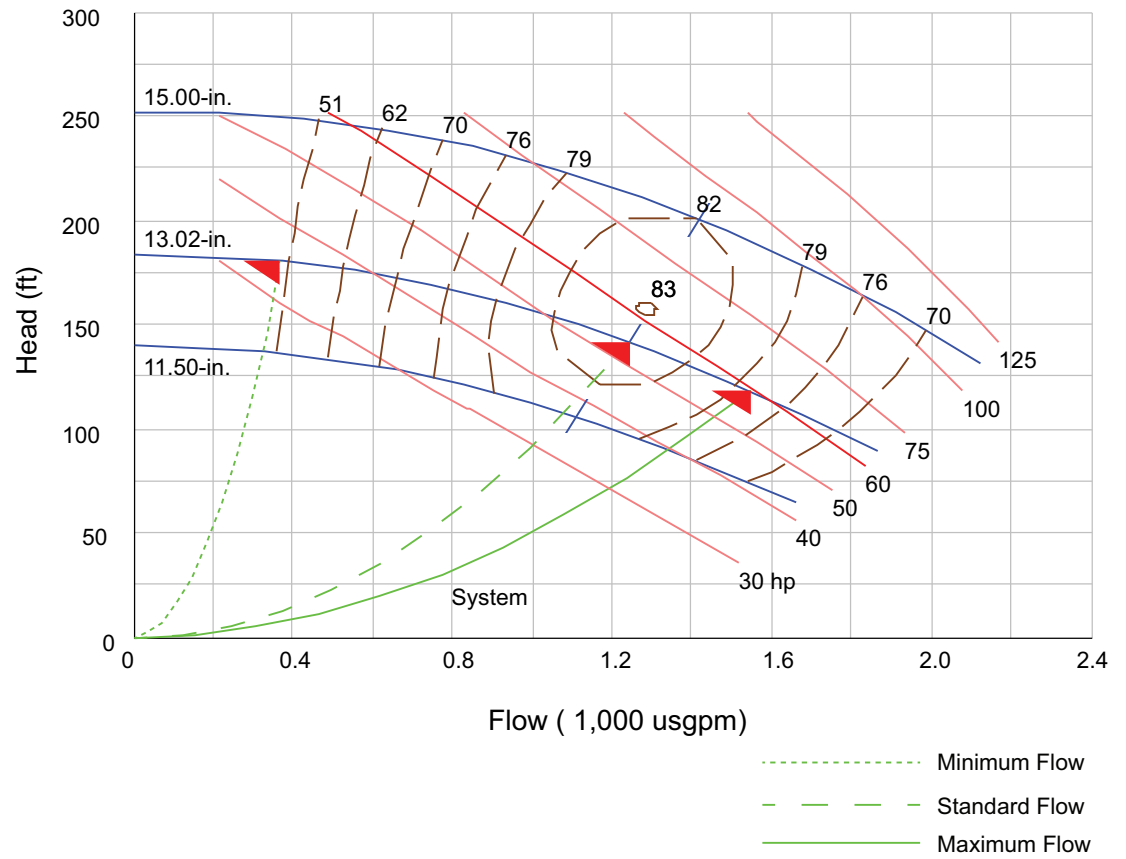
Figure 20. CSPC0060F1 pump curve
