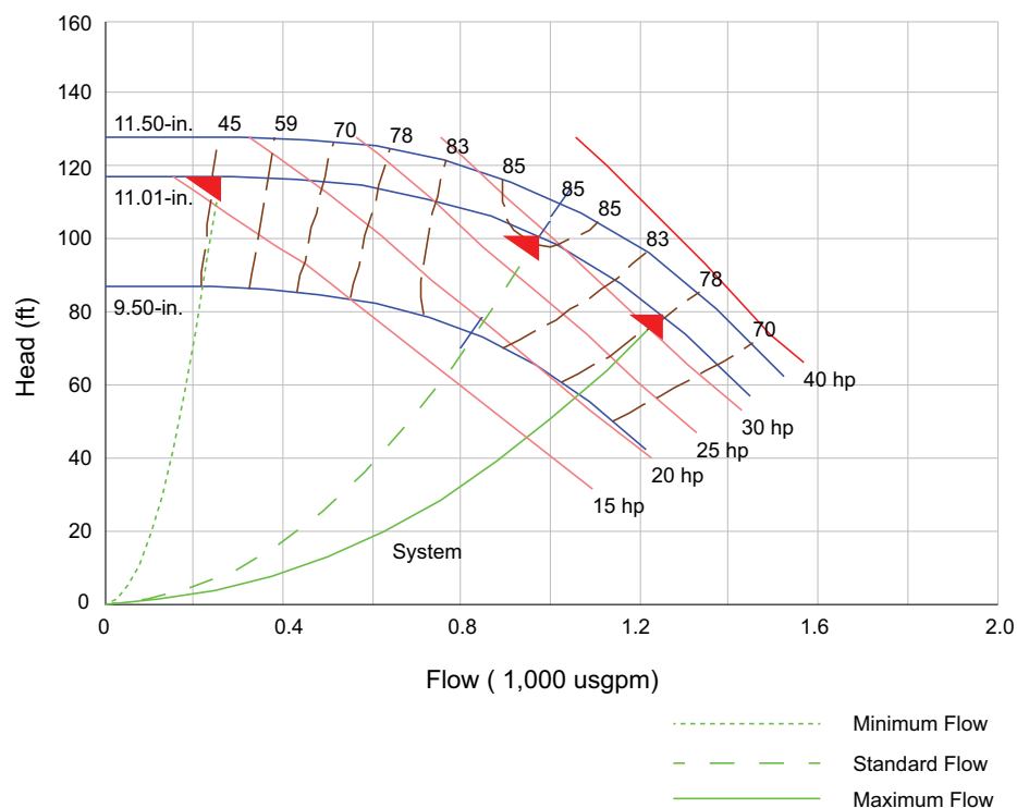
Figure 36. 250 ton RTAC (F0) pump curve
