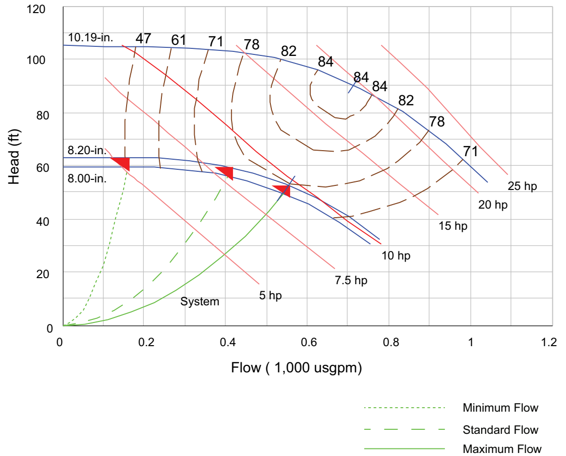
Figure 2. CSPC0010F0 (AA through AH) pump curve
