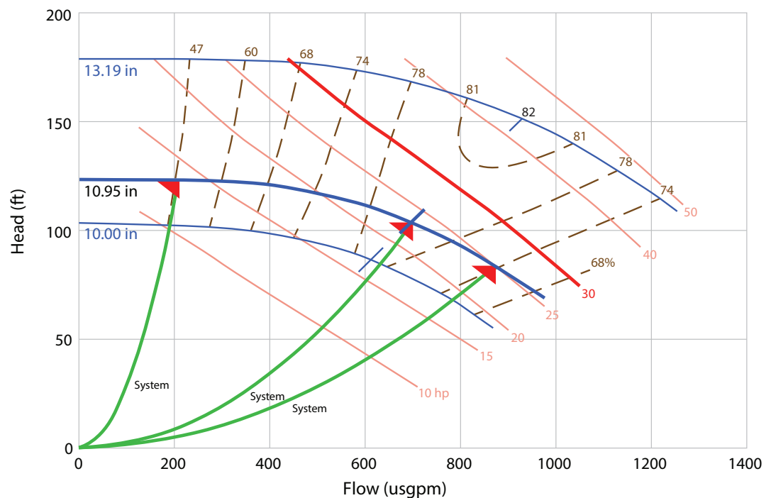
Figure 37. 250 ton RTAC (F2 to F3) pump curve
