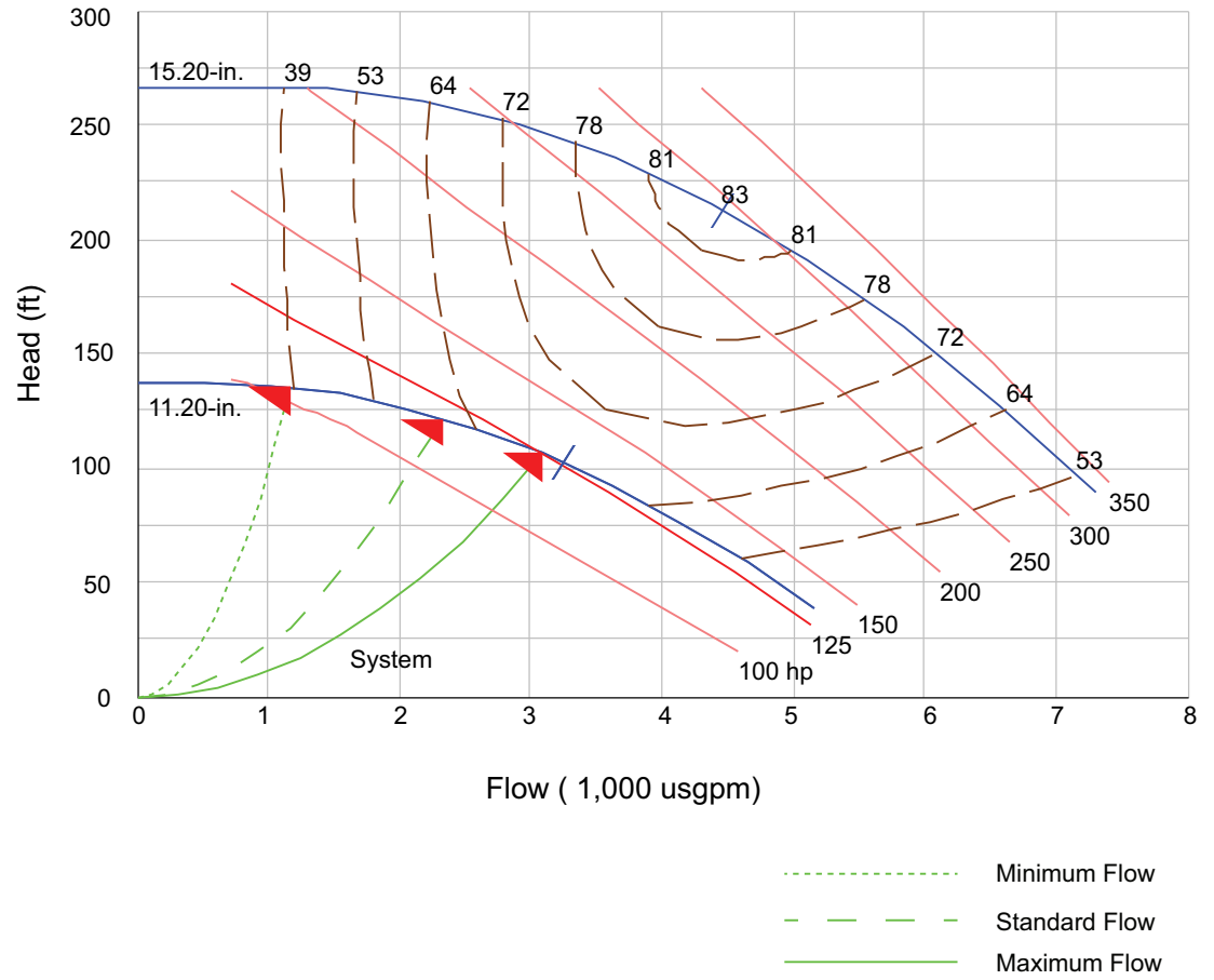
Figure 25. CSPC0125F1 (AG through AQ) pump curve
