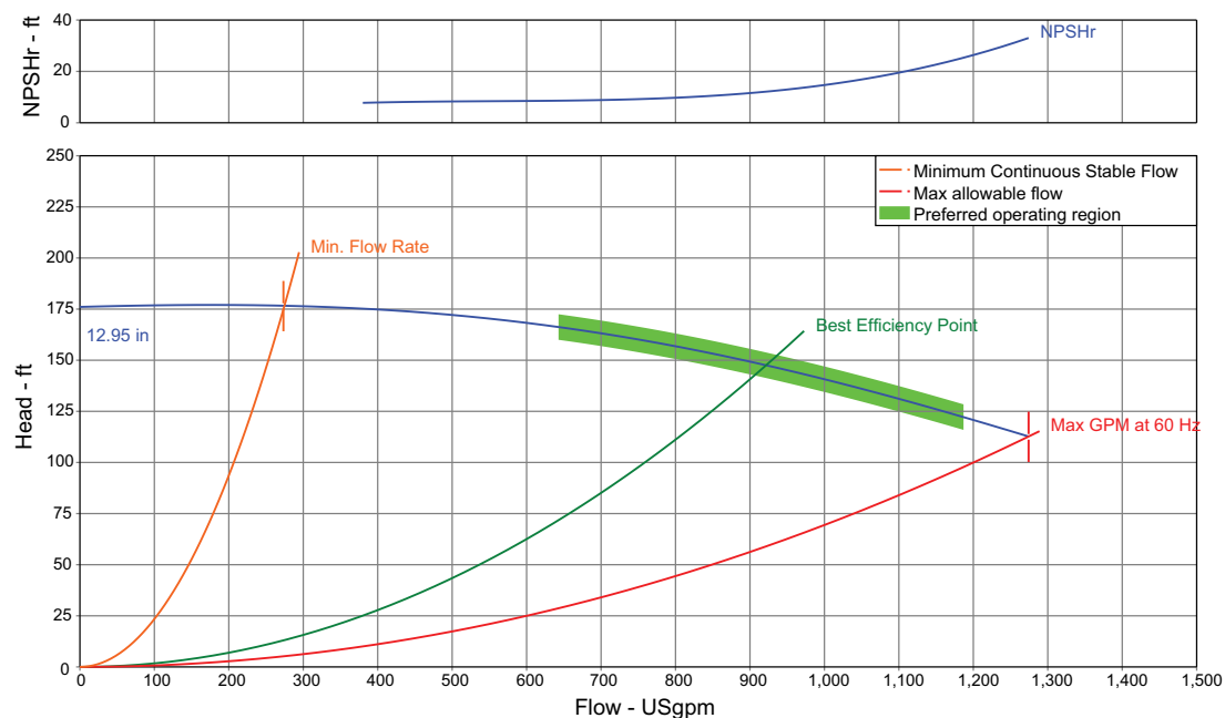
Figure 42. 300 to 440 Ton ACRC (F0) single speed pump curve
