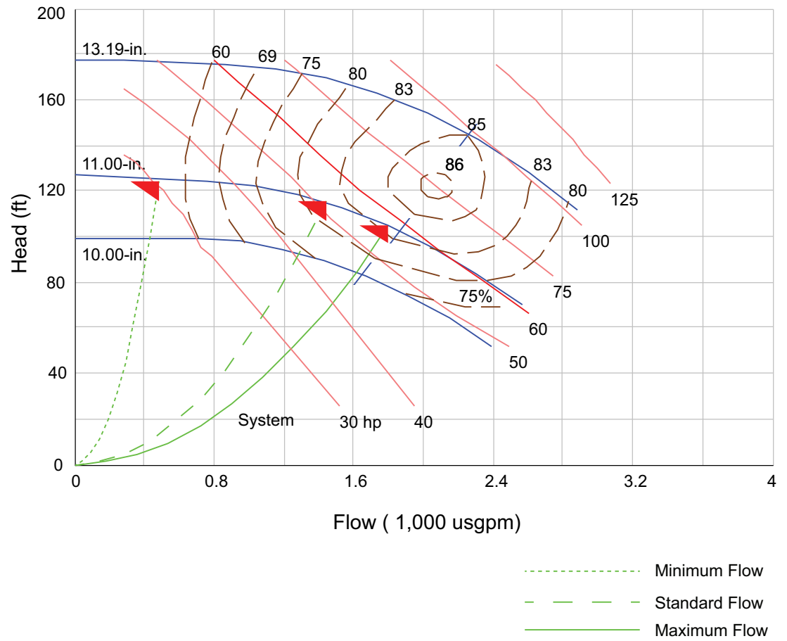
Figure 18. CSPC0060F0 (AA through AL) pump curve
