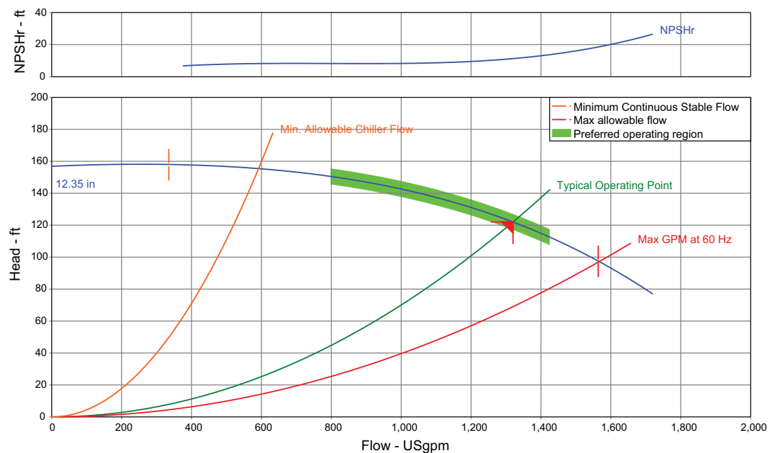
Figure 48. 550 Ton ACRC (F0) single speed pump curve
