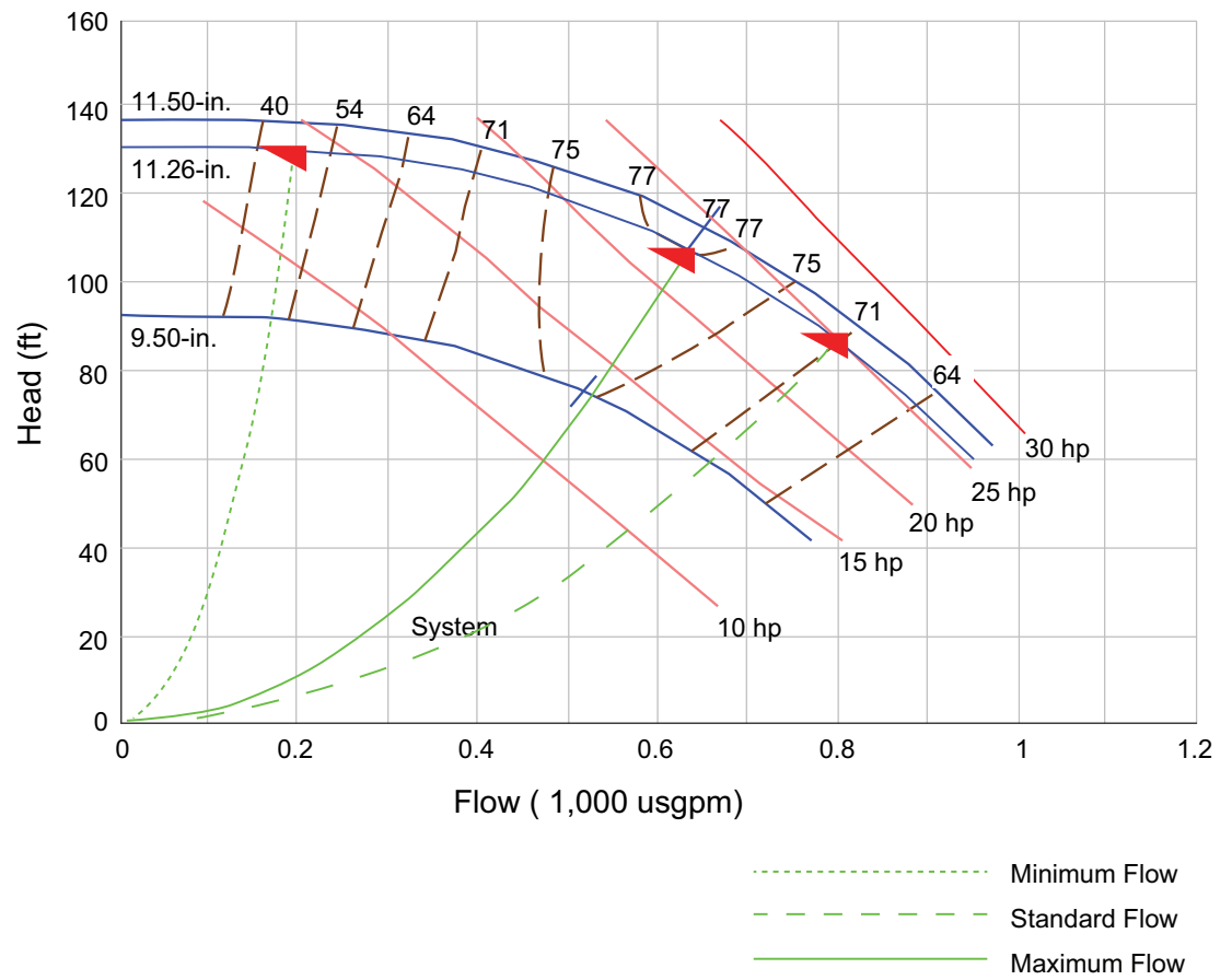
Figure 10. 30 HP pump curve – 1800 rpm
