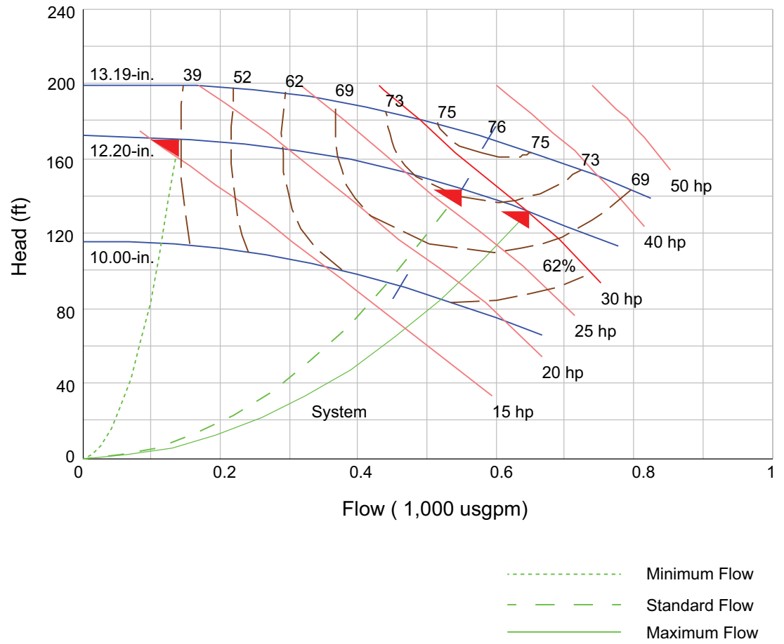
Figure 7. CSPC0030F0 pump curve
