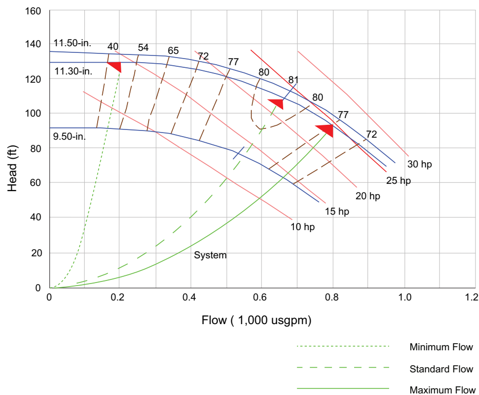
Figure 32. 155/170/200 ton RTAC (F0) pump curve
