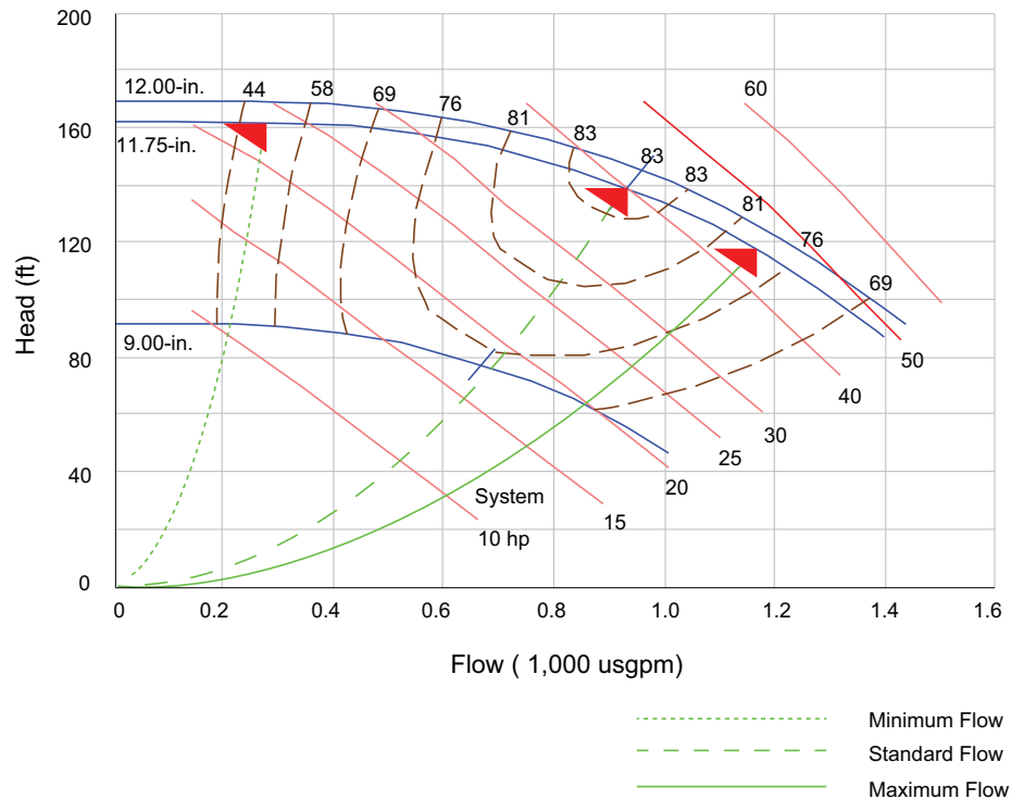
Figure 38. 400 ton RTAA and 300/400 ton RTAC (F0) pump curve
