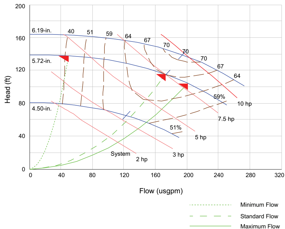
Figure 29. 40 to 60 ton CGAM pump curve
