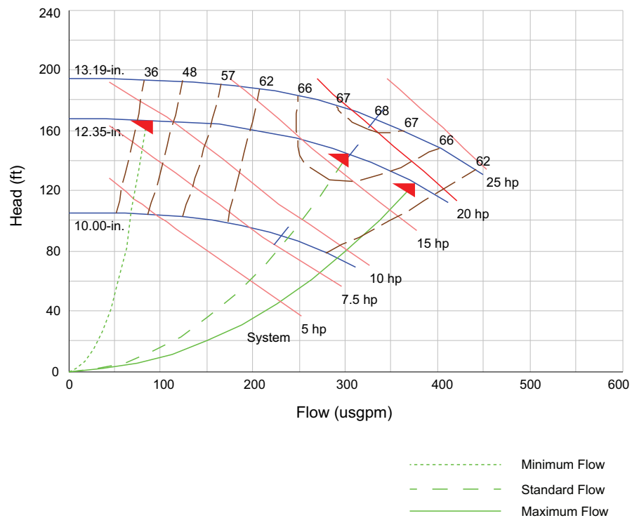
Figure 30. 80 to 120 ton CGAM (F1 to F3) pump curve
