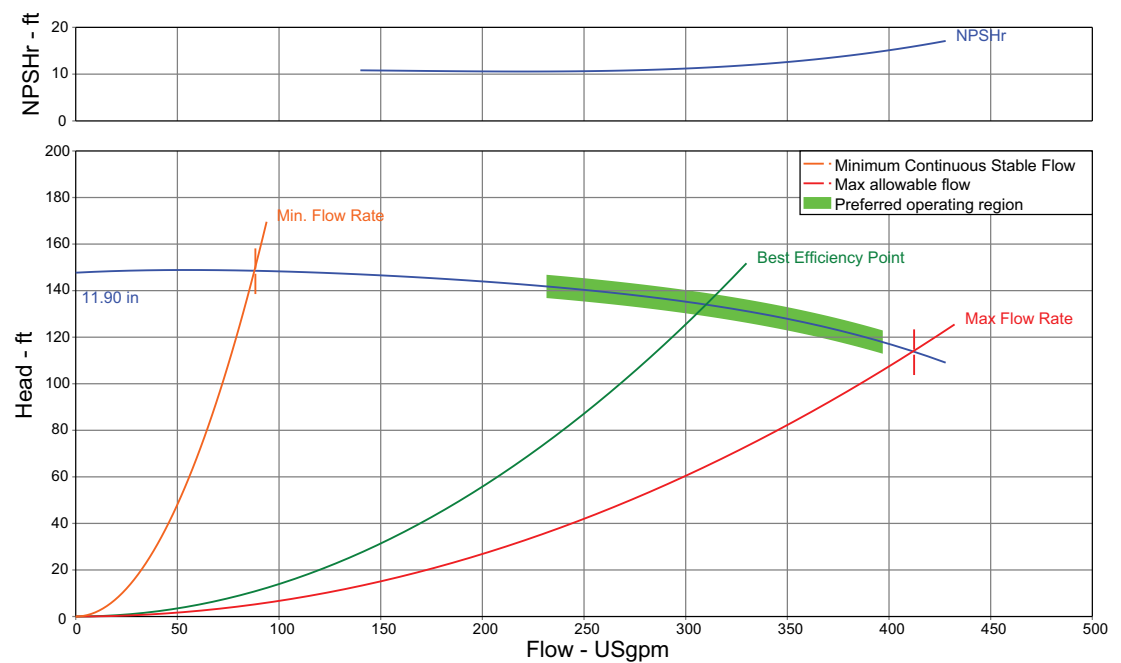
Figure 31. 80 to 120 ton CGAM (F4) pump curve
