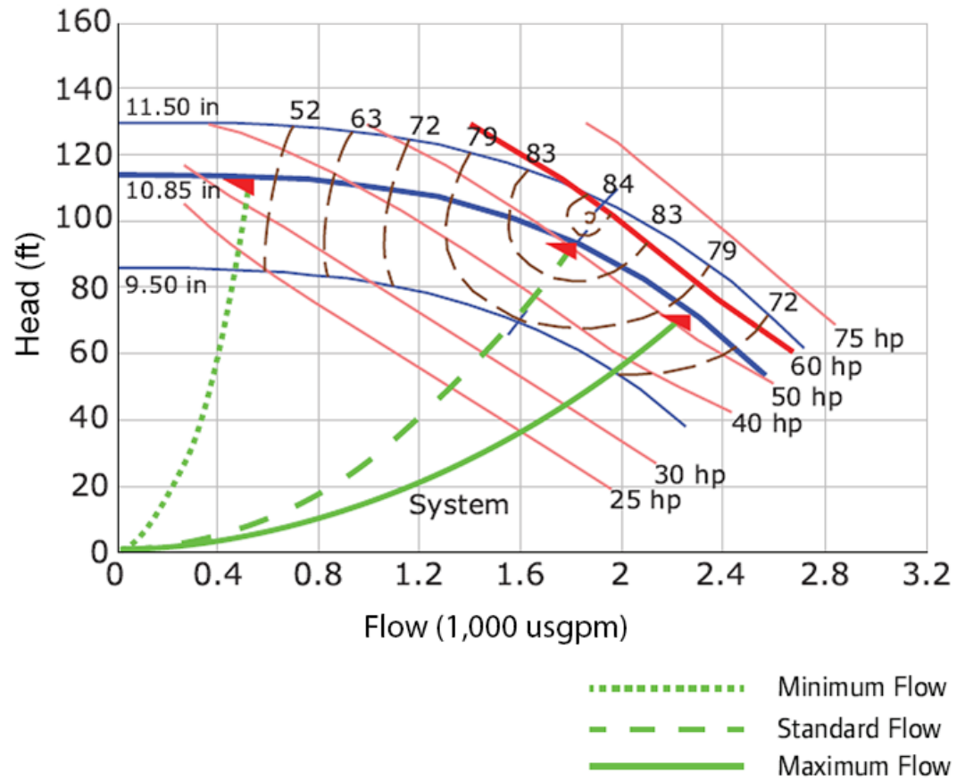
Figure 21. RSPC0060F2 pump curve
