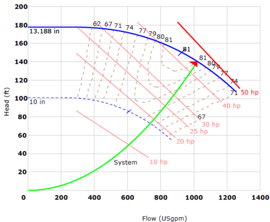
Figure 40. 300 to 440 Ton RTAG single speed pump curve
