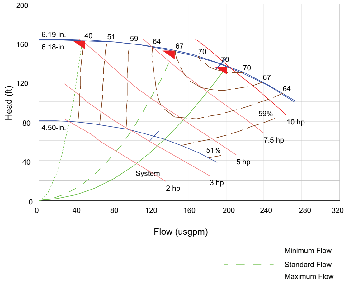
Figure 3. CSPC0010F0 (AL through AO) pump curve
