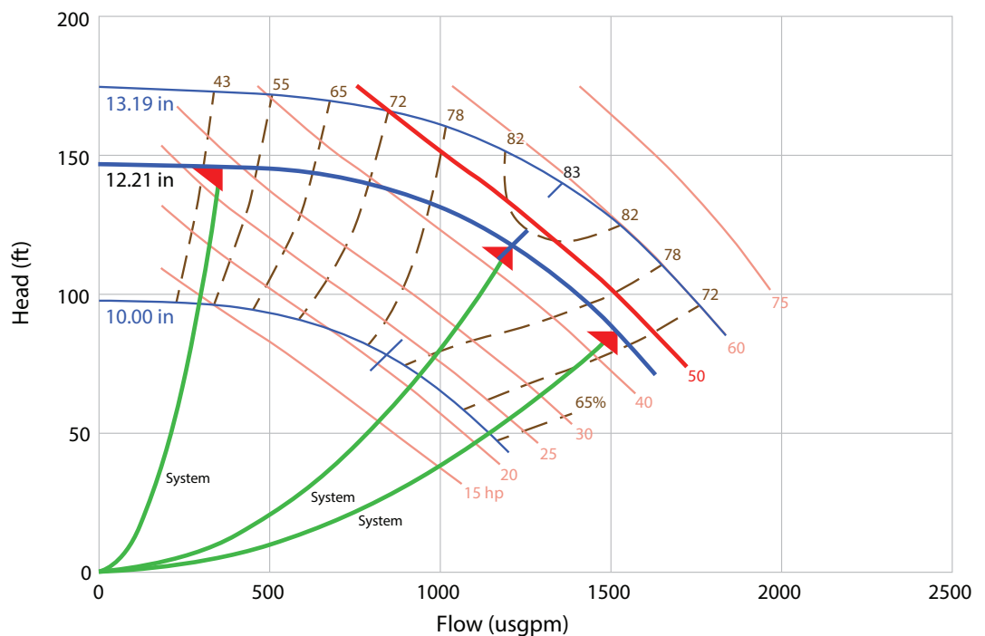
Figure 45. 500 Ton RTAC (F2 to F4) pump curve
