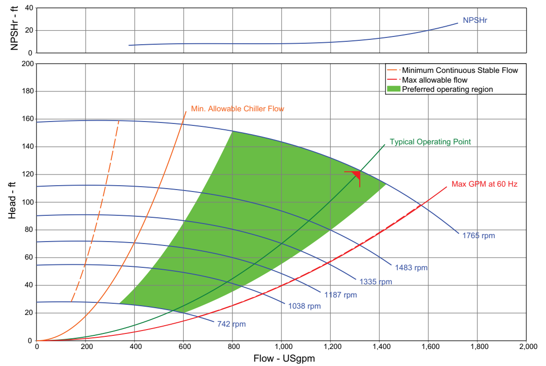
Figure 49. 550 Ton ACRC (F0) multi speed pump curve
