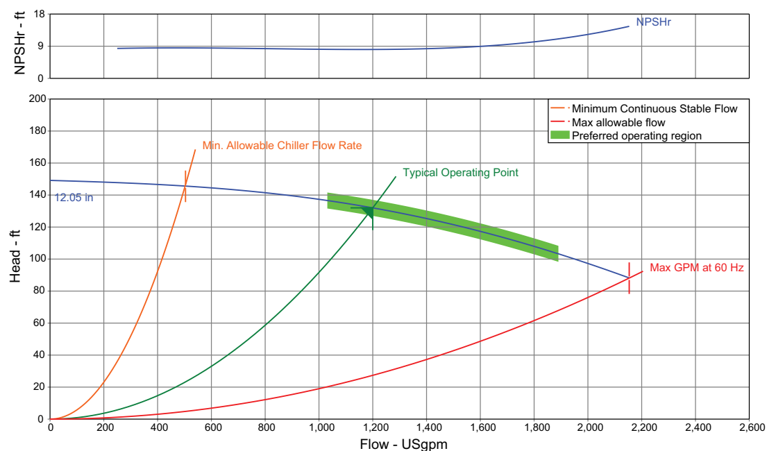
Figure 46. 500 Ton RTAF (F0) single speed pump curve
