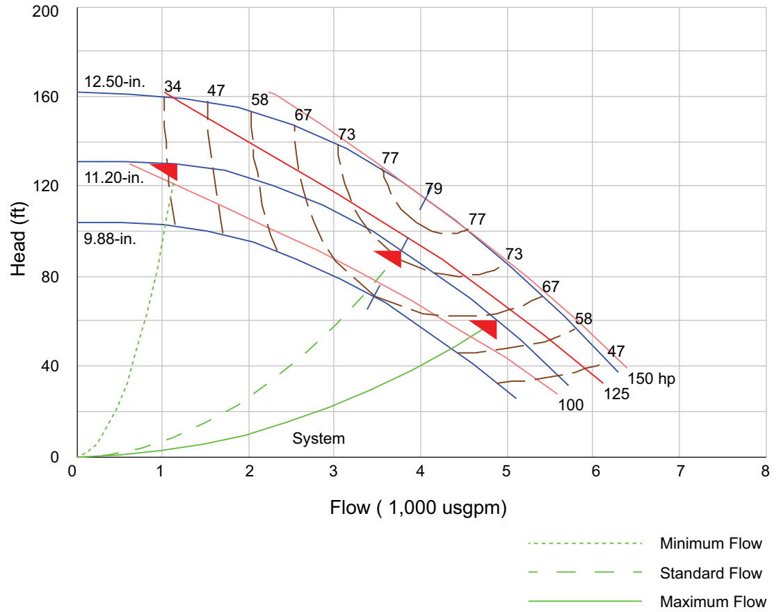
Figure 24. CSPC0125F1 (AA through AF) pump curve
