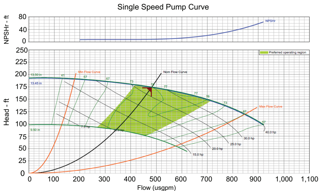
Figure 34. 200 ton ACSA (F0 to F1)/200 ton AXCA (F1) pump curve — single speed
