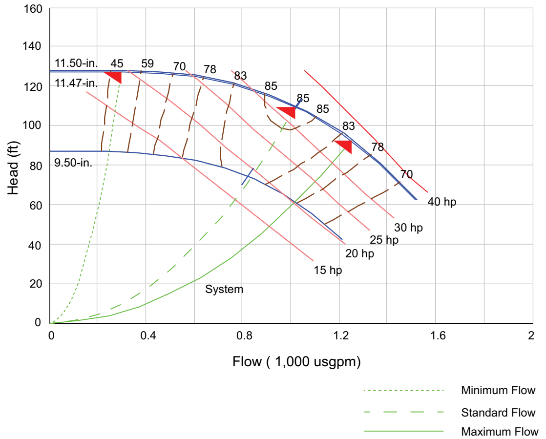
Figure 12. CSPC0040F0 pump curve
