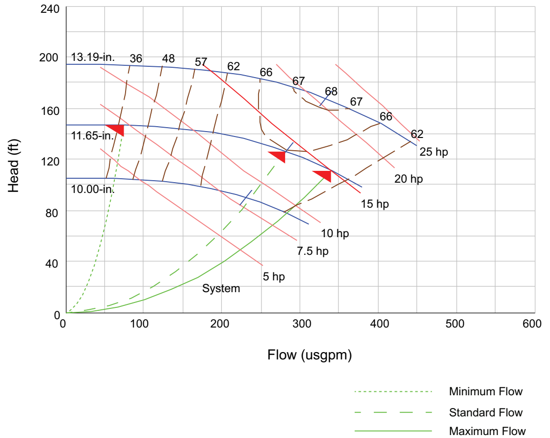
Figure 5. CSPC0015F0 (AM through AR) pump curve
