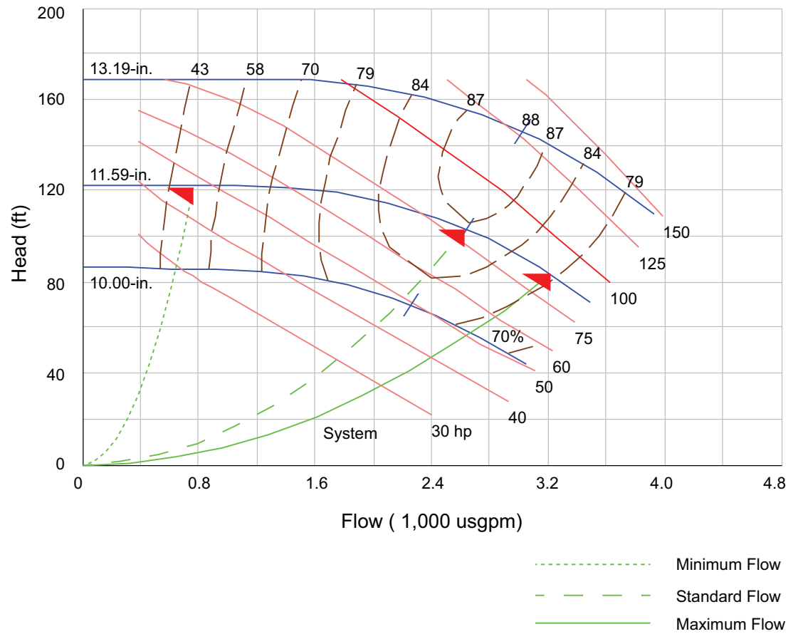
Figure 23. CSPC0100F0 pump curve
