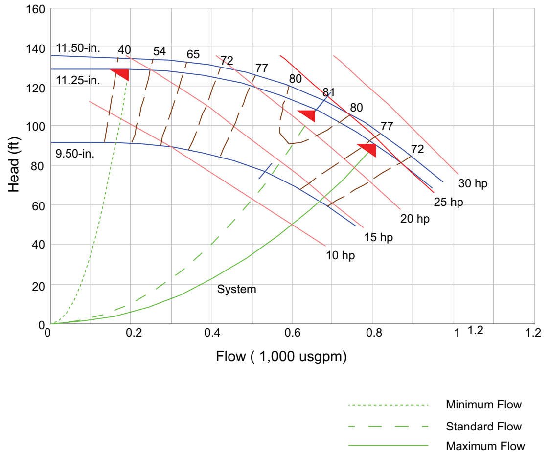
Figure 6. CSPC0025F0 pump curve
