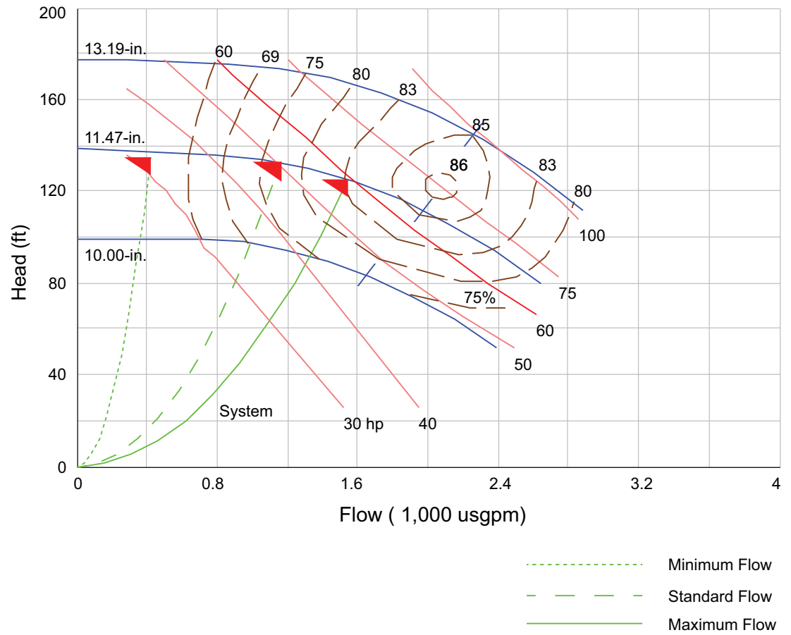
Figure 19. CSPC0060F0 (AM through AU) pump curve
