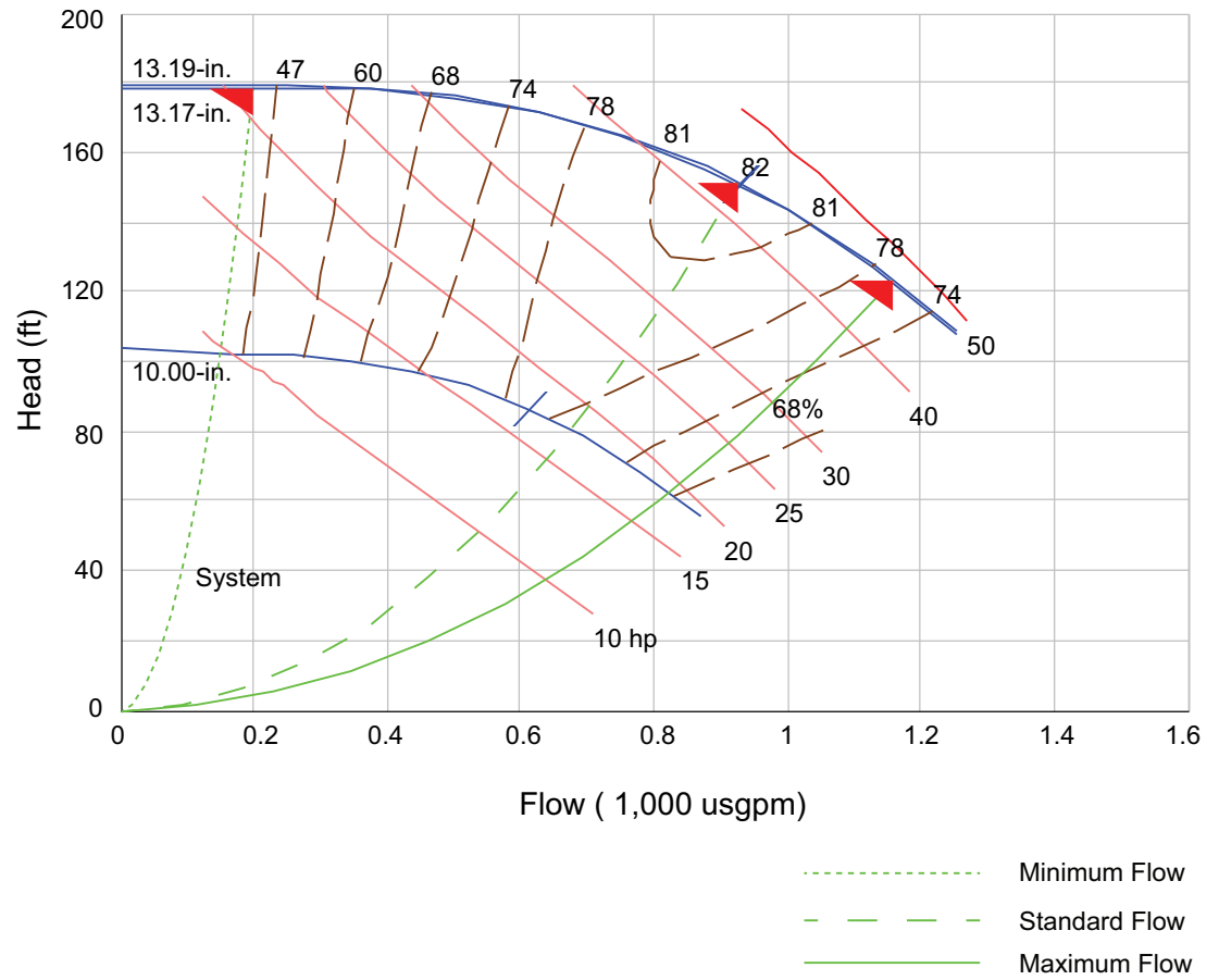
Figure 15. CSPC0050F0 pump curve
