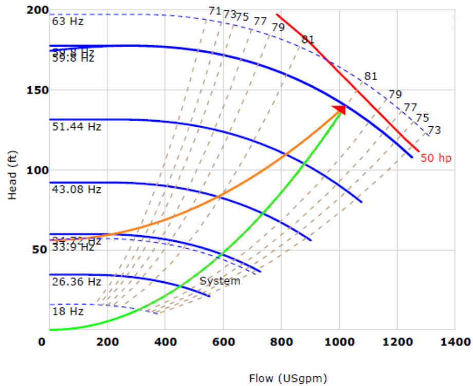
Figure 41. 300 to 440 Ton RTAG multi speed pump curve
