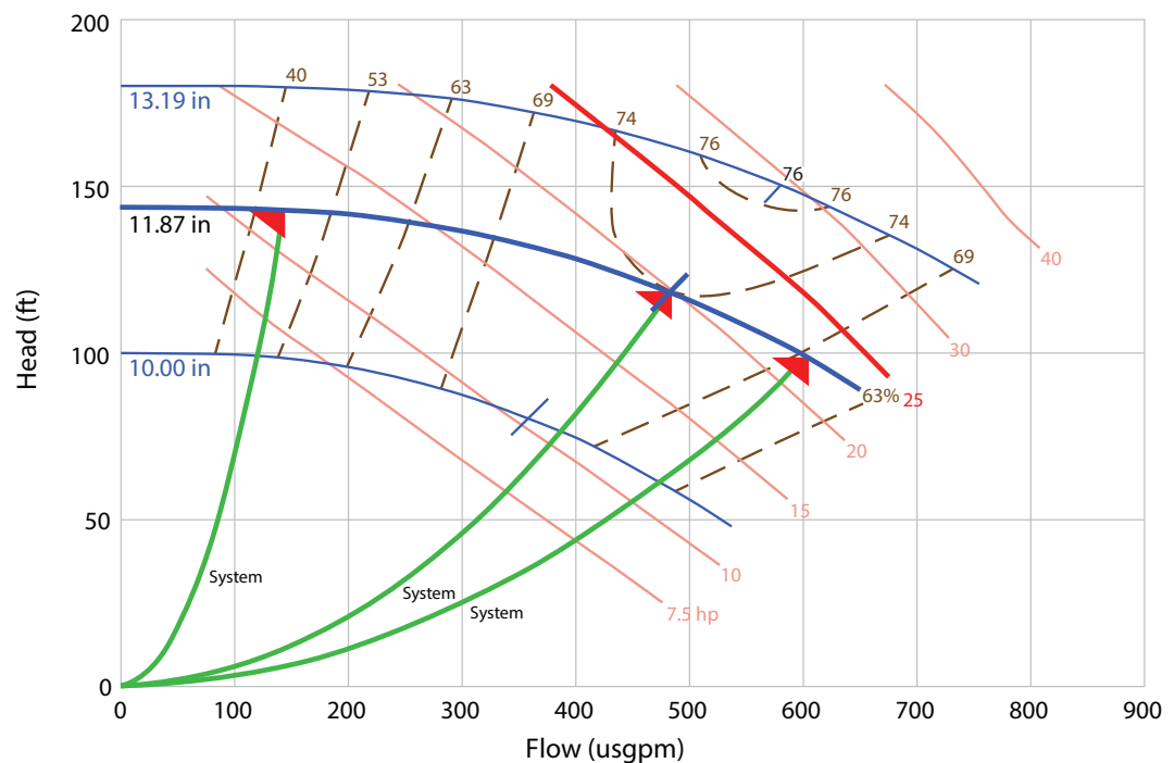
Figure 33. 155/170/200 ton RTAC (F2 to F3) pump curve
