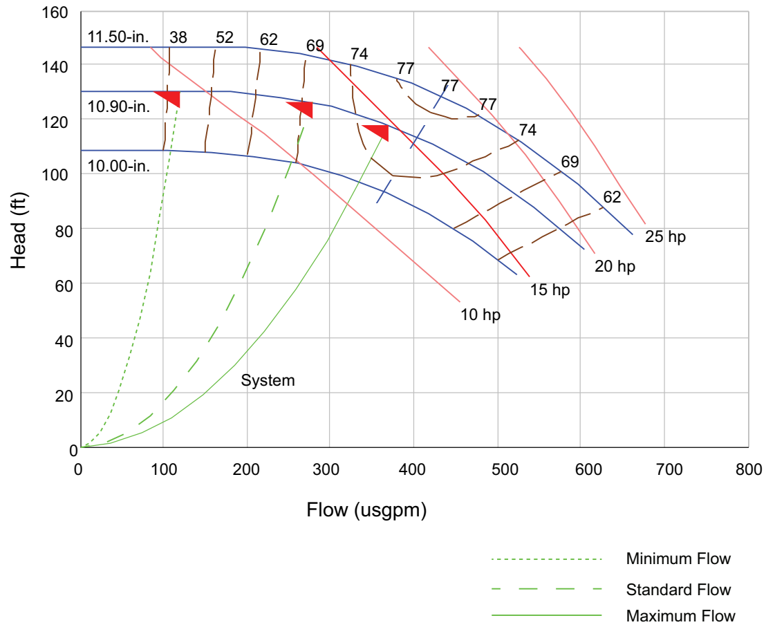
Figure 4. CSPC0015F0 (AA through AL) pump curve
