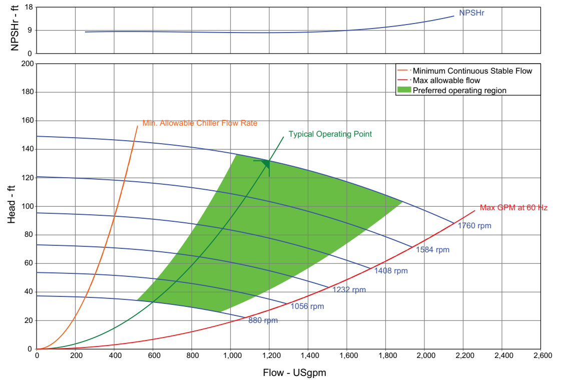
Figure 47. 500 Ton RTAF (F0) multi speed pump curve
