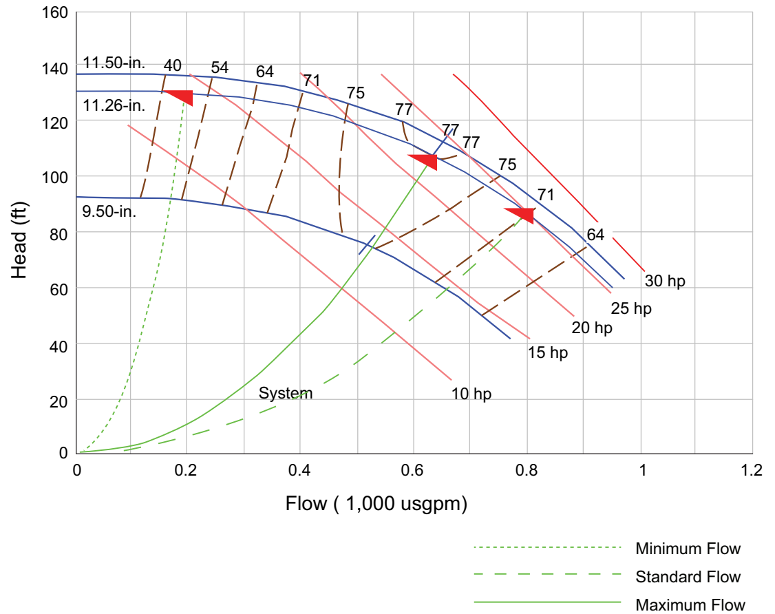
Figure 8. 30 HP pump curve – 1800 rpm
