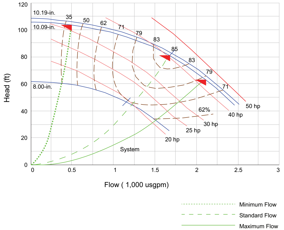
Figure 16. RSPC0050F2 pump curve
