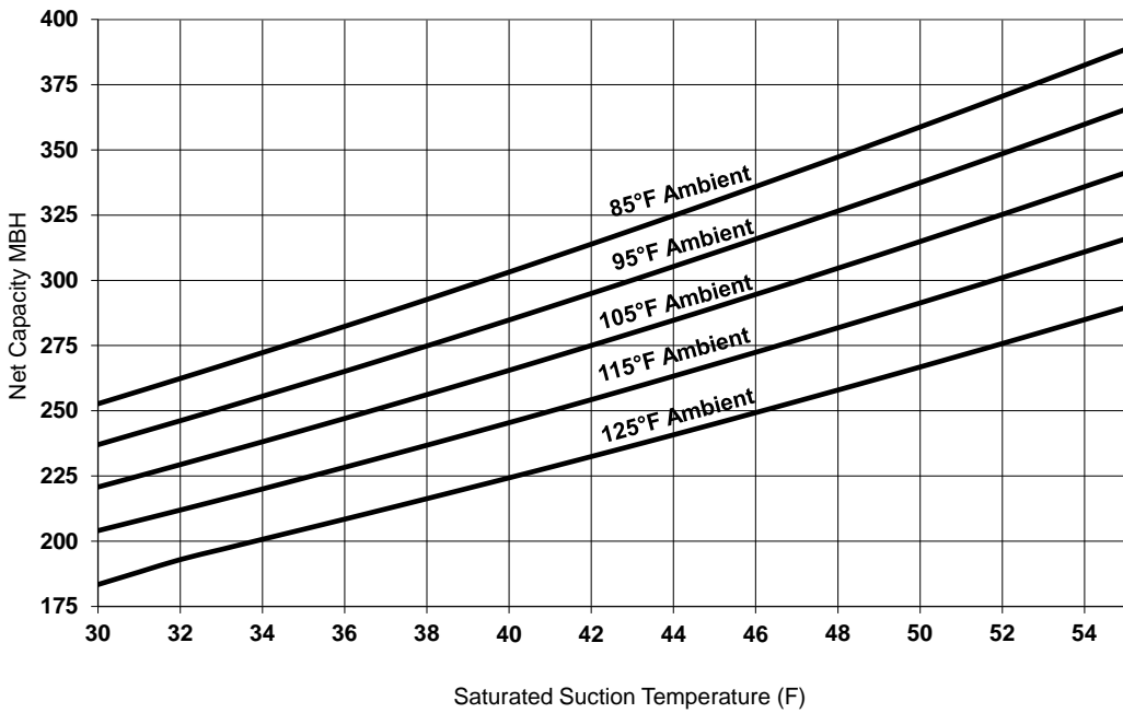
Figure 7. Performance — RA 25 ton 60 Hz (R-454B)
