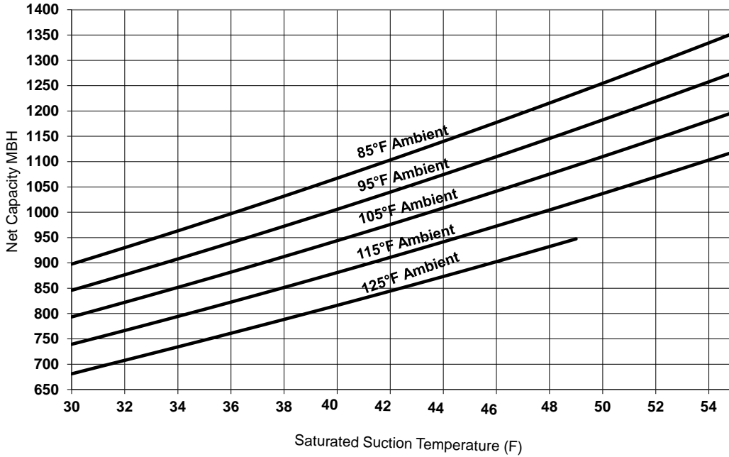
Figure 17. Performance — RA 80 ton 60 Hz (R-454B)
