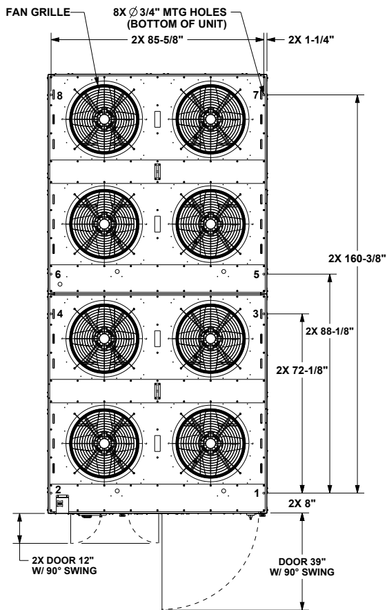
Figure 56. Air-cooled condensing unit — 80 ton
