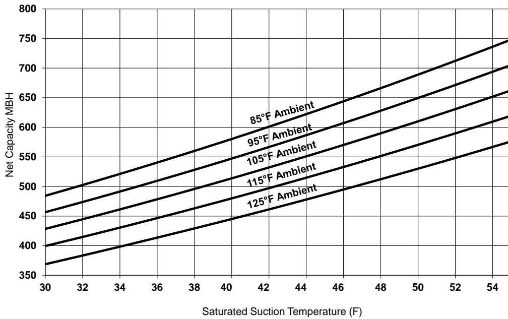
Figure 13. Performance — RA 50 ton 60 Hz (R-454B)
