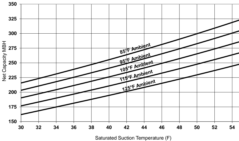
Figure 5. Performance — RA 20 ton 60 Hz (R-454B)
