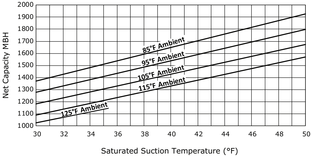
Figure 21. Performance — RA 120 ton 60 Hz (R-454B)
