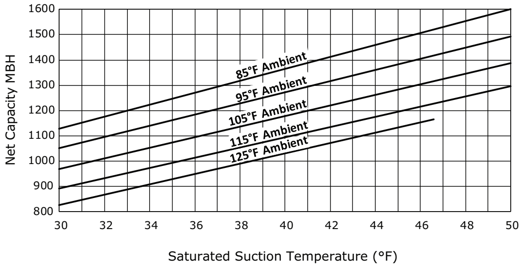
Figure 19. Performance — RA 100 ton 60 Hz (R-454B)
