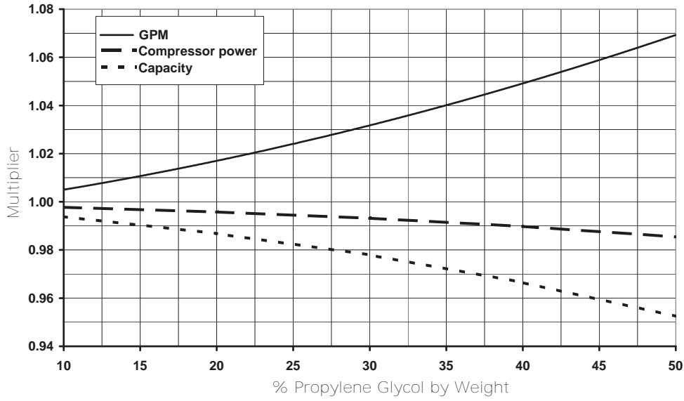
Figure 42. Remote EVP propylene glycol GPM, capacity, compressor power adjustment
