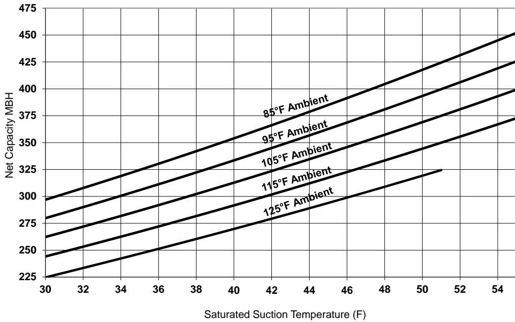
Figure 9. Performance — RA 30 ton 60 Hz (R-454B)
