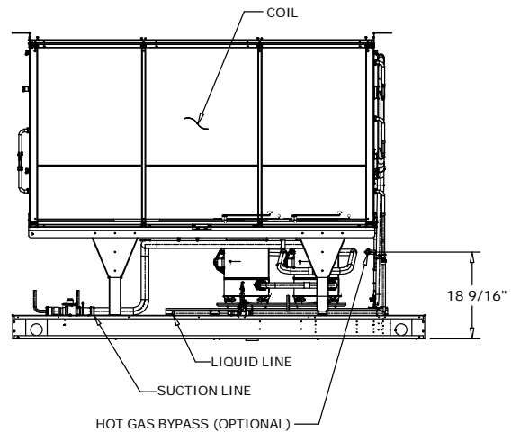
BACK VIEW OF UNIT CONNECTION DRAWING
