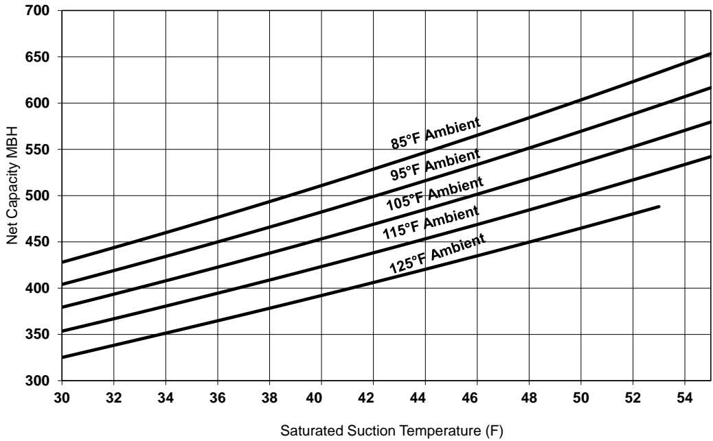
Figure 11. Performance — RA 40 ton 60 Hz (R-454B)
