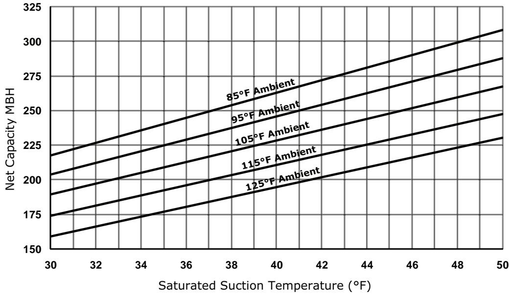
Figure 5. Performance — RA 20 ton 60 Hz (R-454B)
