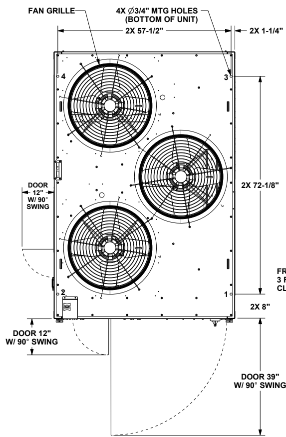
Figure 46. Air-cooled condensing unit — 25 and 30 tons
