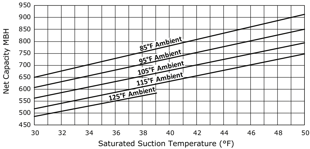
Figure 15. Performance — RA 60 ton 60 Hz (R-454B)
