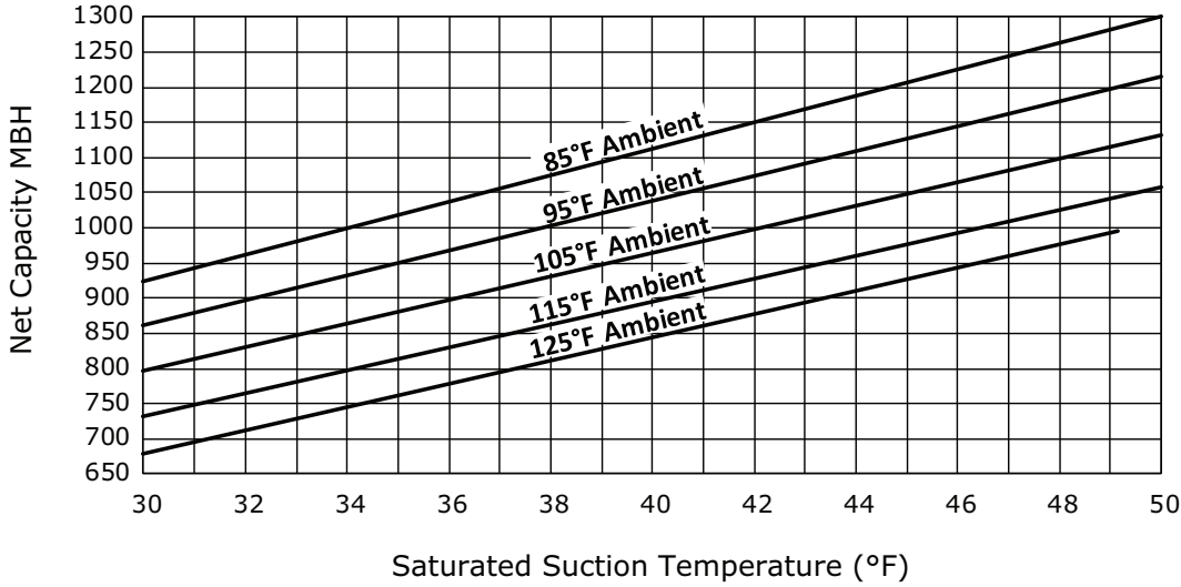
Figure 17. Performance — RA 80 ton 60 Hz (R-454B)
