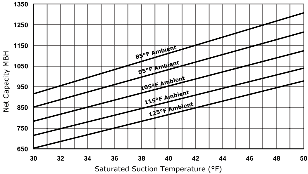
Figure 37. Performance — RA 100 ton 50 Hz (R-454B)
