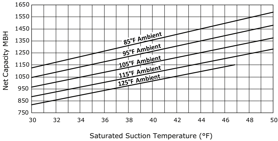
Figure 39. Performance — RA 120 ton 50 Hz (R-454B)
