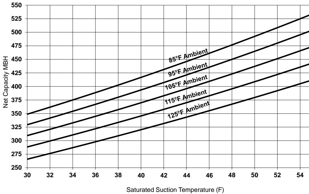
Figure 29. Performance — RA 40 ton 50 Hz (R-454B)
