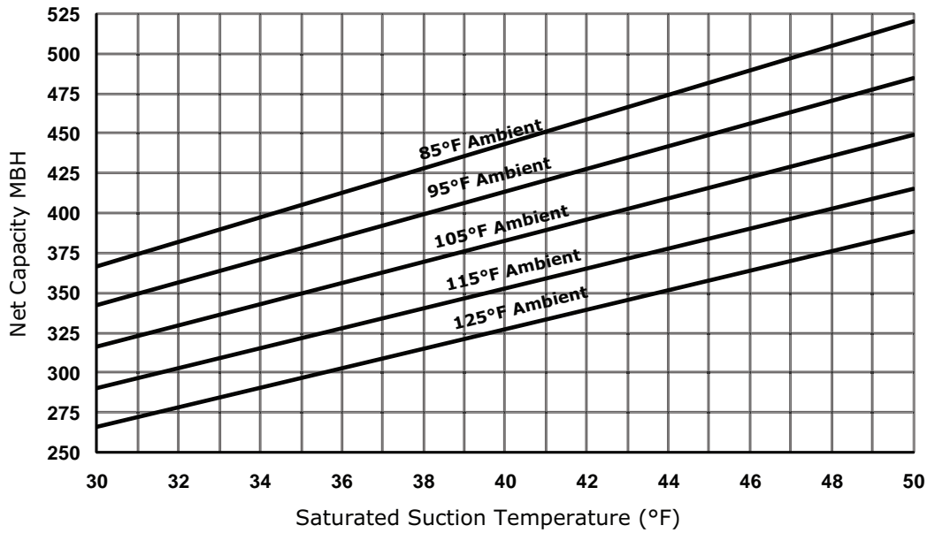
Figure 29. Performance — RA 40 ton 50 Hz (R-454B)
