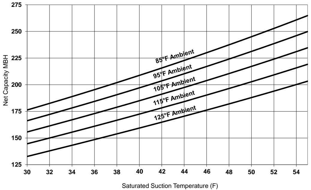
Figure 23. Performance — RA 20 ton 50 Hz (R-454B)
