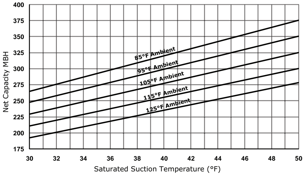
Figure 7. Performance — RA 25 ton 60 Hz (R-454B)
