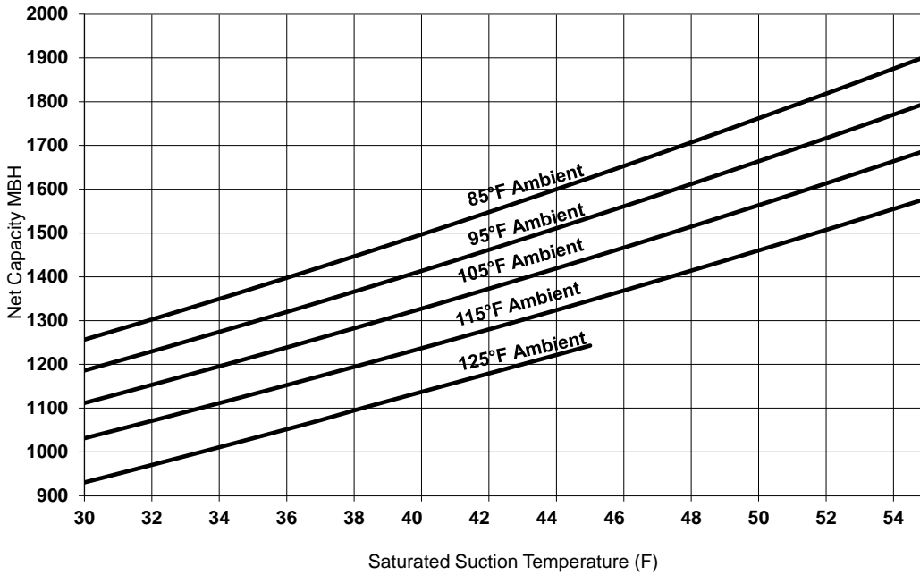
Figure 21. Performance — RA 120 ton 60 Hz (R-454B)
