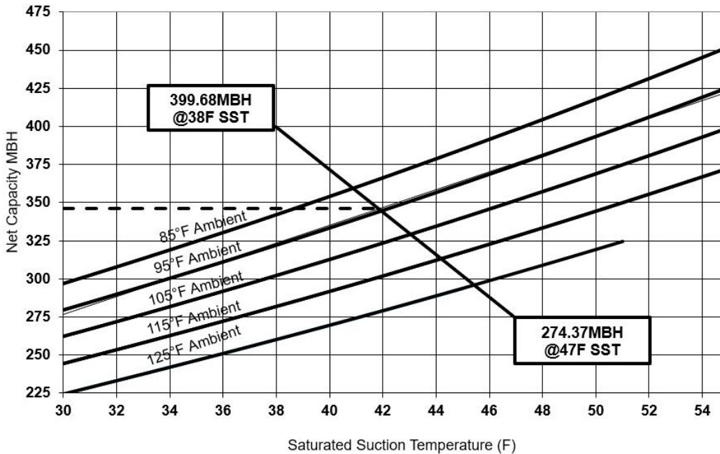
Figure 3. Performance – R-454B 30 ton, 60 Hz
