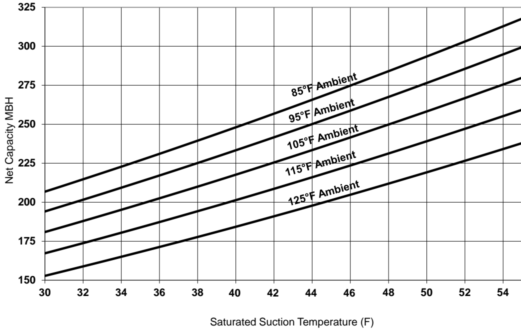
Figure 25. Performance — RA 25 ton 50 Hz (R-454B)
