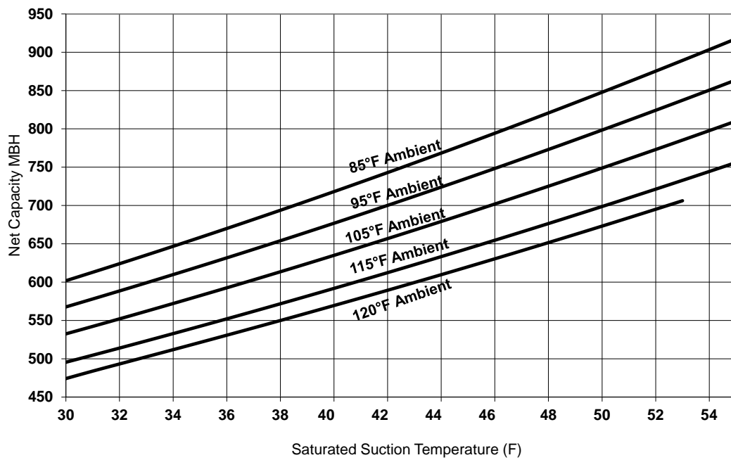
Figure 15. Performance — RA 60 ton 60 Hz (R-454B)
