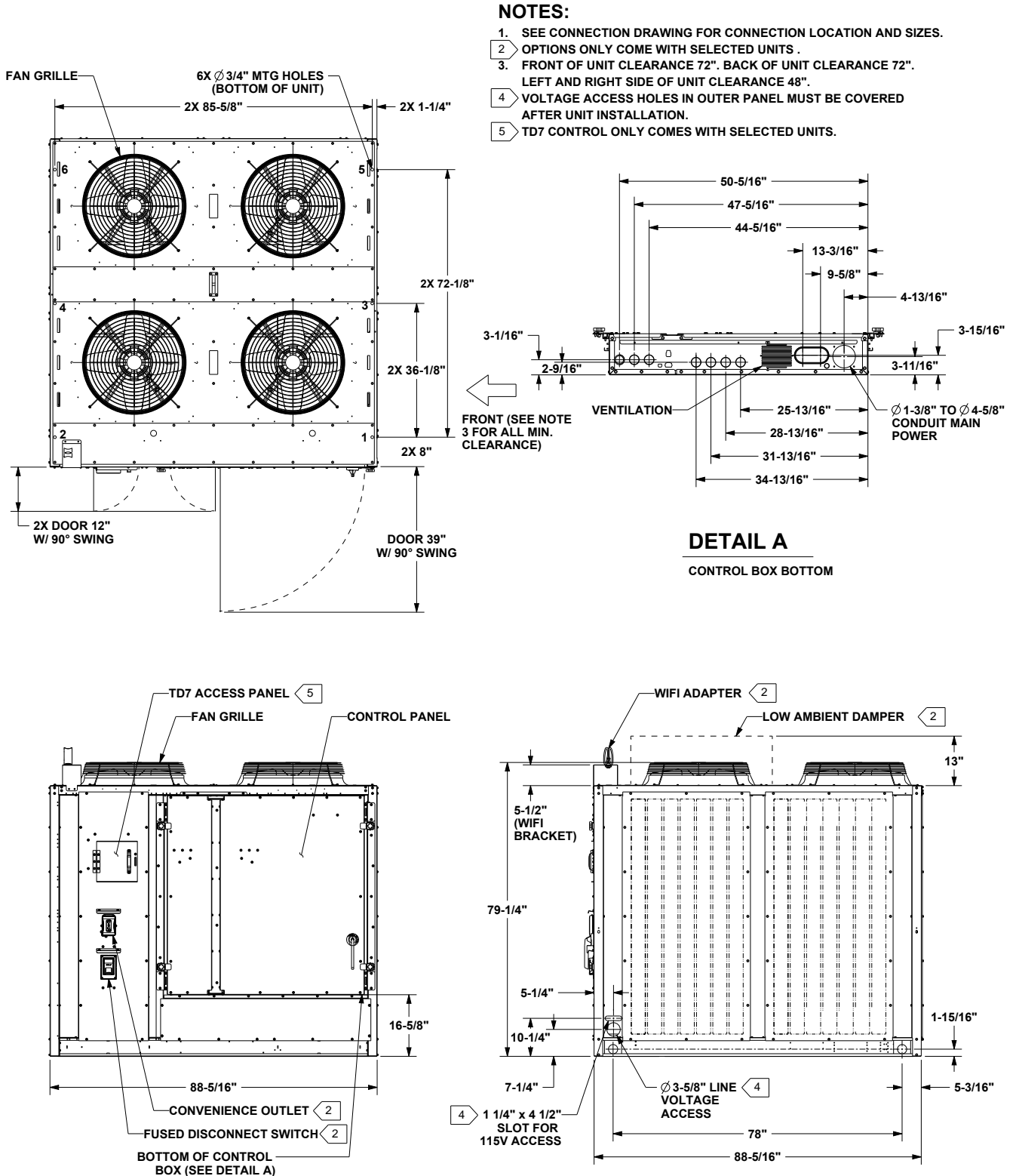
Figure 50. Air-cooled condensing unit — 40 ton
