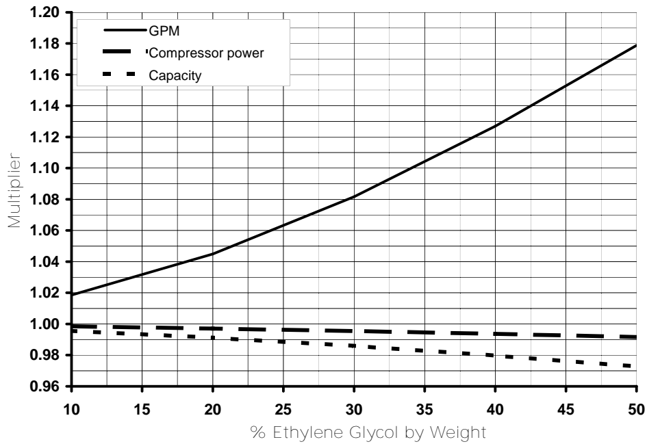
Figure 41. Remote EVP ethylene glycol GPM, capacity, compressor power adjustment
