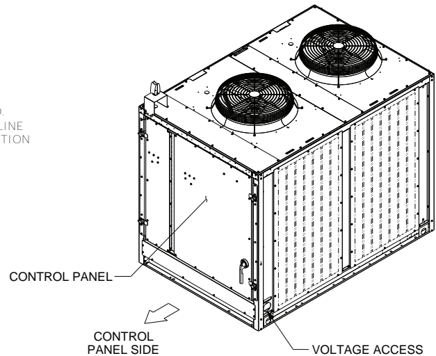
ORIENTATION VIEW OF UNIT ISOMETRIC DRAWING
