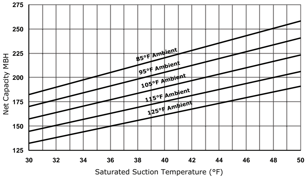
Figure 23. Performance — RA 20 ton 50 Hz (R-454B)
