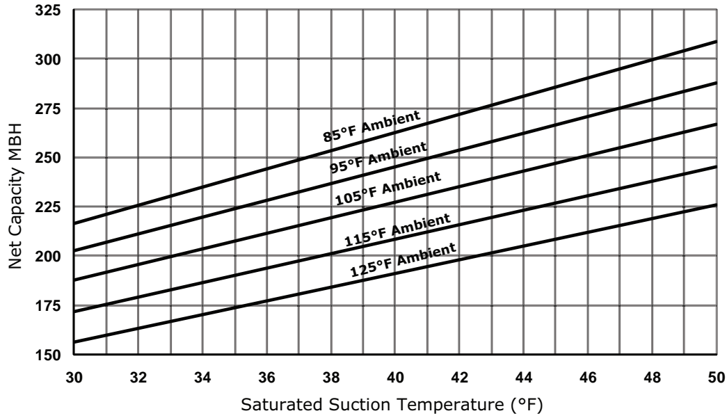
Figure 25. Performance — RA 25 ton 50 Hz (R-454B)
