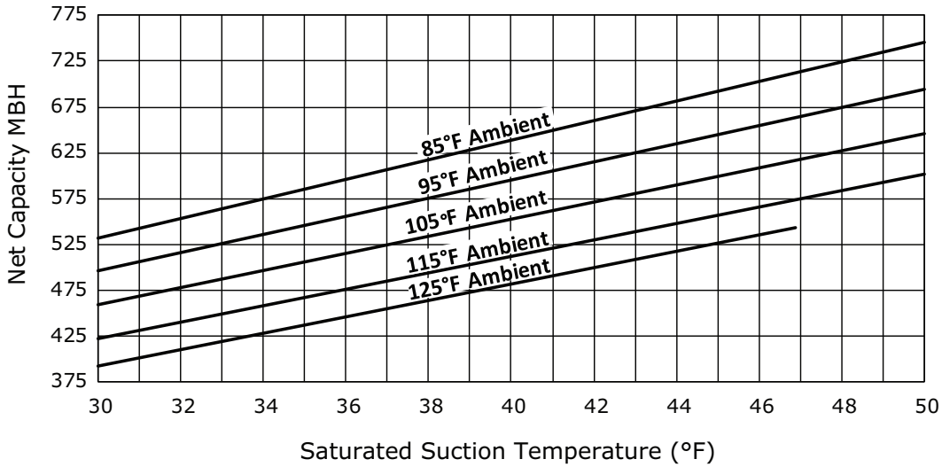
Figure 33. Performance — RA 60 ton 50 Hz (R-454B)
