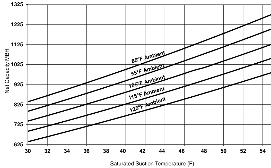
Figure 37. Performance — RA 100 ton 50 Hz (R-454B)
