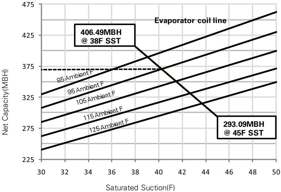
Figure 2. Performance – R-410A 30 ton, 60 Hz
