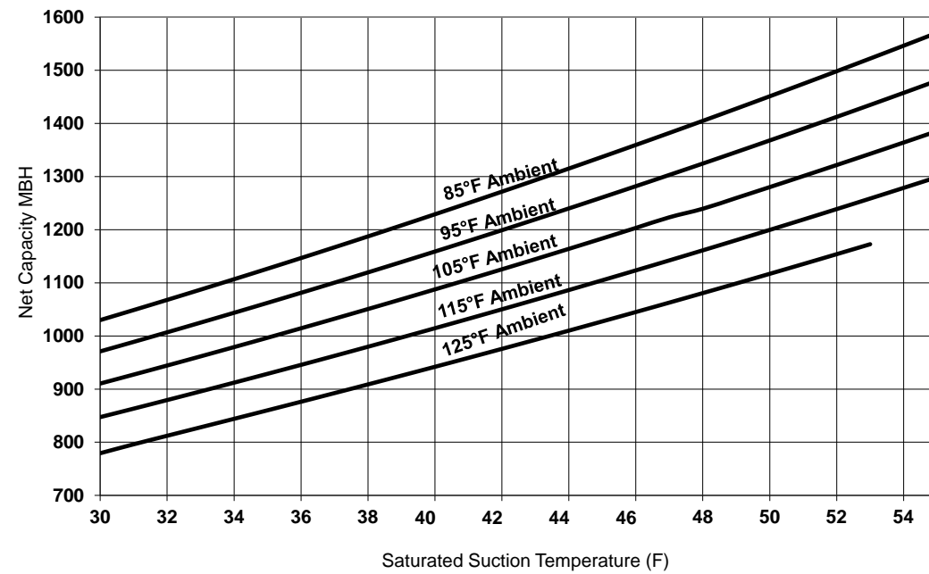
Figure 19. Performance — RA 100 ton 60 Hz (R-454B)
