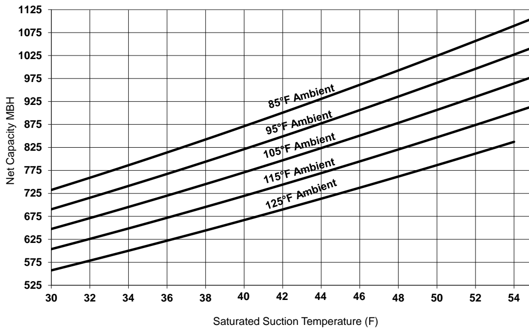
Figure 35. Performance — RA 80 ton 50 Hz (R-454B)
