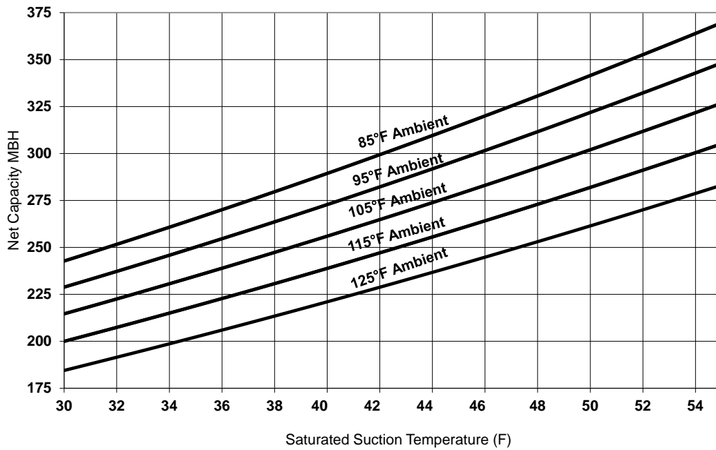
Figure 27. Performance — RA 30 ton 50 Hz (R-454B)
