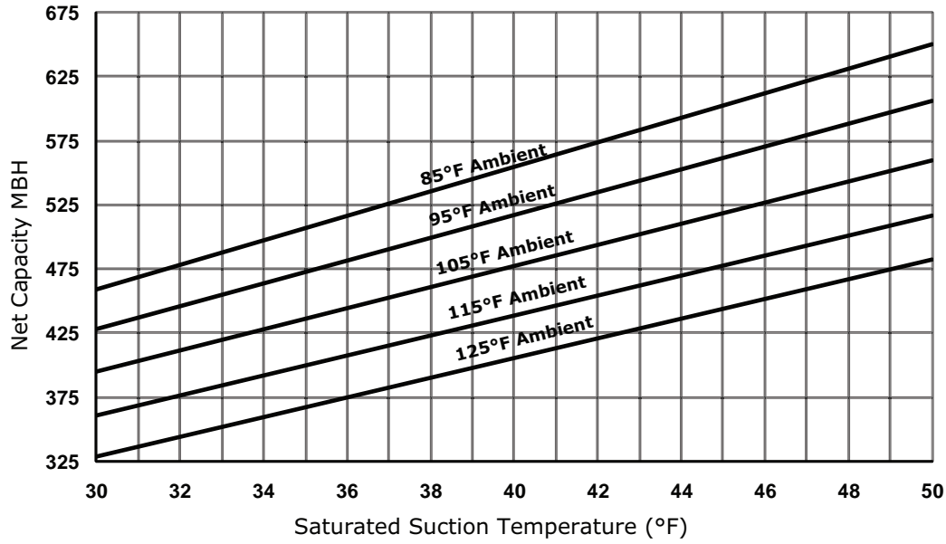
Figure 31. Performance — RA 50 ton 50 Hz (R-454B)
