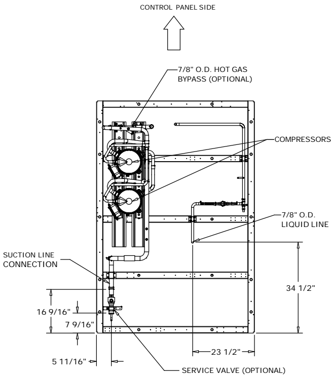
Figure 47. Air-cooled condensing unit connections — 25 and 30 tons (R-410A)
