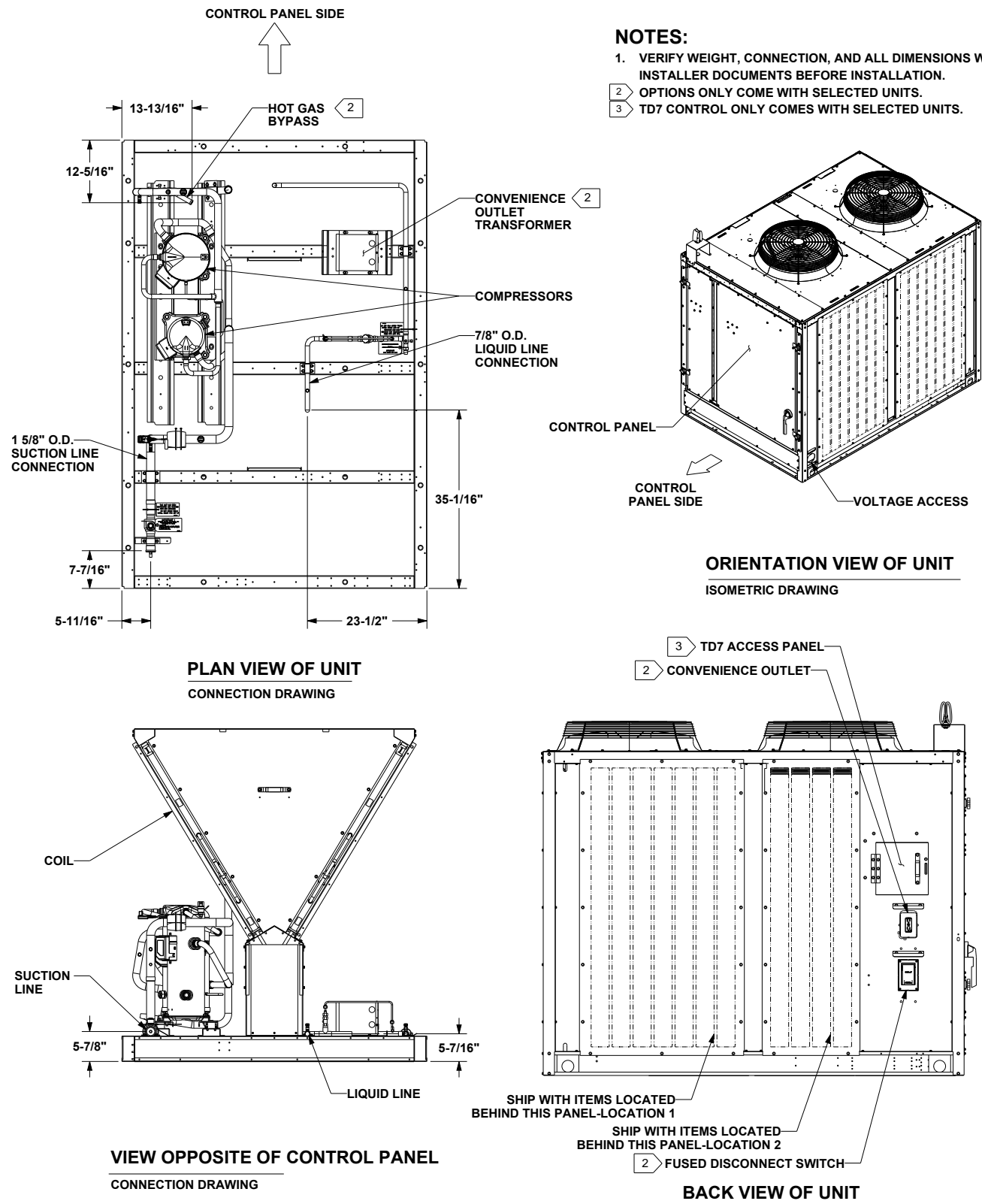
Figure 45. Air-cooled condensing unit connections — 20 ton (R-454B)
