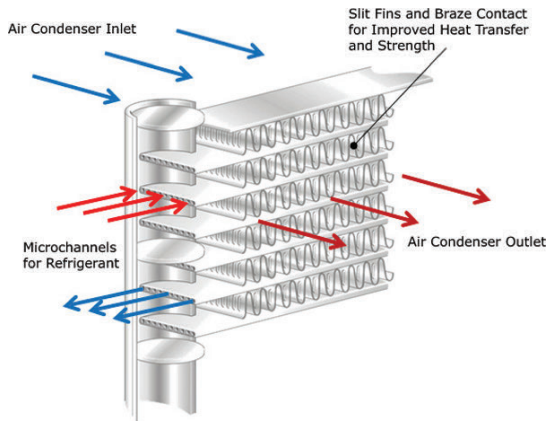
Figure 1. Microchannel condenser coil
