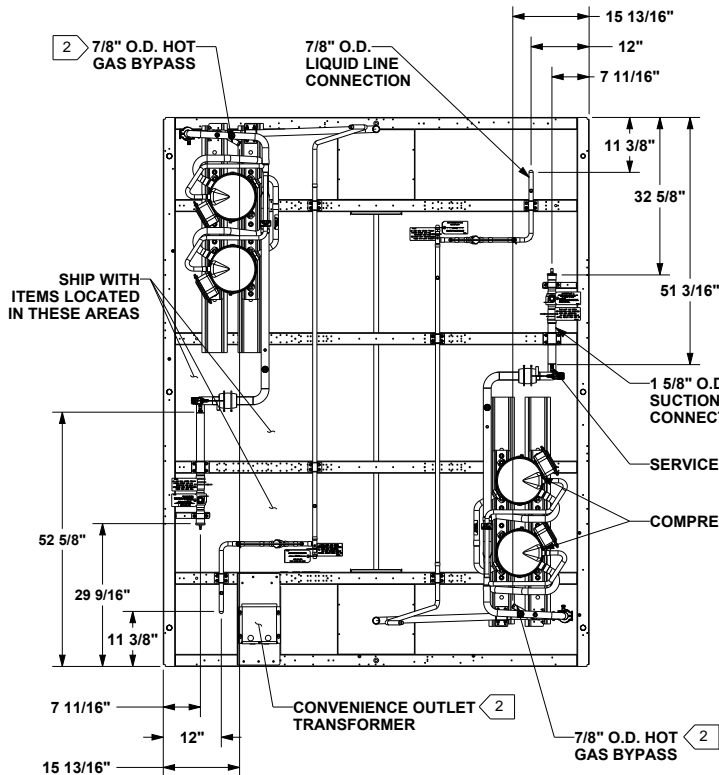
Figure 55. Air-cooled condensing unit connections — 60 ton
