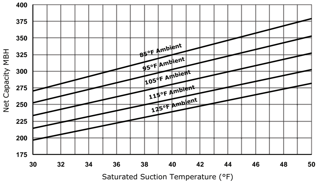
Figure 27. Performance — RA 30 ton 50 Hz (R-454B)
