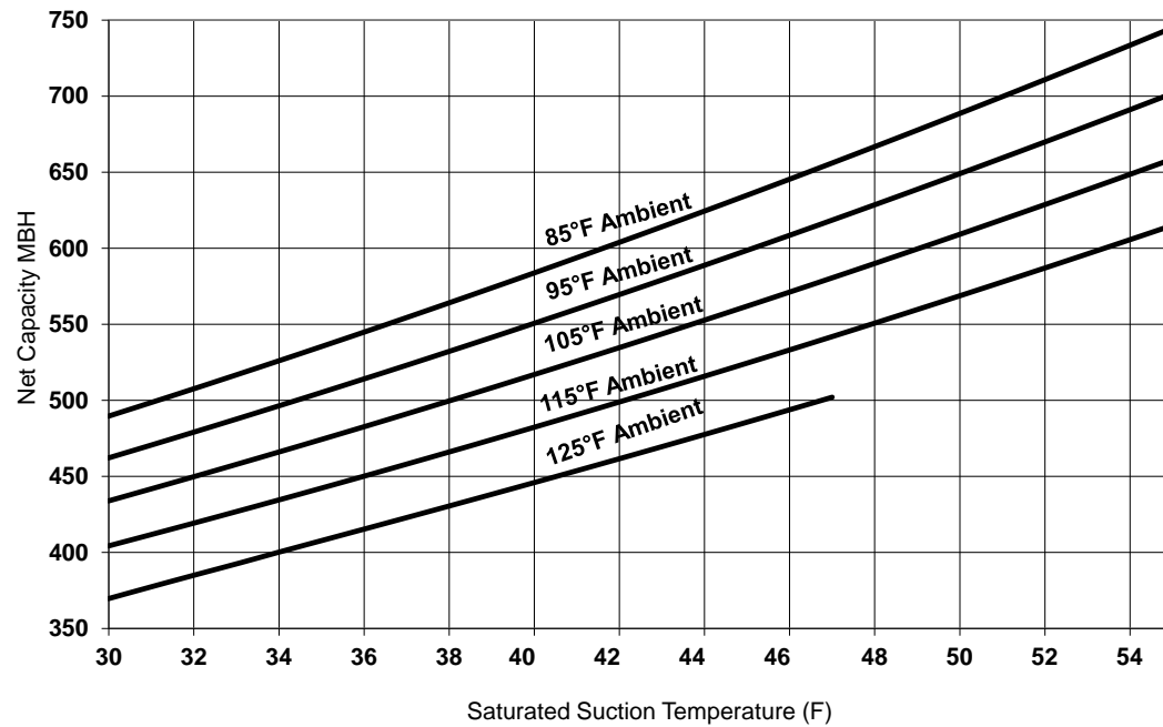
Figure 33. Performance — RA 60 ton 50 Hz (R-454B)
