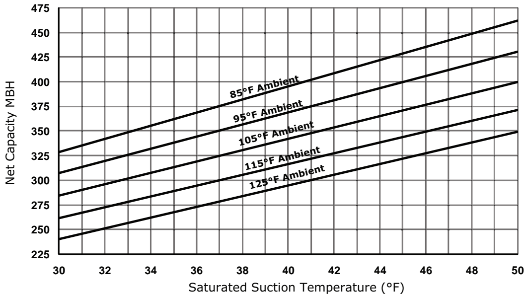
Figure 9. Performance — RA 30 ton 60 Hz (R-454B)
