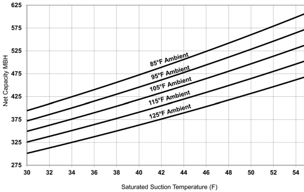
Figure 31. Performance — RA 50 ton 50 Hz (R-454B)
