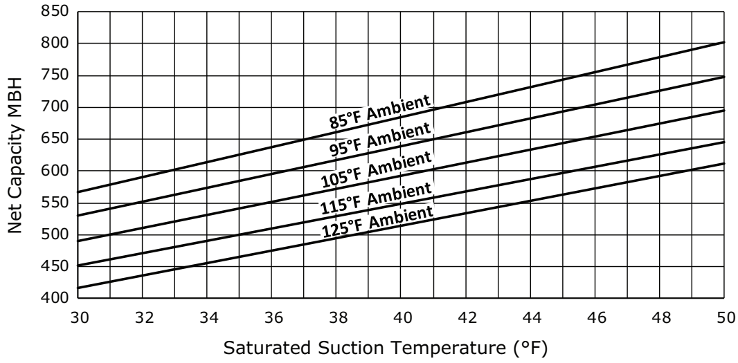
Figure 13. Performance — RA 50 ton 60 Hz (R-454B)
