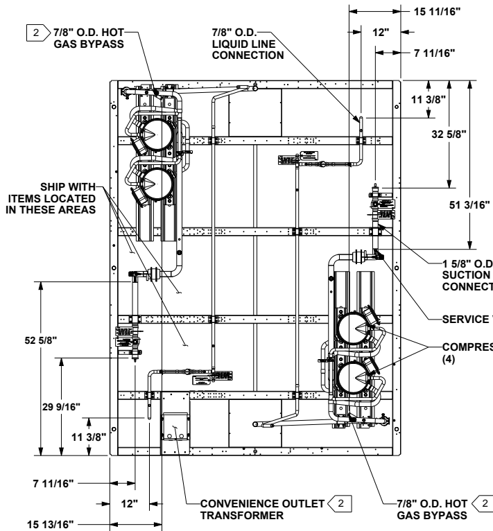
Figure 53. Air-cooled condensing unit connections — 50 ton
