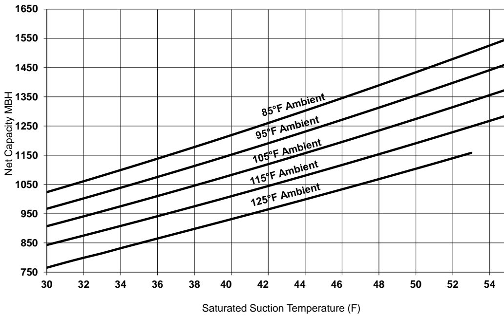
Figure 39. Performance — RA 120 ton 50 Hz (R-454B)
