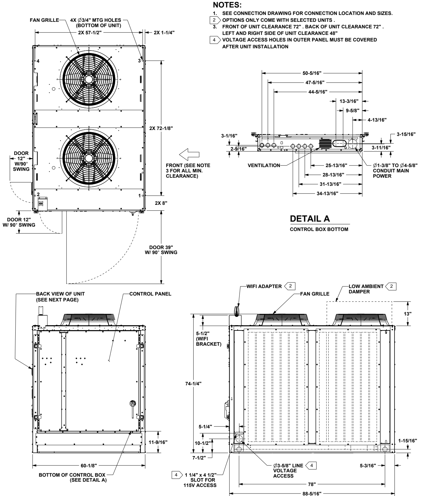
Figure 43. Air-cooled condensing unit — 20 ton
