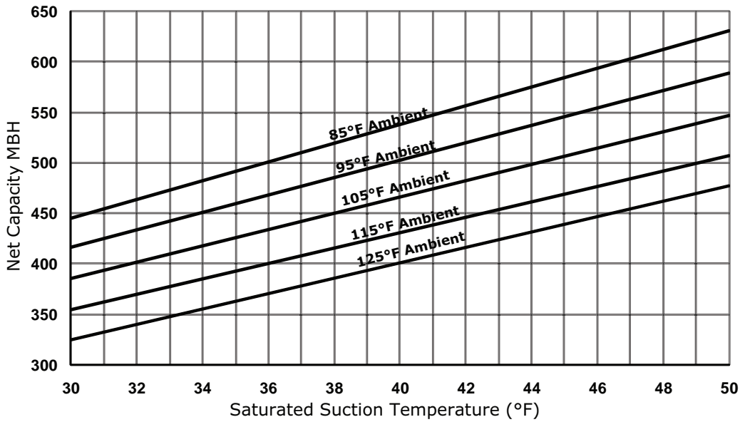
Figure 11. Performance — RA 40 ton 60 Hz (R-454B)
