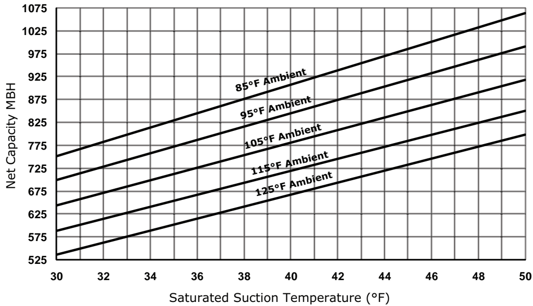
Figure 35. Performance — RA 80 ton 50 Hz (R-454B)
