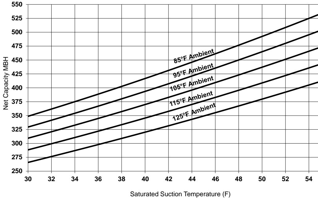
Figure 14. Performance — RA 40 ton 50 Hz
