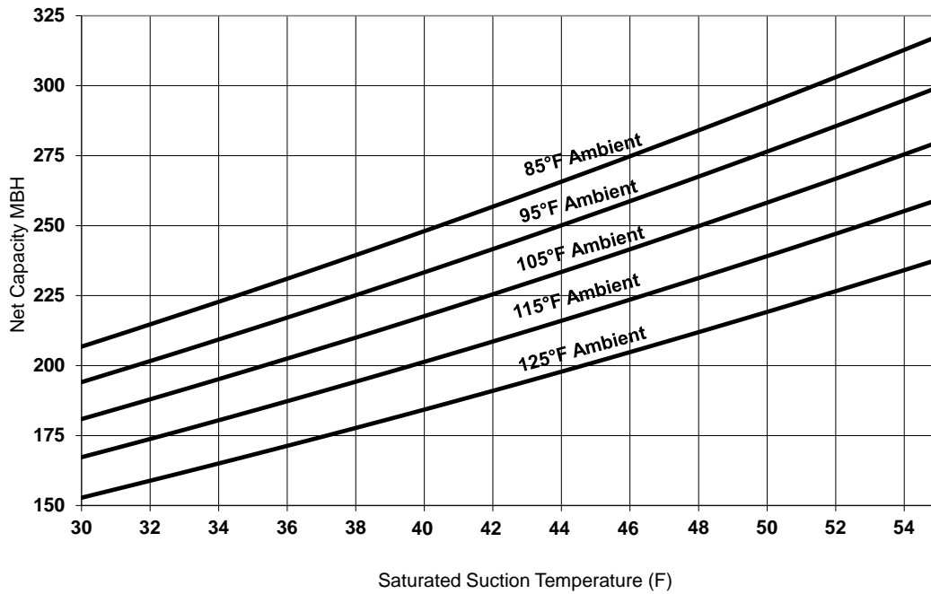
Figure 13. Performance — RA 30 ton 50 Hz
