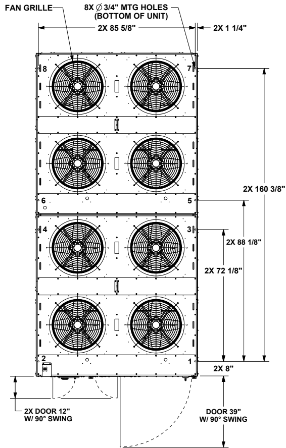
Figure 34. Air-cooled condensing unit — 80 ton
