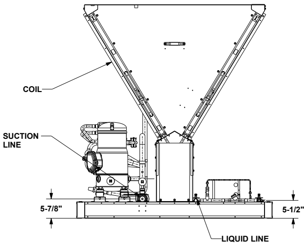
VIEW OPPOSITE OF CONTROL PANEL CONNECTION DRAWING
