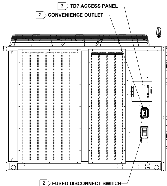
BACK VIEW OF UNIT
