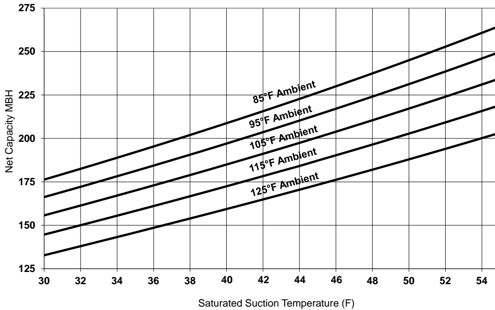
Figure 11. Performance — RA 20 ton 50 Hz
