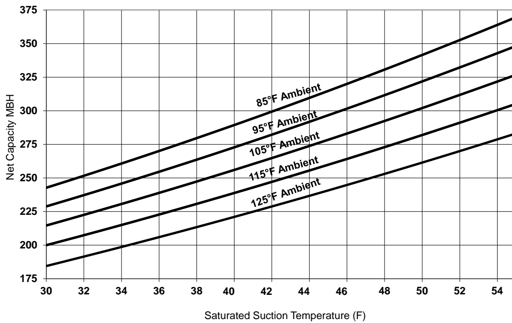
Figure 13. Performance — RA 30 ton 50 Hz
