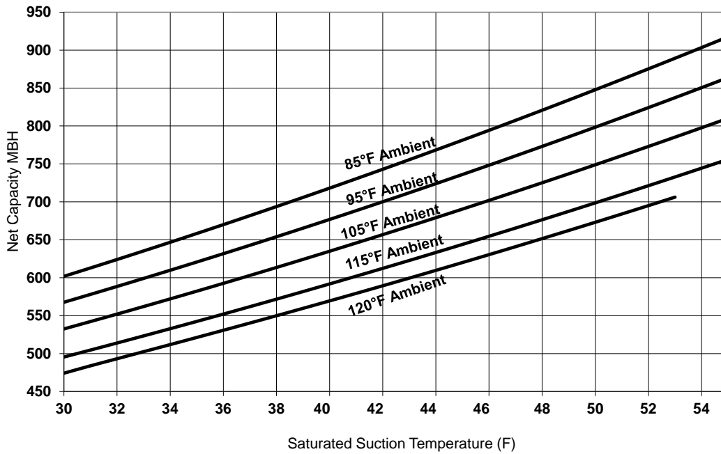
Figure 7. Performance — RA 60 ton 60 Hz
