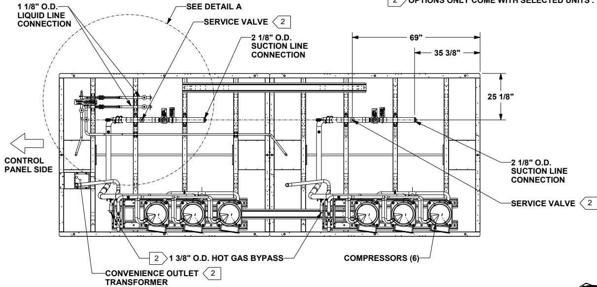
PLAN VIEW OF UNIT CONNECTION DRAWING
