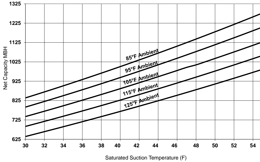
Figure 19. Performance — RA 120 ton 50 Hz
