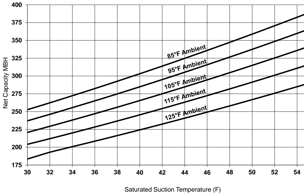
Figure 3. Performance — RA 25 ton 60 Hz
