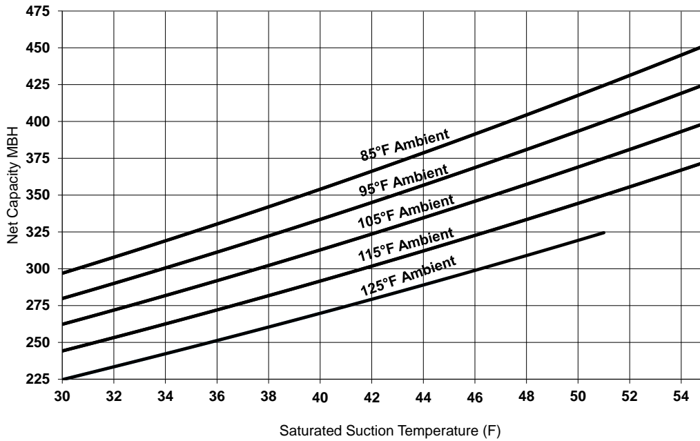
Figure 5. Performance — RA 40 ton 60 Hz
