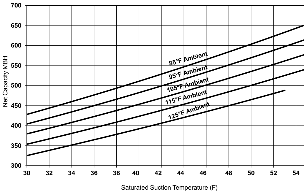
Figure 5. Performance — RA 40 ton 60 Hz
