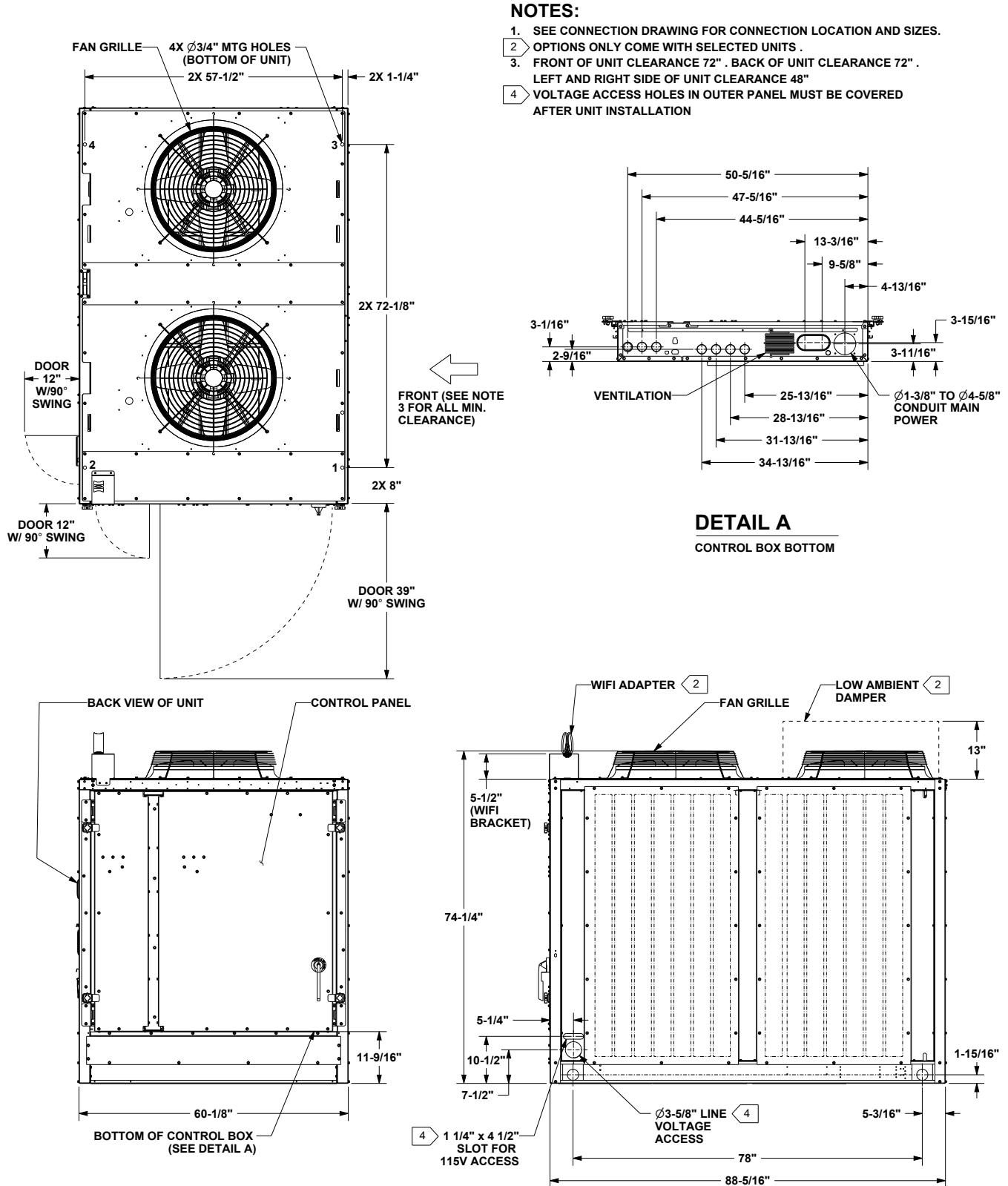
Figure 23. Air-cooled condensing unit — 20 ton
