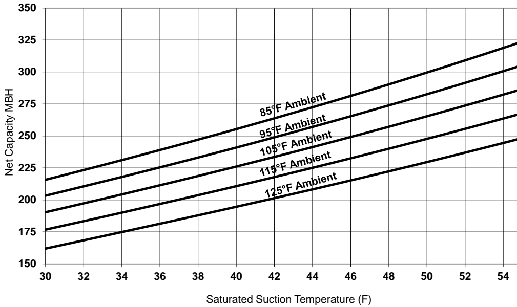
Figure 3. Performance — RA 25 ton 60 Hz
