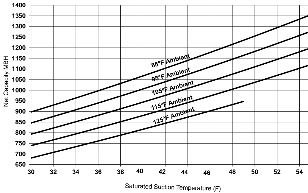
Figure 9. Performance — RA 100 ton 60 Hz
