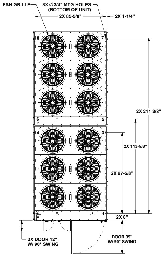
Figure 36. Air-cooled condensing unit — 100 and 120 tons
