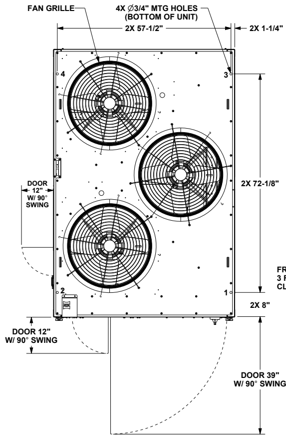
Figure 25. Air-cooled condensing unit — 25 and 30 tons
