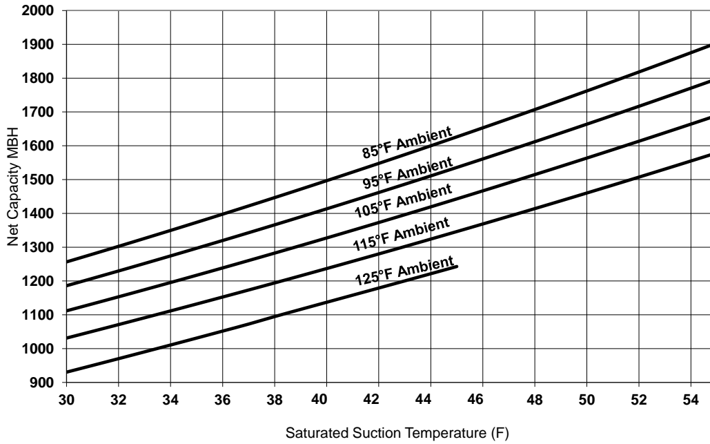
Figure 10. Performance — RA 120 ton 60 Hz
