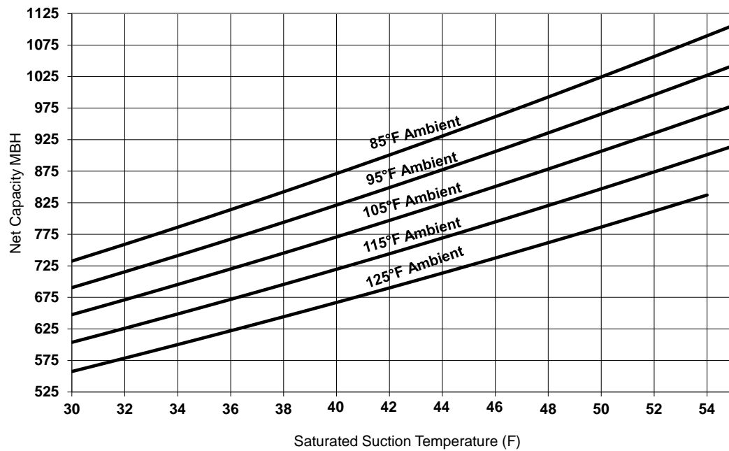
Figure 17. Performance — RA 80 ton 50 Hz
