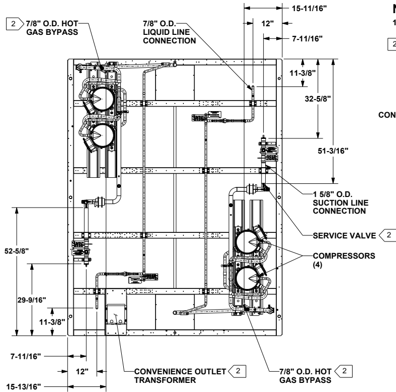
Figure 31. Air-cooled condensing unit connections — 50 ton
