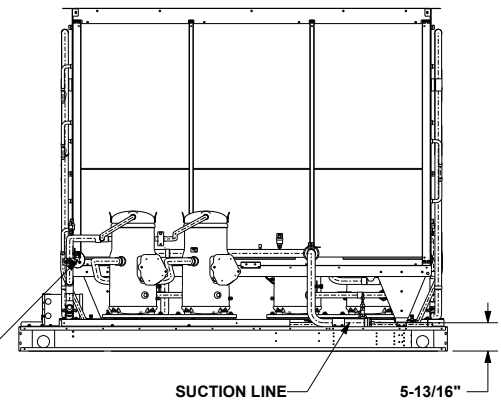
FRONT OF UNIT CONNECTION DRAWING
