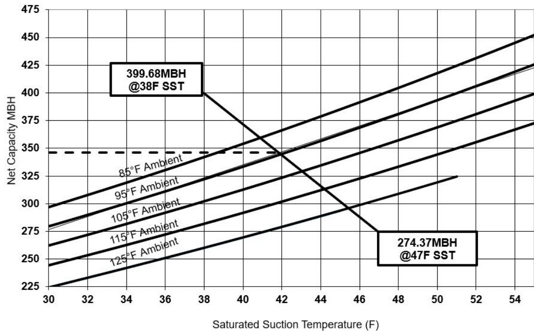
Figure 1. Performance - RAUK 30 ton 60 Hz
