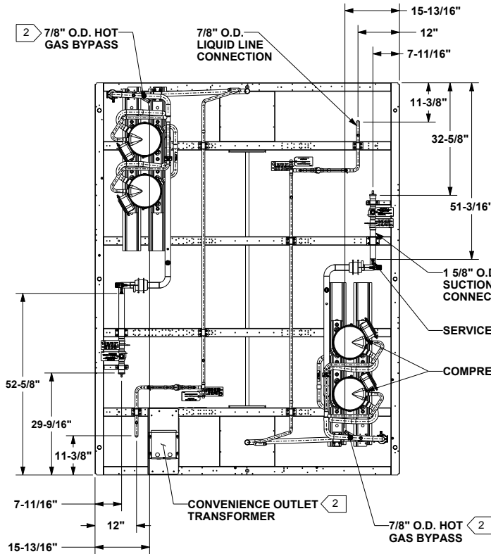
Figure 33. Air-cooled condensing unit connections — 60 ton
