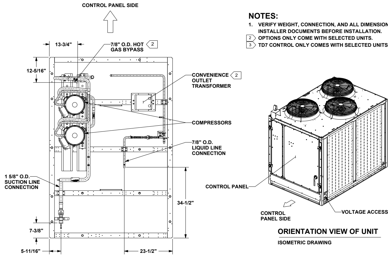
PLAN VIEW OF UNIT CONNECTION DRAWING
