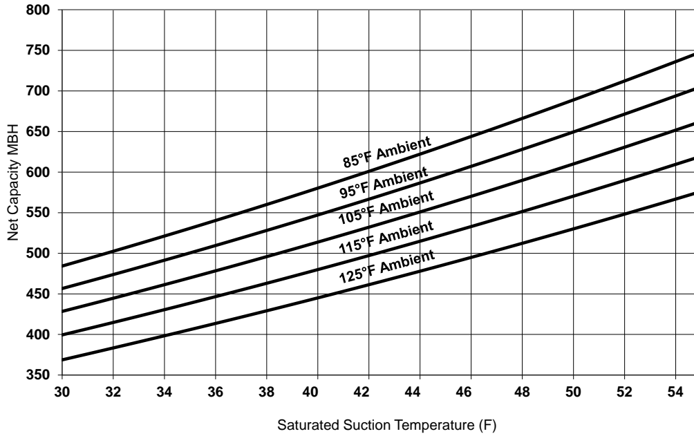
Figure 7. Performance — RA 60 ton 60 Hz
