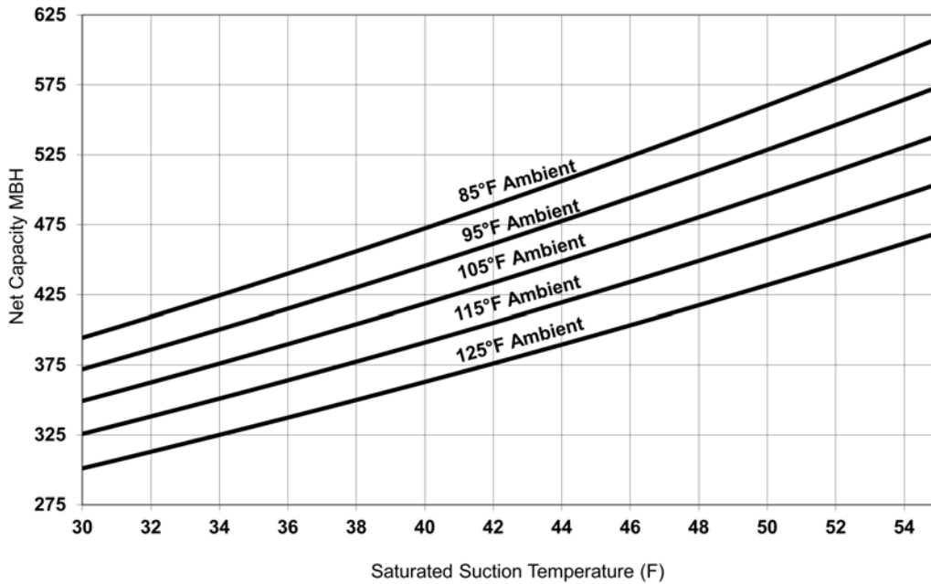
Figure 15. Performance — RA 50 ton 50 Hz
