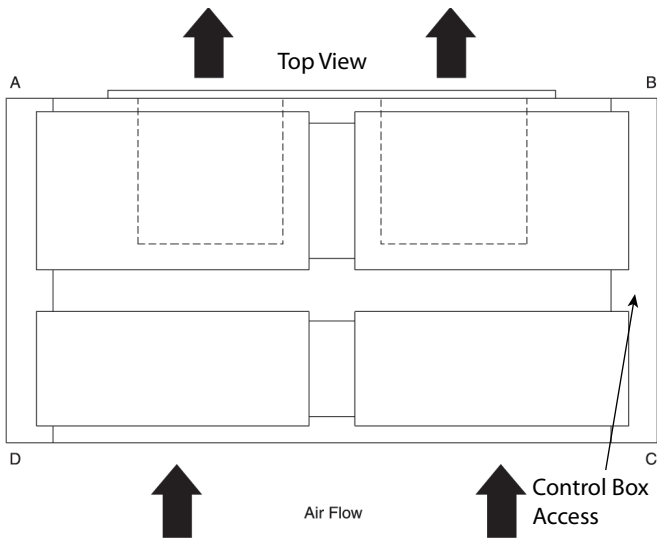
Figure 48. Horizontal — TWE150, 180, 240, 300
