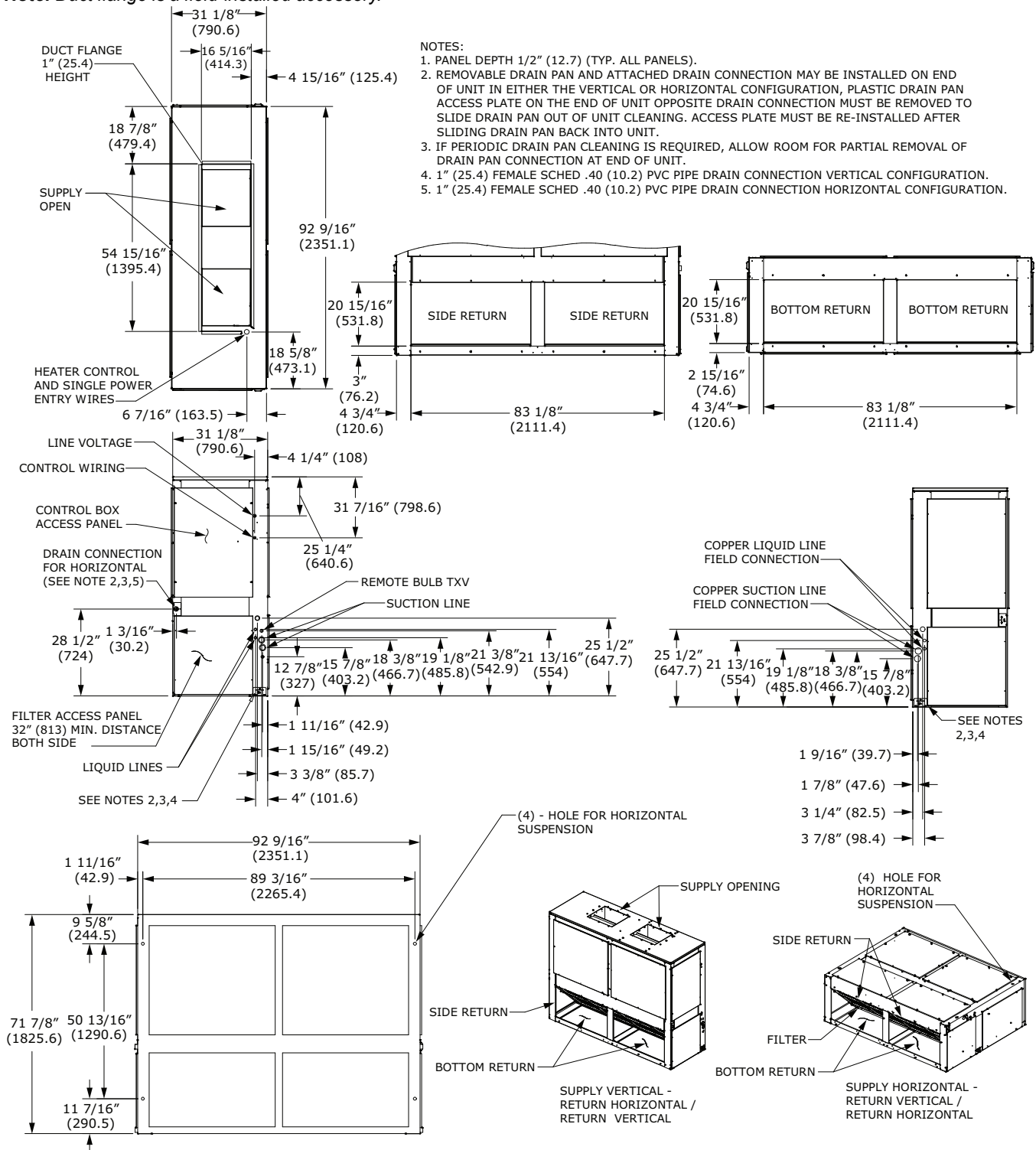
Figure 33. 20 and 25 ton air handler, dual circuit – in. (mm)
