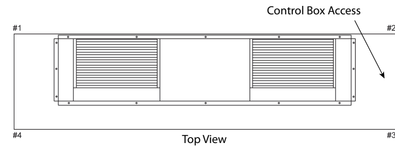
Figure 47. Horizontal — TWE060, 072, 090, 120
