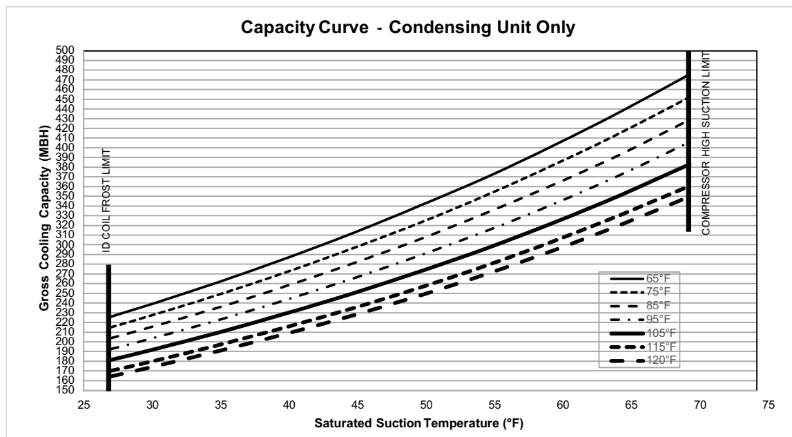
Figure 17. TWA240K*D capacity curves
