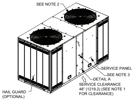
Figure 25. 25 ton condensing, manifolded compressor – in (mm)
