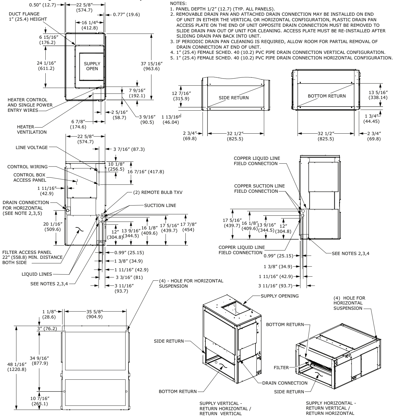
Figure 27. 5 ton air handler, dual circuit – in. (mm)
