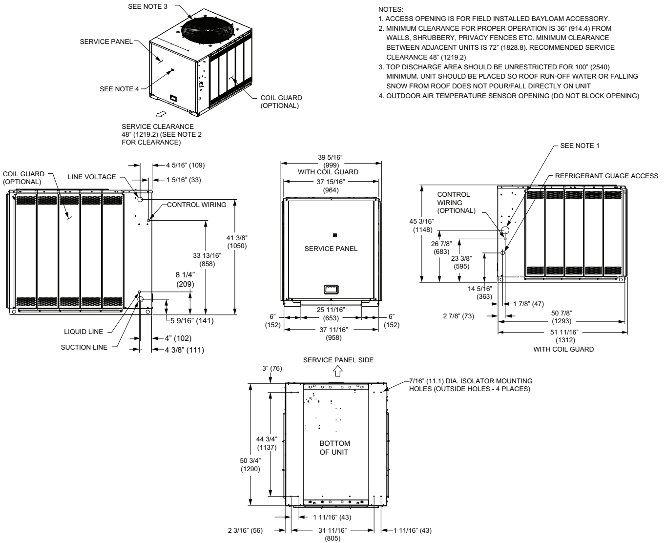
Figure 22. 10 ton heat pump, single compressor – in (mm)
