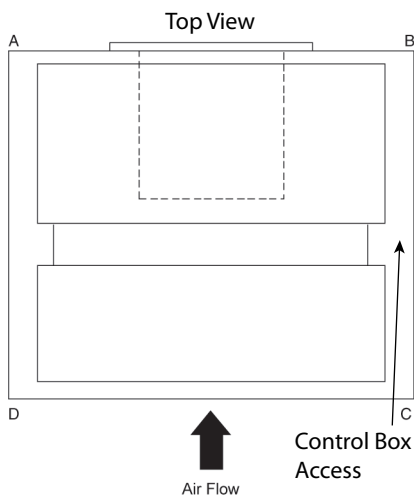
Figure 47. Horizontal — TWE060, 072, 090, 120
