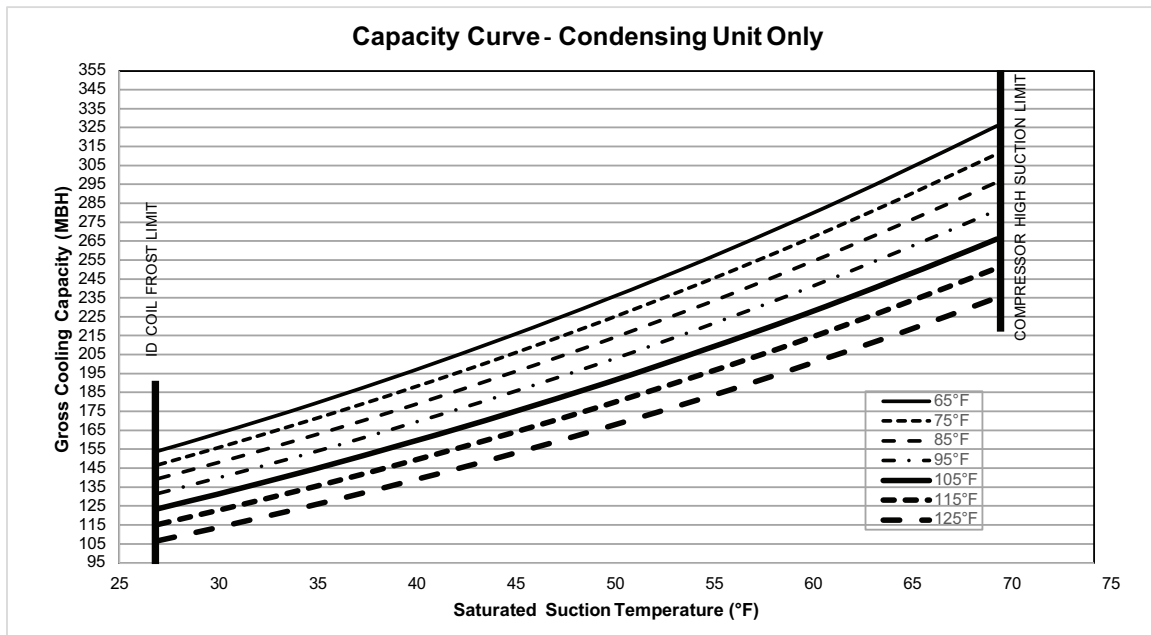
Figure 16. TWA180K*D capacity curves
