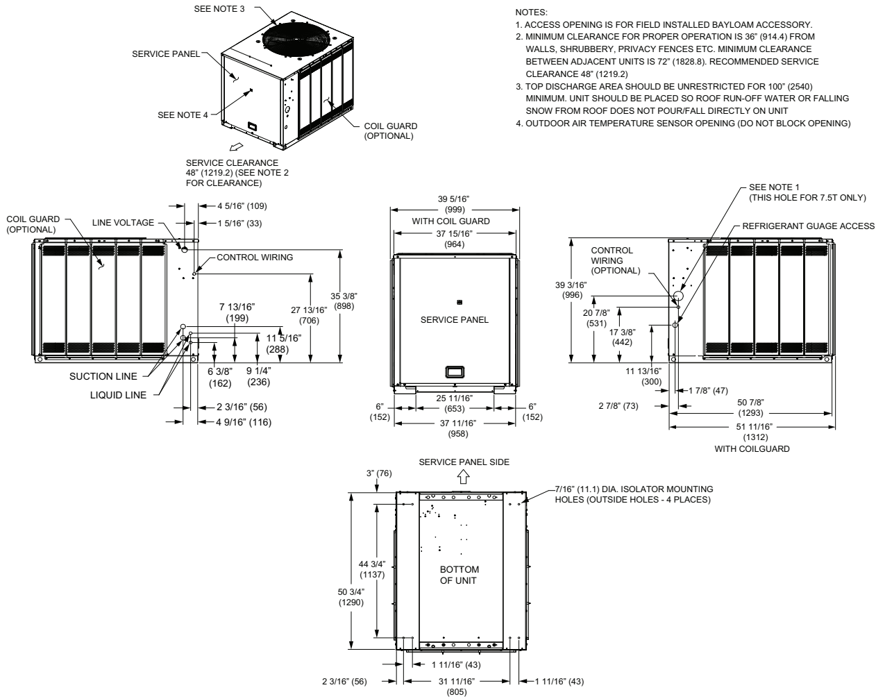
Figure 21. 6-7.5 ton heat pump, dual compressor – in (mm)
