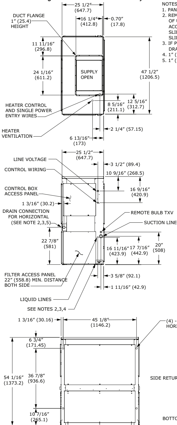
Figure 28. 7.5 ton air handler, single circuit – in. (mm)
