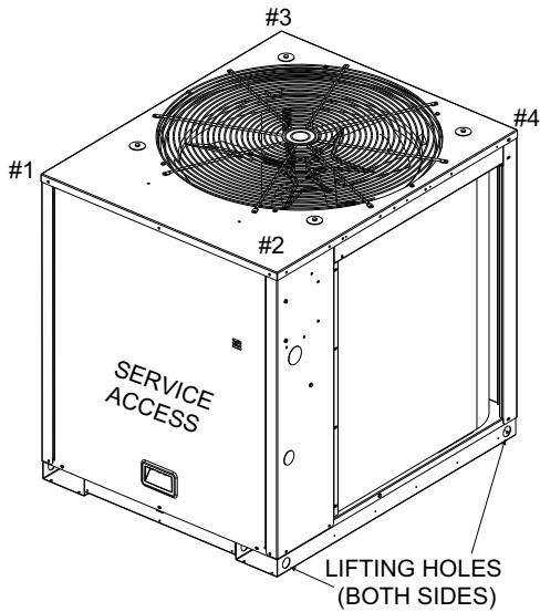
Figure 43. TWA072, 090, 120, 150
