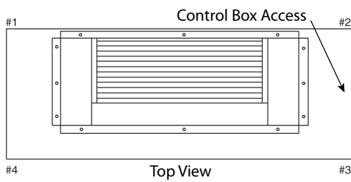
Figure 46. Vertical — TWE150, 180, 240, 300
