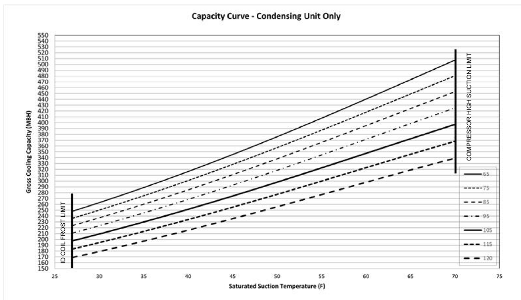
Figure 18. TWA300KD capacity curve
