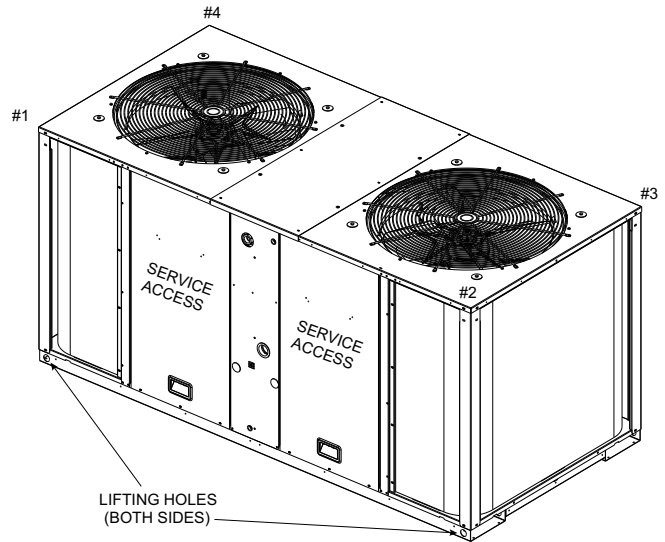
Figure 44. TWA180, 240, 300
