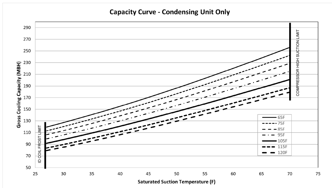
Figure 15. TWA150KD capacity curves
