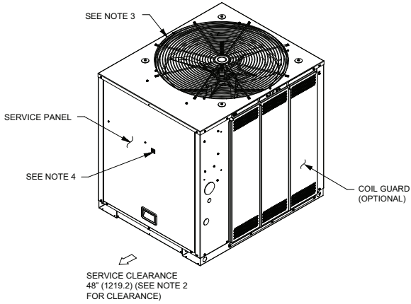
Figure 20. 6-7.5 ton heat pump, single compressor – in (mm)
