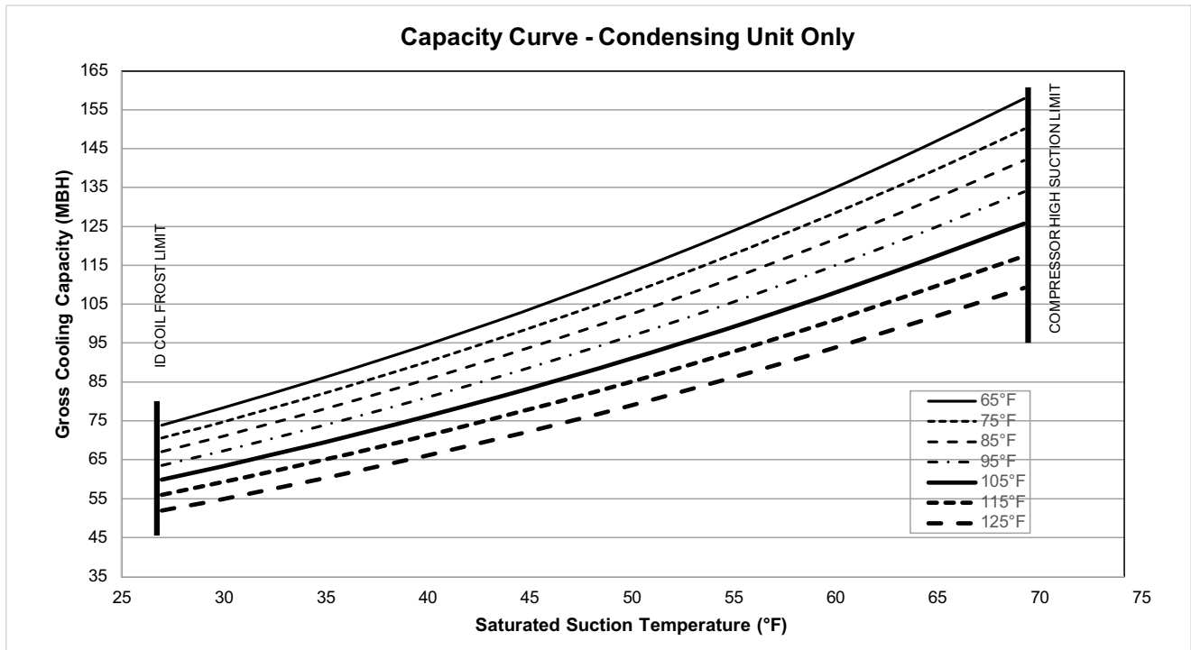
Figure 11. TTA090K*A capacity curve
