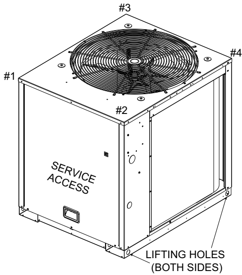
Figure 51. TTA072, 090, 120, 150
