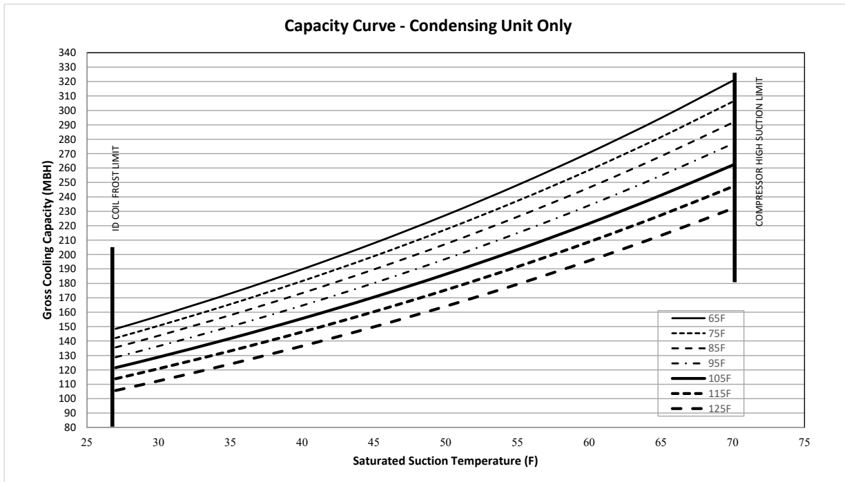
Figure 19. TTA180K*C – both compressors – capacity curve
