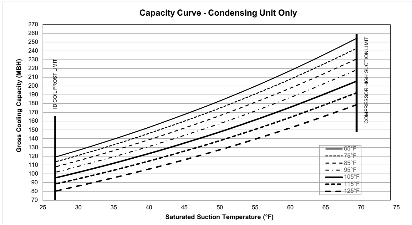
Figure 16. TTA150K*D capacity curve
