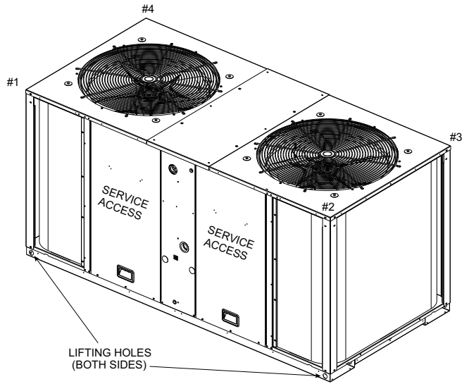
Figure 52. TTA180, 240, 300
