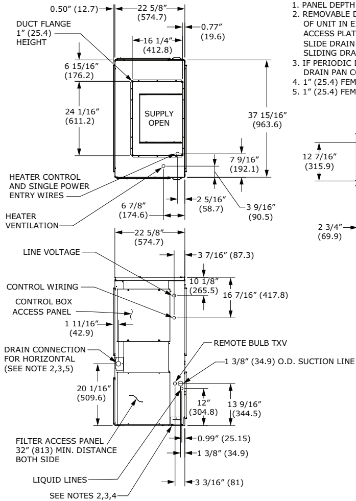
Figure 34. 5 ton air handler, single circuit – in. (mm)
