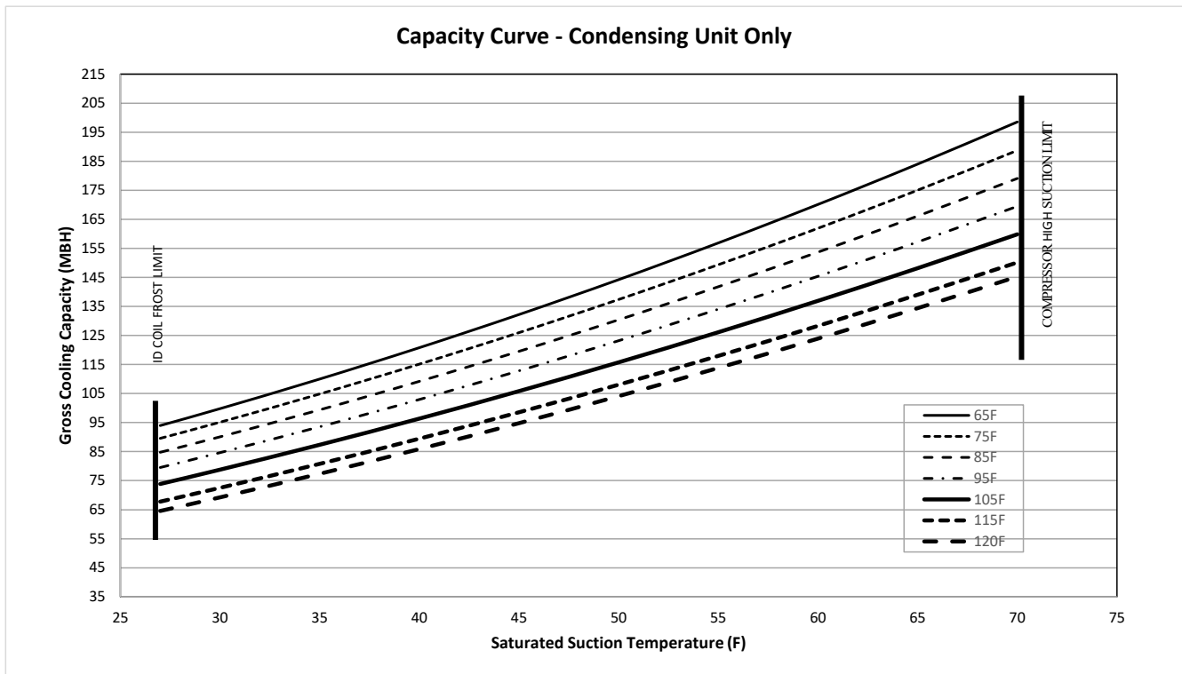
Figure 15. TTA120K*C – both compressors – capacity curve
