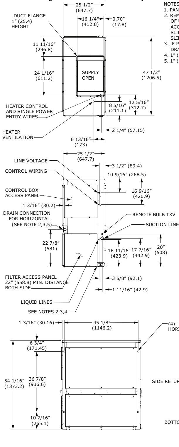
Figure 36. 7.5 ton air handler, single circuit – in. (mm)
