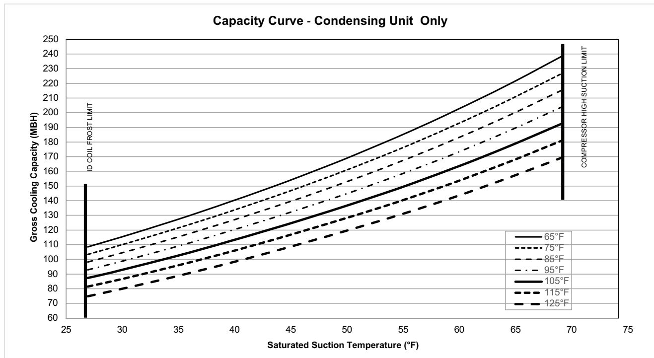
Figure 21. TTA240K*C – one compressor – capacity curve
