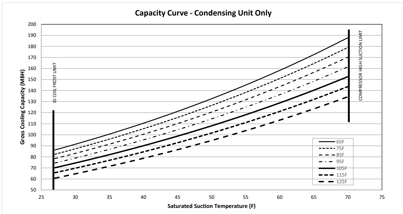
Figure 18. TTA180K*C – one compressor – capacity curve
