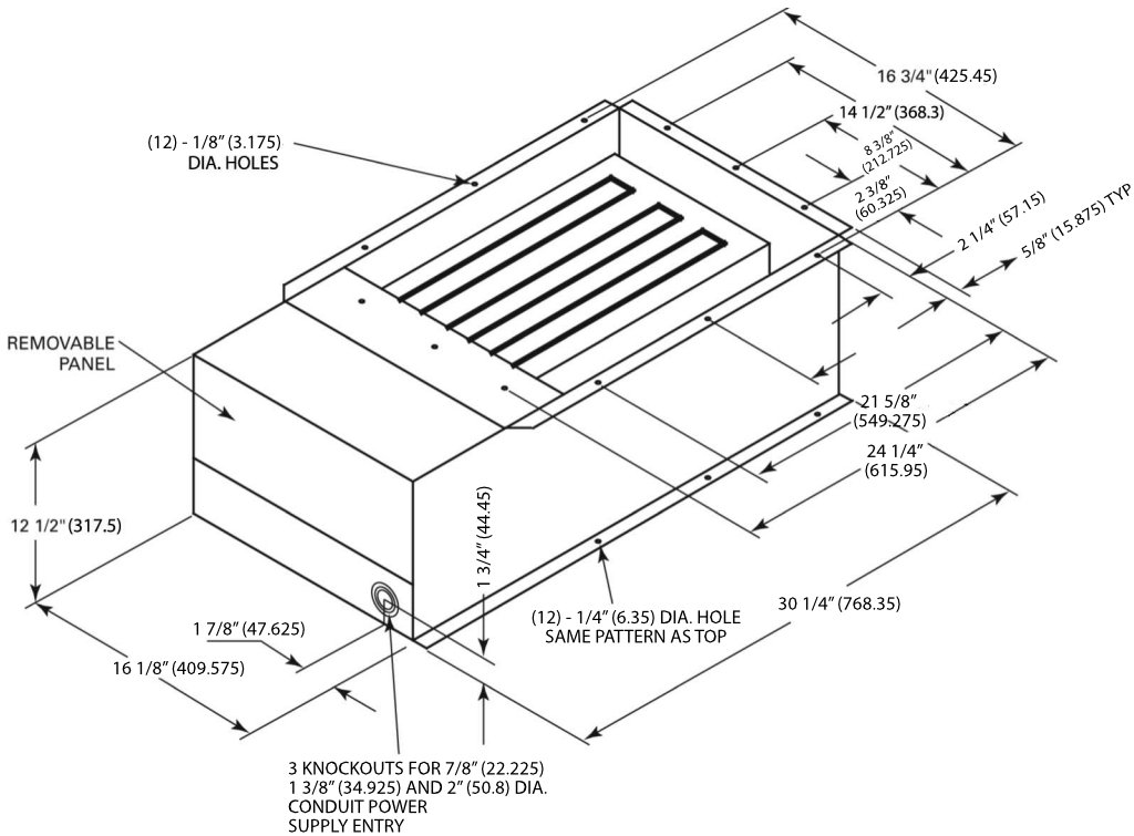
Figure 44. Electric heater accessory for 5-10 ton air handlers – in (mm)
