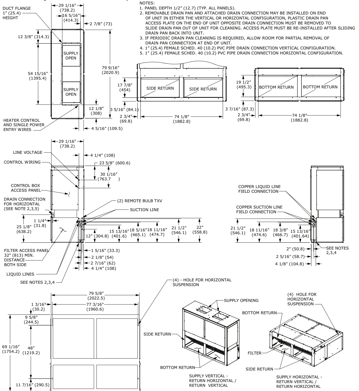
Figure 40. 12.5, 15 ton air handler, dual circuit – in. (mm)
