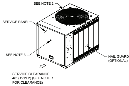
Figure 30. 12.5 ton condensing, dual compressor – in (mm)
