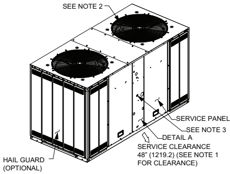
Figure 33. 25 ton condensing, manifolded compressor – in (mm)
