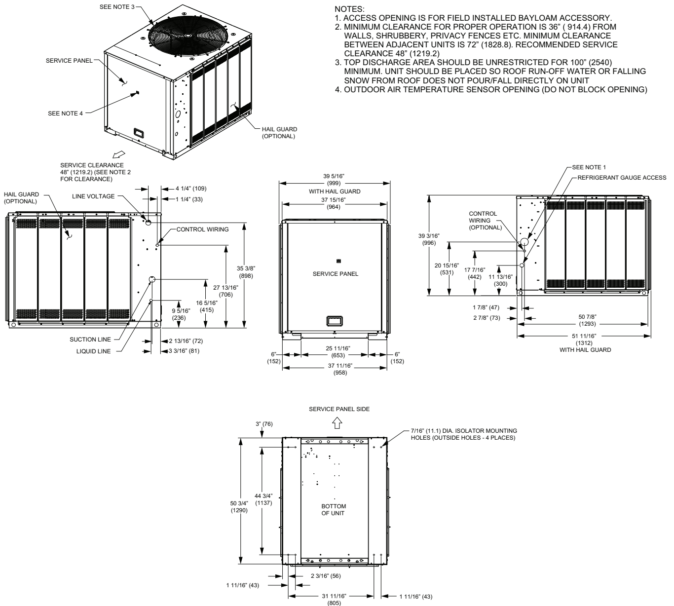
Figure 28. 10 ton condensing, manifolded compressor – in (mm)
