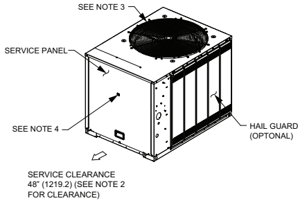
Figure 29. 10 ton condensing, dual compressor – in (mm)
