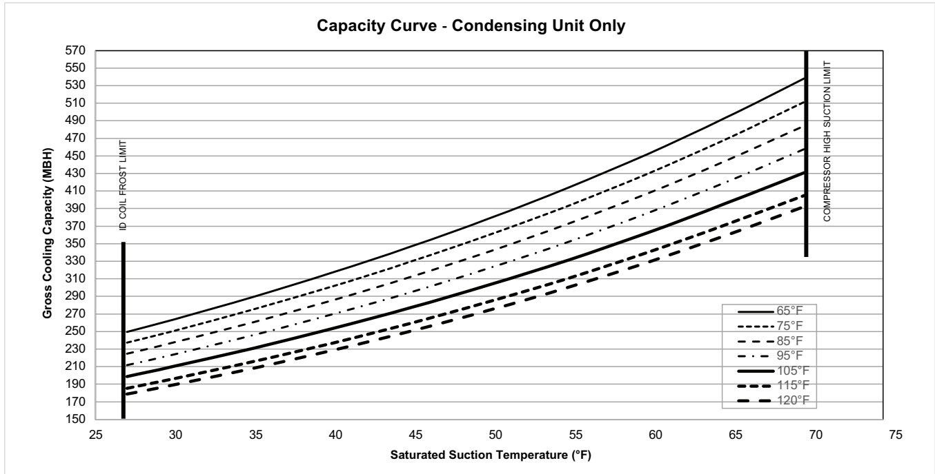
Figure 24. TTA300K*C – both compressors – capacity curve
