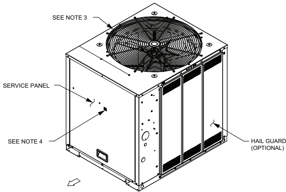
Figure 27. 6, 7.5 ton condensing, dual compressor – in (mm)
