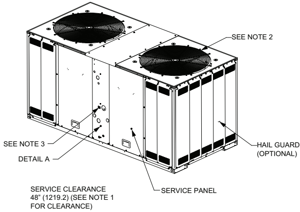
Figure 31. 15, 20 ton condensing, dual compressor – in (mm)
