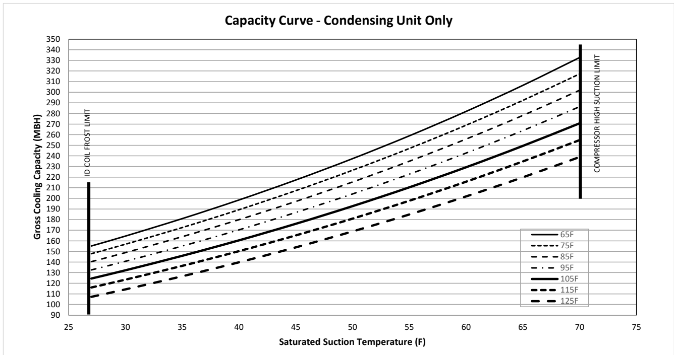
Figure 17. TTA180K*D capacity curve
