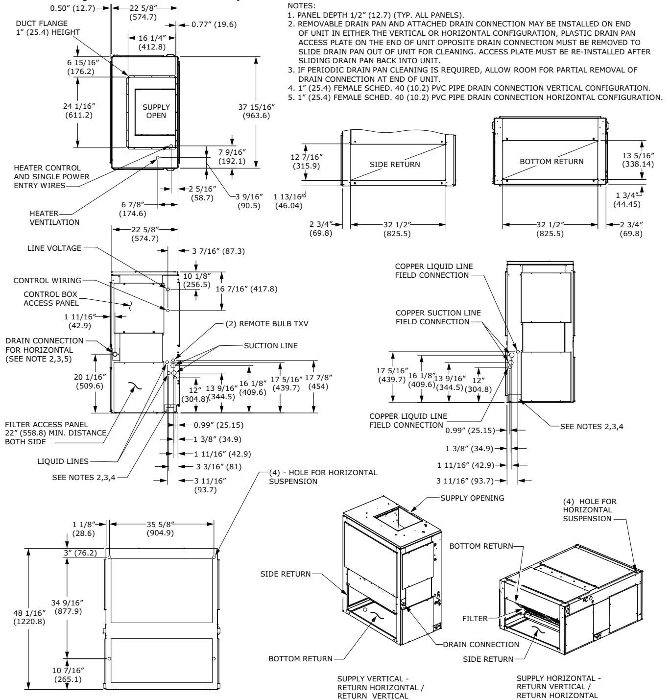
Figure 35. 5 ton air handler, dual circuit – in. (mm)
