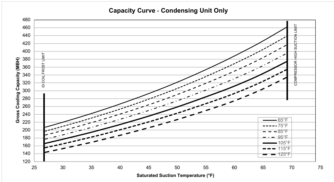
Figure 22. TTA240K*C – both compressors – capacity curve
