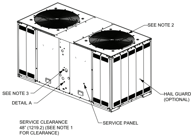
Figure 32. 15, 20 ton condensing, manifolded compressor – in (mm)
