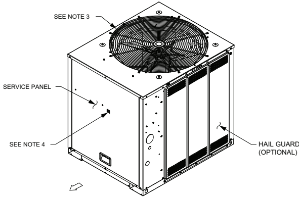
Figure 26. 6, 7.5 ton condensing, single compressor – in (mm)
