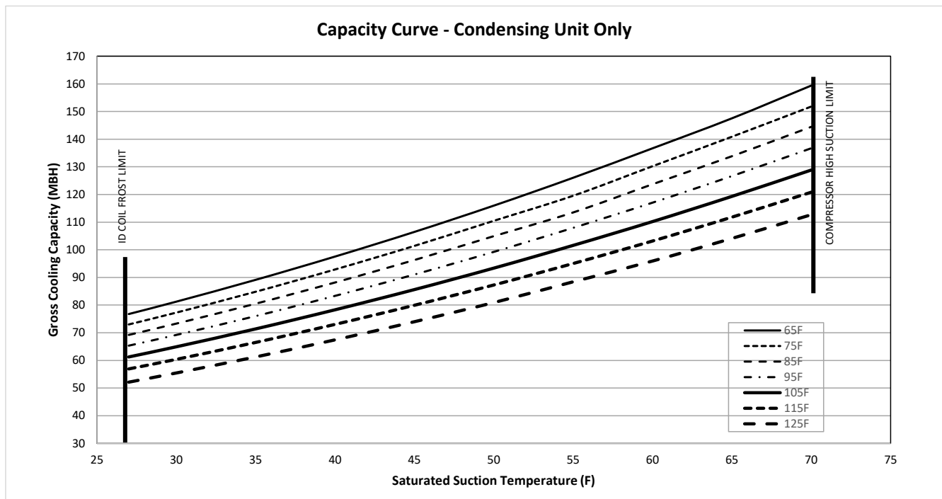
Figure 12. TTA090K*D capacity curve
