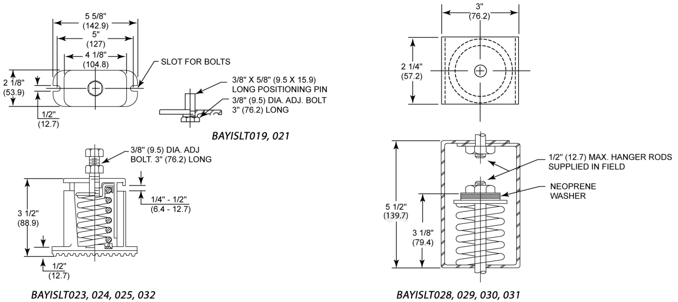
Figure 43. Spring isolator accessory dimensions – in (mm)
