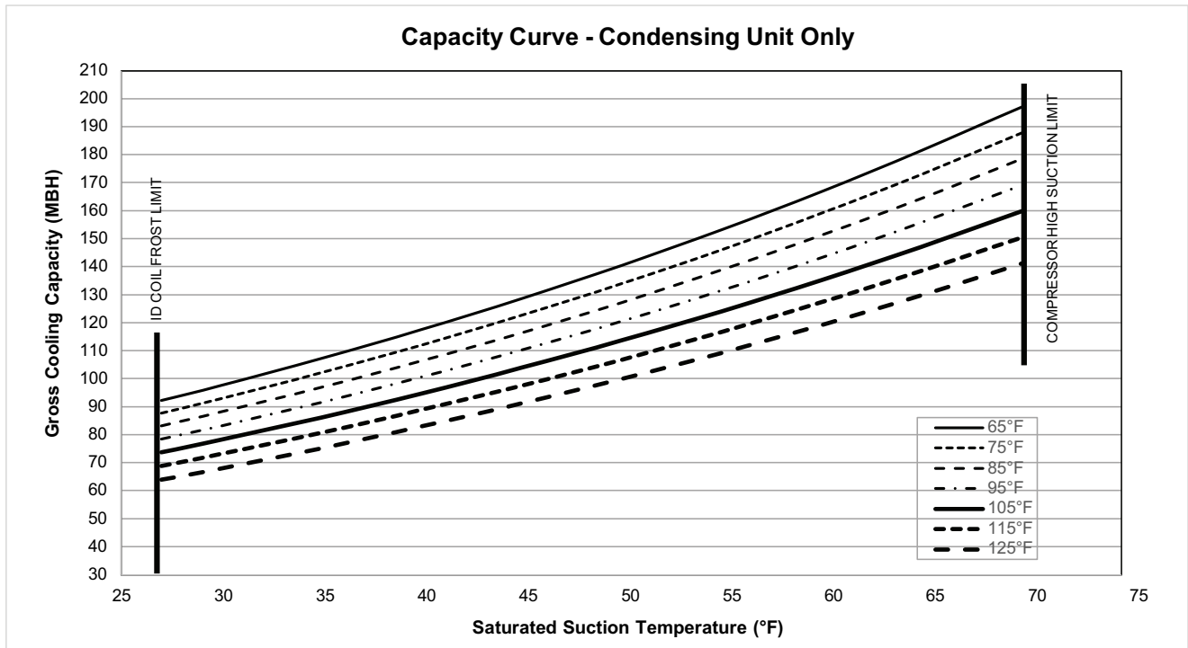
Figure 13. TTA120K*D capacity curve
