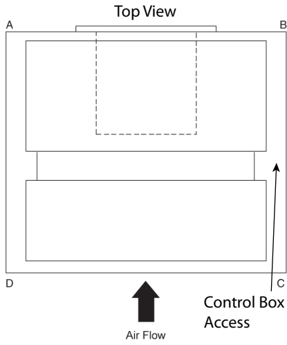
Figure 56. Horizontal — TWE150, 180, 240, 300
