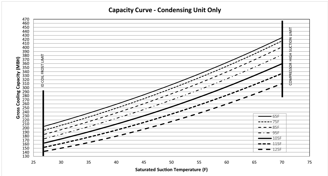
Figure 20. TTA240K*D capacity curve
