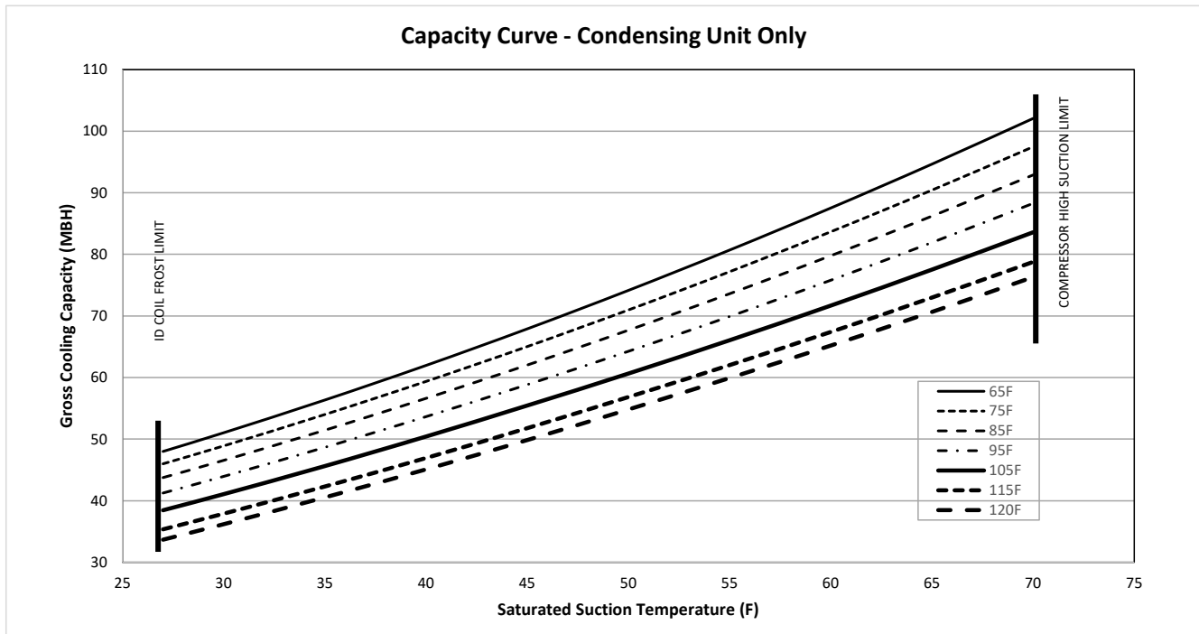
Figure 14. TTA120K*C – one compressor – capacity curve
