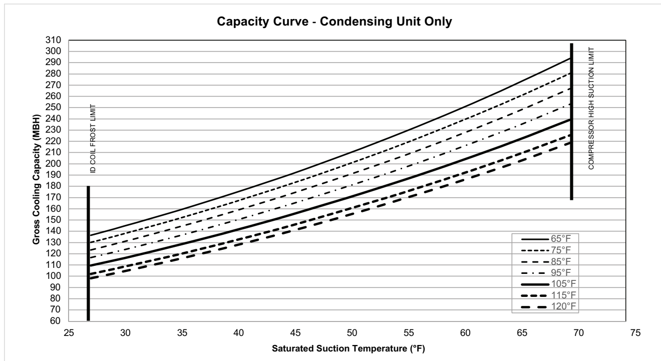
Figure 23. TTA300K*C – one compressor – capacity curve
