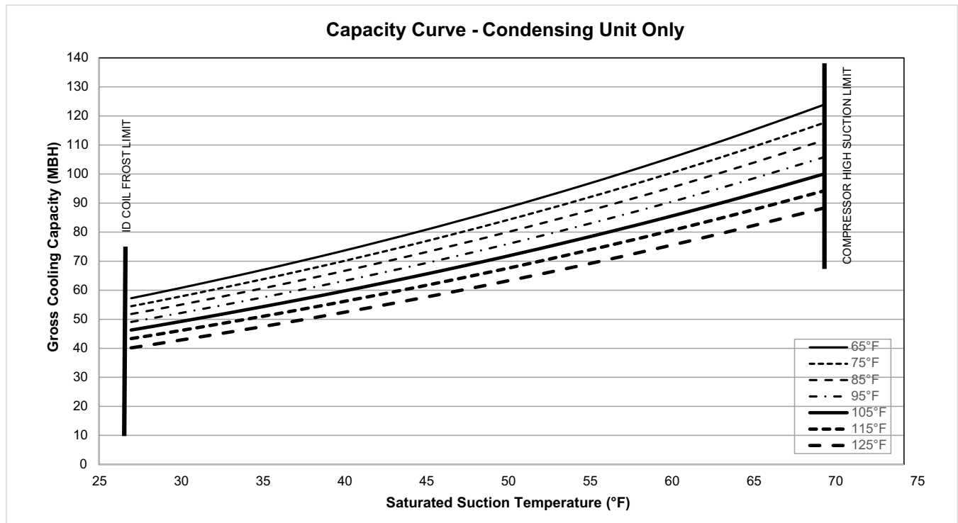
Figure 9. TTA072K*A capacity curve
