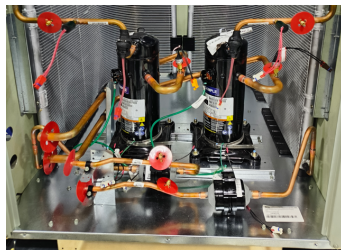
Figure 1. Compressors
