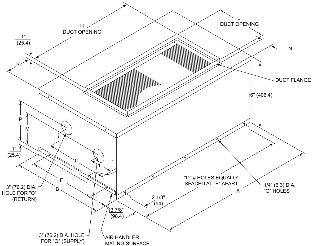
Figure 47. Hot water coil accessory – in (mm)
