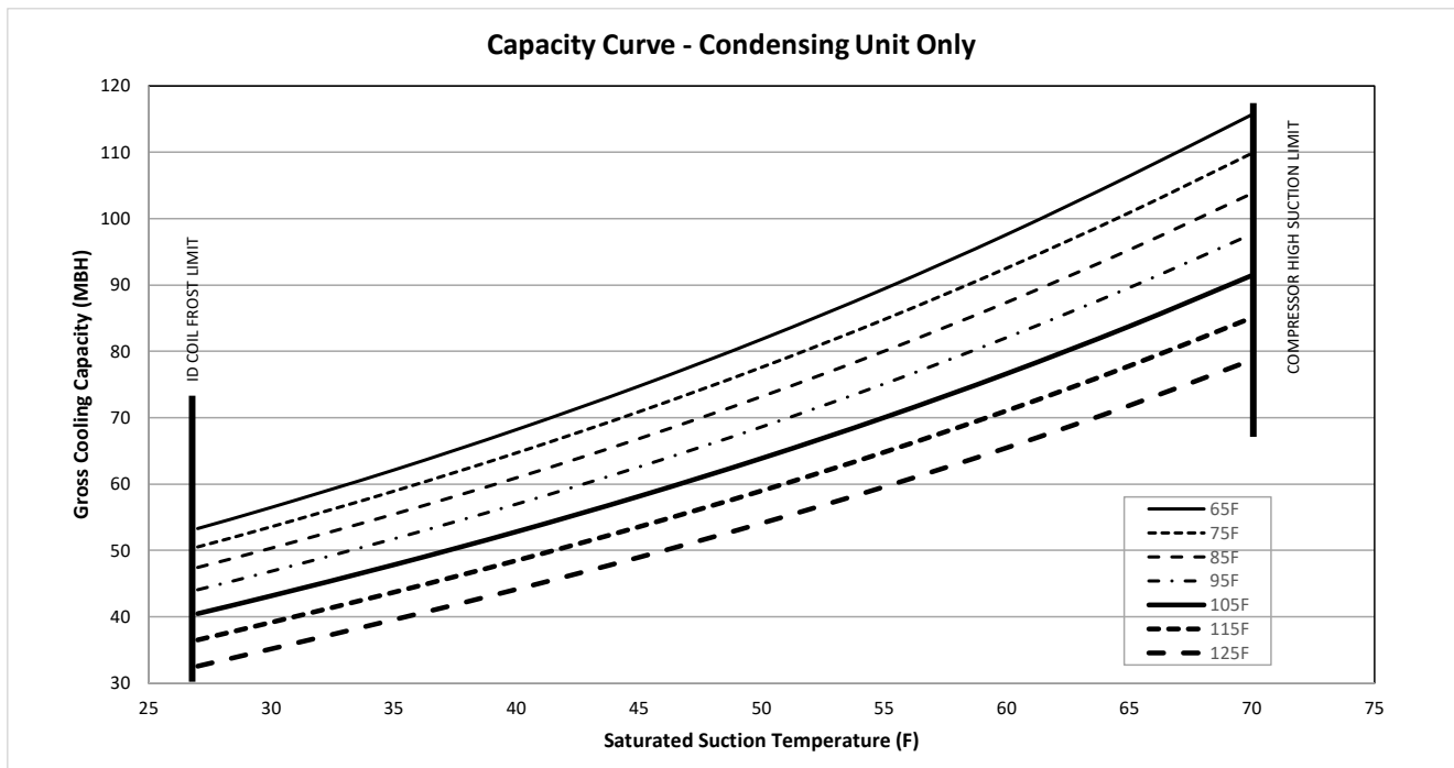
Figure 10. TTA072K*D capacity curve
