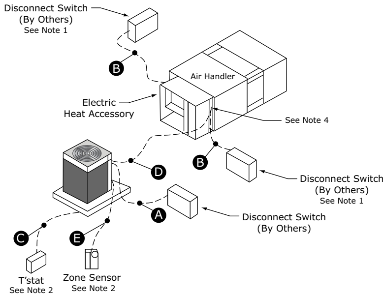
Figure 26. Symbio™ jobsite connections
