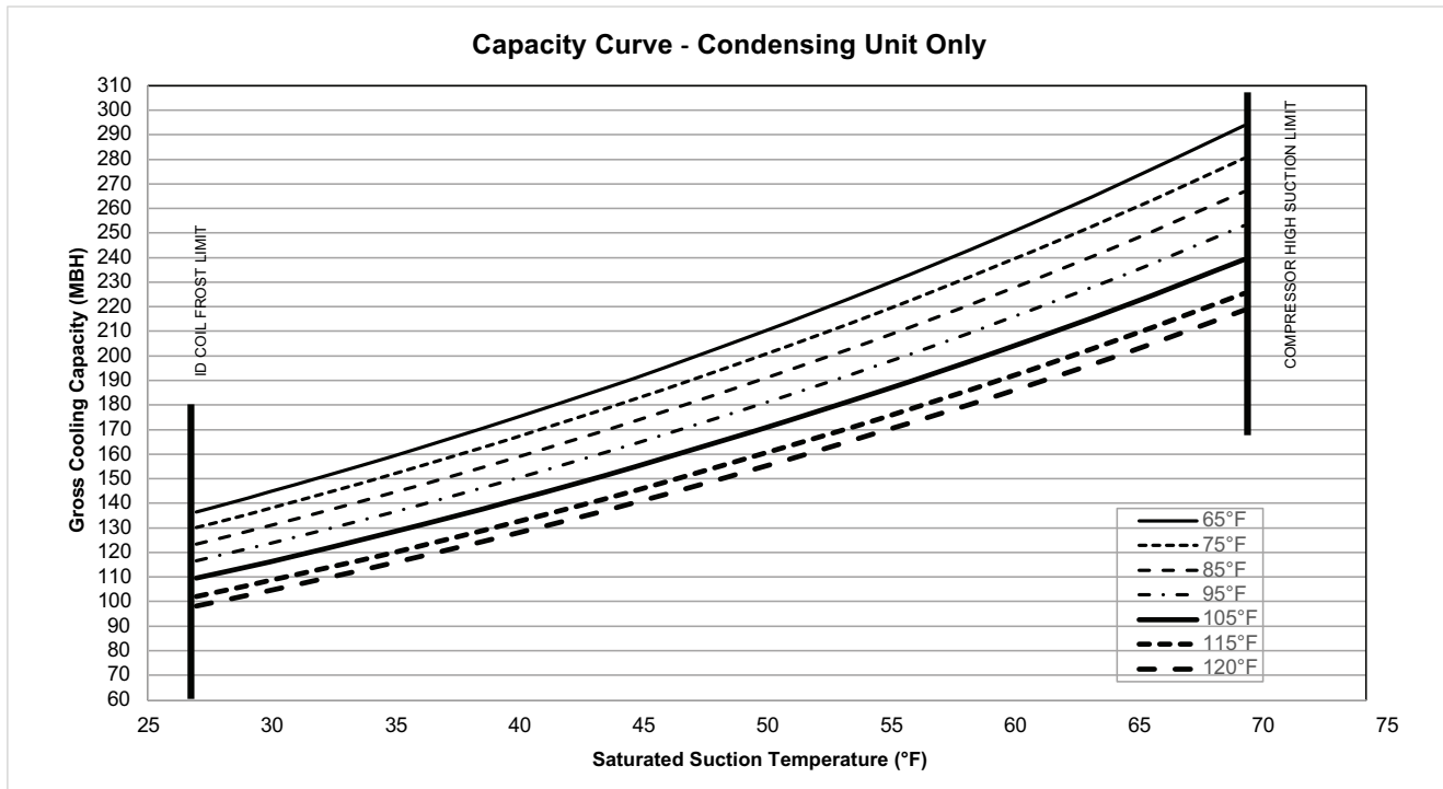
Figure 24. TTA300K*C – one compressor – capacity curve
