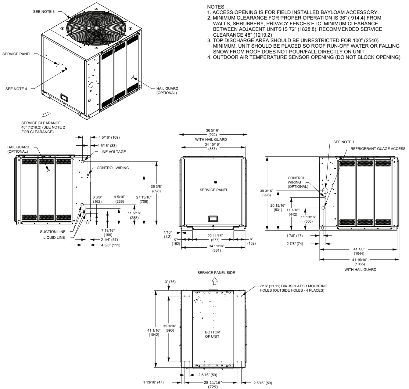
Figure 28. 6, 7.5 ton condensing, dual compressor – in (mm)
