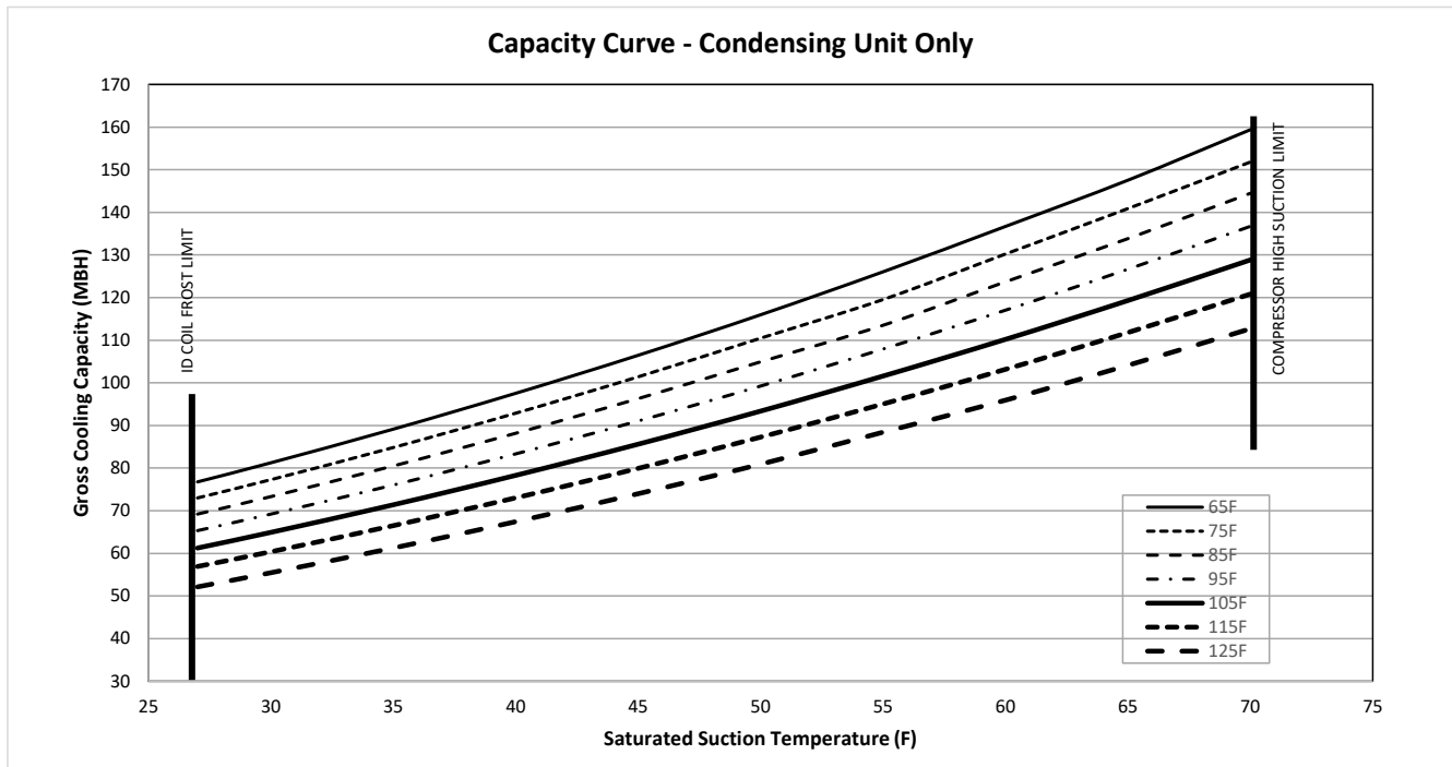
Figure 13. TTA090K*D capacity curve
