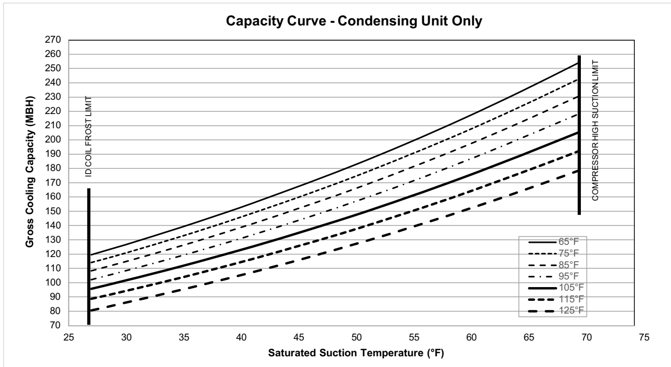
Figure 17. TTA150K*D capacity curve
