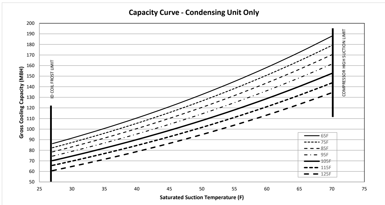
Figure 19. TTA180K*C – one compressor – capacity curve
