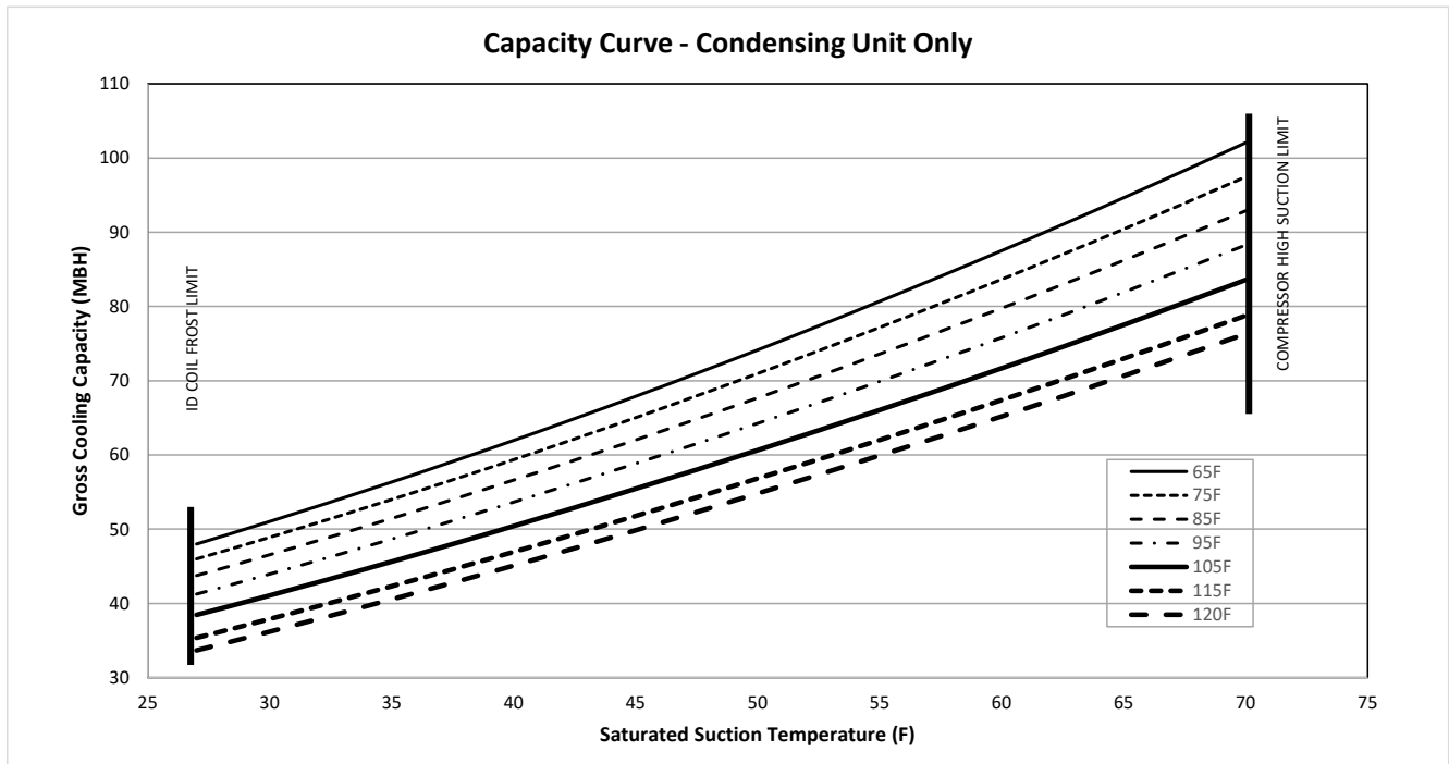
Figure 15. TTA120K*C – one compressor – capacity curve
