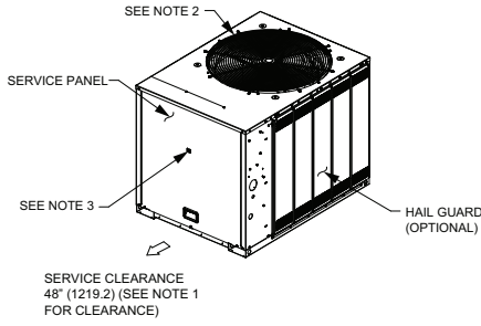
Figure 31. 12.5 ton condensing, dual compressor – in (mm)
