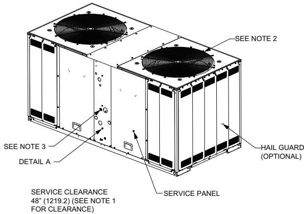
Figure 33. 15, 20 ton condensing, manifolded compressor – in (mm)
