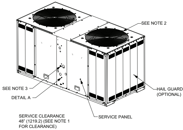
Figure 32. 15, 20 ton condensing, dual compressor – in (mm)
