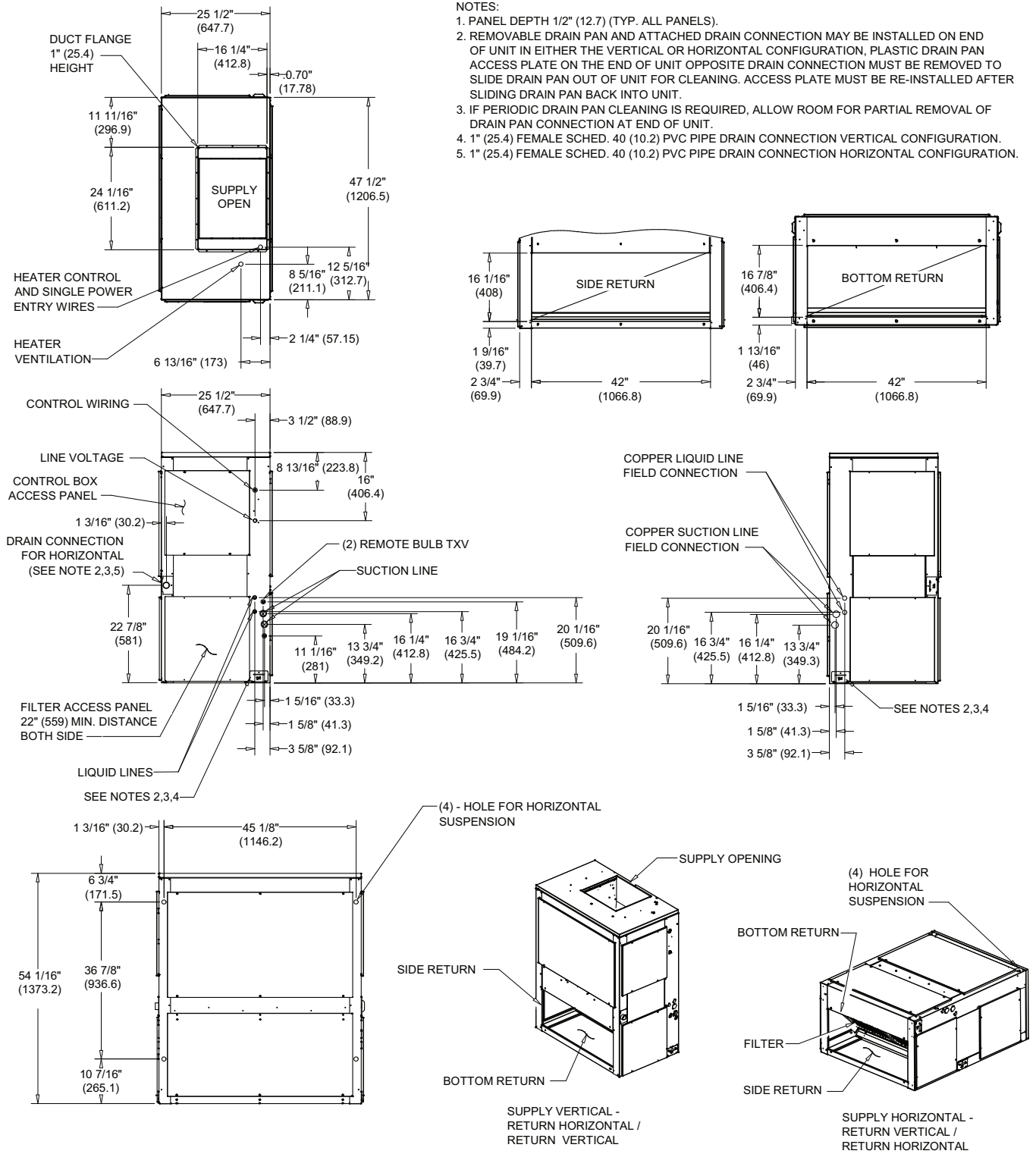
Figure 38. 6, 7.5 ton air handler, dual circuit – in. (mm)
