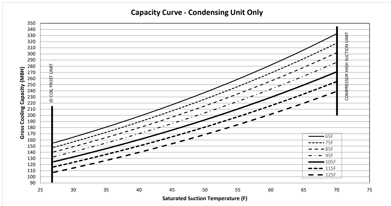
Figure 18. TTA180K*D capacity curve
