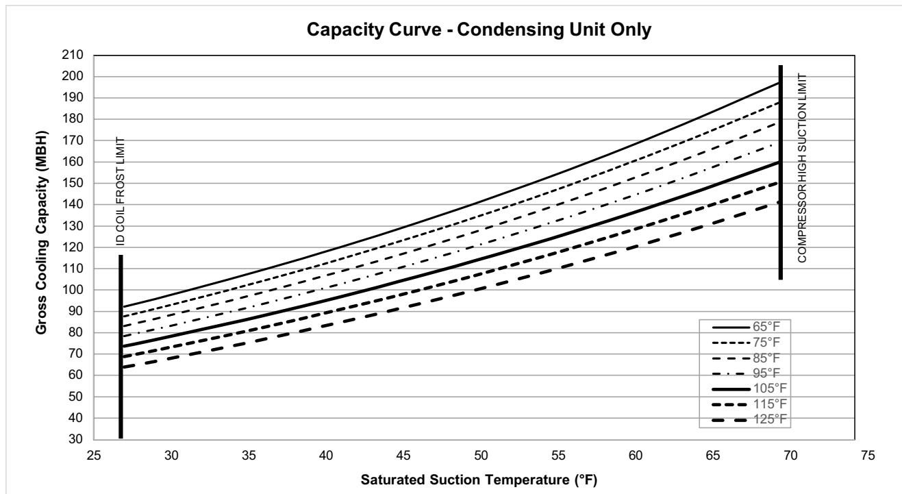
Figure 14. TTA120K*D capacity curve
