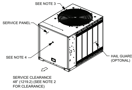
Figure 30. 10 ton condensing, dual compressor – in (mm)
