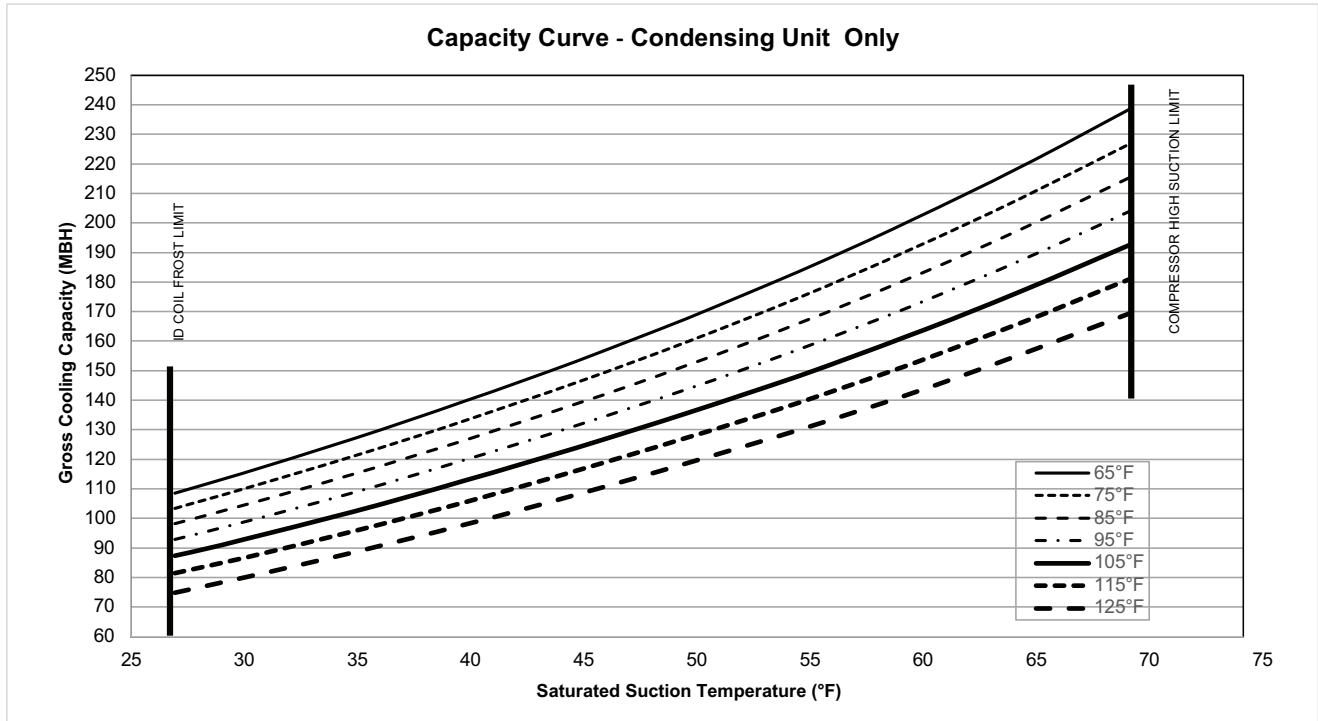
Figure 22. TTA240K*C – one compressor – capacity curve
