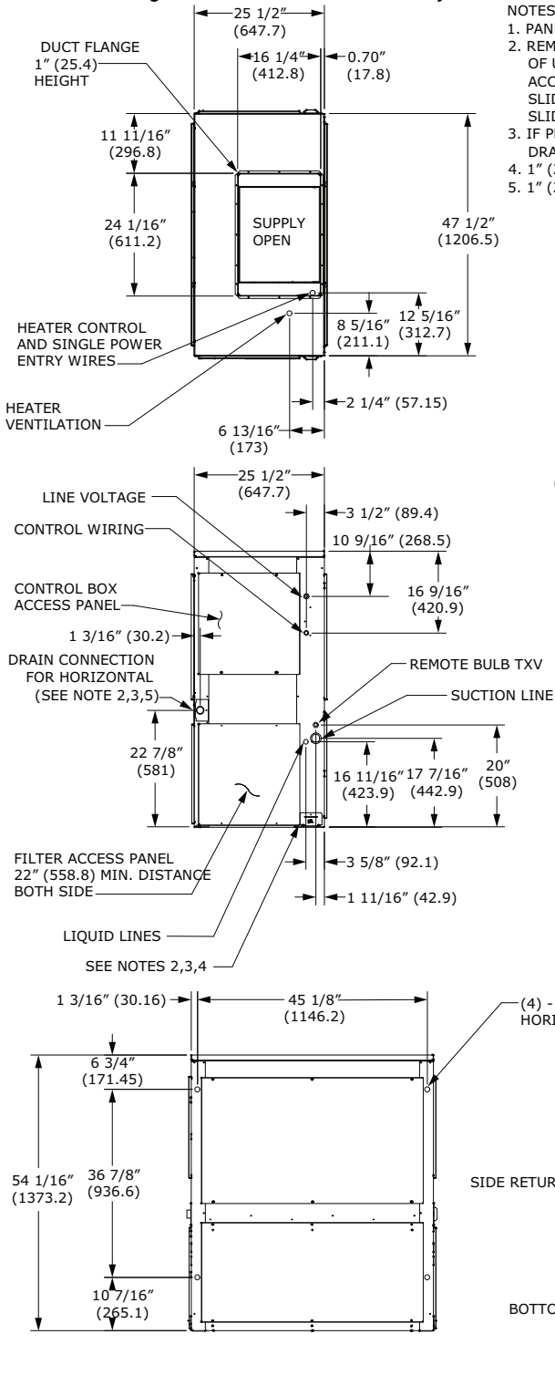
Figure 37. 7.5 ton air handler, single circuit – in. (mm)
