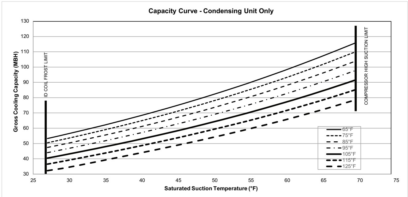
Figure 11. TTA072K*D capacity curve
