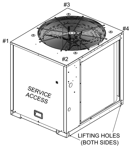
Figure 52. TTA072, 090, 120, 150
