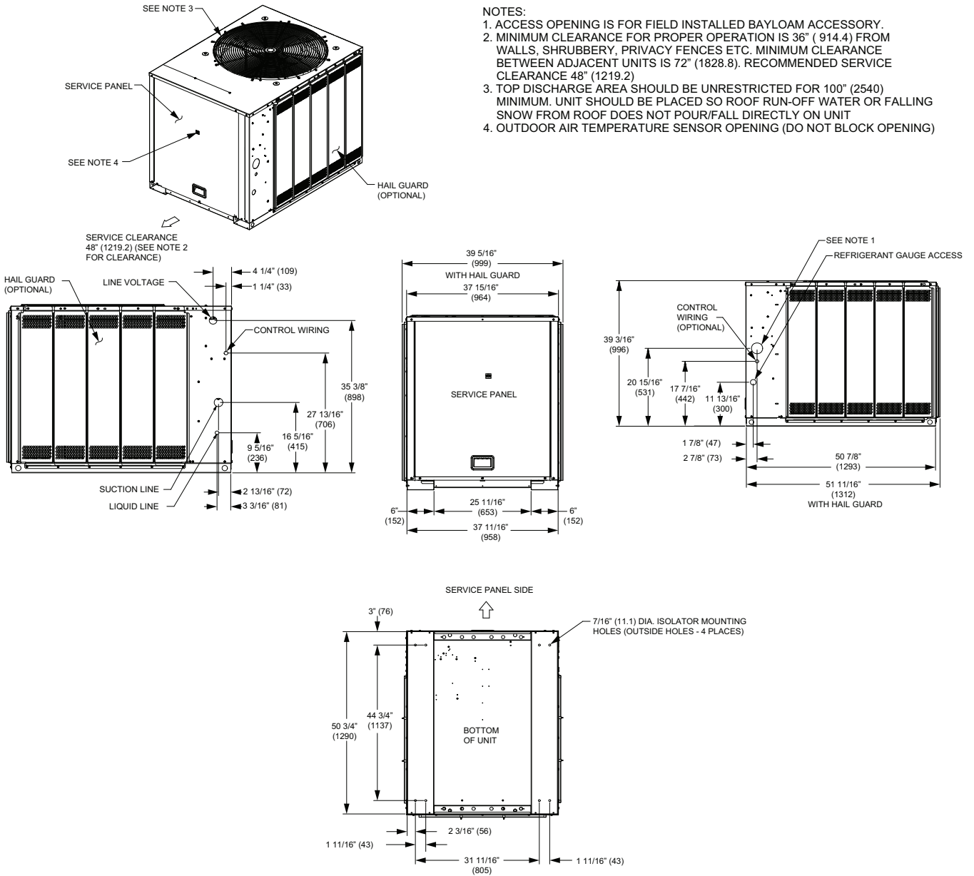
Figure 29. 10 ton condensing, manifolded compressor – in (mm)
