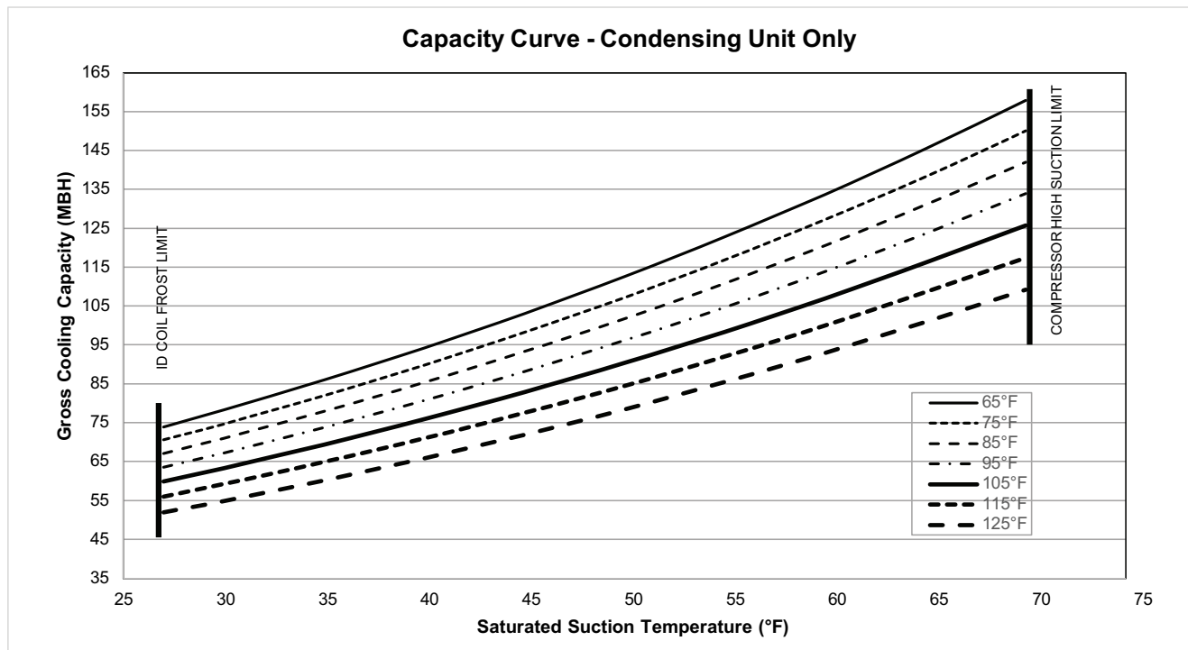
Figure 12. TTA090K*A capacity curve
