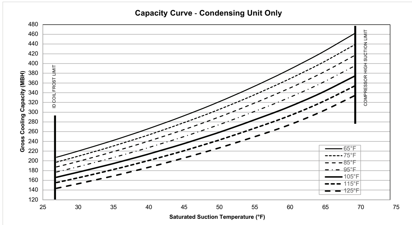
Figure 23. TTA240K*C – both compressors – capacity curve
