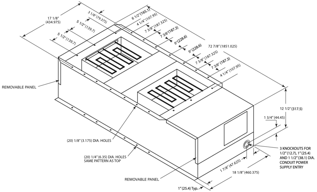
Figure 46. Electric heater accessory for 12.5-25 ton air handlers – in (mm)
