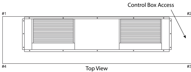
Figure 55. Vertical — TWE150, 180, 240, 300
