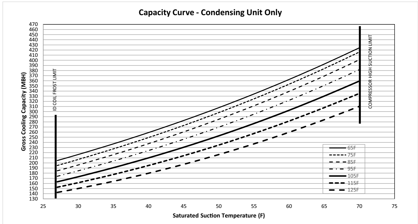
Figure 21. TTA240K*D capacity curve
