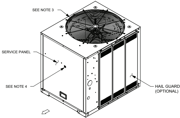
Figure 27. 6, 7.5 ton condensing, single compressor – in (mm)
