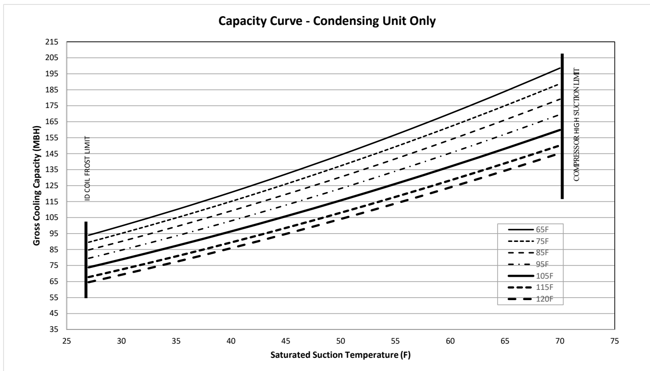
Figure 16. TTA120K*C – both compressors – capacity curve
