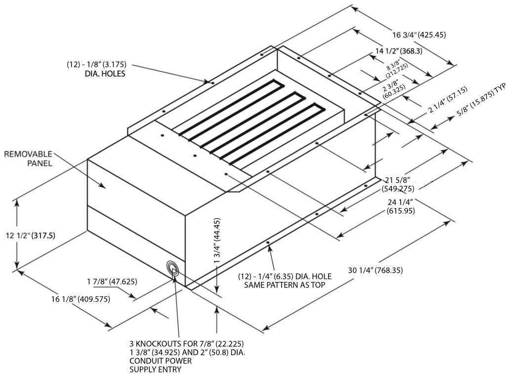
Figure 45. Electric heater accessory for 5-10 ton air handlers – in (mm)
