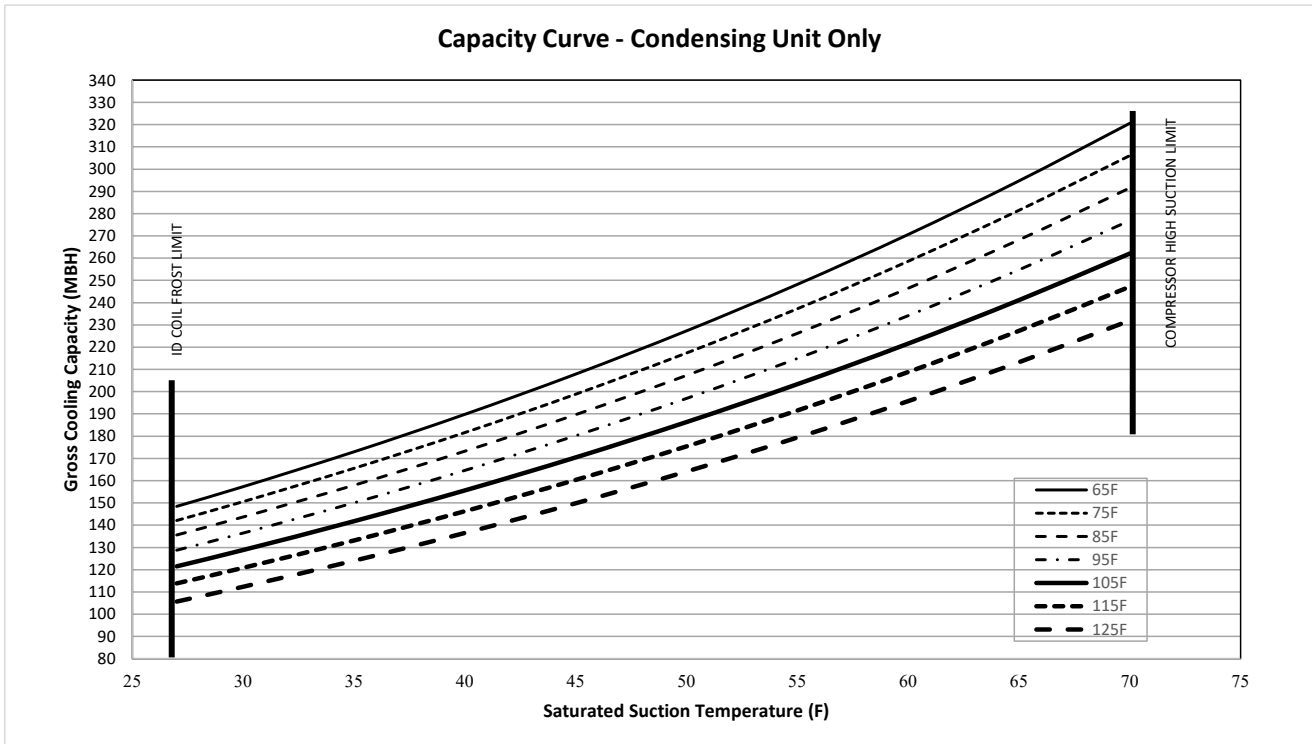
Figure 20. TTA180K*C – both compressors – capacity curve
