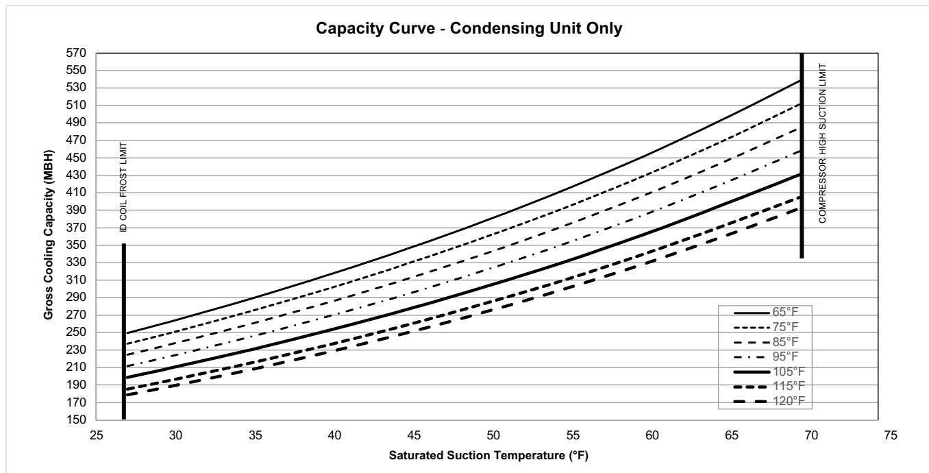
Figure 25. TTA300K*C – both compressors – capacity curve
