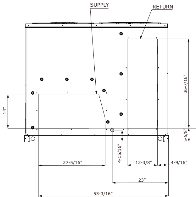
Figure 8. Cooling with optional electric heat and gas/electric models — roof curb (in inches)
