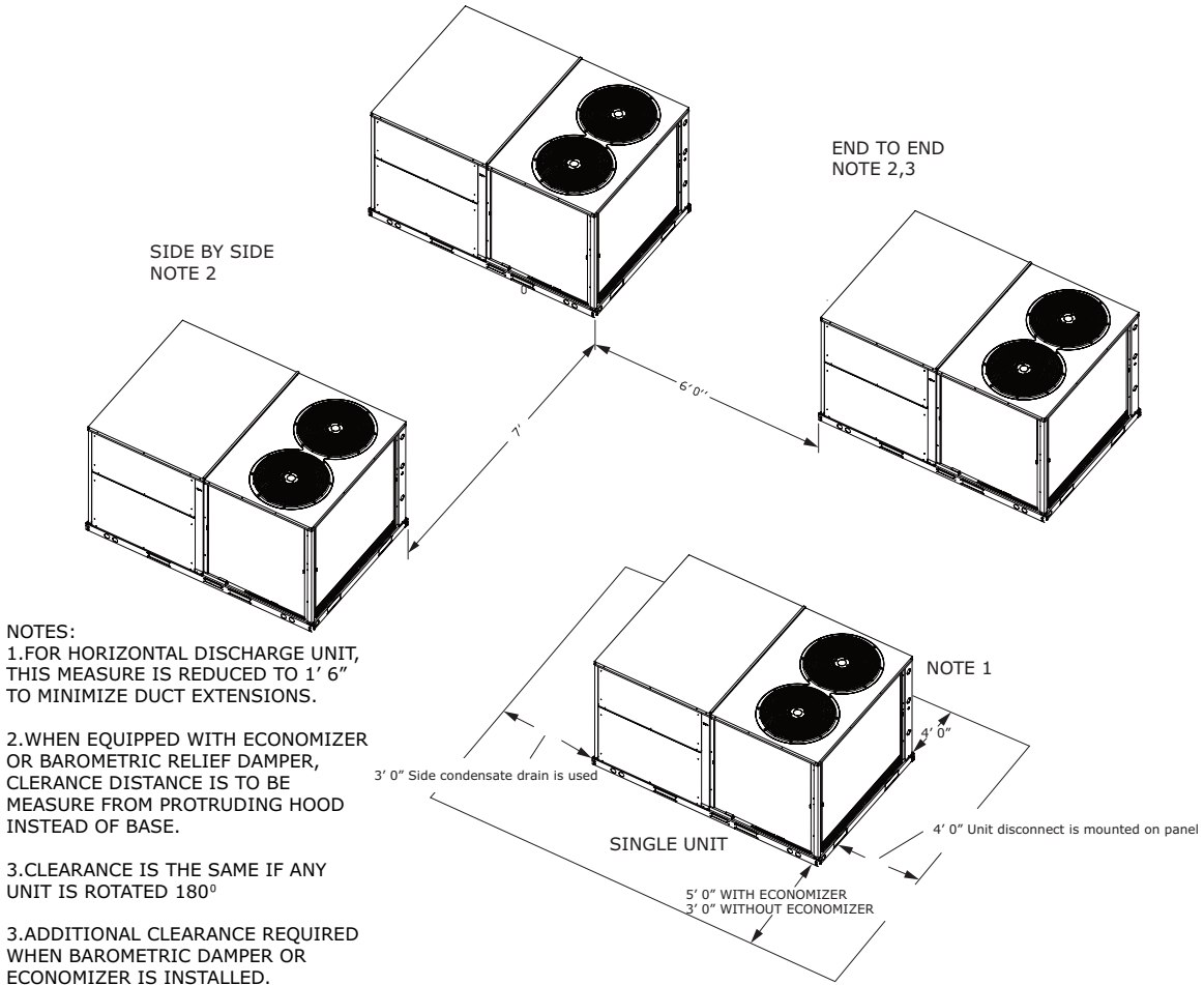
Figure 4. Cooling with optional electrical heat and gas/electric units — overview
