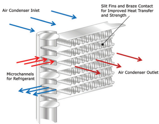
Figure 2. Microchannel condenser coil
