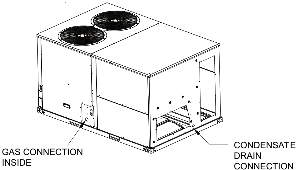
Figure 4. Cooling with optional electrical heat and gas/electric units — overview
