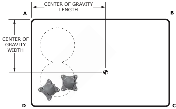
Figure 10. Center of gravity/corner weights
