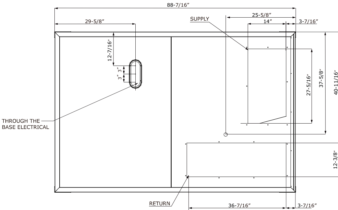
Figure 6. Cooling with optional electrical heat and gas/electric units — bottom view (in inches)
