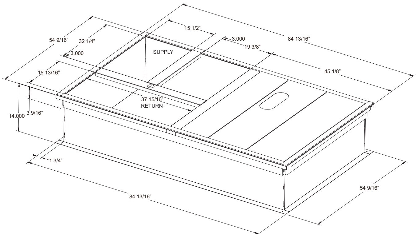
Figure 8. Cooling with optional electric heat and gas/electric models — roof curb (in inches)
