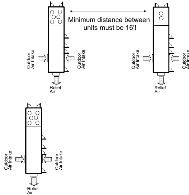
Figure 5. Unit placement
