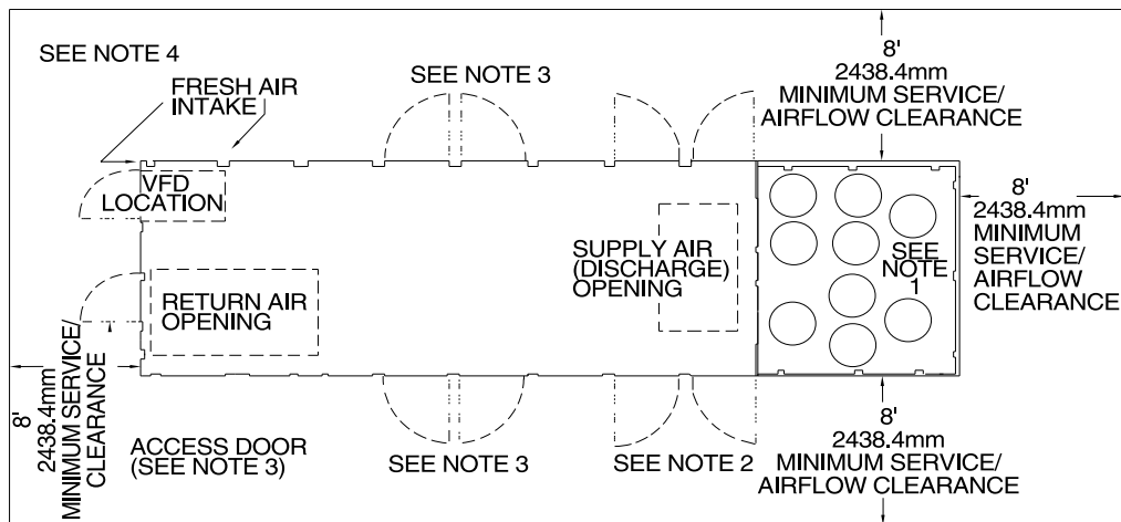
Figure 42. Service clearance — 90 to 130 tons air-cooled
