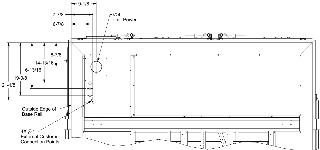
Figure 36. Wire entry dimensions — 20 to 75 tons
