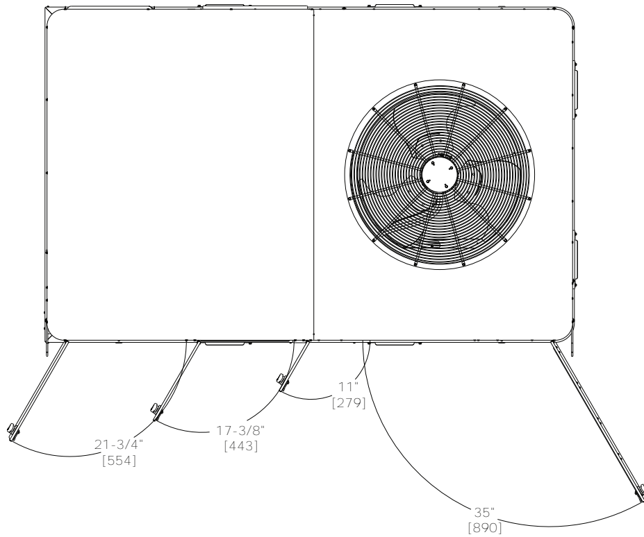
Figure 23. B.0 and C.0 cabinets – standard economizer, manual or motorized fresh air damper
