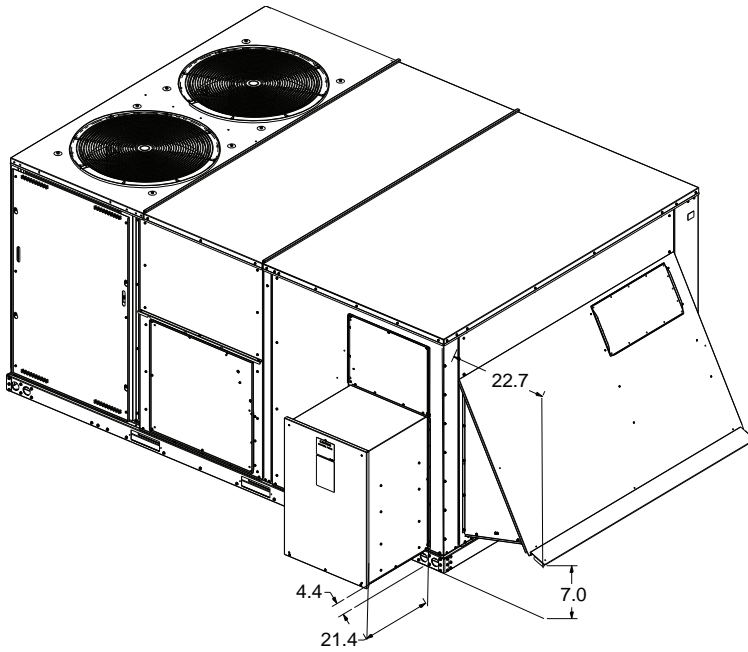
Figure 33. Gas pipe height
