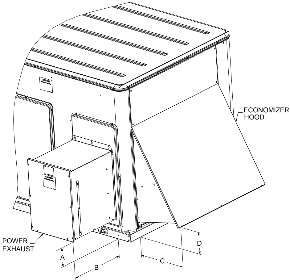
Figure 24. B.0 and C.0 cabinet – power exhaust with standard economizer
