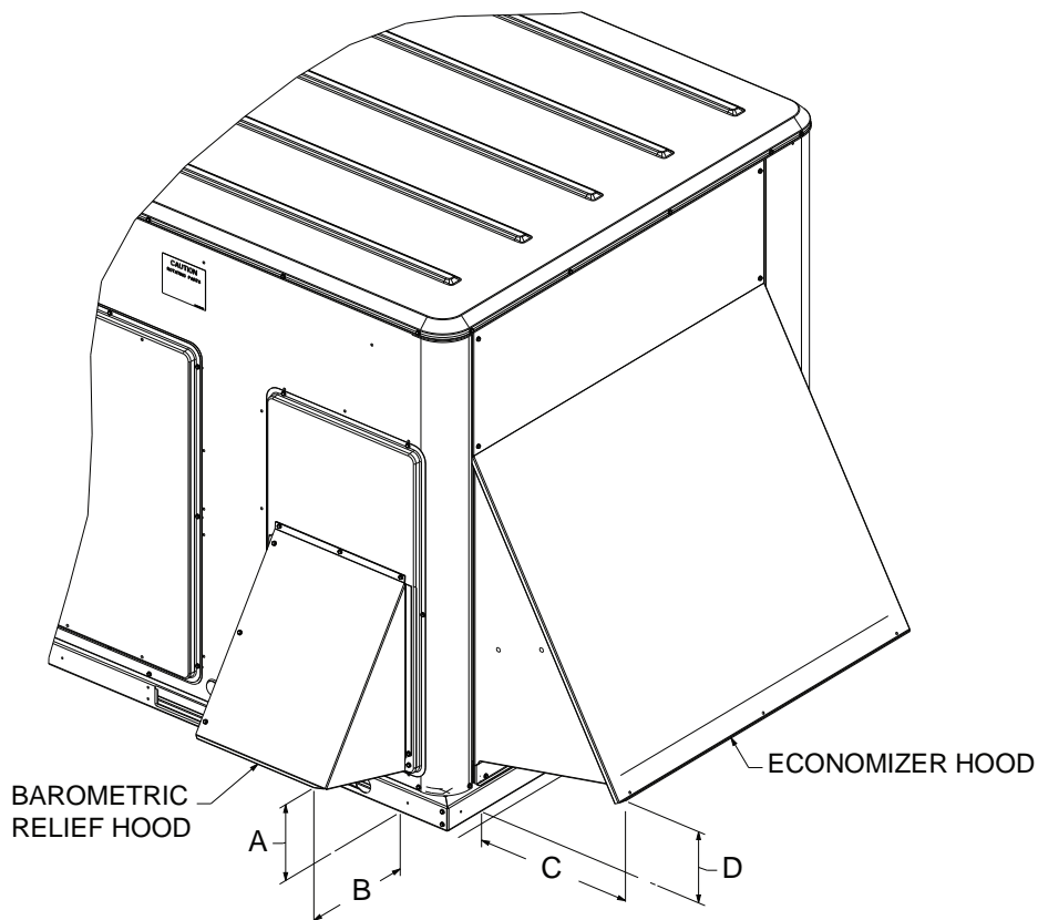
Figure 23. B.0 and C.0 cabinets – standard economizer, manual or motorized fresh air damper
