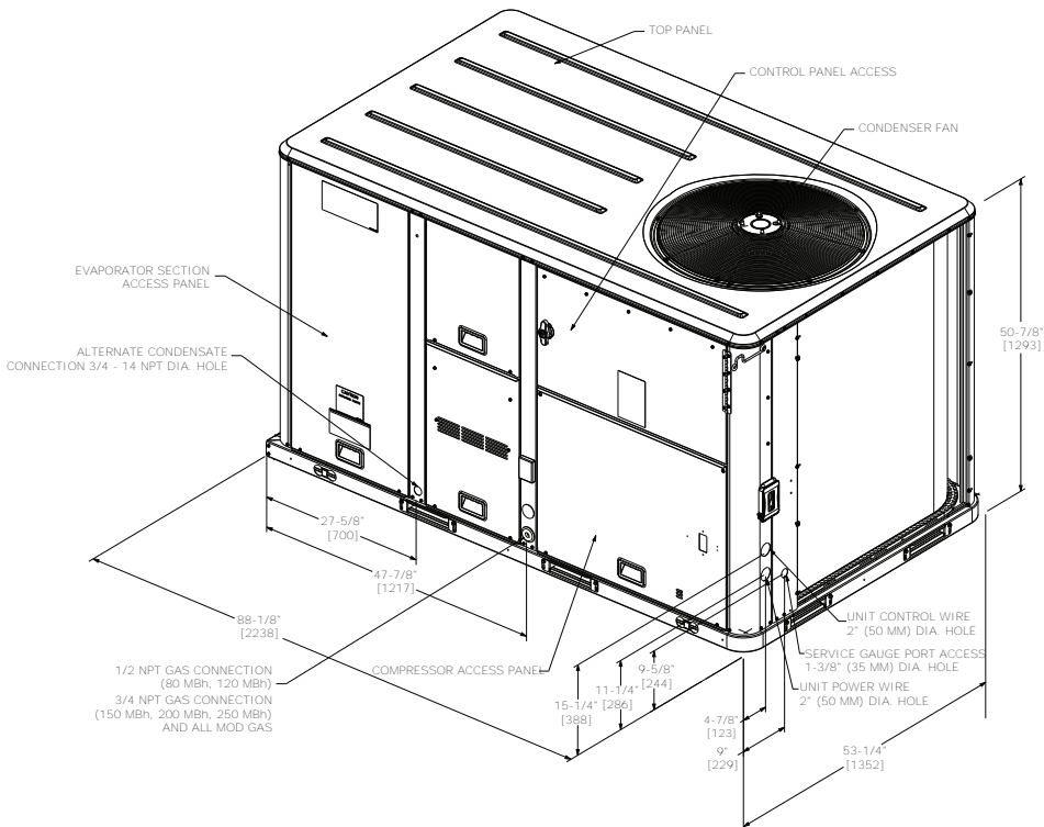
Figure 10. B.0 cabinet
