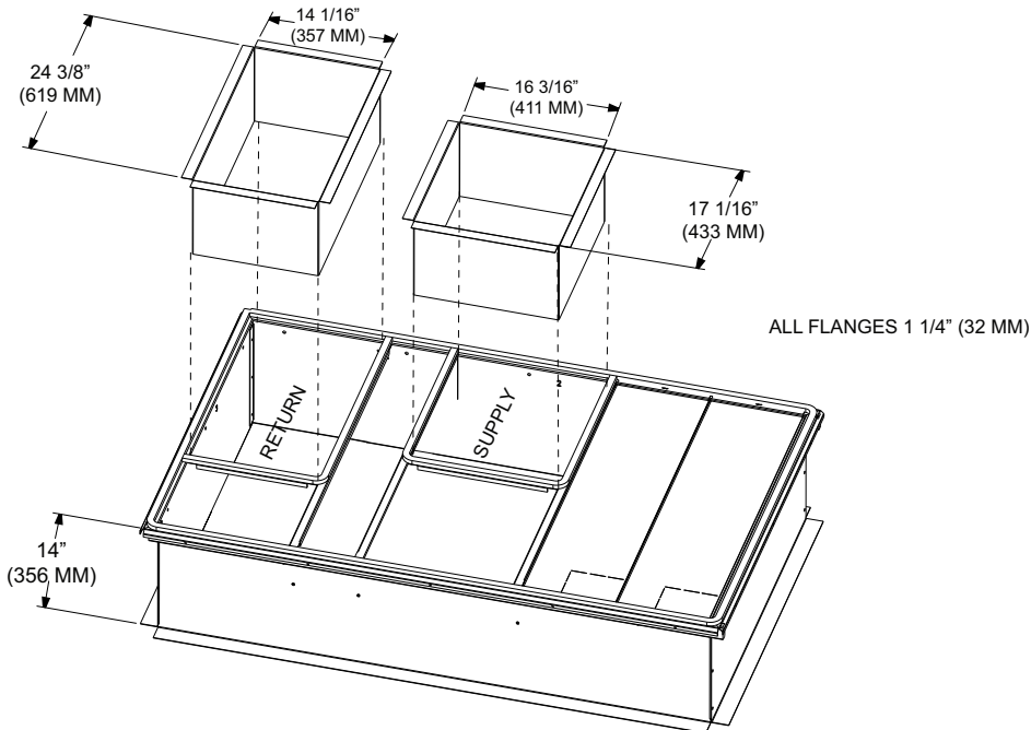
Figure 30. A.0 cabinet – downflow duct connections, field fabricated
