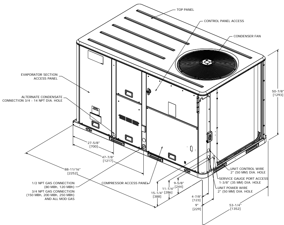
Figure 32. B.0 cabinet
