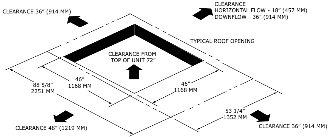
Figure 36. B.0 cabinet – roof curb
