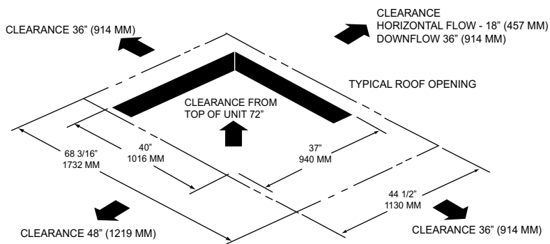
Figure 28. A.0 cabinet – unit clearance and roof opening
