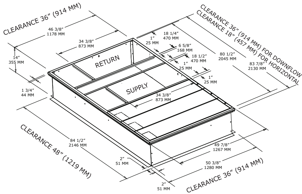
Figure 36. B.0 cabinet – roof curb
