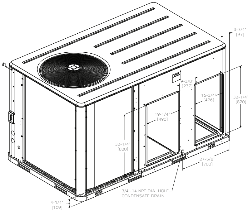
Figure 34. B.0 cabinet – horizontal airflow supply/return
