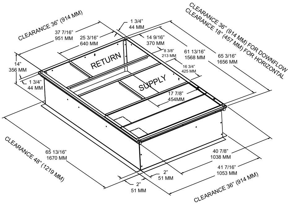
Figure 30. A.0 cabinet – downflow duct connections, field fabricated
