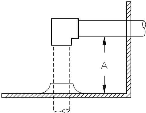
Figure 55. Gas pipe height
