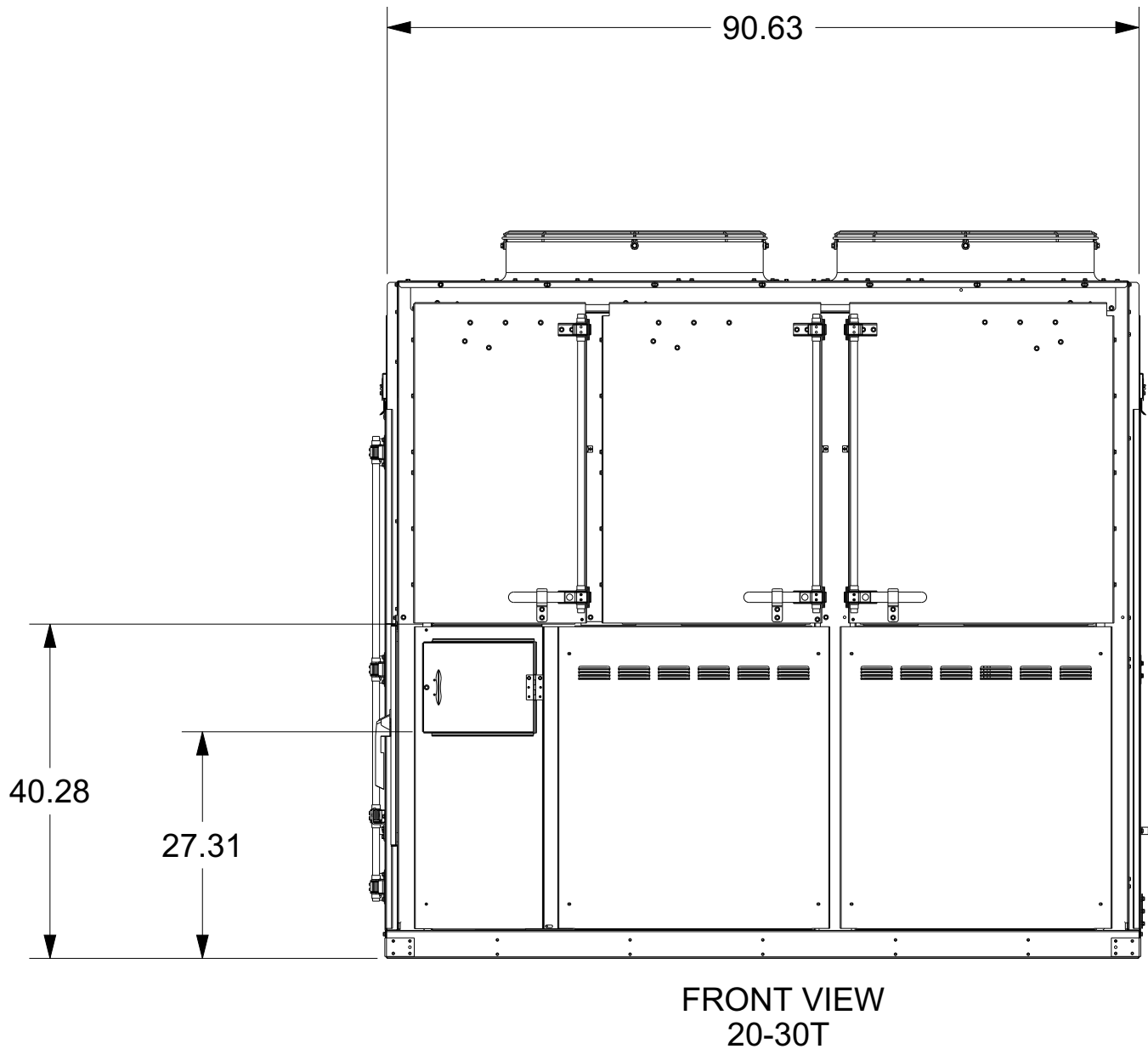
Figure 31. 20 to 30 ton — front view (inches)
