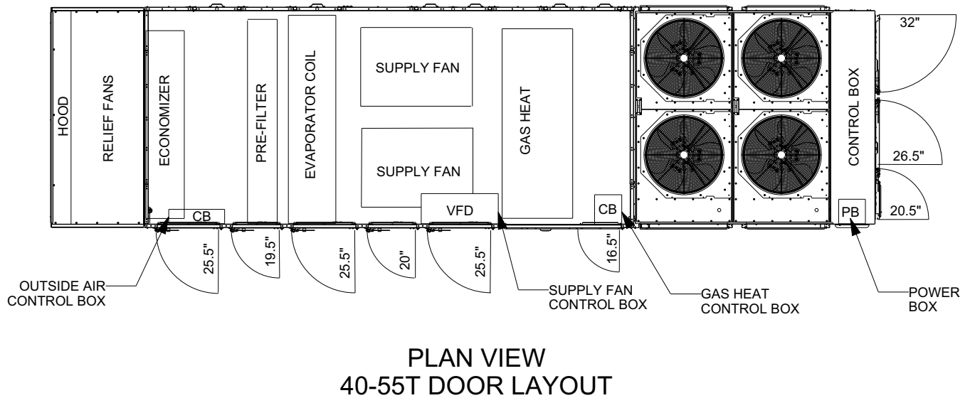
Figure 45. Minimum access clearances – 40 to 55 ton
