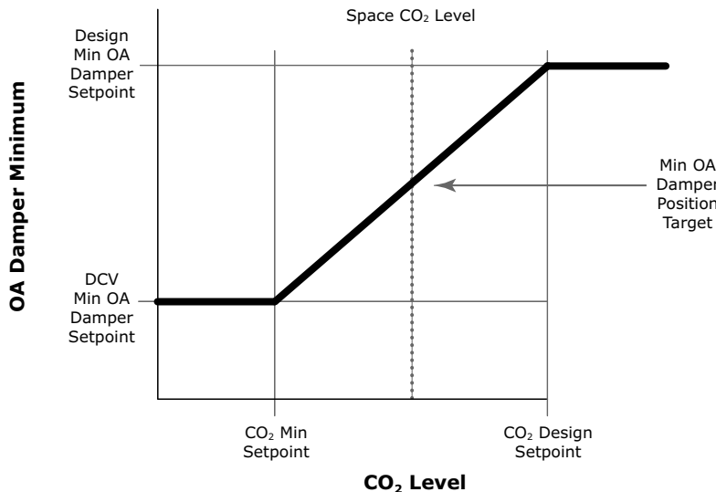
Figure 7. CO 2 control
