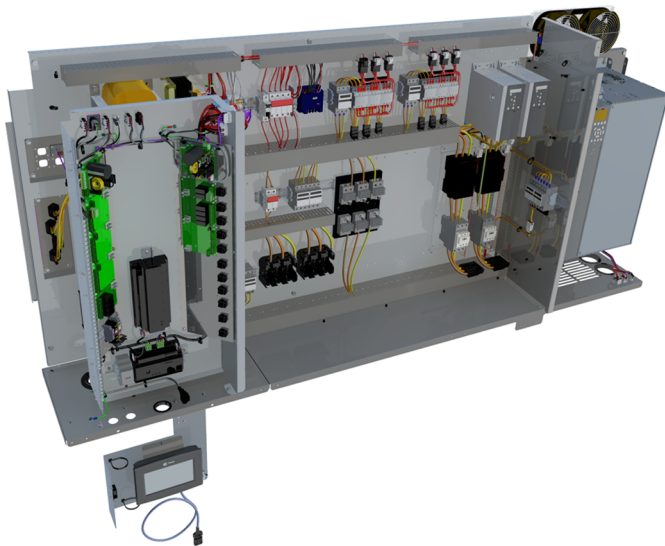
Figure 3. Control panel
