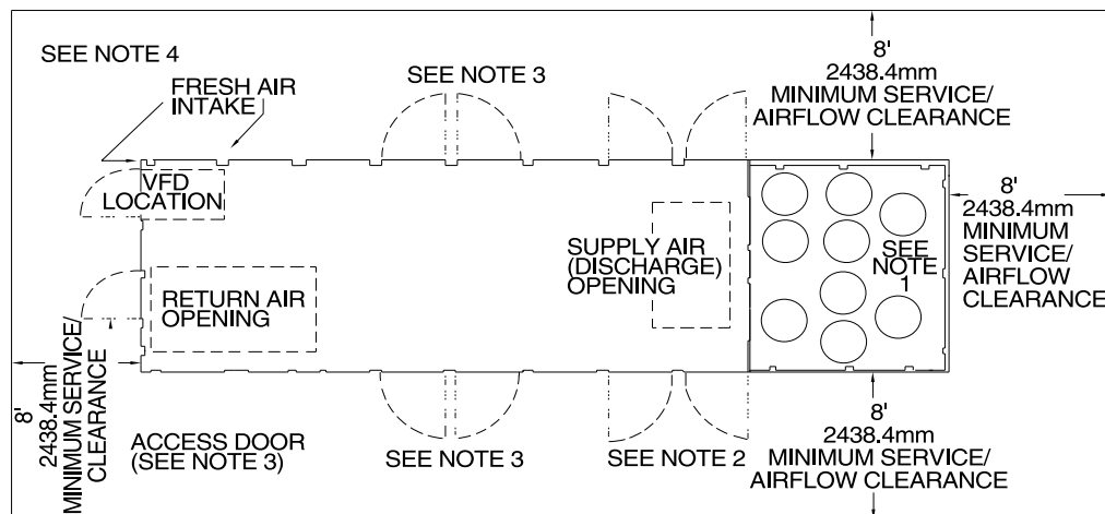
Figure 8. Service clearance — 90 to 130 tons air-cooled
