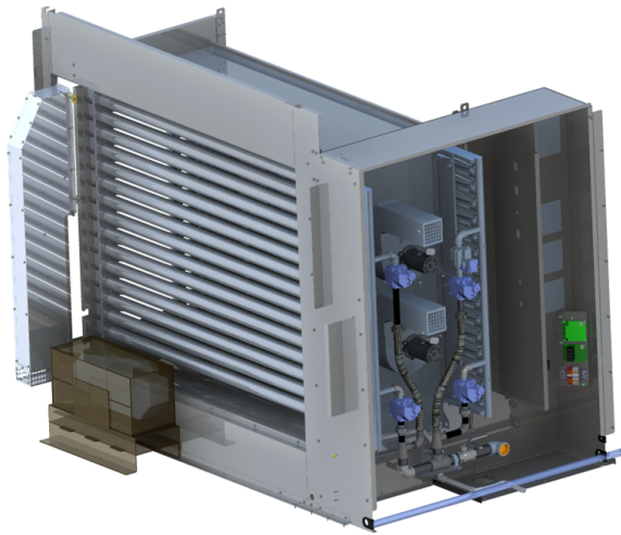
Figure 4. Gas heat configuration
