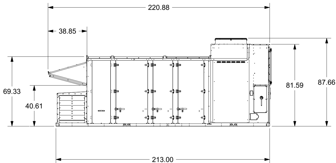
LEFT SIDE VIEW 20-30T / NO HEAT / RELIEF FANS / PANEL FILTERS
