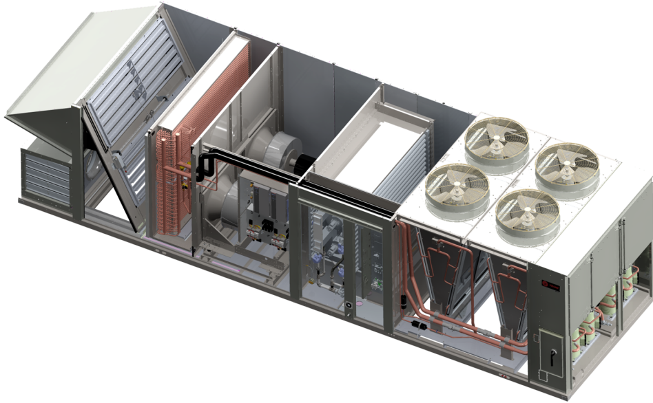
Figure 1. IntelliPak® 3
