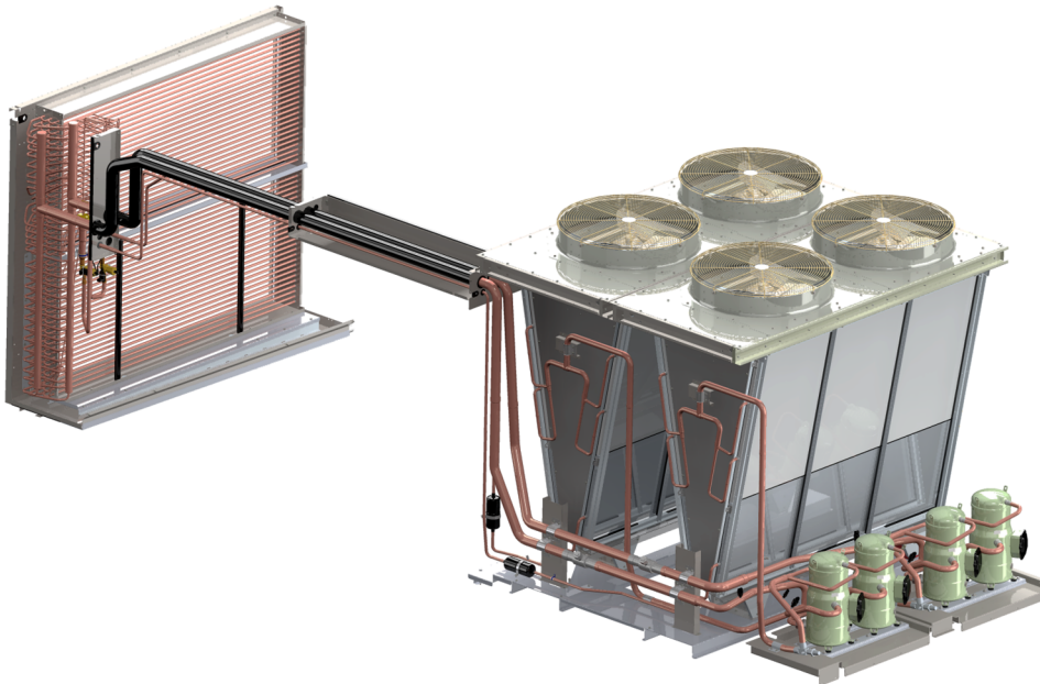
Figure 2. Refrigeration piping
