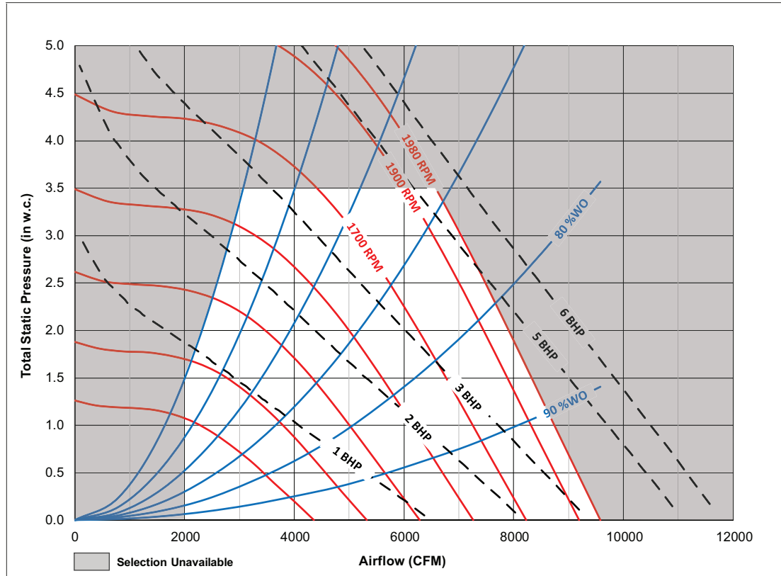
Figure 21. 20 to 25 ton, 6 hp relief fan, single fan
