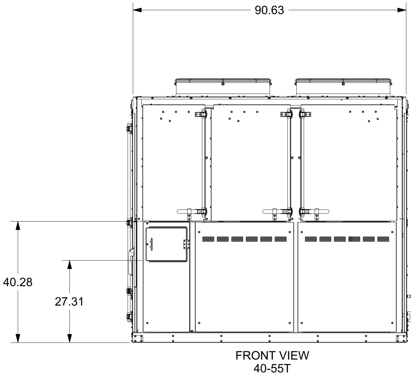
Figure 33. 40 to 55 ton — front view (inches)
