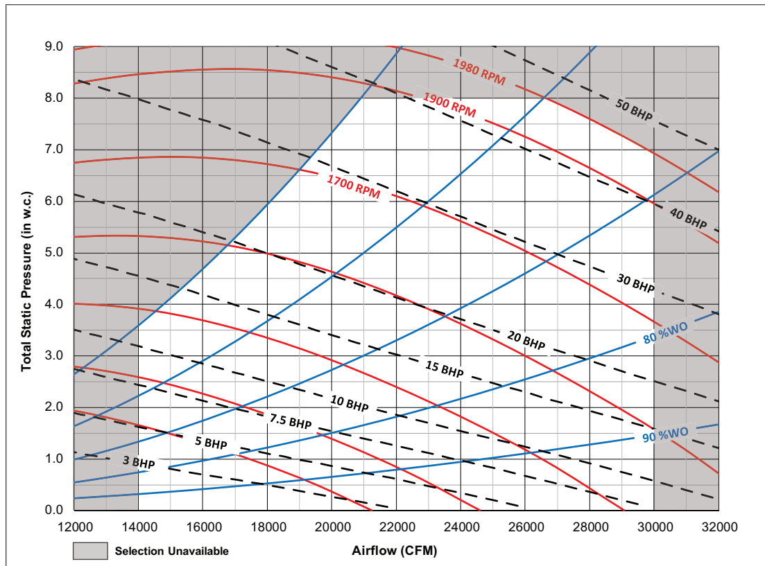
Figure 20. 60 and 75 ton, 27.0 inch - 9 blade - 100% width supply fan
