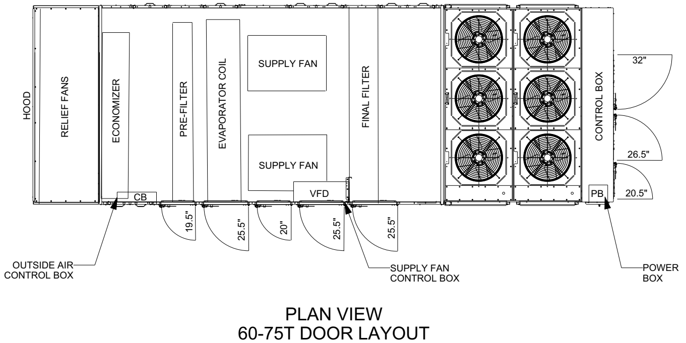
Figure 46. Minimum access clearances – 60 to 75 ton
