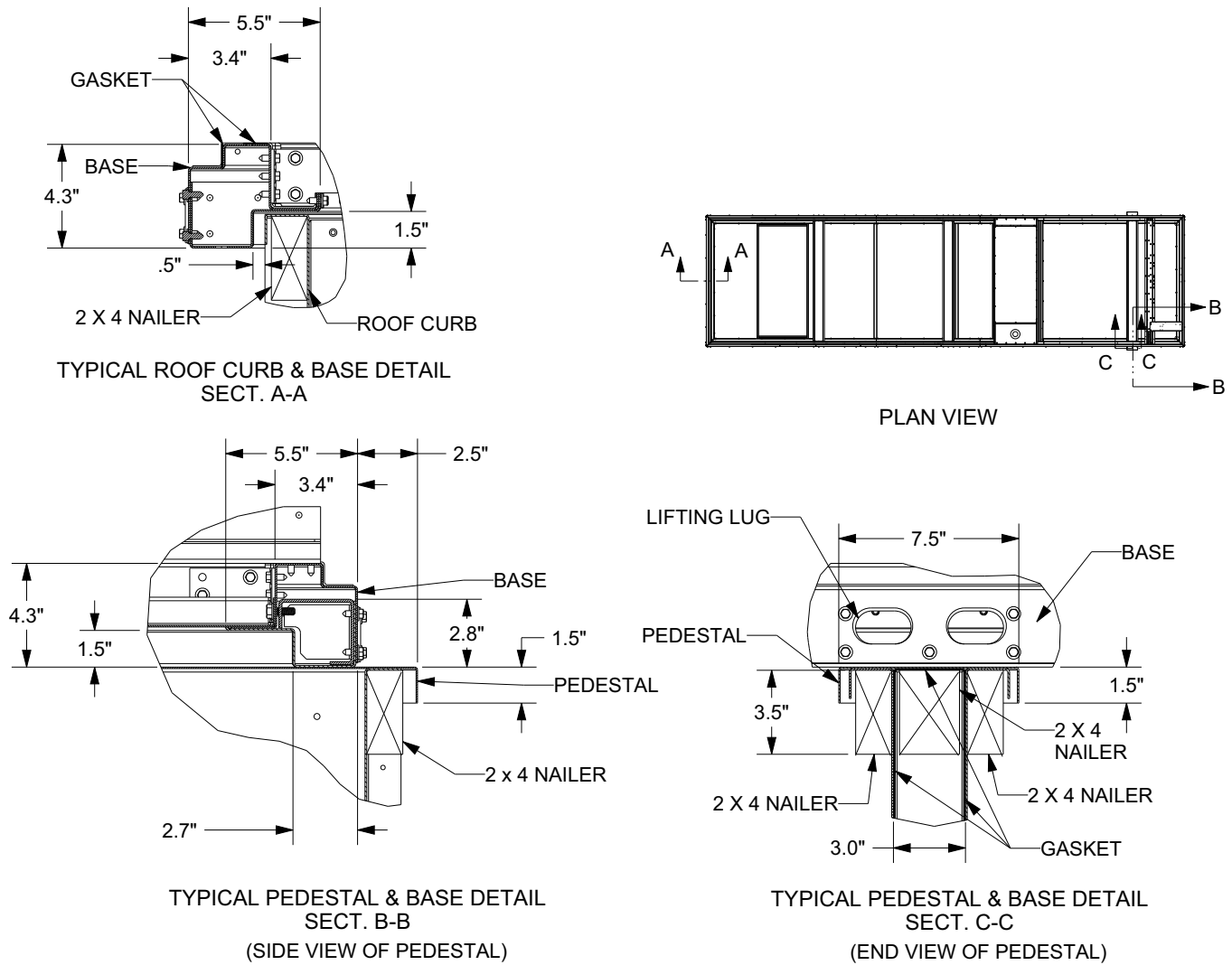
Figure 42. Base and pedestal
