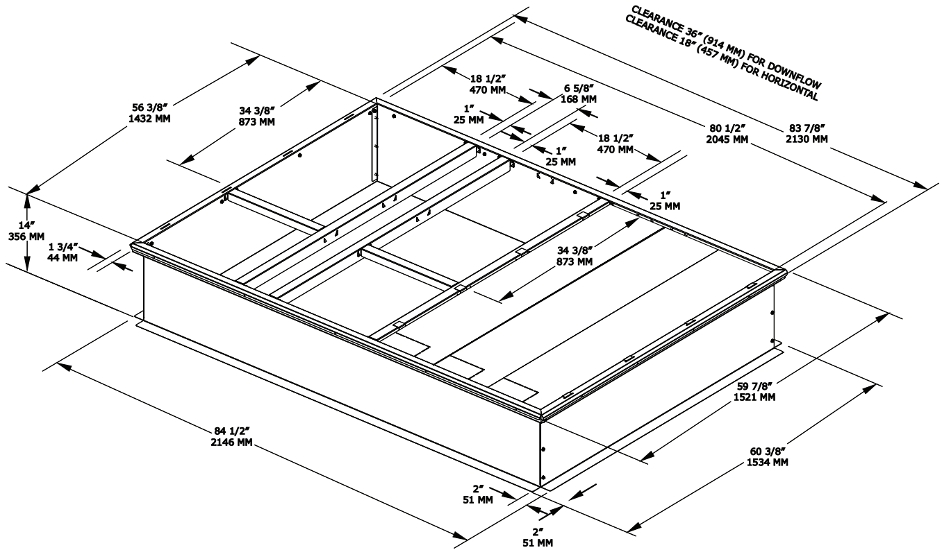
Figure 15. 12.5 tons standard efficiency – roof curb
