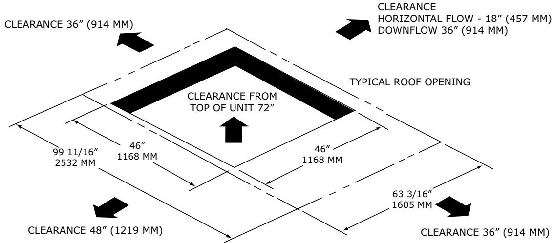
Figure 15. 12.5 tons standard efficiency – roof curb
