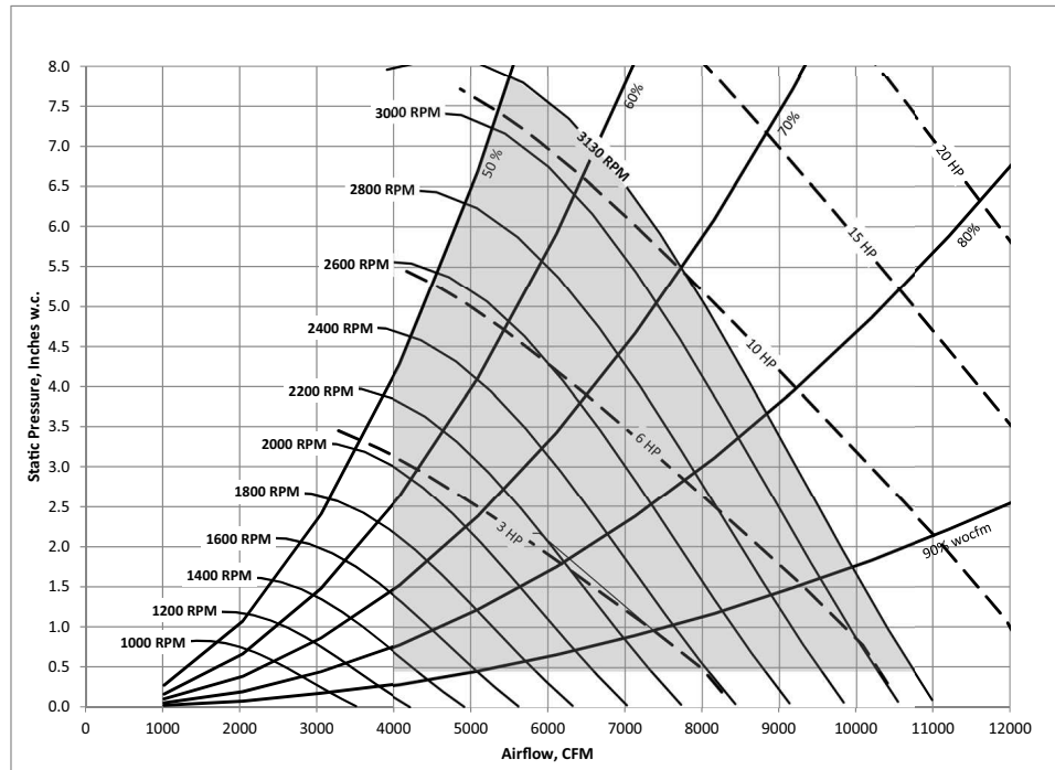
Figure 12. 20, 25 and 30 ton, 16.5 inch - 9 Blade - 80% width supply fan
