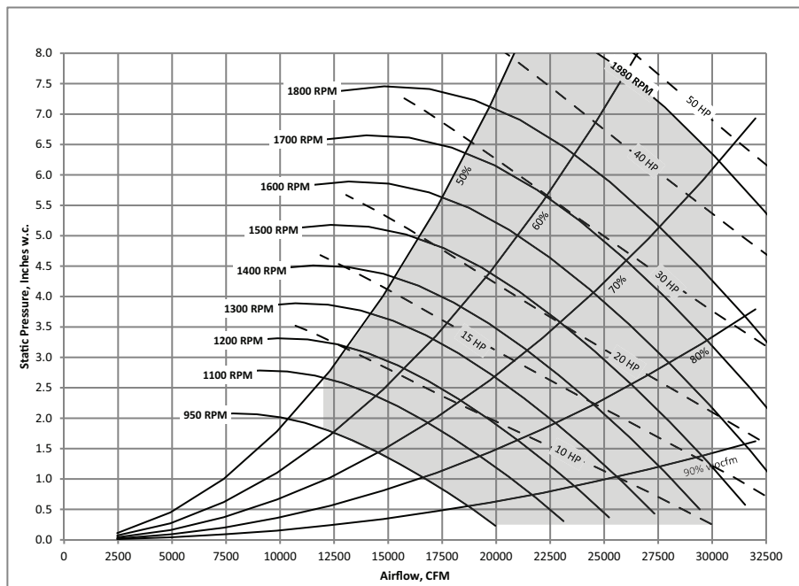
Figure 22. 60 and 75 ton, 27.0 inch - 9 blade - 100% width supply fan
