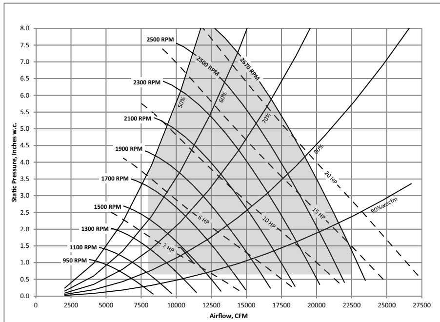
Figure 18. 40, 50 and 55 ton, 20.0 inch - 9 blade - 100% width supply fan
