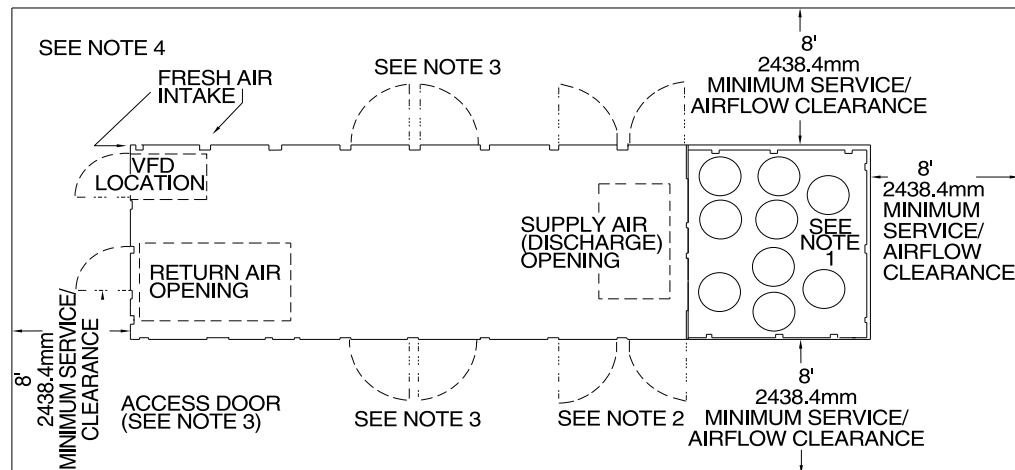
Figure 10. Service clearance — 90 to 130 tons air-cooled
