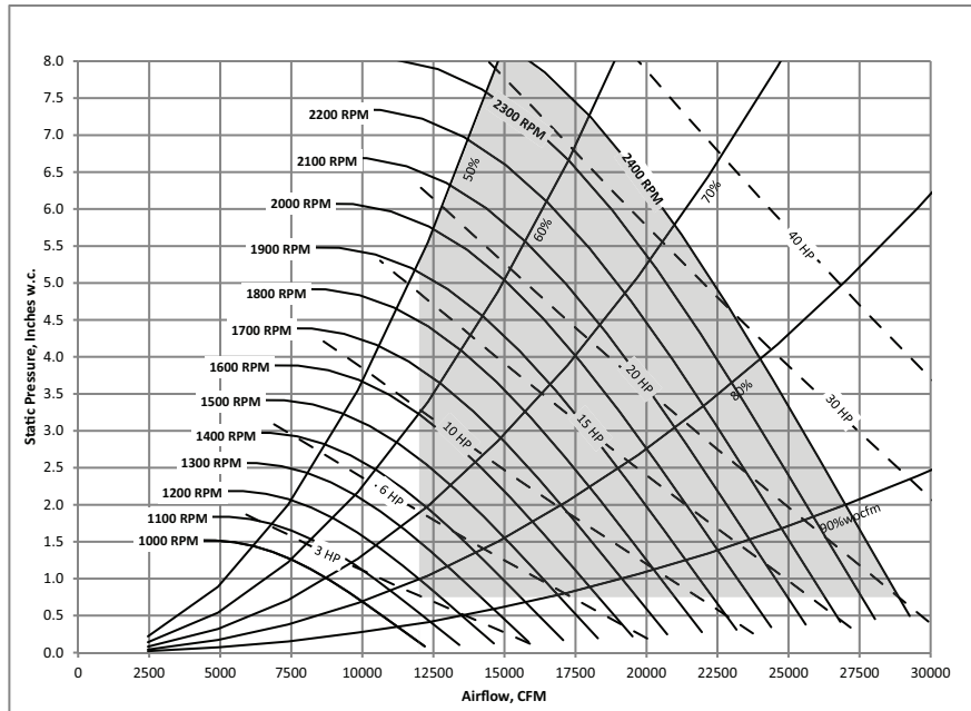
Figure 21. 60, 70 and 75 ton, 22.2 inch - 9 blade - 100% width supply fan
