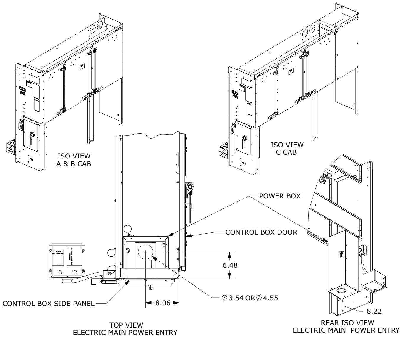
Figure 45. Electrical connections (inches)
