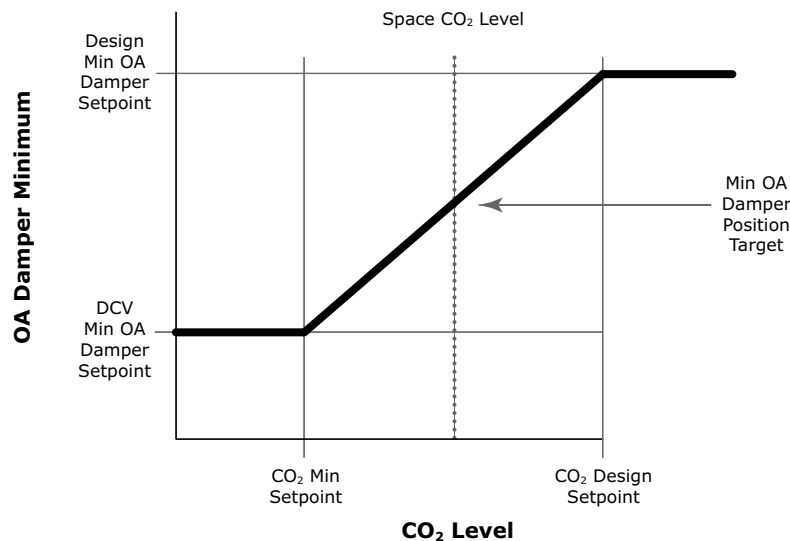
Figure 9. CO 2 control
