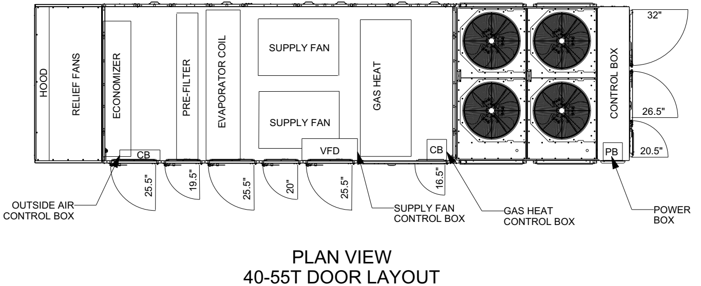
Figure 47. Minimum access clearances – 40 to 55 ton
