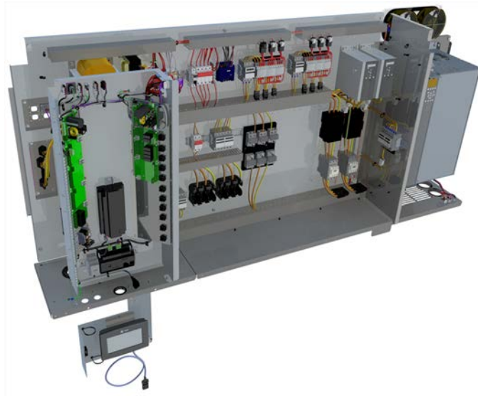
Figure 5. Control panel
