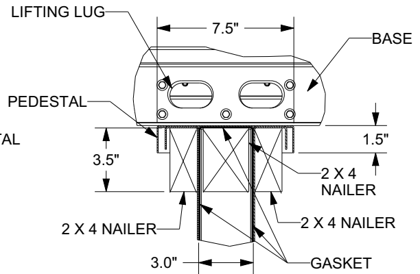
TYPICAL PEDESTAL & BASE DETAIL SECT. C-C (END VIEW OF PEDESTAL)
