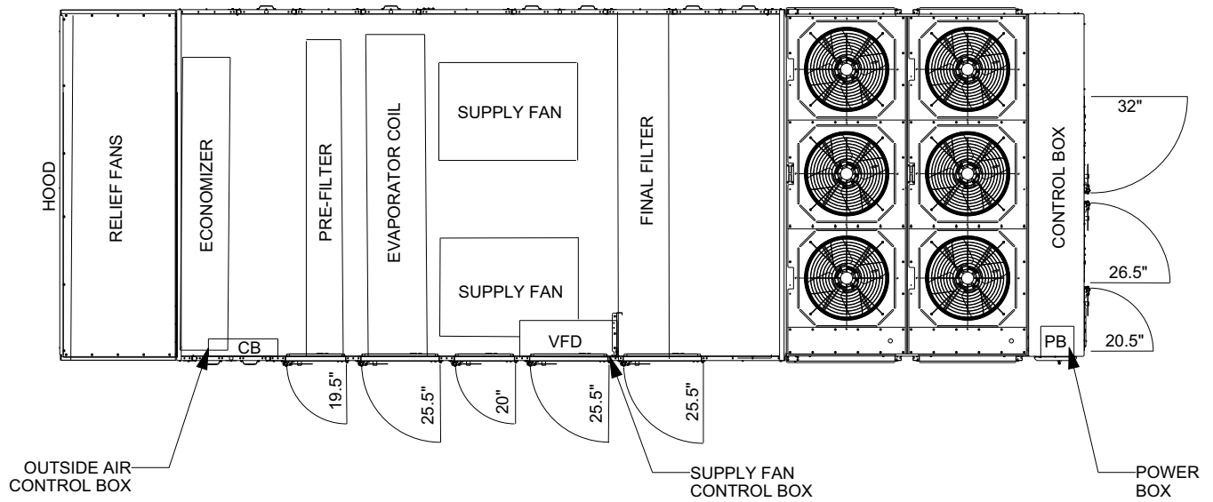
Figure 48. Minimum access clearances – 60 to 75 ton
