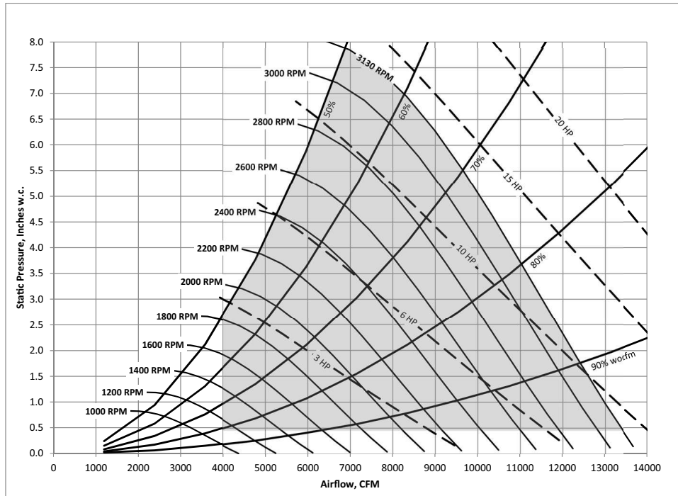
Figure 13. 20, 25 and 30 ton, 16.5 inches - 9 blade - 100% width supply fan
