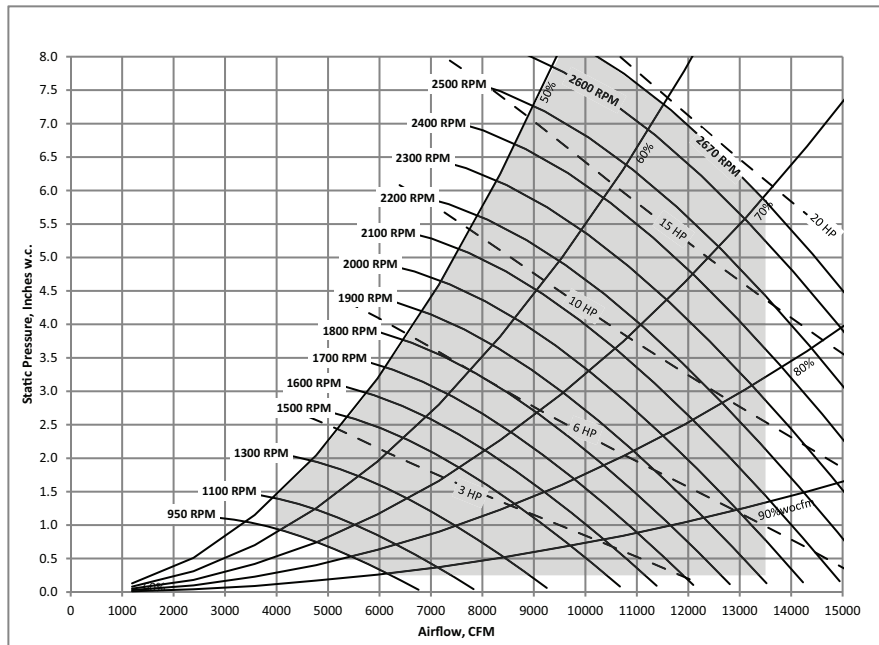
Figure 14. 20, 25 and 30 ton, 20.0 inch - 9 blade - 80% width supply fan
