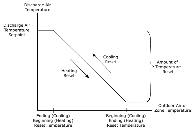
Figure 8. Discharge air temperature reset
