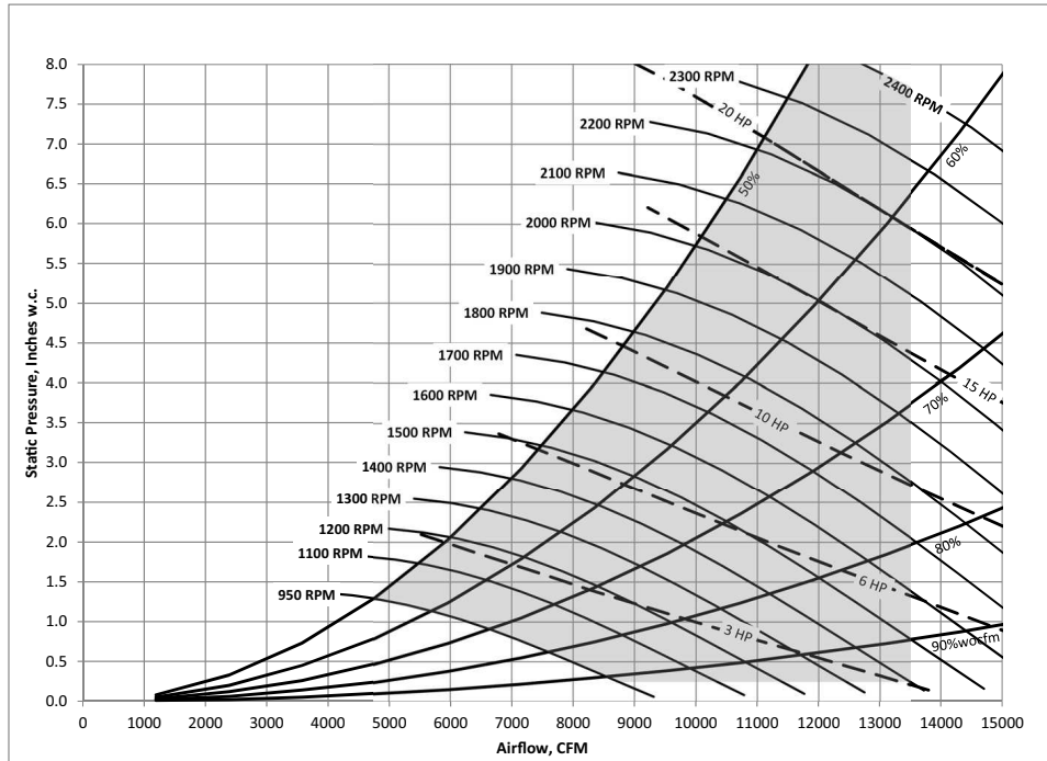
Figure 16. 20, 25 and 30 ton, 22.2 inch - 9 blade - 80% width supply fan
