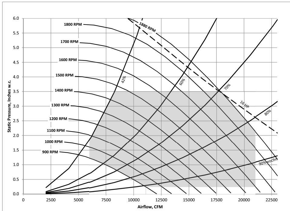
Figure 29. 50 and 55 ton, 16 hp relief fan, two-fan array
