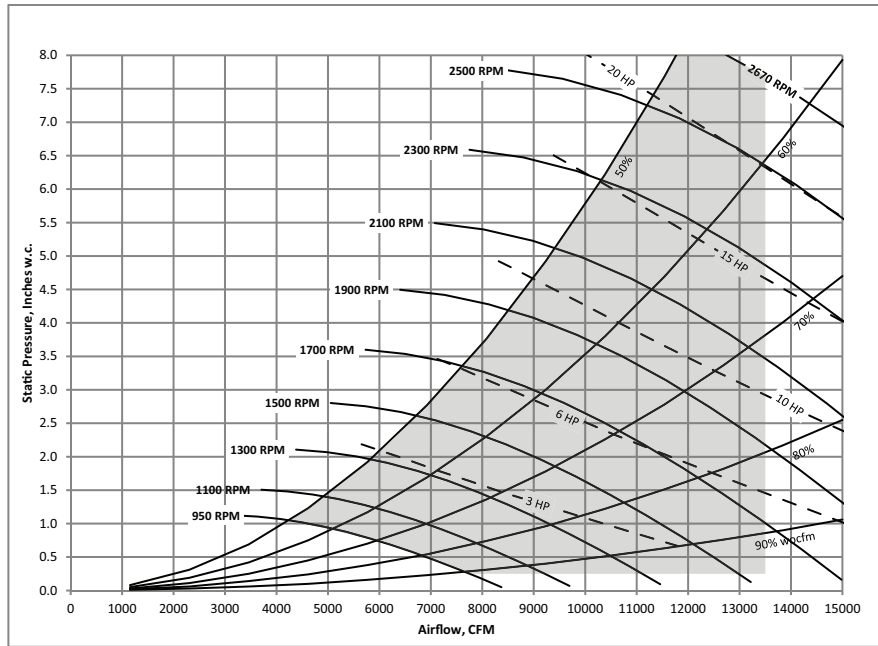
Figure 15. 20, 25 and 30 ton, 20.0 inch - 9 blade - 100% width supply fan
