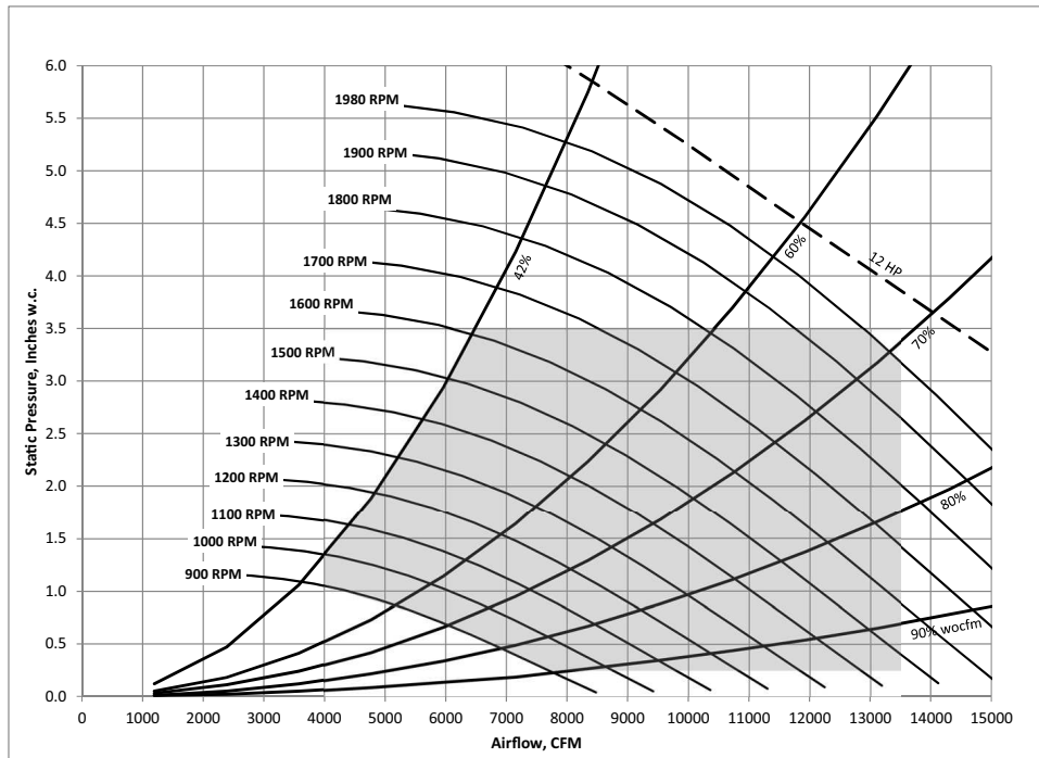
Figure 25. 30 ton, 12 hp relief fan, two-fan array
