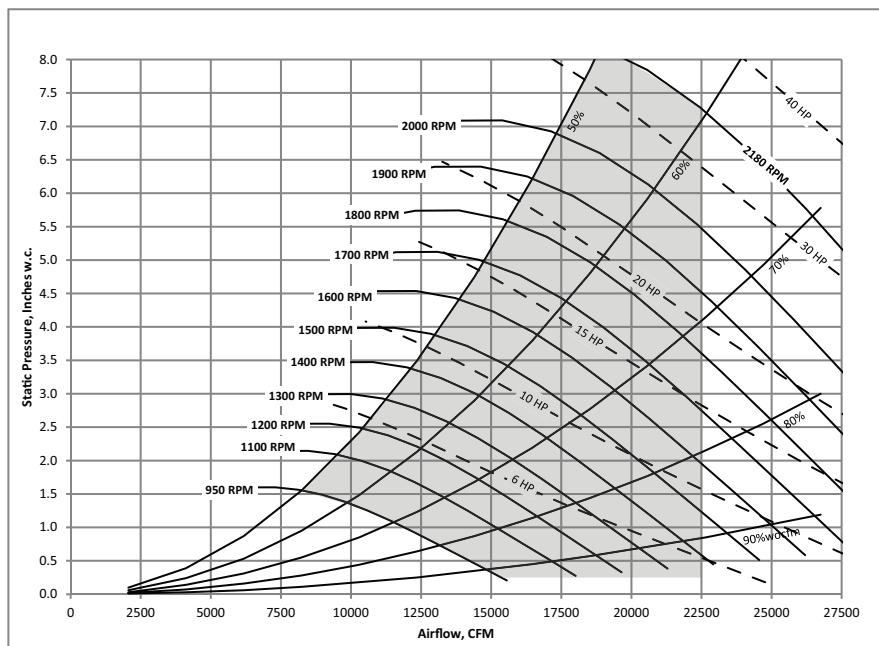
Figure 20. 40, 50 and 55 ton, 24.5 inch - 9 blade - 100% width supply fan
