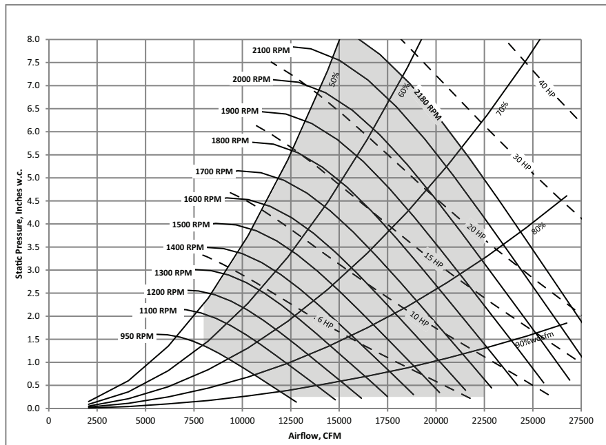
Figure 19. 40, 50 and 55 ton, 24.5 inch - 9 blade - 80% width supply fan
