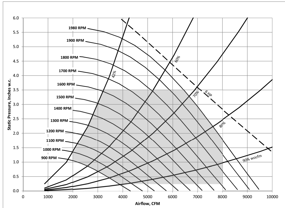
Figure 23. 20 to 25 ton, 6 hp relief fan, single fan
