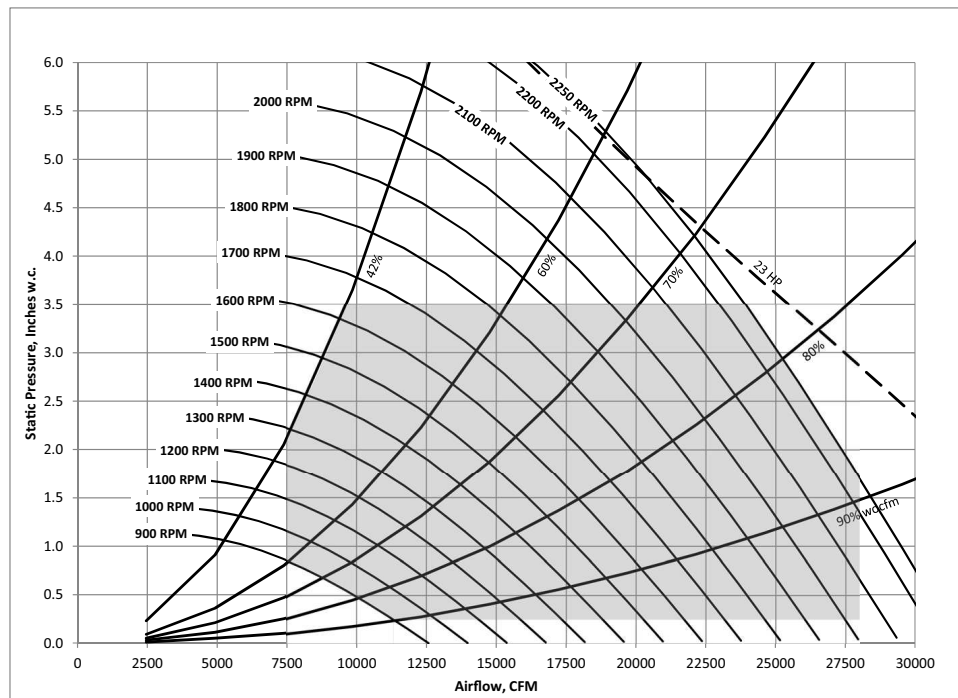
Figure 31. 60, 70 and 75 ton, 23 hp relief fan, three-fan array
