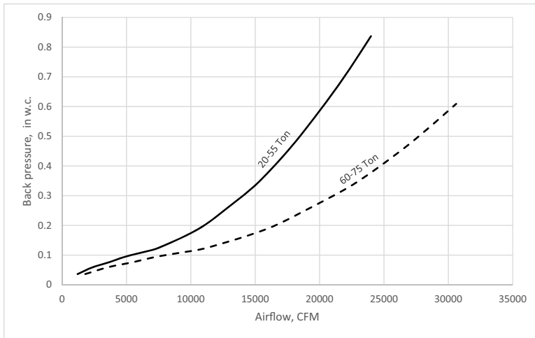
Figure 32. Barometric Relief Damper Performance
