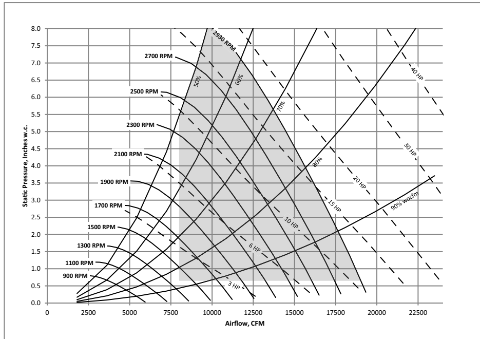
Figure 17. 40, 50 and 55 ton, 18.2 inch - 9 blade - 100% width supply fan
