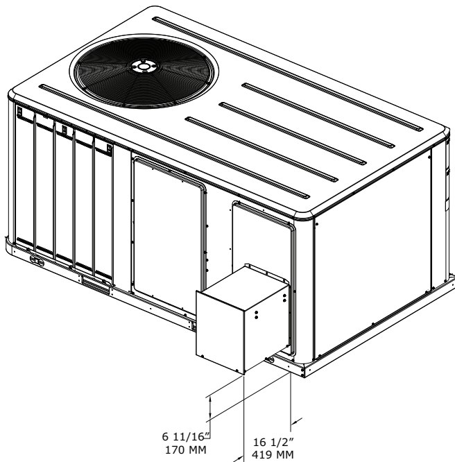
Figure 28. Cooling and gas/electric - 6 to 8.5 tons ultra high efficiency - power exhaust (a)
