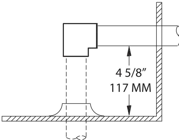
Figure 31. Gas/electric - 6 to 10 tons ultra high efficiency - height of gas pipe required from inside of base of unit to gas shut-off assembly (factory provided) YZC models only (a)
