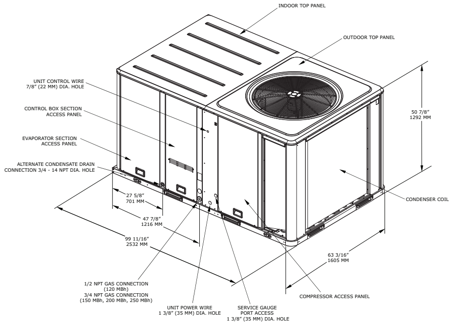
Figure 32. Cooling and gas/electric - 10 tons ultra high efficiency (a)
