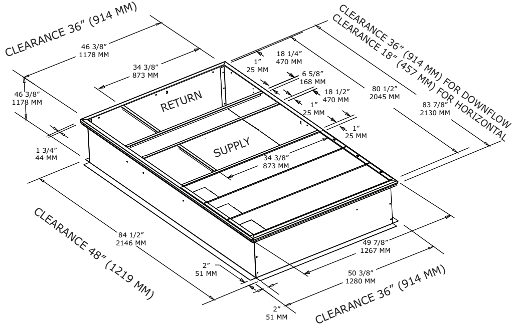
Figure 26. Cooling and gas/electric - 6 to 8.5 tons ultra high efficiency - roof curb (a)
