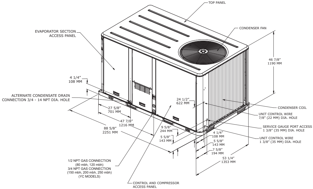
Figure 22. Cooling and gas/electric - 6 to 8.5 tons ultra high efficiency (a)
