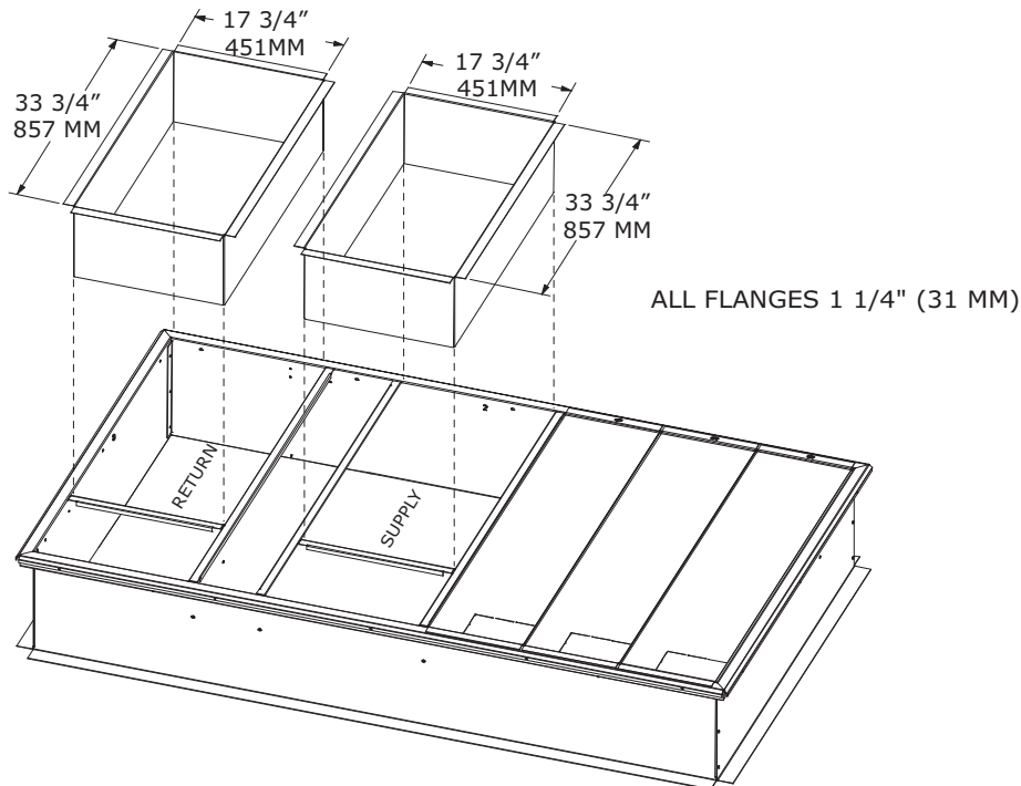
Figure 27. Cooling and gas/electric - 6 to 10 tons ultra high efficiency - duct connections field fabricated (a)
