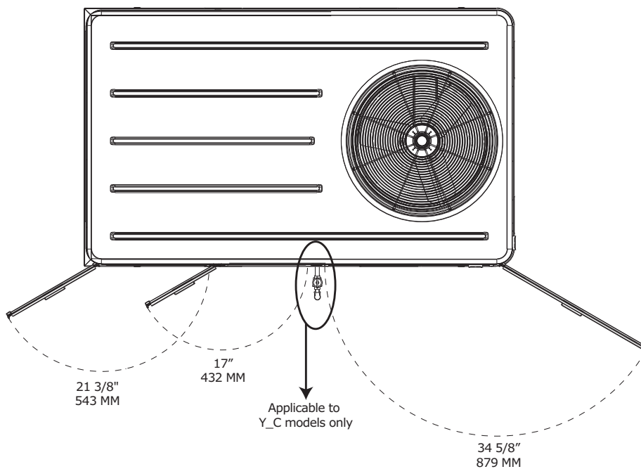
Figure 21. Cooling and gas/electric - 4 to 5 tons ultra high efficiency- swing diameter for hinged door(s) option (a)
