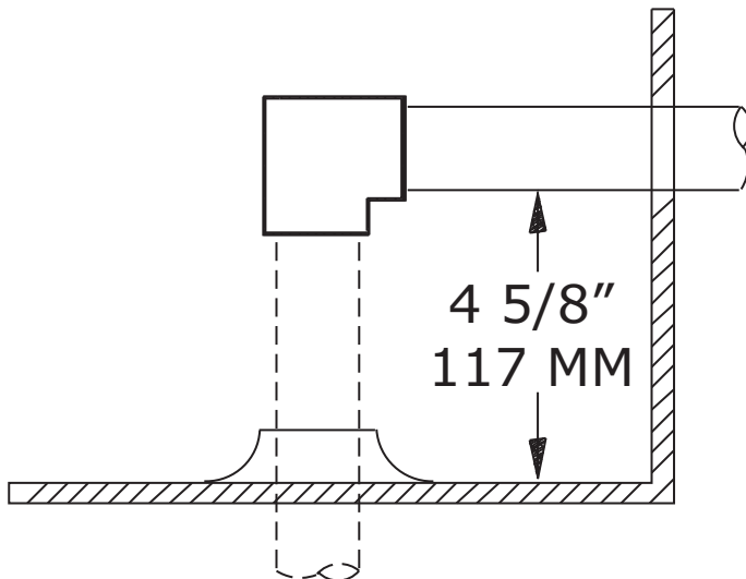
Figure 13. Gas/electric models - 3 tons ultra high efficiency- height of gas pipe required from inside base of unit to gas shut off assembly (factory provided) - Y_C models only (a)
