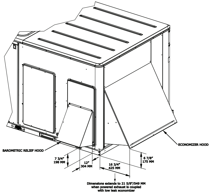
Figure 30. Cooling and gas/electric - 6 to 10 tons ultra high efficiency - economizer, manual or motorized fresh air damper (a)
