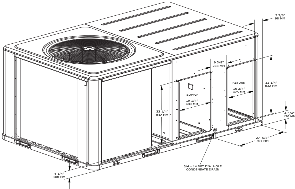
Figure 24. Cooling and gas/electric - 6 to 10 tons ultra high efficiency - horizontal airflow supply and return (a)
