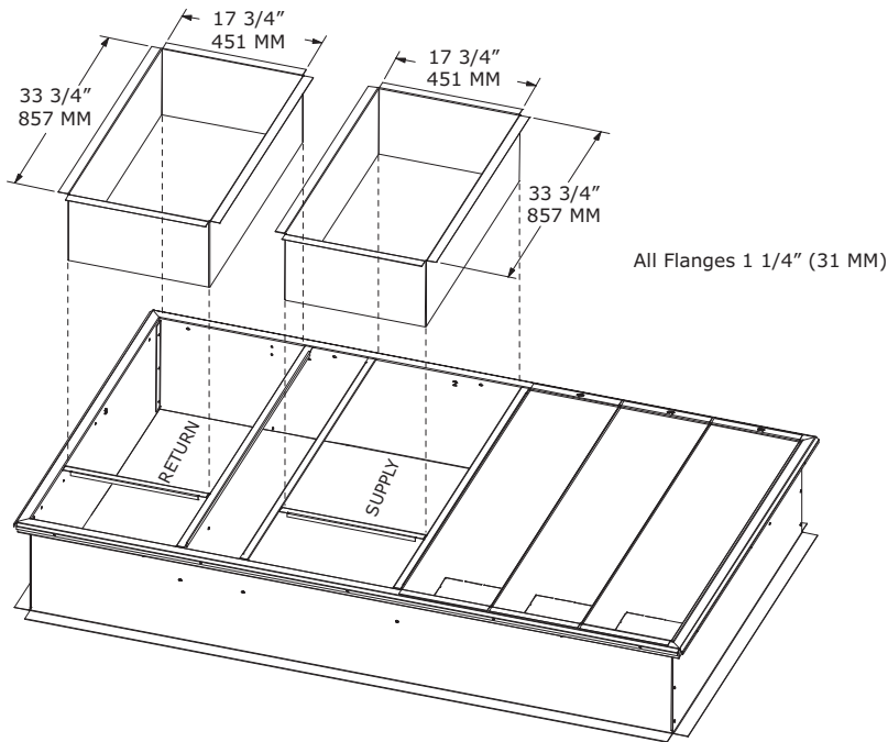
Figure 20. Cooling and gas/electric - 4 to 5 tons ultra high efficiency - economizer, manual or motorized fresh air damper (a)
