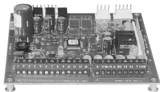
Figure 3. ReliaTel™ board
