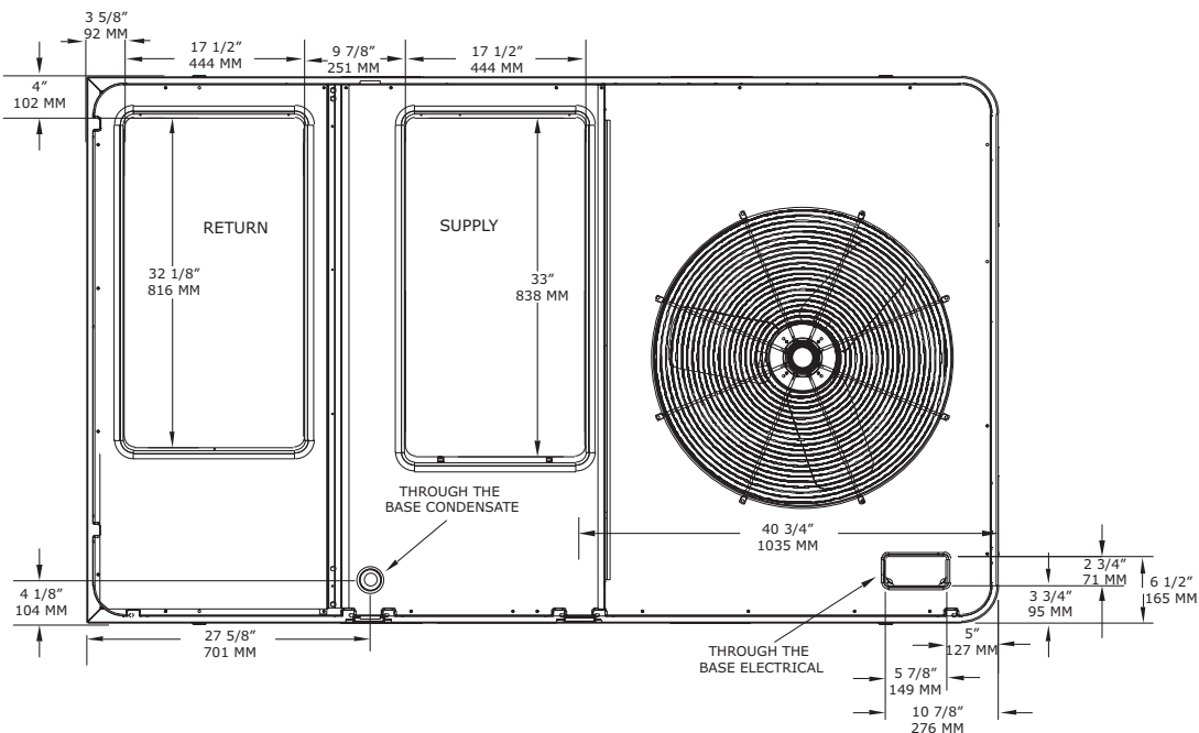
Figure 23. Cooling and gas/electric - 6 to 8.5 tons ultra high efficiency - downflow supply/return through-the-base utilities (a)
