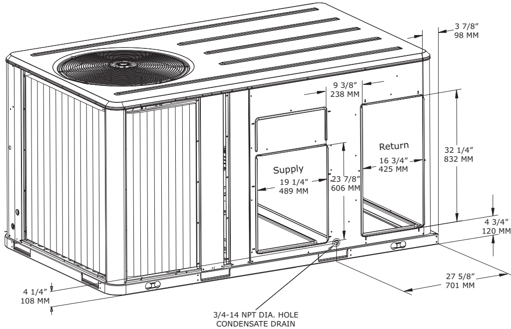
Figure 16. Cooling and gas/electric - 4 to 5 tons ultra high efficiency- horizontal airflow supply and return (a)
