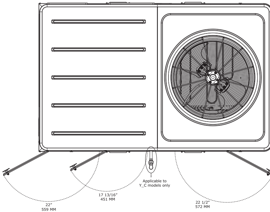
Figure 37. Cooling and gas/electric - 10 tons ultra high efficiency - swing diameter for hinged door(s) option (a)
