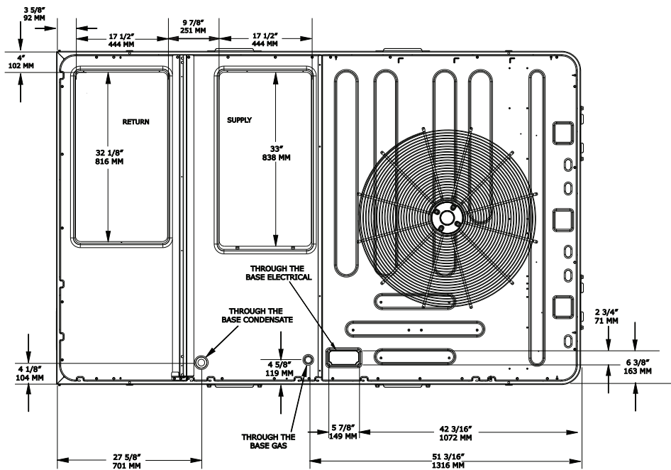
Figure 33. Cooling and gas/electric - 10 tons ultra high efficiency - downflow airflow supply/return, through-the-base utilities (a)
