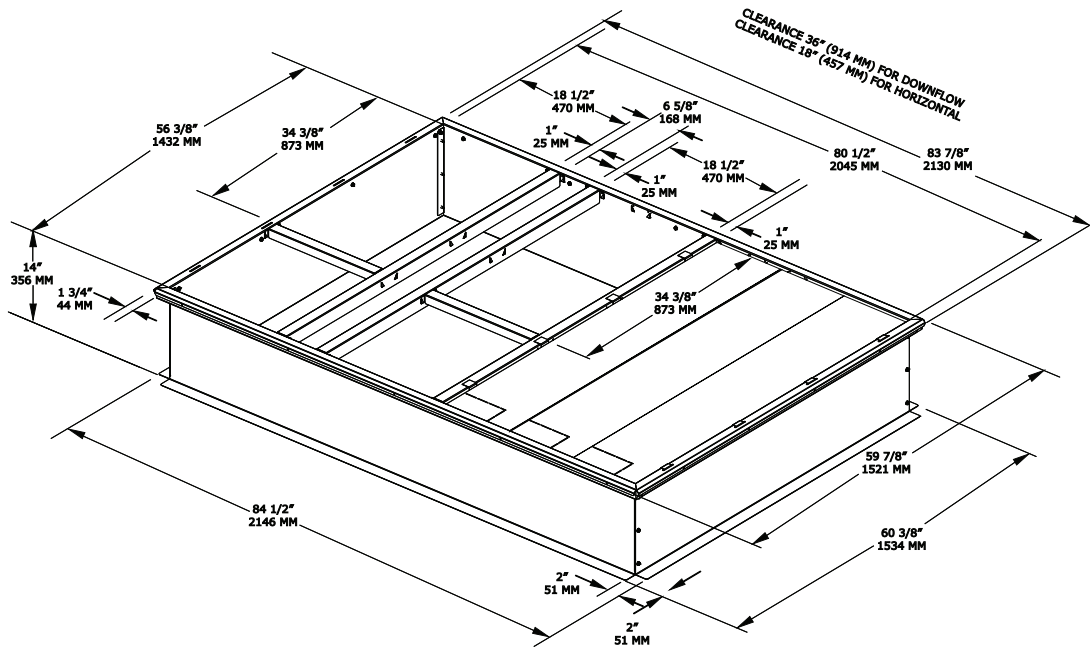
Figure 35. Cooling and gas/electric - 10 tons ultra high efficiency - roof curb (a)
