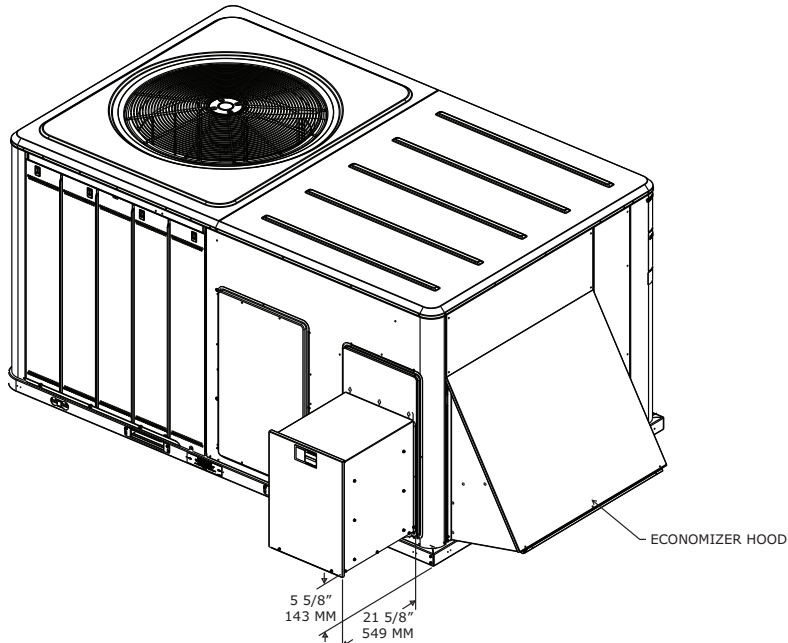
Figure 36. Cooling and gas/electric - 10 tons ultra high efficiency - power exhaust (a)
