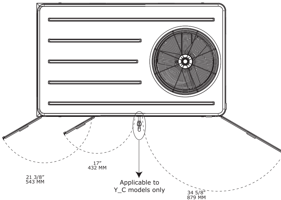
Figure 29. Cooling and gas/electric - 6 to 8.5 tons ultra high efficiency - swing diameter for hinged door(s) option (a)
