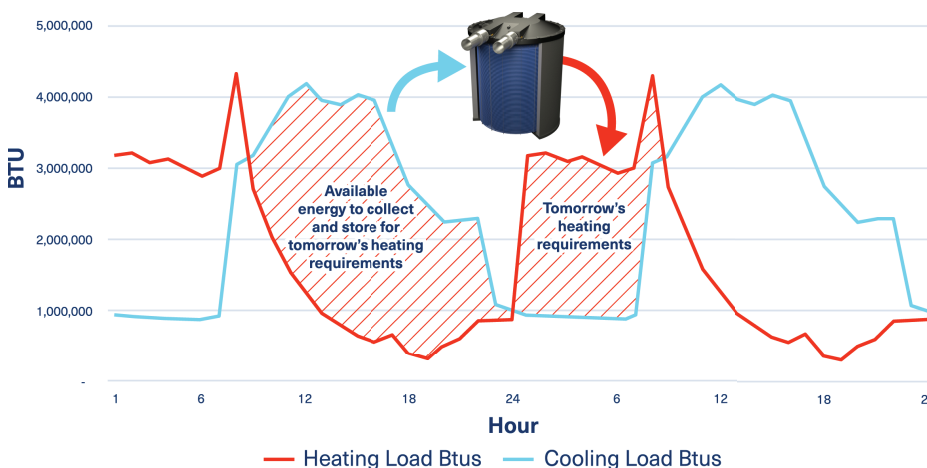
Figure 1. Winter peak heating and cooling load profile
