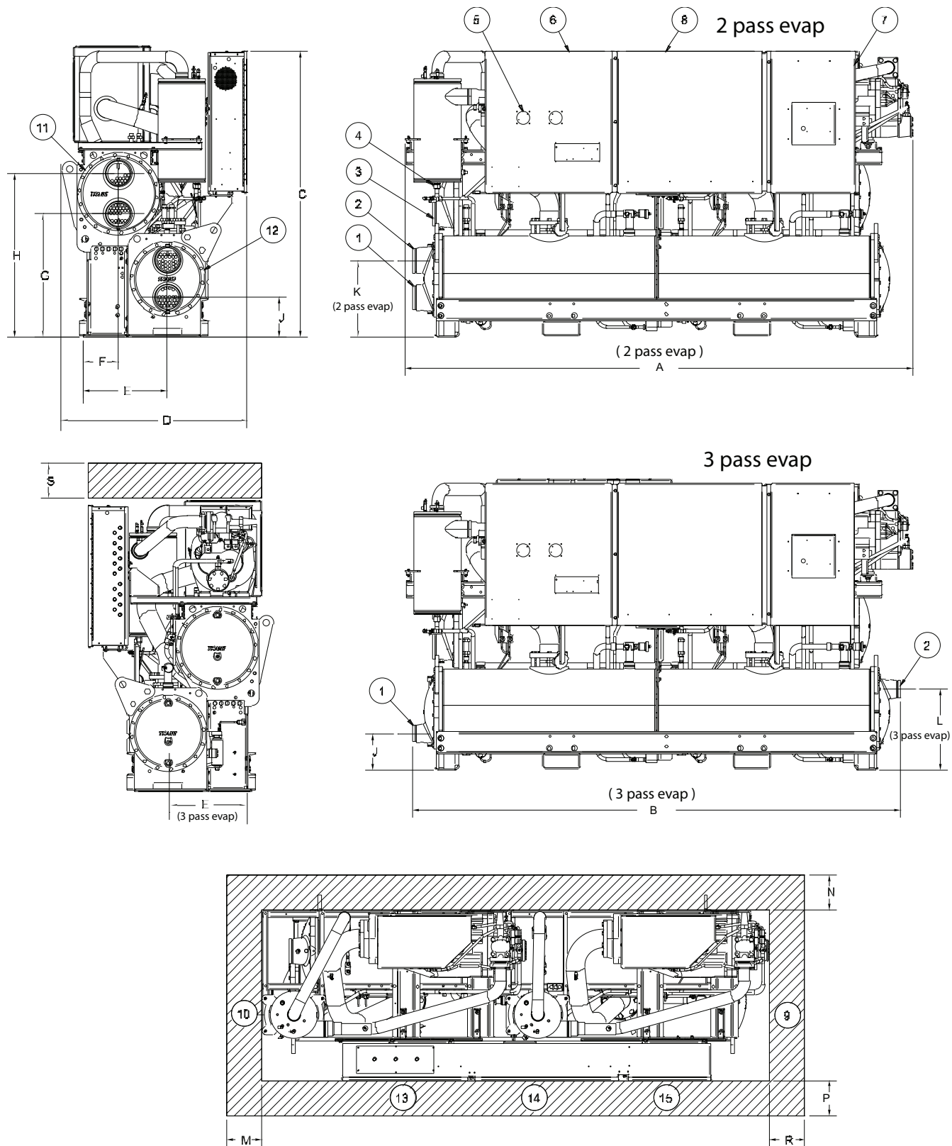
Figure 3. RTWD, 150 to 250 tons, 60 Hz
