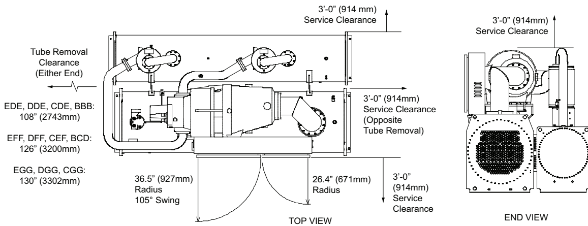
Figure 8. Service clearances
