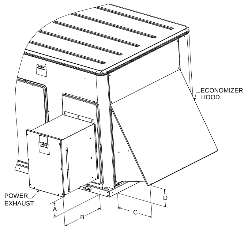
Figure 43. A.0, B.0 and C.0 cabinets – power exhaust with standard economizer
