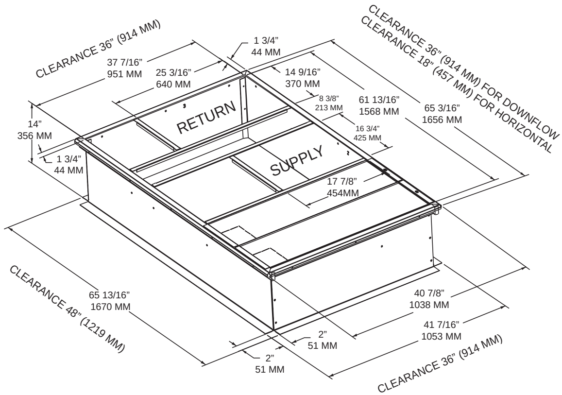
Figure 26. A.0 cabinet – roof curb
