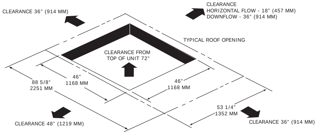
Figure 33. B.O cabinet – roof curb
