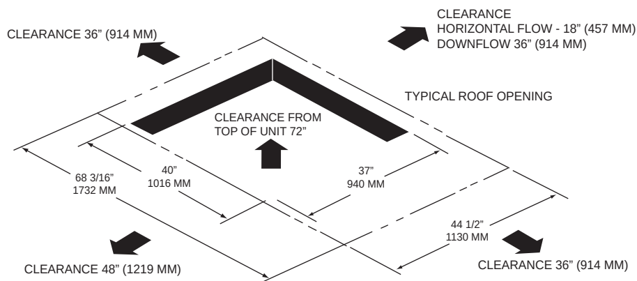
Figure 25. A.0 cabinet – unit clearance and roof opening
