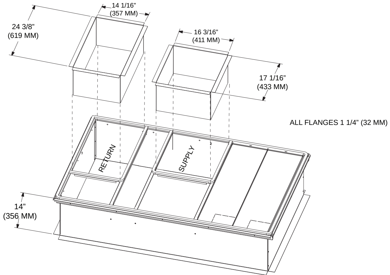
Figure 27. A.0 cabinet – downflow duct connections, field fabricated
