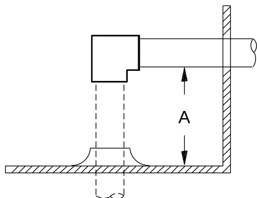
Figure 52. Gas pipe height
