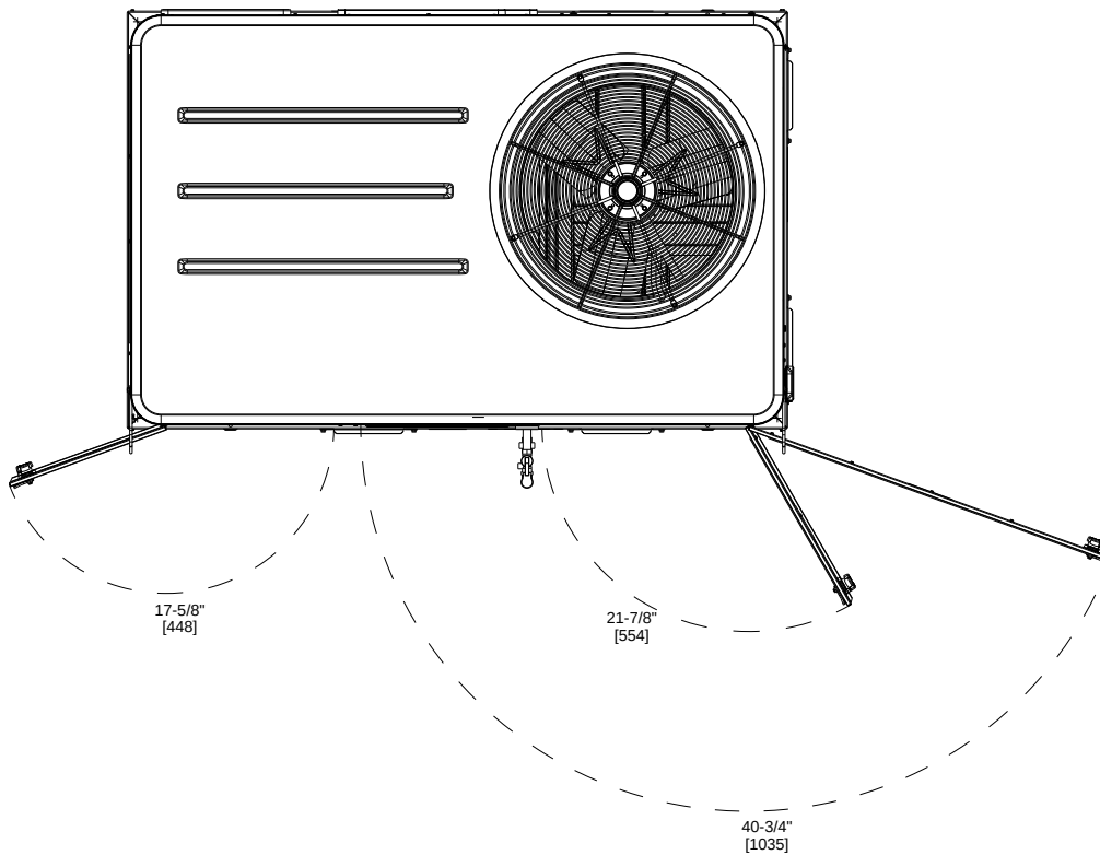
Figure 29. B.0 cabinet
