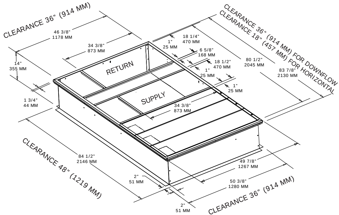
Figure 33. B.O cabinet – roof curb
