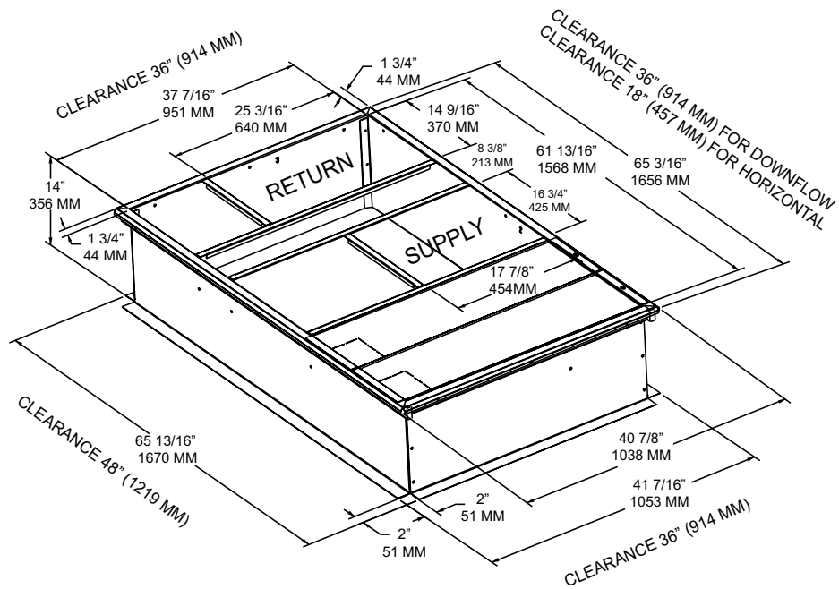
Figure 19. A.O cabinet – downflow duct connections, field fabricated
