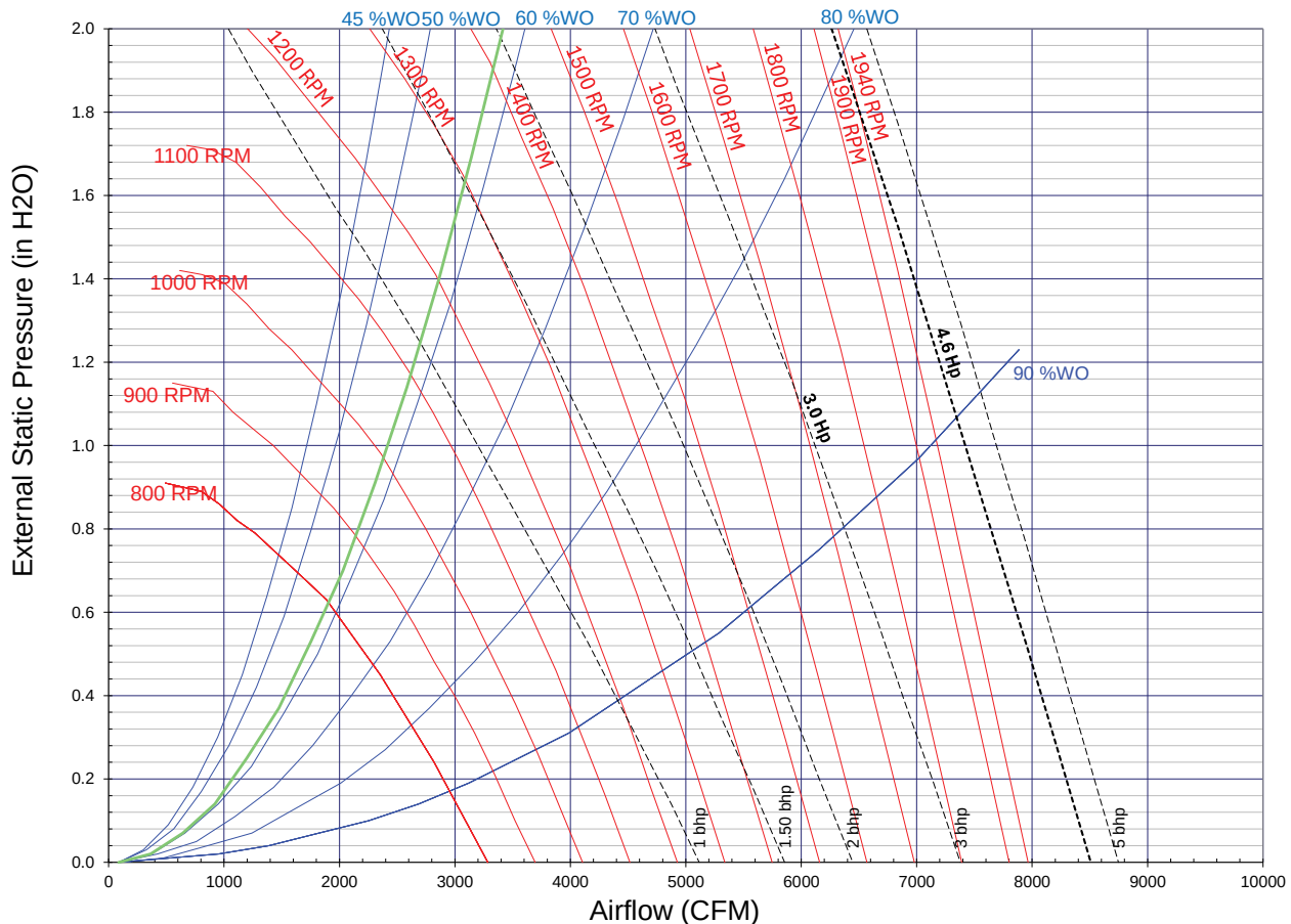
Figure 6. Fan curves — 10 ton (model WHK), downflow
