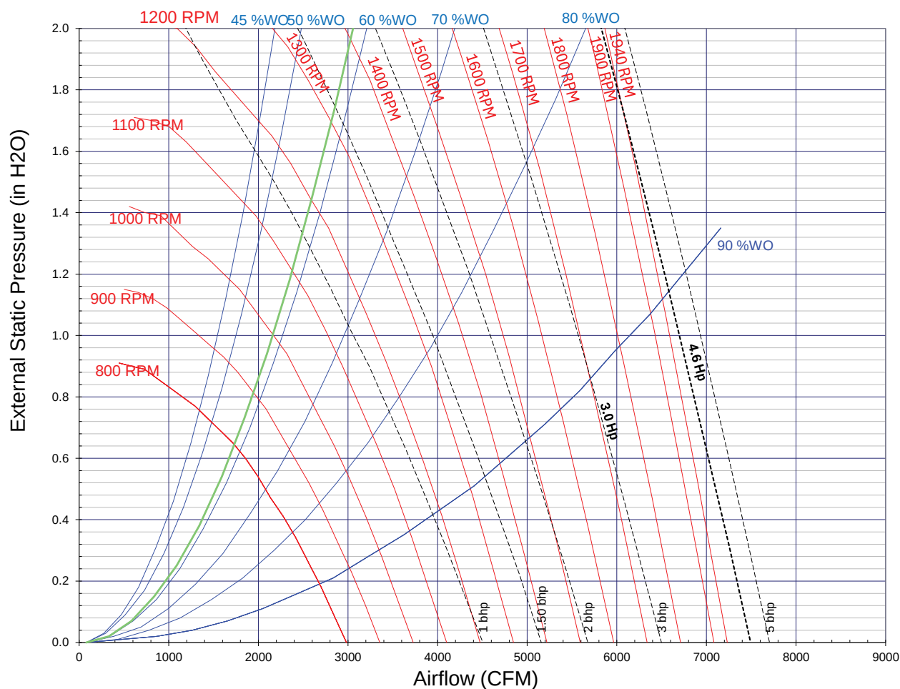
Figure 8. Fan curves — 6 to 8.5 tons (model WSK, WHK), 10 Ton (WSK), horizontal
