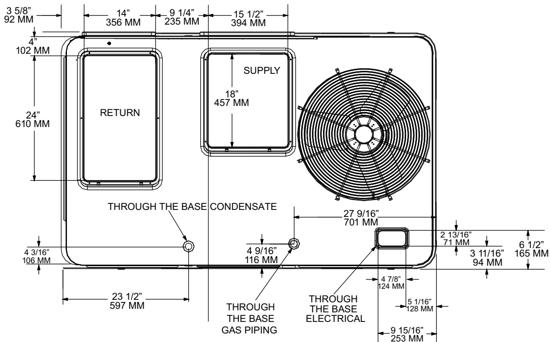
Figure 15. A.O cabinet – downflow airflow supply/return, through-the-base utilities
