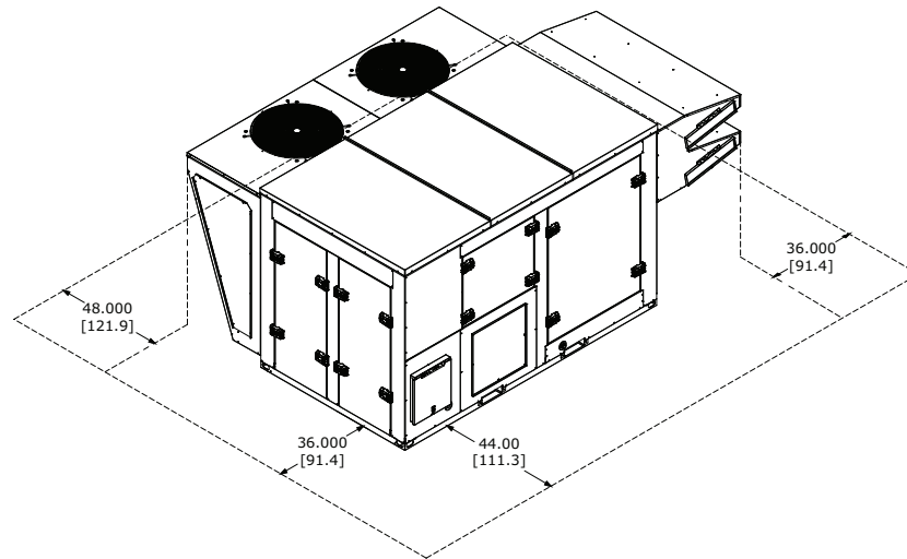
Figure 12. Installation clearances for units with no powered exhaust or ERV, in. (cm)
