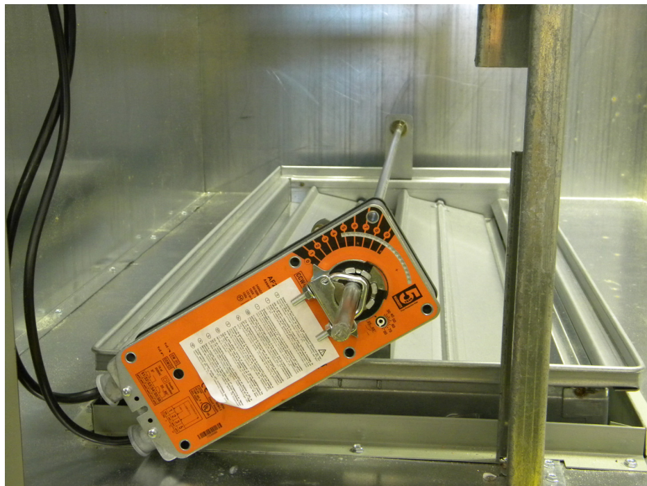
Figure 46. Return air damper
