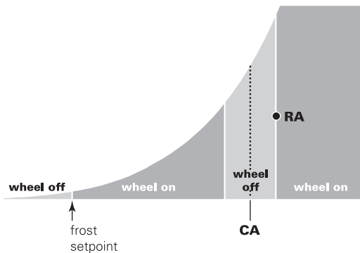
Figure 10. Dry-bulb control in a neutral DB/dry DP application
