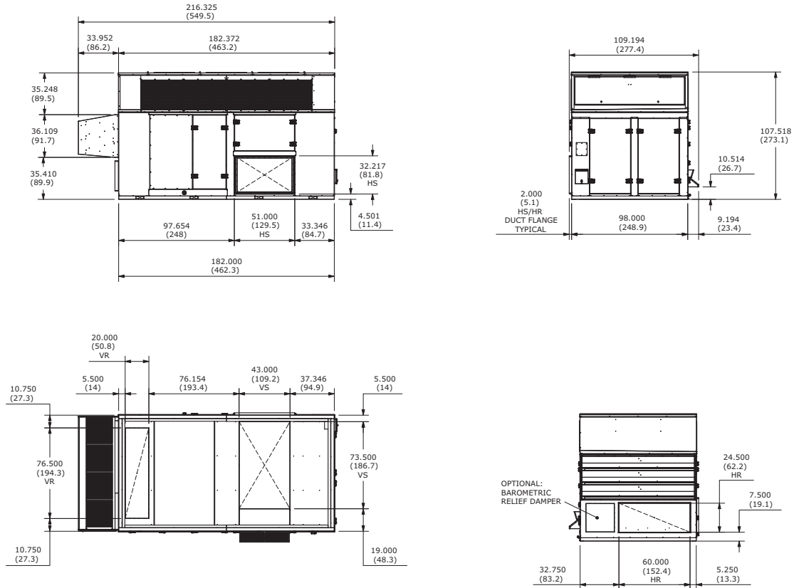
Figure 29. Unit dimensional data for OAN unit with no powered exhaust or ERV, in. (cm)
