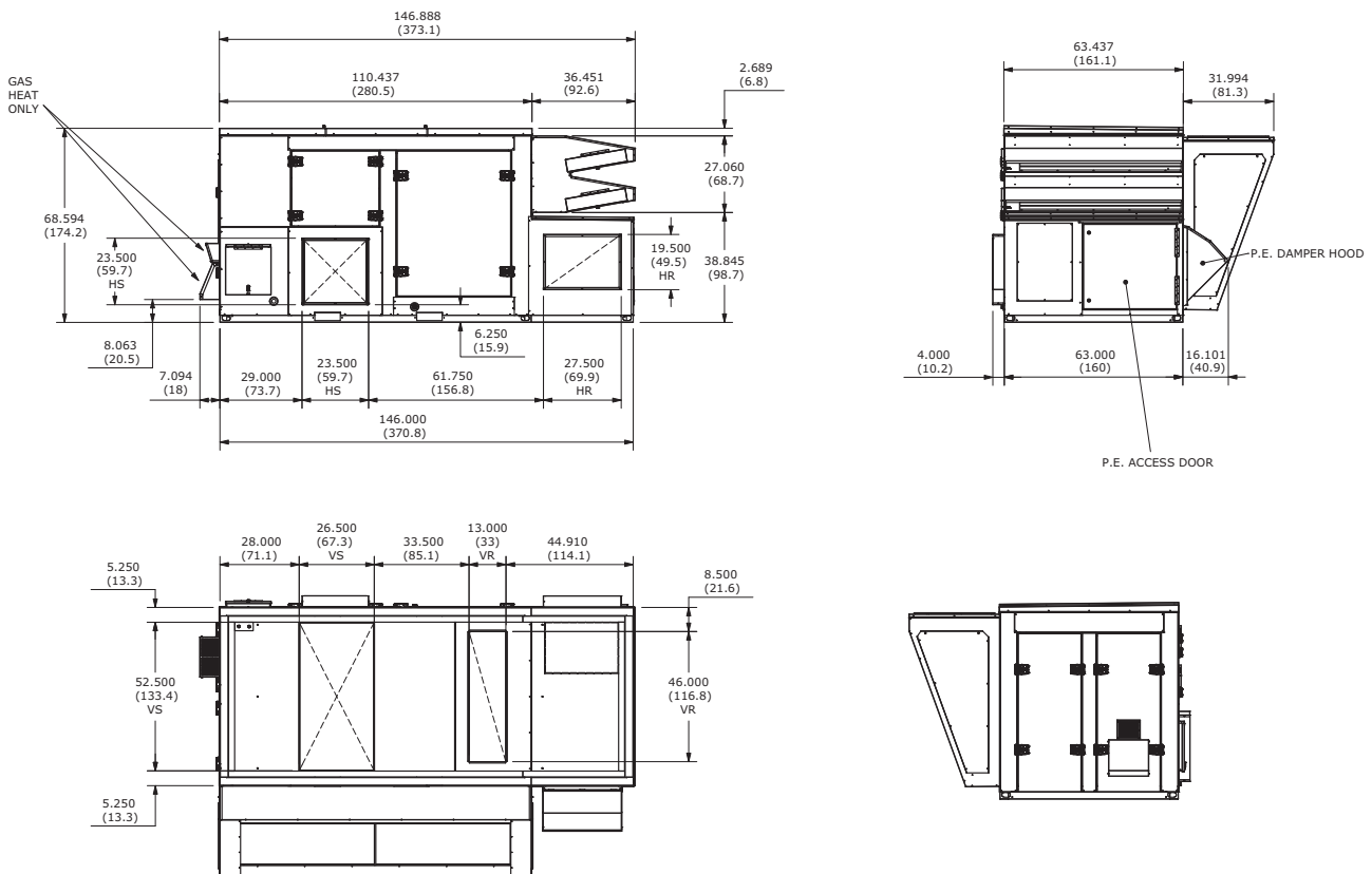
Figure 20. Unit dimensional data for OAD cabinet with powered exhaust but no ERV, in. (cm)
