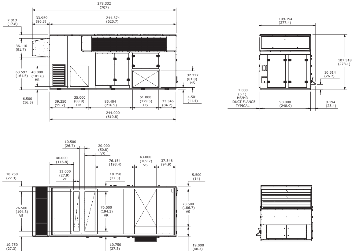
Figure 30. Unit dimensional data for OAN cabinet with powered exhaust but no ERV, in. (cm)
