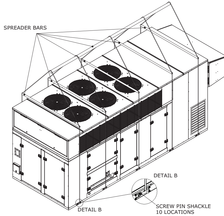
Figure 39. Ten-point lift (OAN cabinet with exhaust fan and no ERV)
