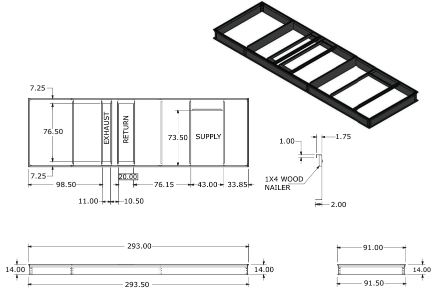
Figure 28. Unit curb data for OAN cabinet with ERV, in. (cm)
