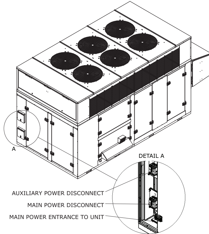
Figure 34. OAN power entrance
