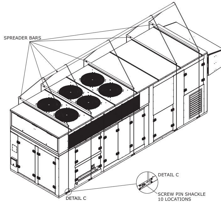
Figure 40. Ten-point lift (OAN cabinet with ERV)
