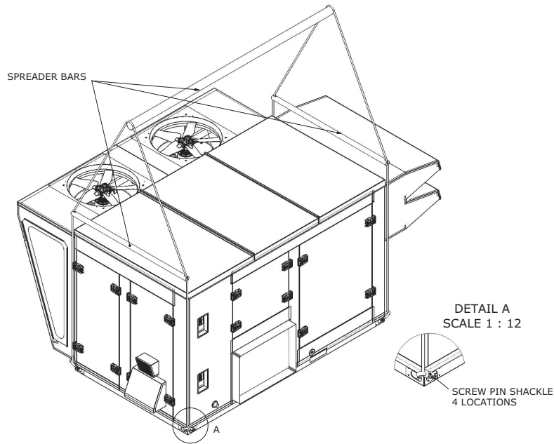
Figure 35. Four-point lift (OAD cabinet with no exhaust fan or ERV)
