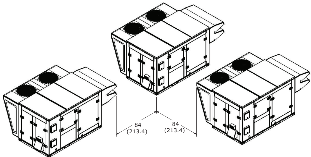
Figure 15. Unit to unit clearance, in. (cm)
