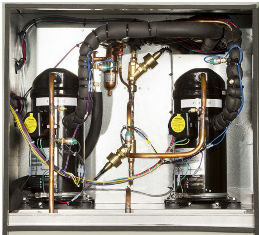
Figure 42. Refrigerant capacity control
