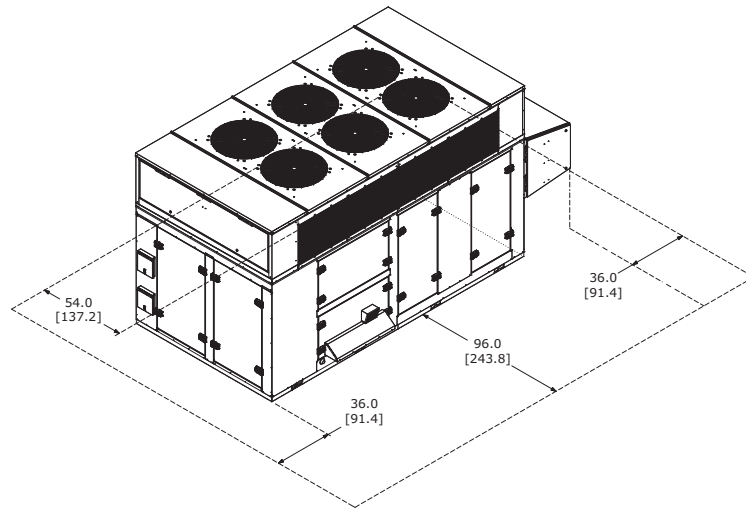
Figure 22. Installation clearances for units with no powered exhaust or ERV, in. (cm)
