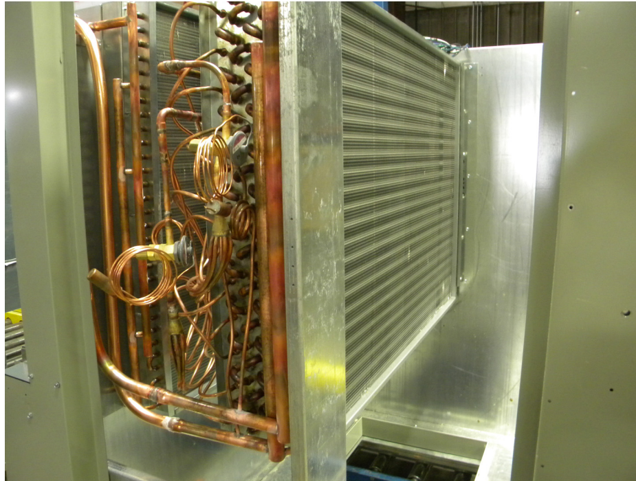
Figure 41. Evaporator and reheat coil
