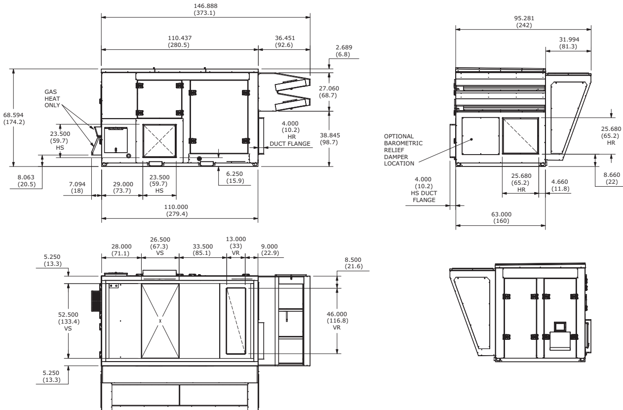
Figure 19. Unit dimensional data for OAD unit with no powered exhaust or ERV, in. (cm)
