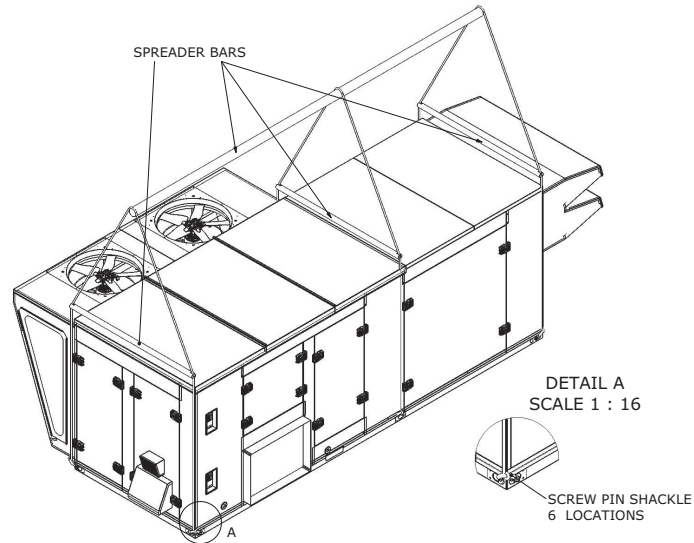
Figure 37. Six-point lift (OAD cabinet with ERV section)
