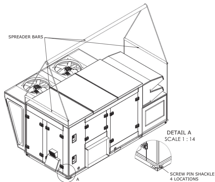
Figure 36. Four-point lift (OAD cabinet with exhaust fan and no ERV)
