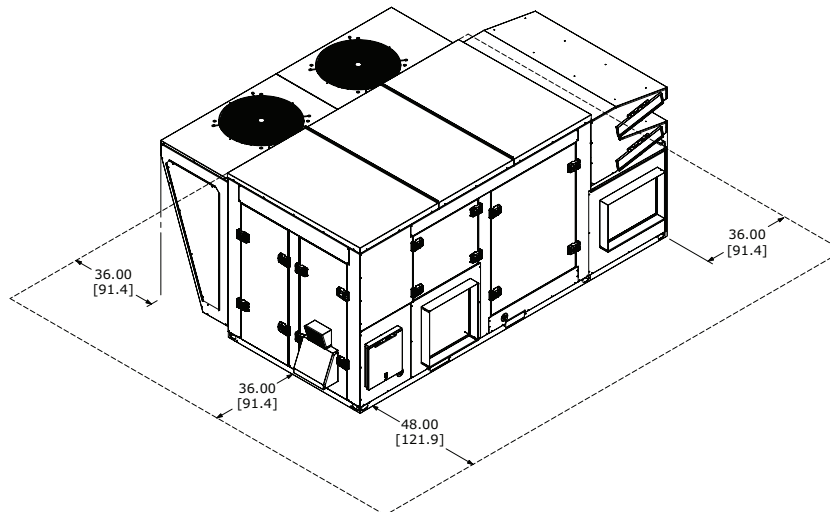
Figure 13. Installation clearances for unit with powered exhaust but no ERV, in. (cm)
