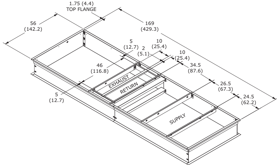
Figure 18. Unit curb data for OAD cabinet with ERV, in. (cm)
