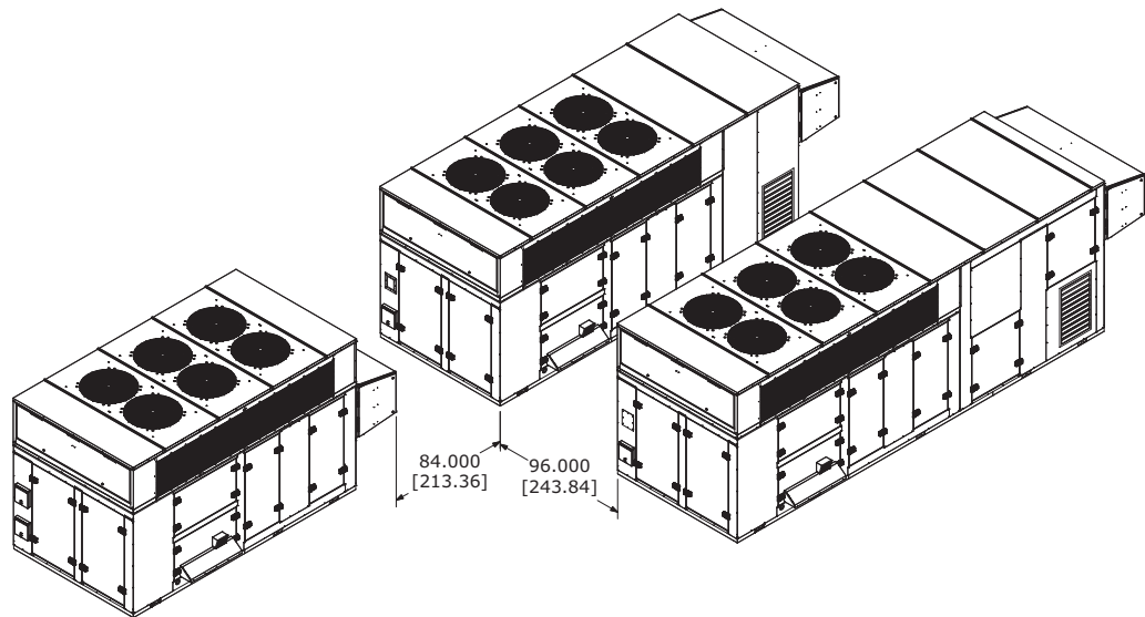
Figure 25. Unit to unit clearance, in. (cm)
