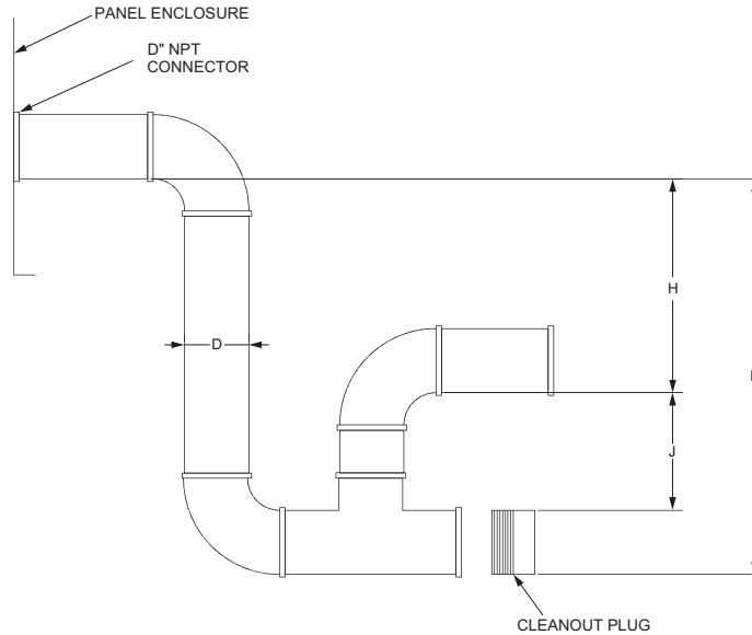
Figure 11. Condensate trap installation
