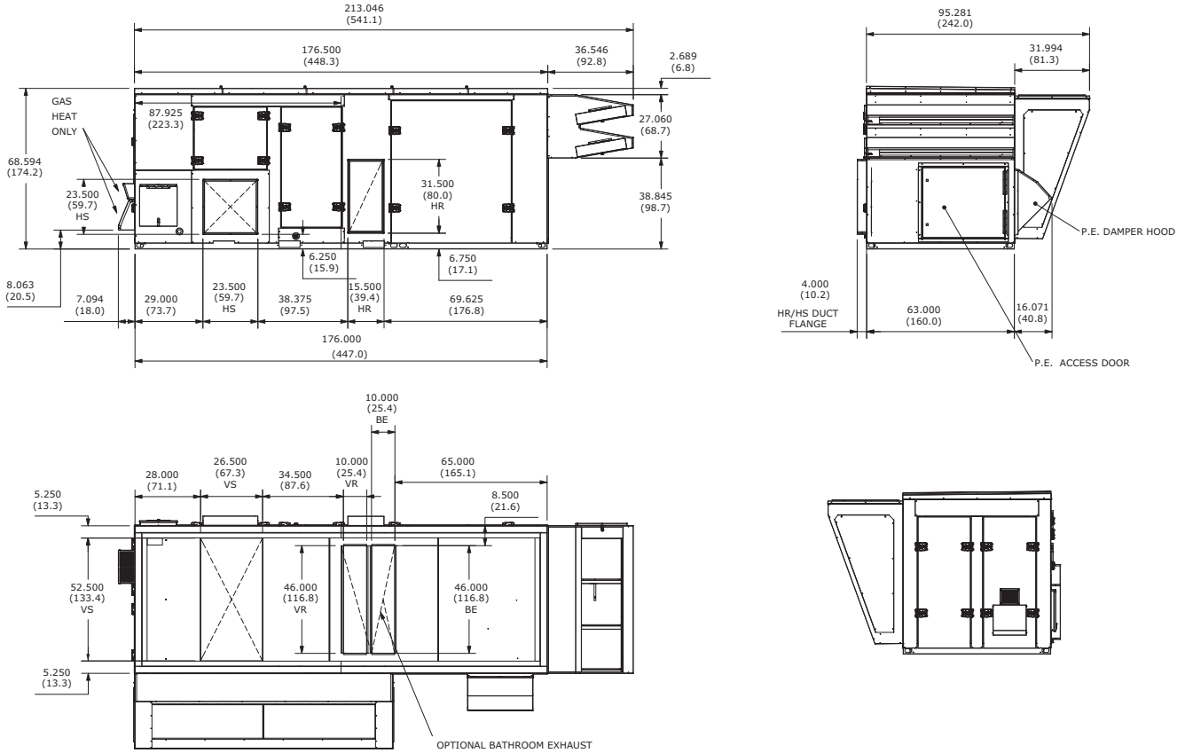
Figure 21. Unit dimensional data for OAD cabinet with ERV, in. (cm)
