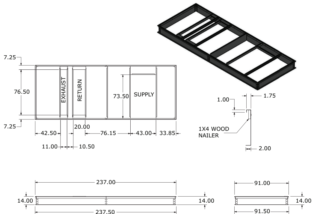
Figure 27. Unit curb data for OAN cabinet with powered exhaust but no ERV, in. (cm)
