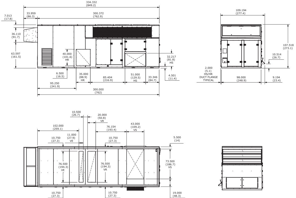
Figure 31. Unit dimensional data for OAN cabinet with ERV, in. (cm)
