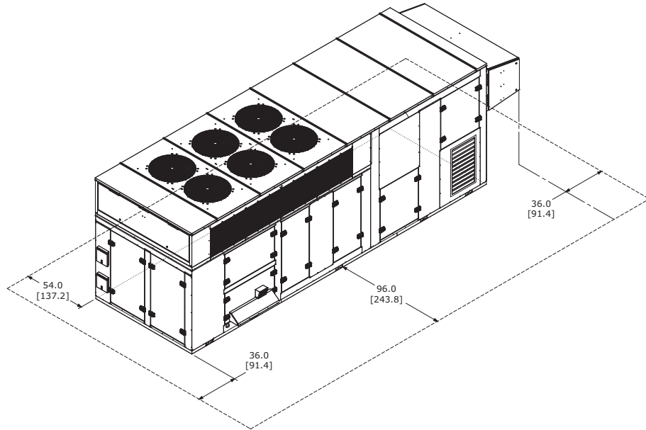
Figure 24. Installation clearances for unit with ERV, in. (cm)
