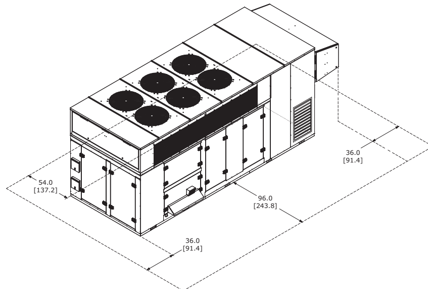
Figure 23. Installation clearances for unit with powered exhaust but no ERV, in. (cm)
