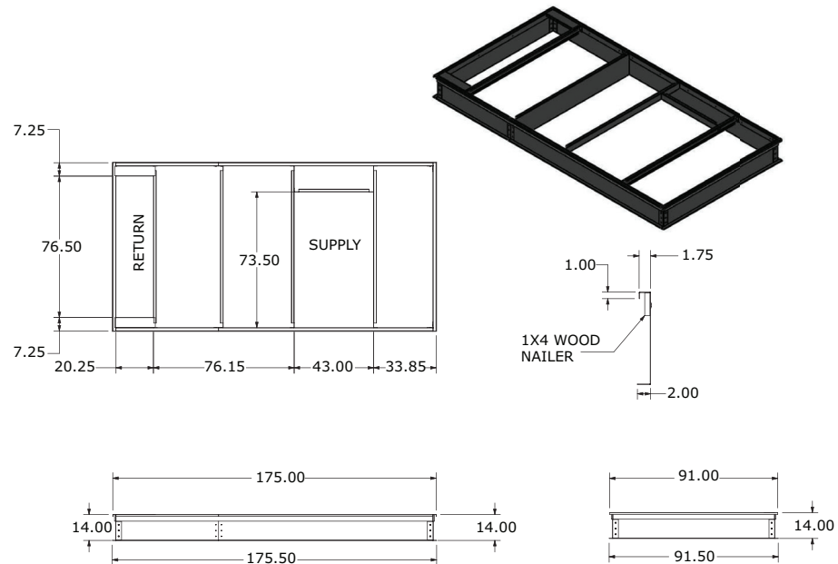
Figure 26. Unit curb data for OAN cabinet with no powered exhaust or ERV, in. (cm)
