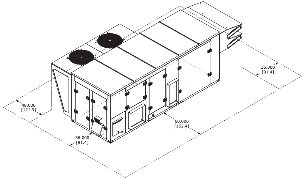
Figure 14. Installation clearances for unit with ERV, in. (cm)
