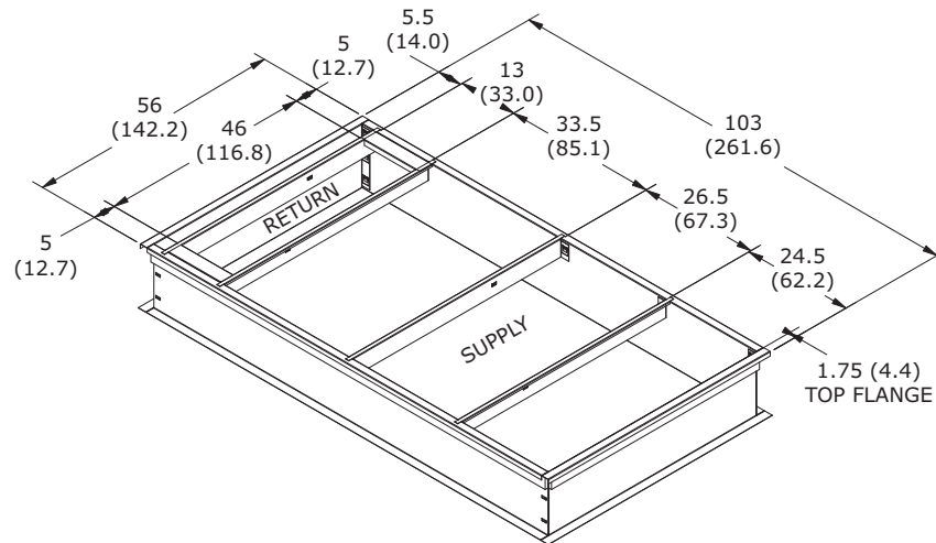
Figure 16. Unit curb data for OAD cabinet with no powered exhaust or ERV, in. (cm)
