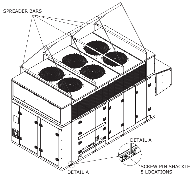
Figure 38. Eight-point lift (OAN cabinet with no exhaust fan or ERV)
