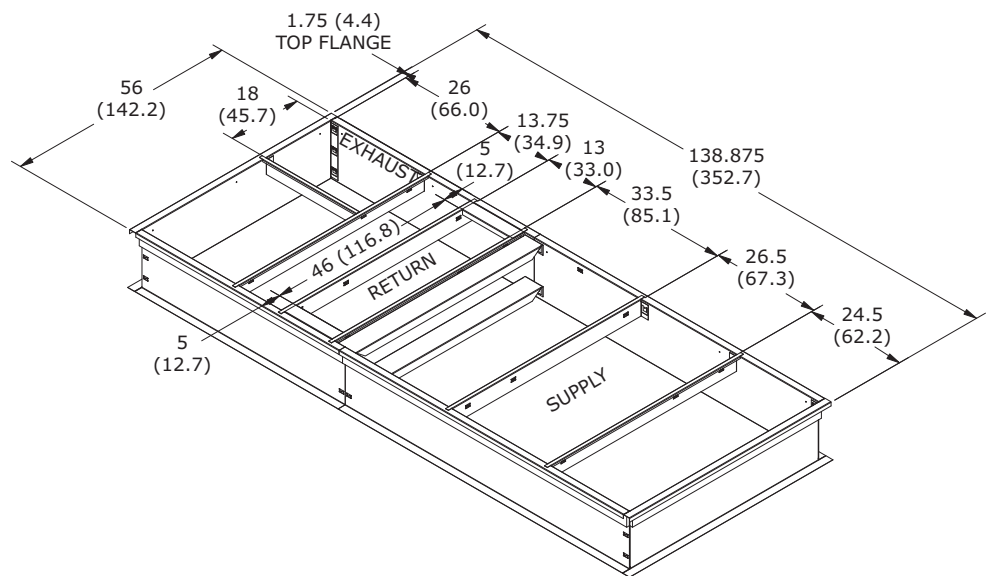
Figure 17. Unit curb data for OAD cabinet with powered exhaust but no ERV, in. (cm)
