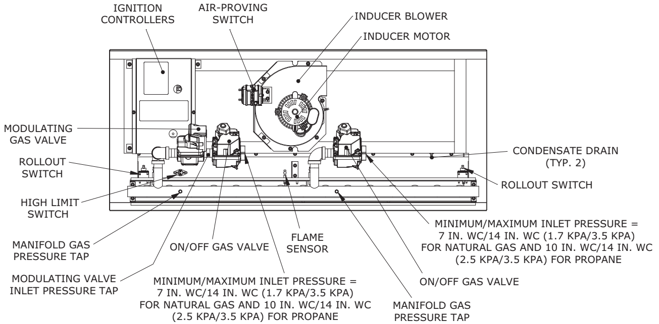
Figure 32. OAD indirect gas-fired furnace heater components
