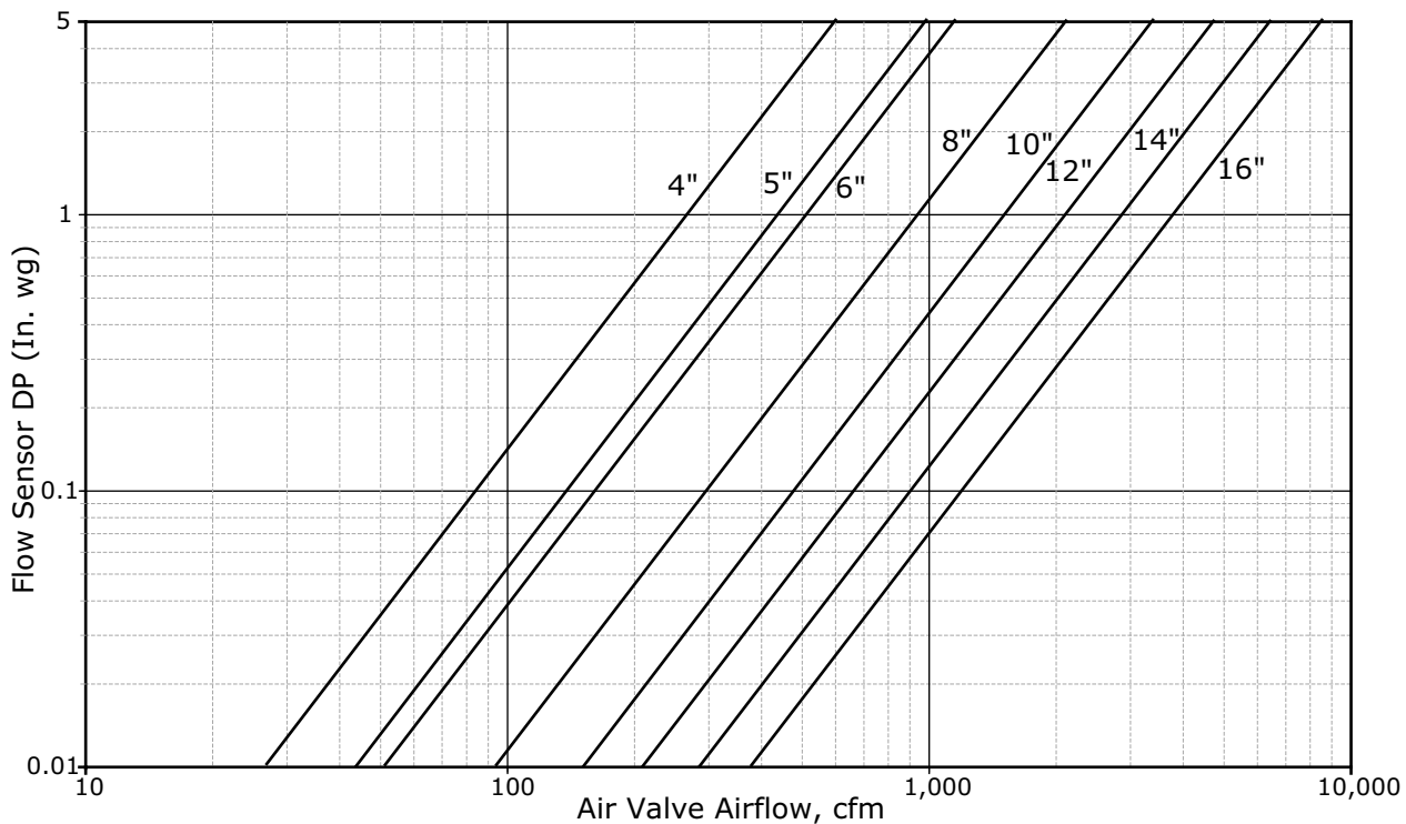
Figure 28. Flow sensor single vs. airflow delivery
