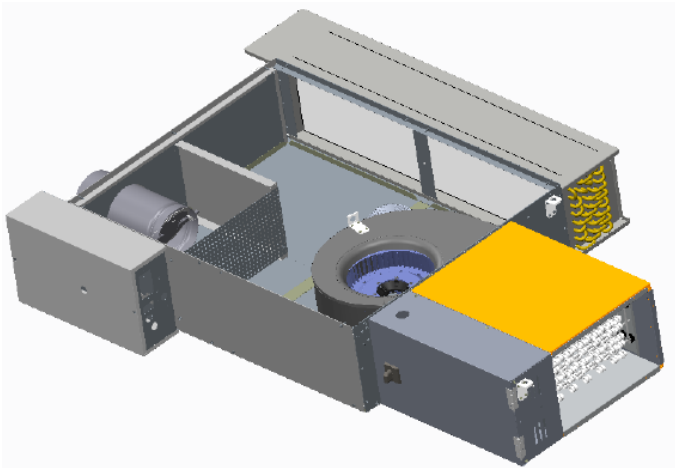
Figure 15. Standard height - sensible cooling w/ electric heat (VDEG)
