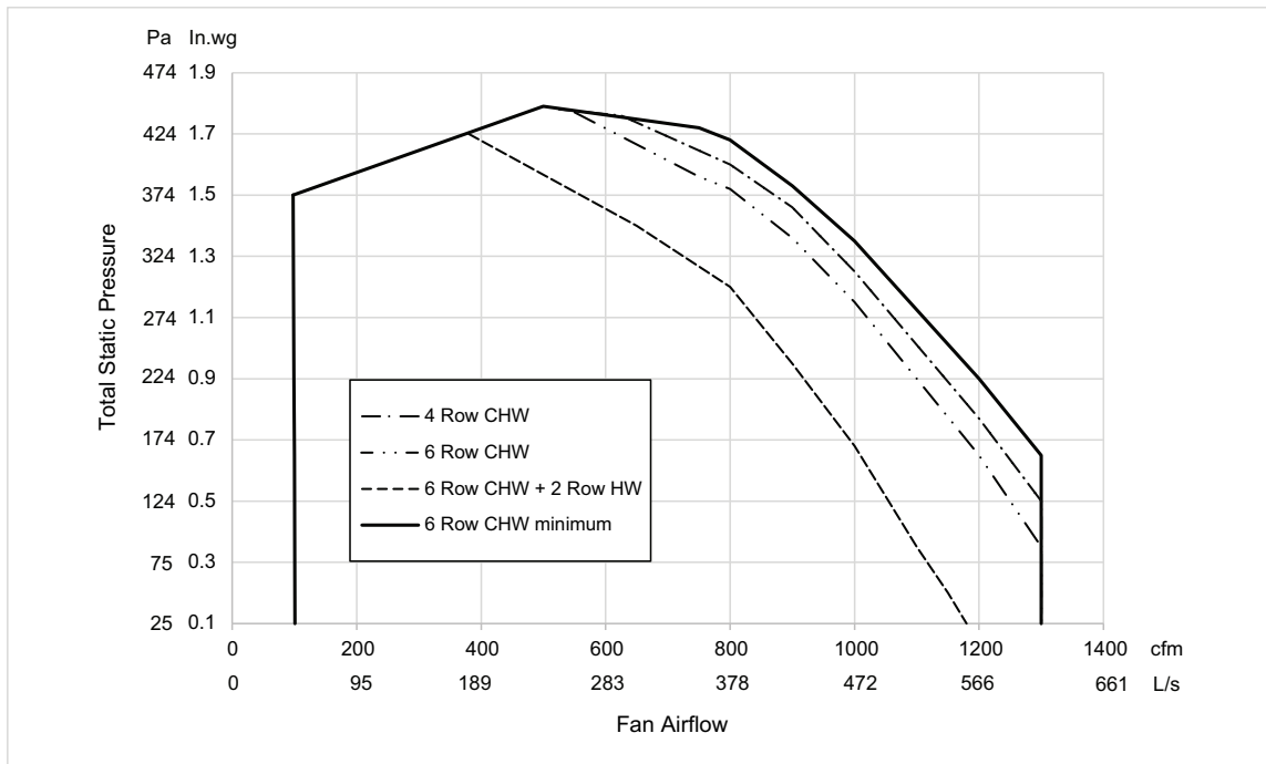
Figure 22. Performance data fan curves, small VDxG – 4 row
