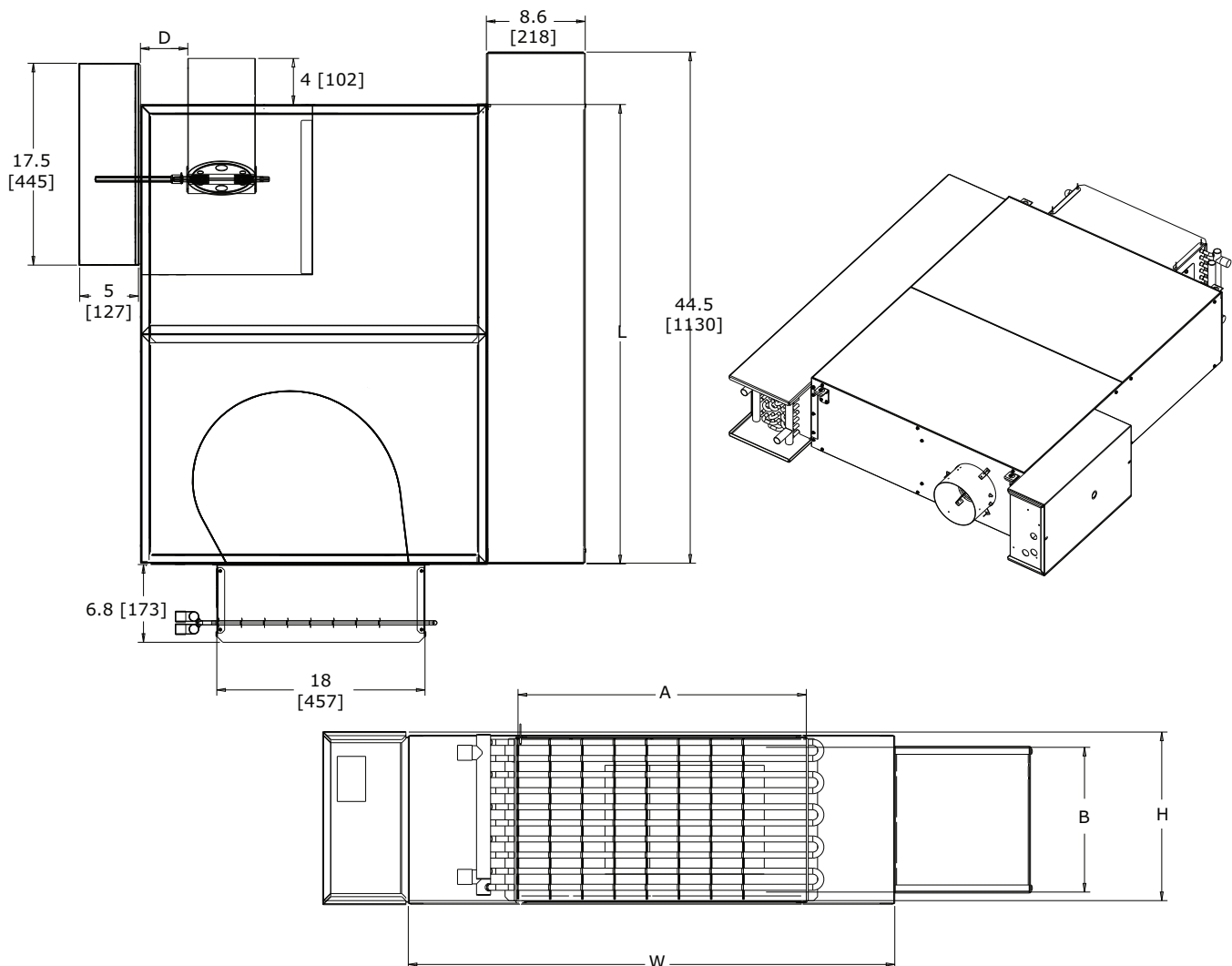
Figure 43. Chilled water sensible cooling terminal unit — hot water (LDWF)
