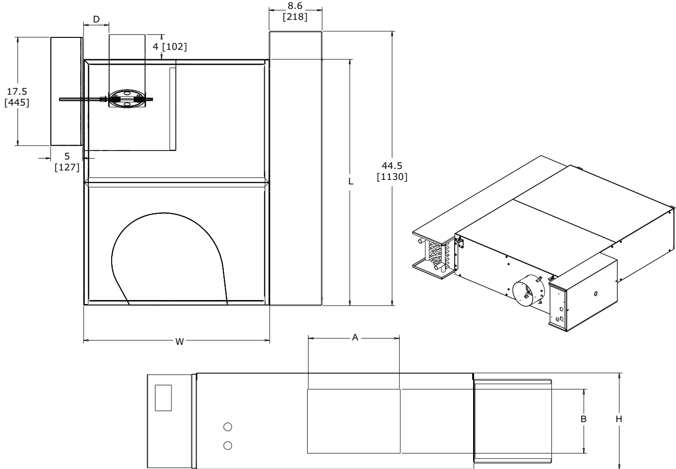
Figure 41. Chilled water sensible cooling terminal unit — cooling only (LDCF)
