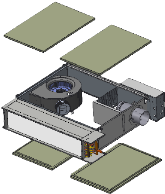
Figure 5. CoolSense chilled water sensible cooling terminal unit
