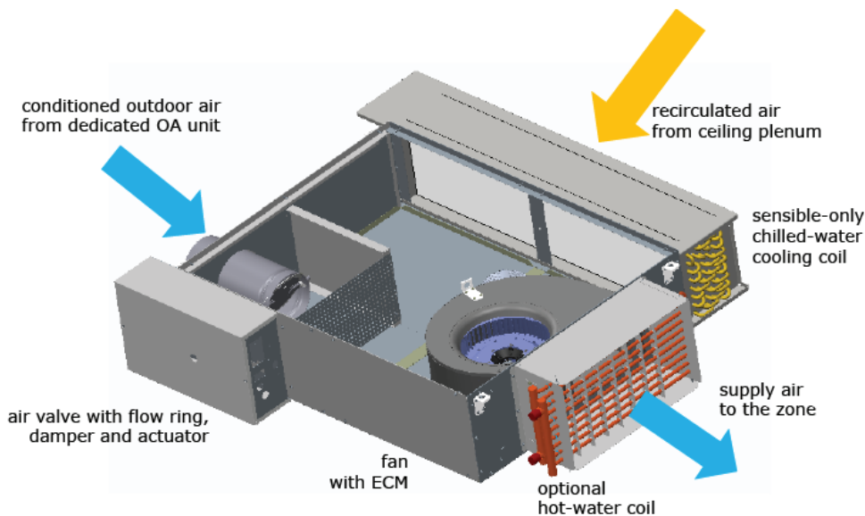
Figure 16. Chilled water sensible cooling terminal unit function
