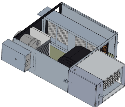
Figure 15. Standard height - sensible cooling w/ electric heat (VDEG)
