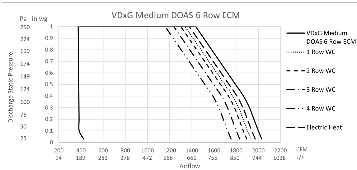
Figure 26. Performance data fan curves, medium VDxG – 6 row
