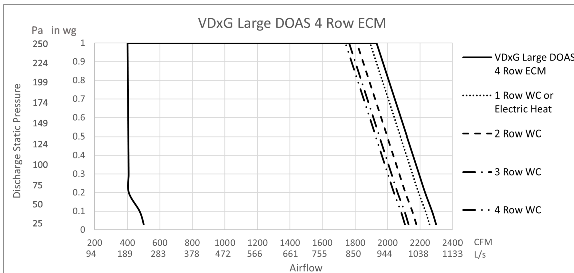
Figure 24. Performance data fan curves, large VDxG – 4 row
