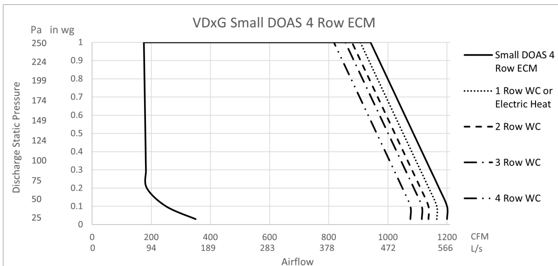
Figure 22. Performance data fan curves, small VDxG – 4 row
