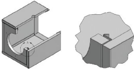
Figure 2. Inter-locking panels
