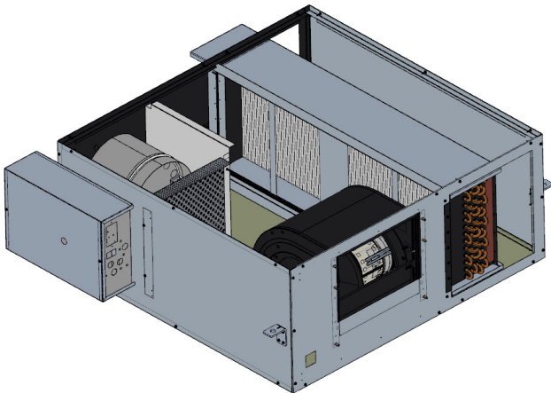
Figure 12. Low height - sensible cooling w/ hot water (LDWF)
