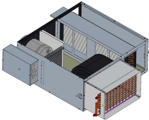
Figure 13. Standard height - sensible cooling w/ hot water (VDWG)
