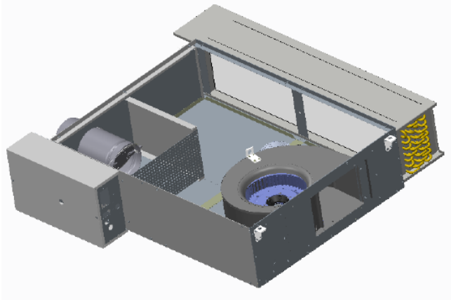
Figure 11. Standard height - sensible cooling only (VDCG)
