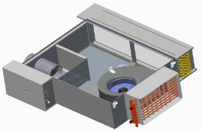
Figure 12. Low height - sensible cooling w/ hot water (LDWF)
