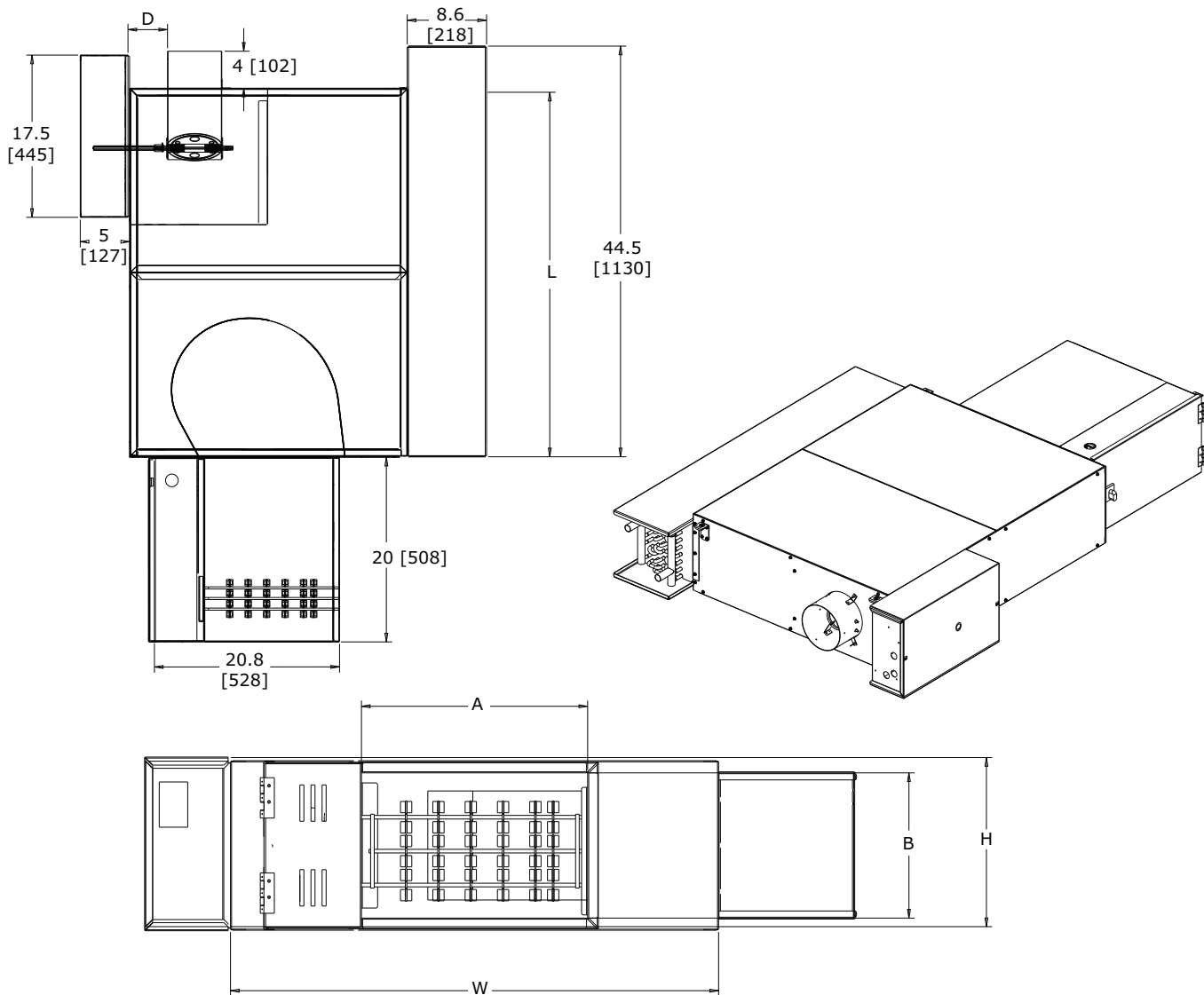
Figure 45. Chilled water sensible cooling terminal unit — electric heat (LDEF)
