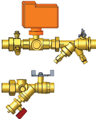
Figure 35. Belimo valve piping package
