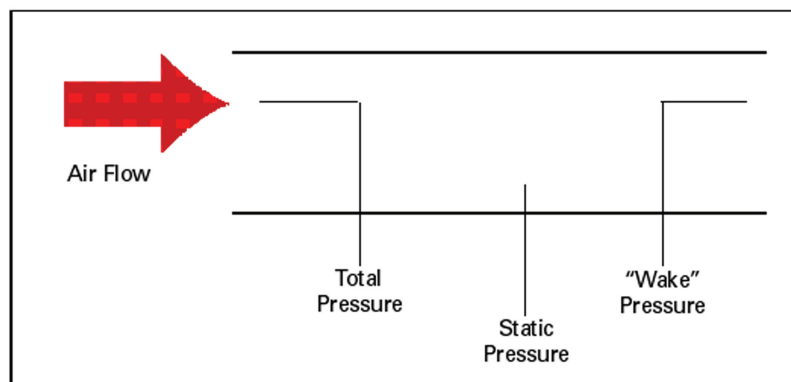
Figure 19. Air pressure measurement orientations
