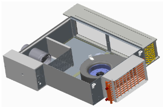
Figure 3. Low height - sensible cooling w/ hot water (LDWF)
