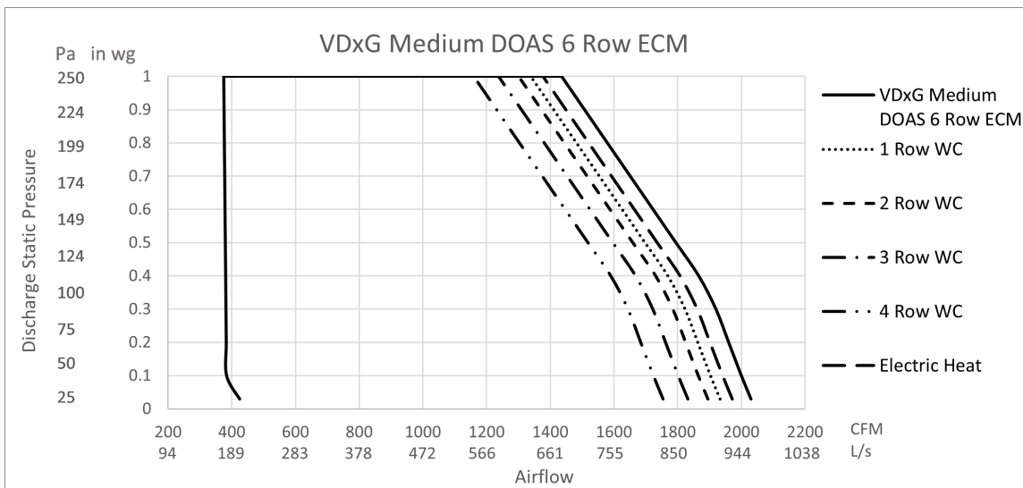
Figure 15. Performance data fan curves, medium VDxG – 6 row
