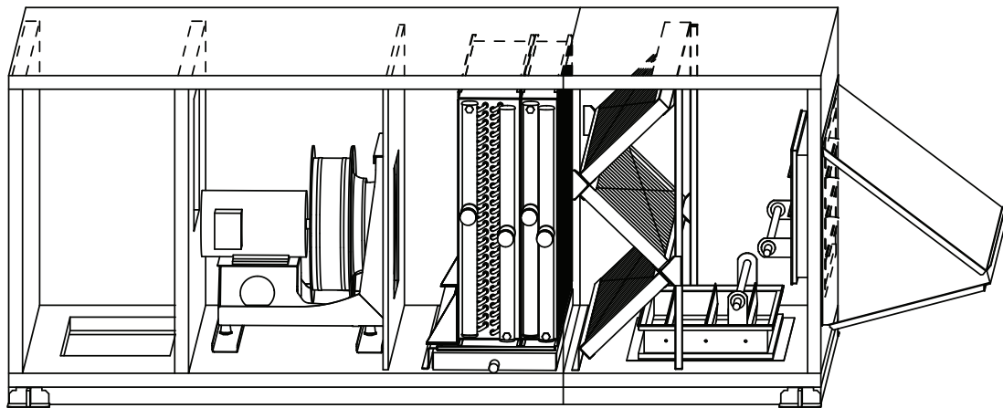
Figure 11. Outdoor unit with DDP fan configuration
