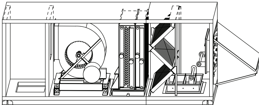
Figure 12. Outdoor unit with FC fan configuration
