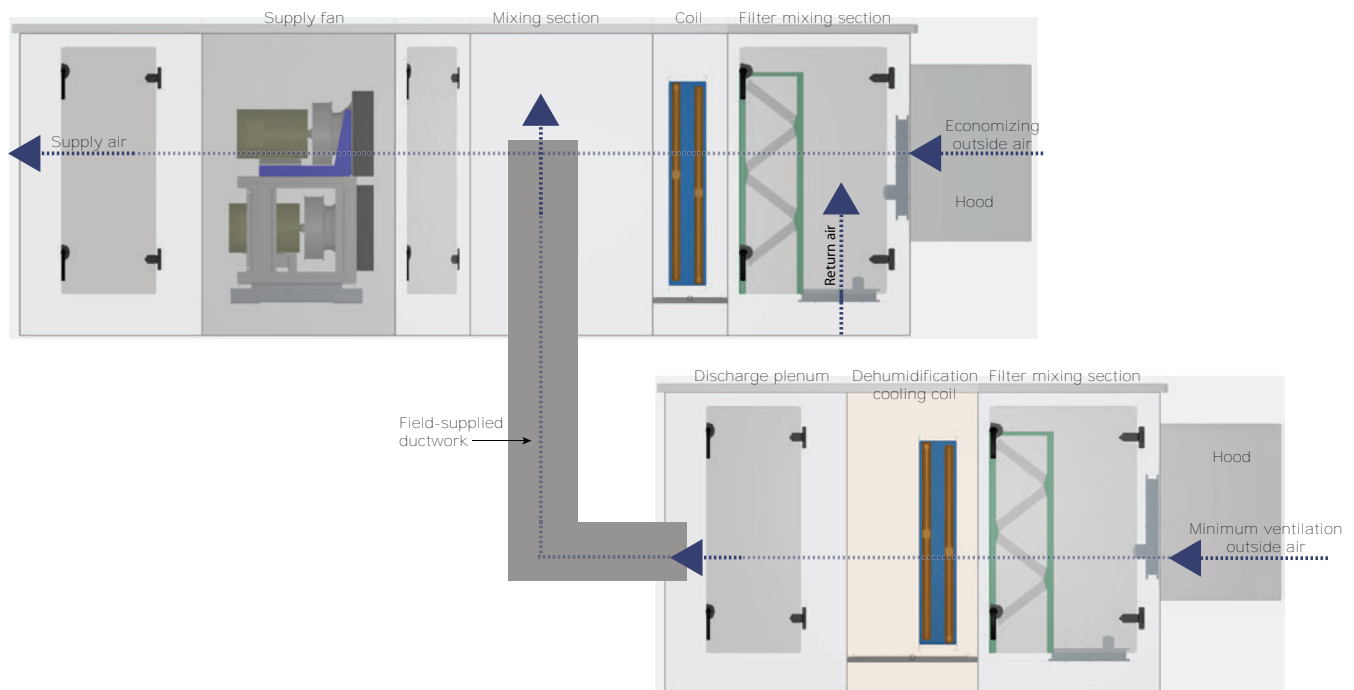
Figure 25. Dehumidifying with two outdoor SDUs (inlet hood shape varies)
