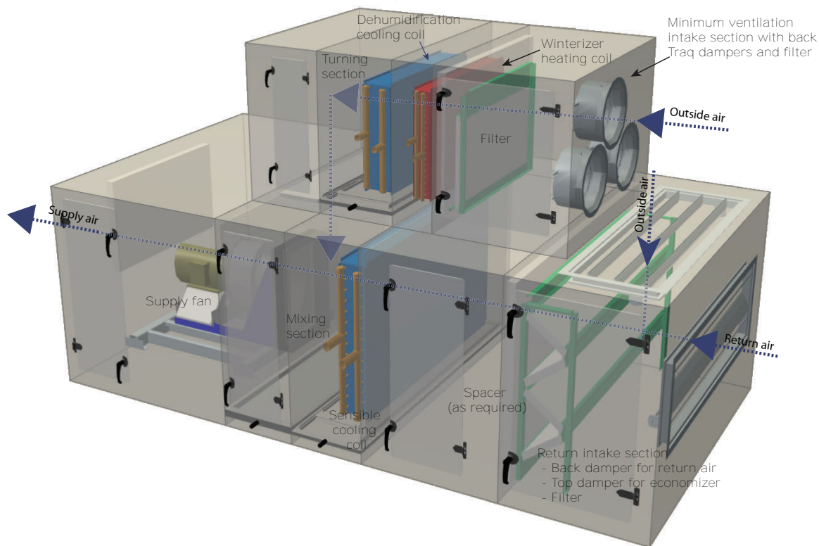
Figure 23. Horizontal indoor SDU
