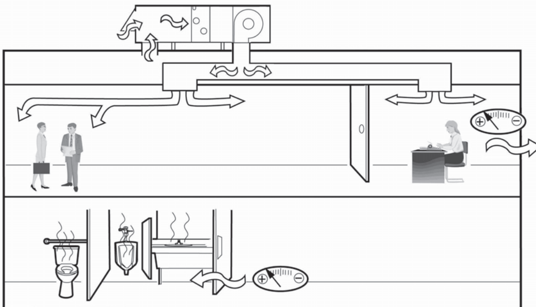
Figure 5. Maintain proper building pressurization
