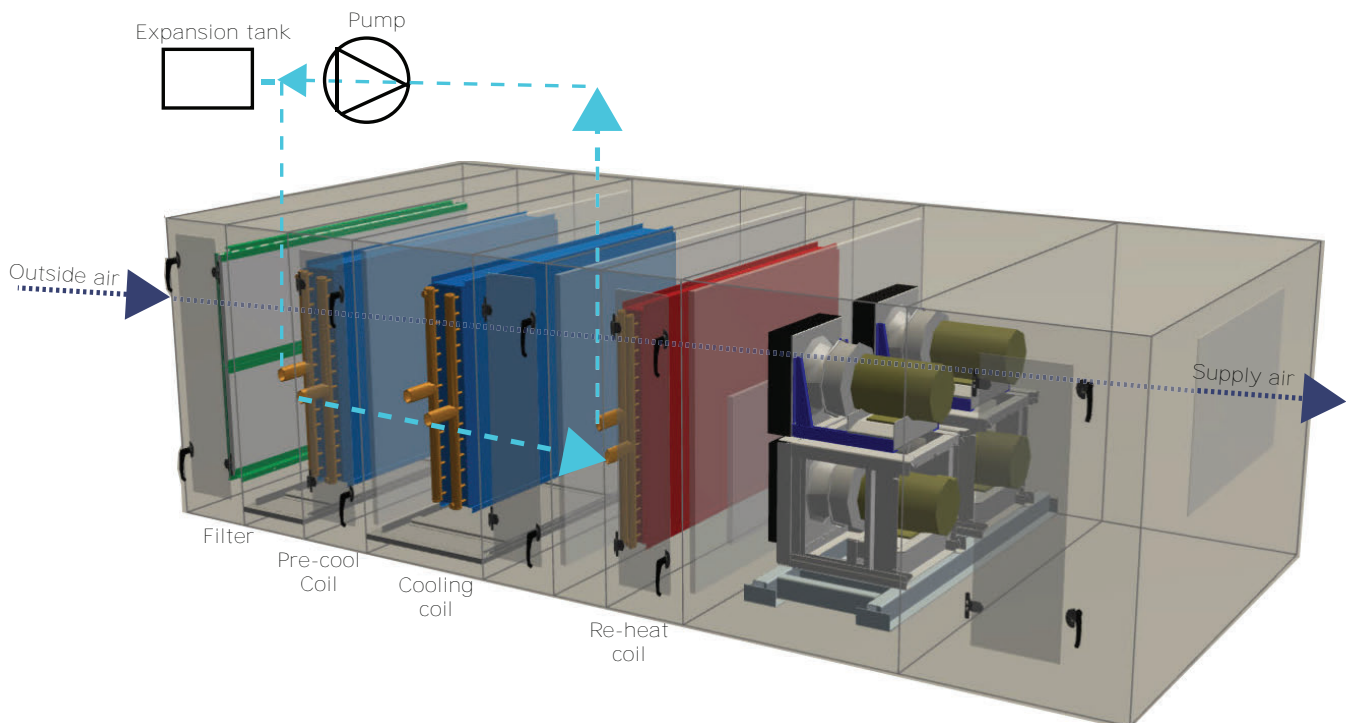
Figure 22. Series dehumidification with coil run-around loops
