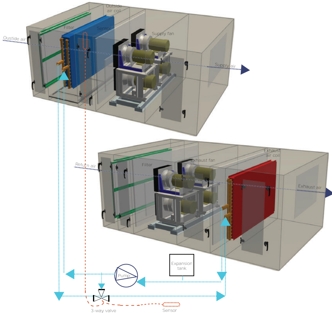
Figure 28. Energy recovery with a runaround coil loop
