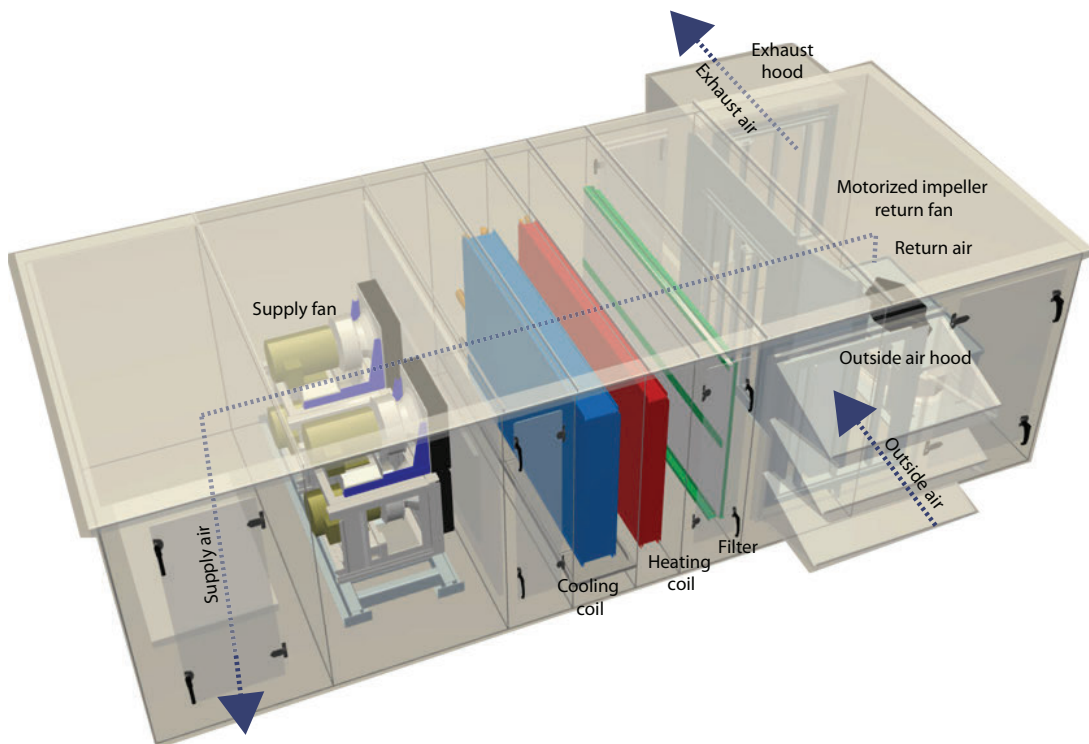
Figure 18. Return fan and economizer arrangement for outdoor units
