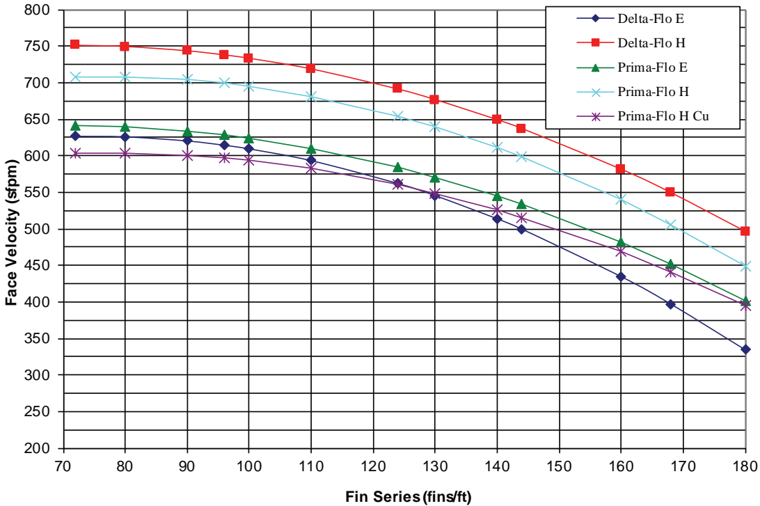
Figure 59. Face velocity limits for moisture carryover with uncoated coils in unit sizes 50-57
