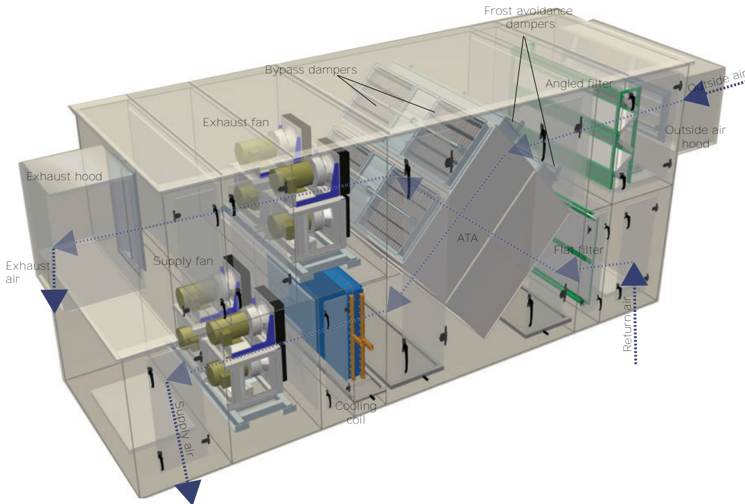
Figure 29. Energy recovery with air-to-air (ATA) plate frame heat exchanger (Outside air hood shape varies)
