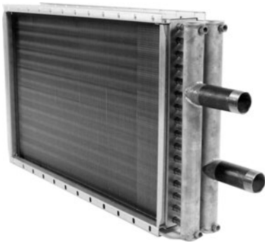
Figure 35. Coil with copper header
