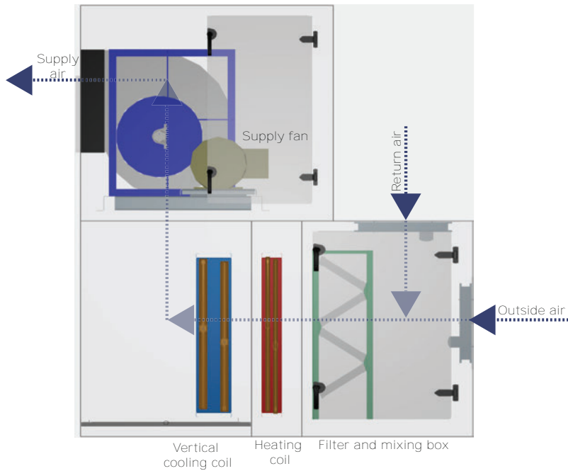
Figure 16. Vertical draw-thru arrangement
