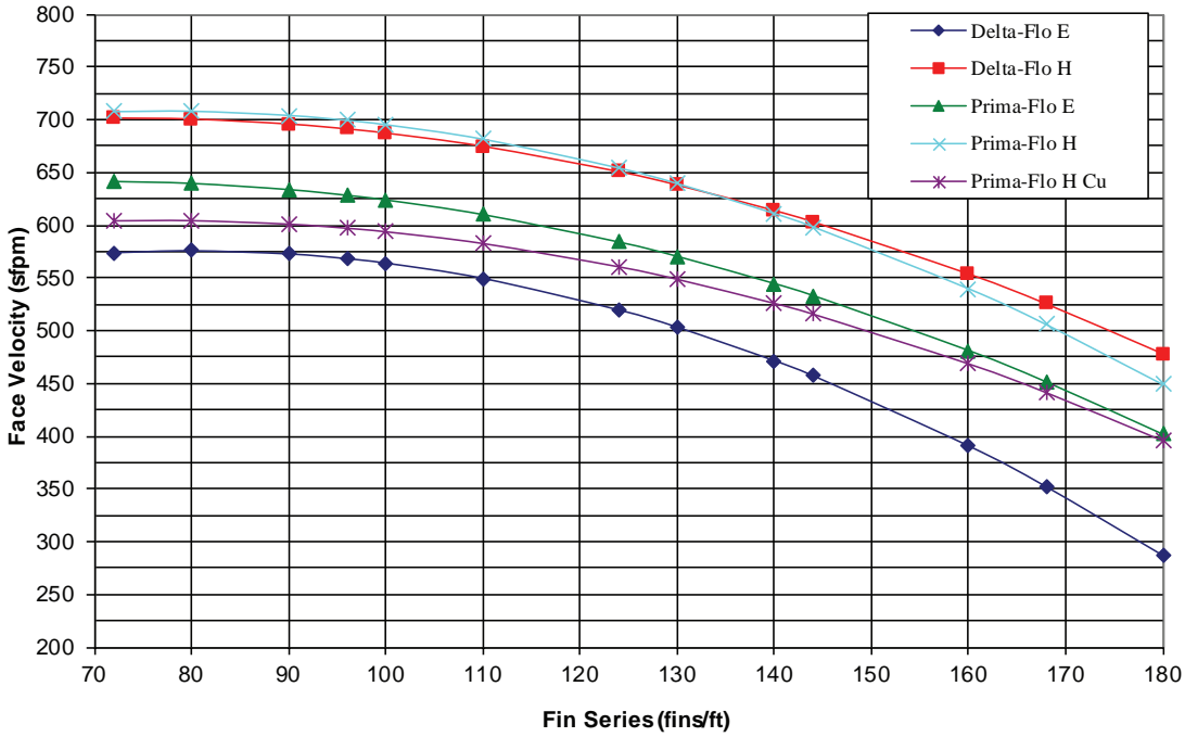
Figure 59. Face velocity limits for moisture carryover with uncoated coils in unit sizes 50-57
