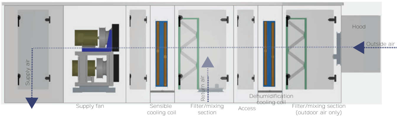
Figure 25. Dehumidifying with two outdoor SDUs (inlet hood shape varies)
