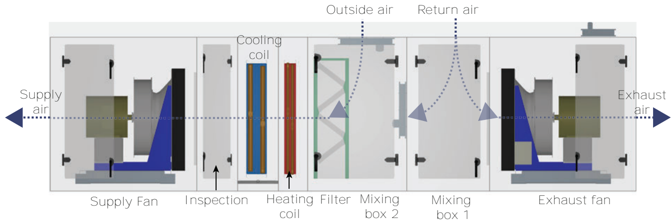
Figure 19. Exhaust fan and economizer arrangement
