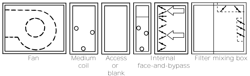
Figure 40. Damper arrangement
