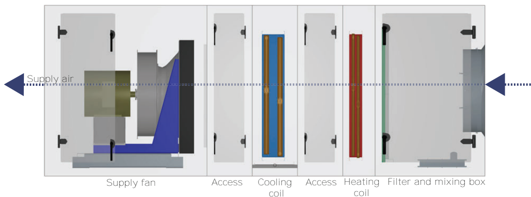
Figure 15. Horizontal draw-thru arrangement
