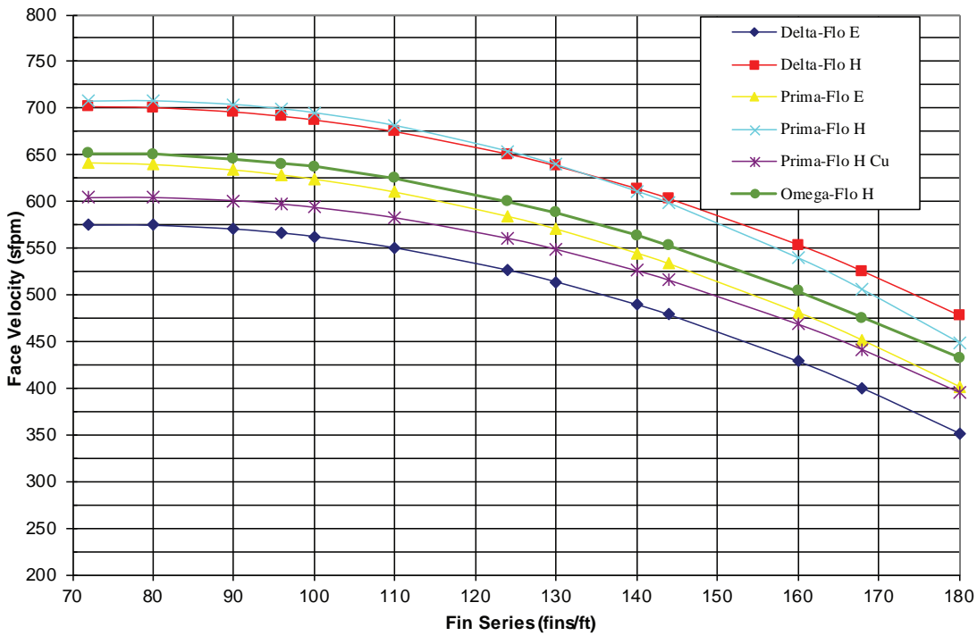
Figure 57. Face-velocity limits for moisture carryover with uncoated coils in unit sizes 21-30
