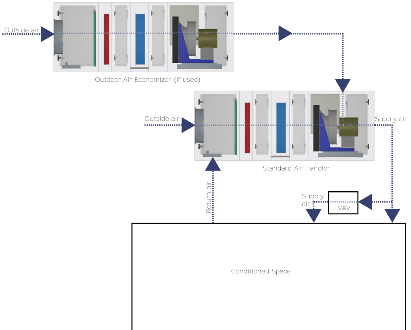
Figure 14. Dual-path design
