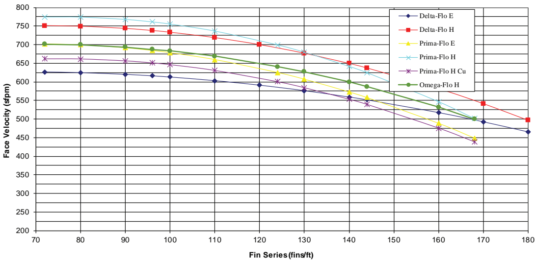
Figure 55. Face-velocity limits for moisture carryover with uncoated coils in unit size 12
