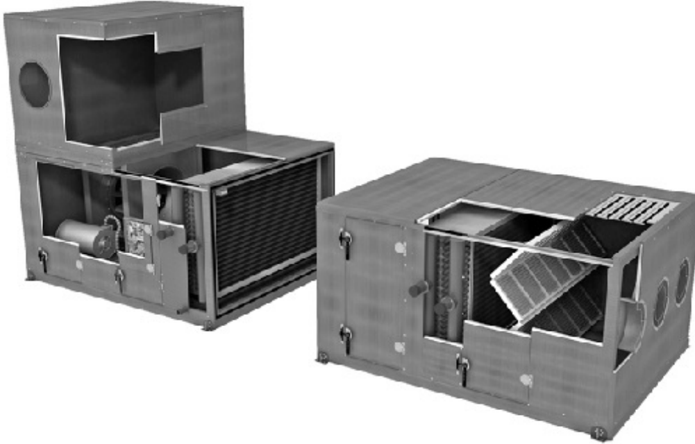
Figure 1. Trane performance climate changer air handler
