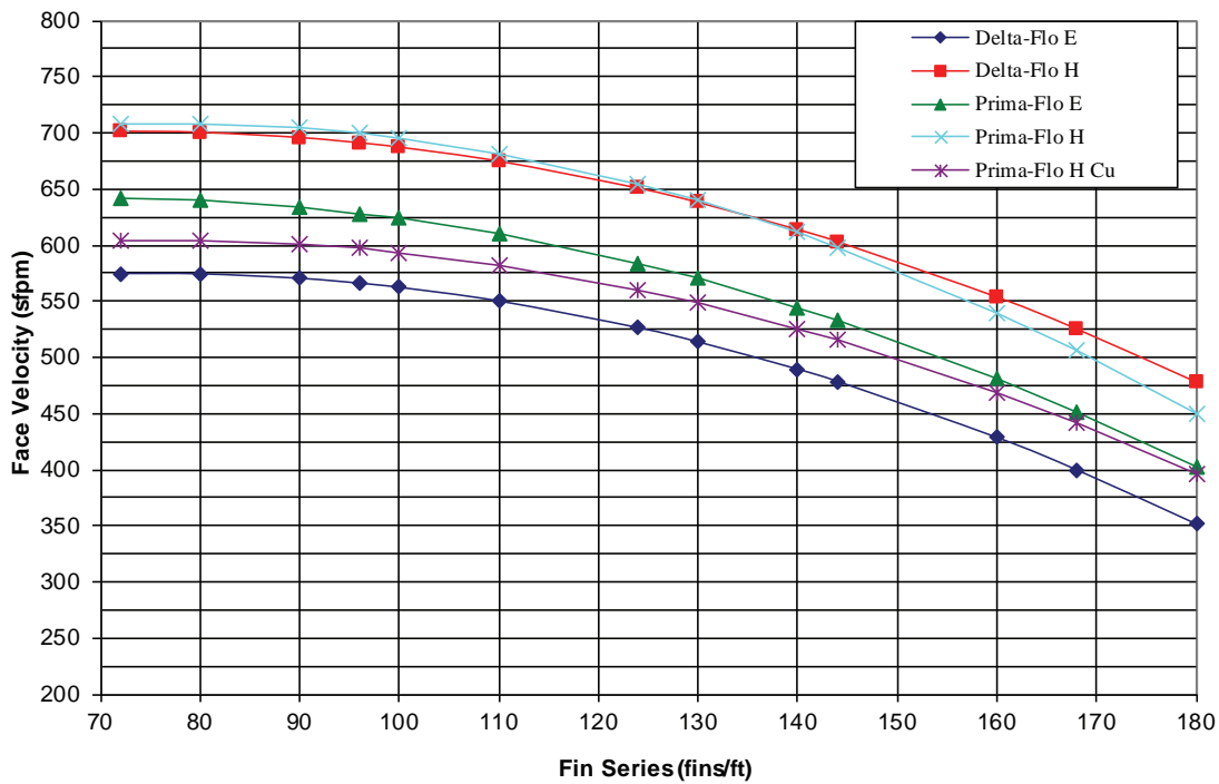
Figure 61. Face velocity limits for moisture carryover with uncoated coils in unit size 80-120
