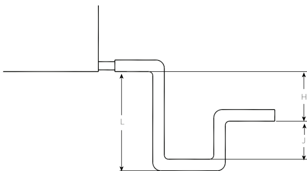
Figure 11. Drain pan trapping for positive and negative pressure applications
