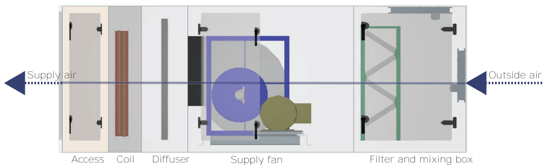
Figure 17. Single-zone blow-thru arrangement
