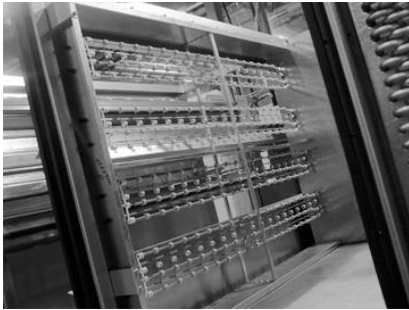
Figure 38. Typical blow through heater
