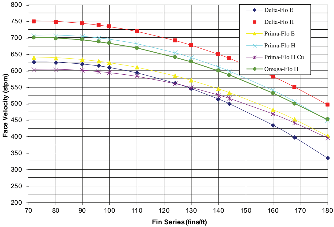
Figure 57. Face-velocity limits for moisture carryover with uncoated coils in unit sizes 21-30
