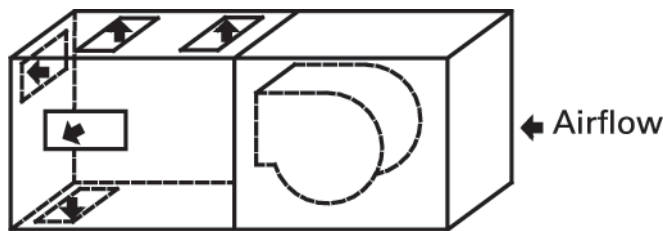
Figure 47. Horizontal plenum
