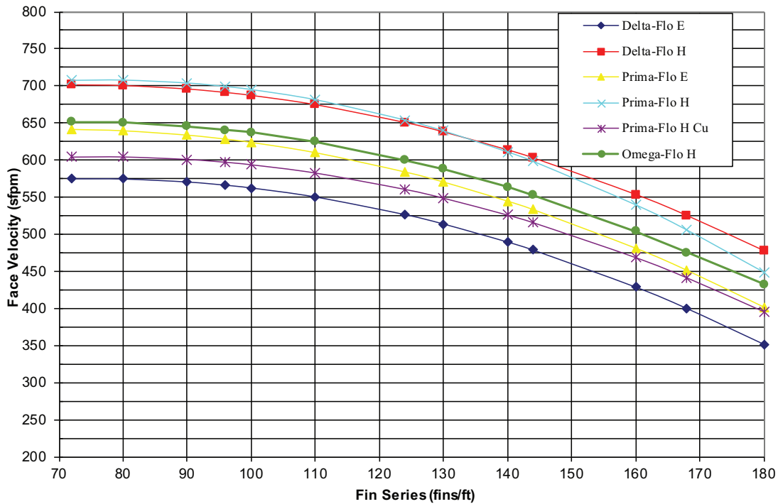
Figure 42. Face-velocity limits for moisture carryover with uncoated coils in unit sizes 21-30
