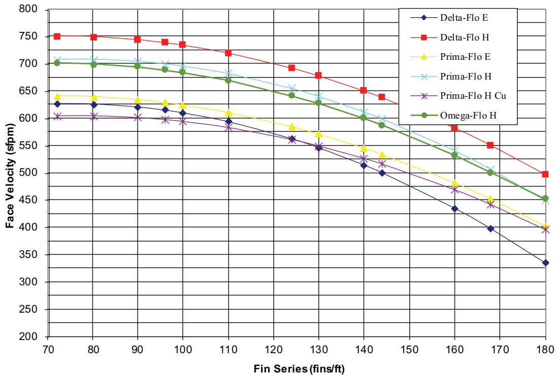
Figure 42. Face-velocity limits for moisture carryover with uncoated coils in unit sizes 21-30
