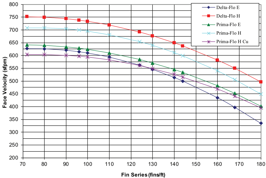
Figure 44. Face velocity limits for moisture carryover with uncoated coils in unit sizes 50-57
