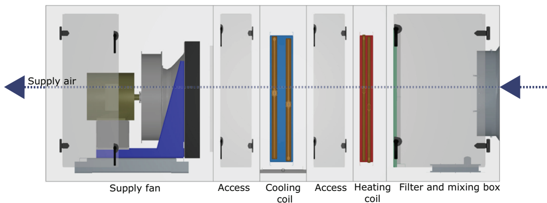
Figure 14. Horizontal draw-thru arrangement
