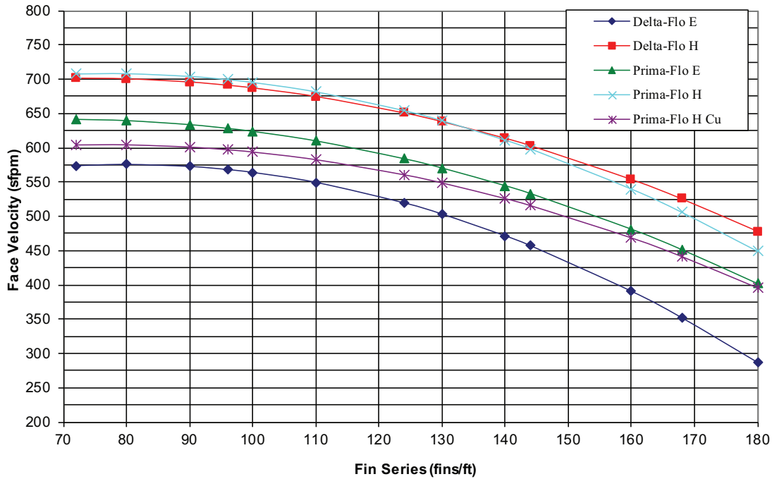
Figure 44. Face velocity limits for moisture carryover with uncoated coils in unit sizes 50-57
