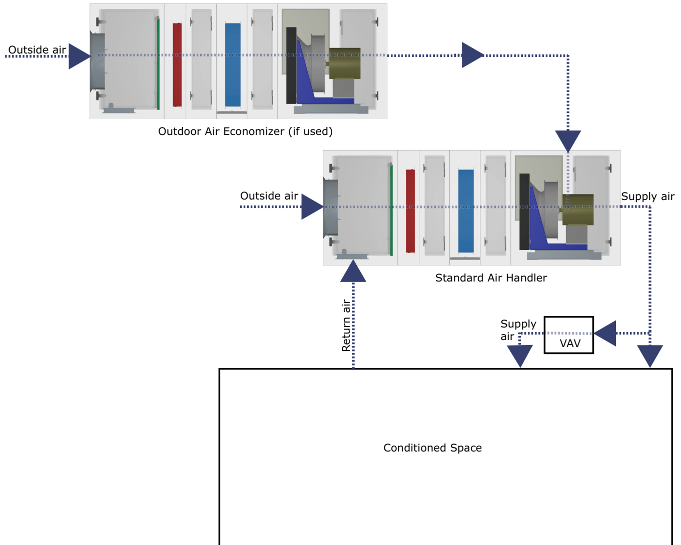
Figure 13. Dual-path design
