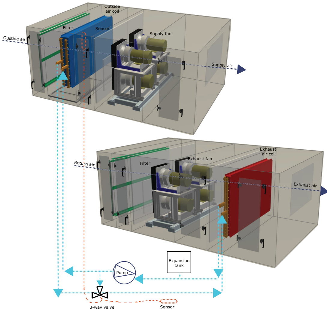
Figure 27. Energy recovery with a runaround coil loop
