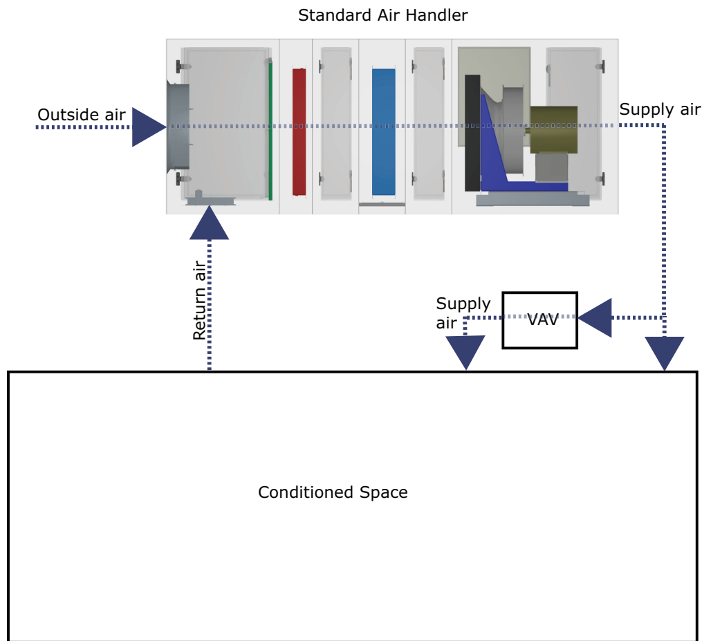
Figure 12. Single-path design
