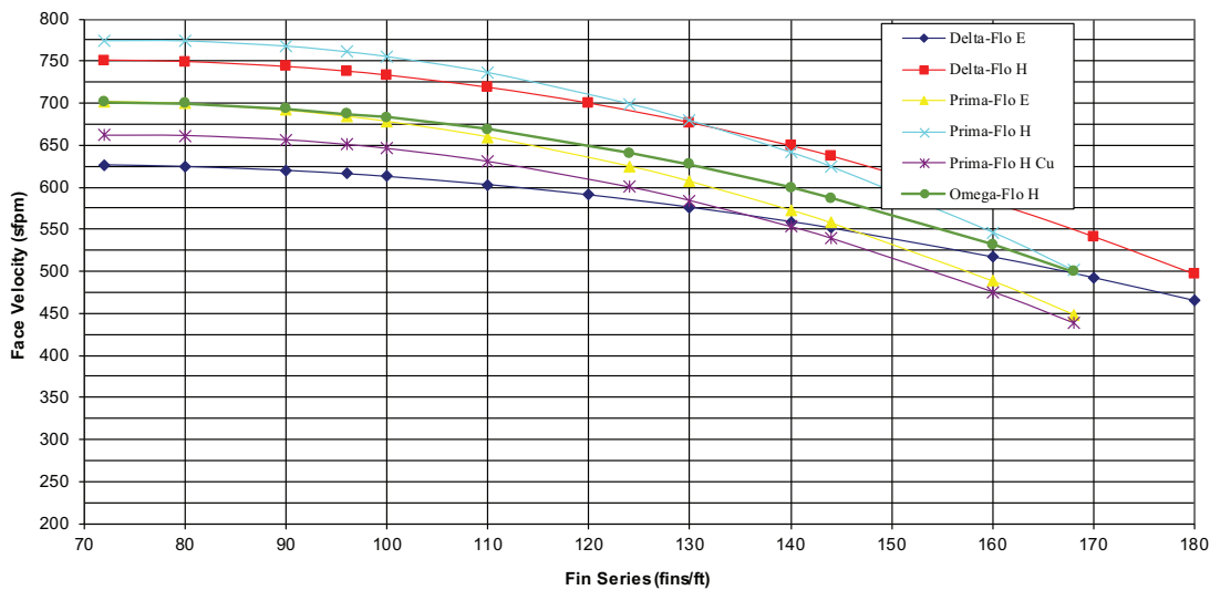
Figure 40. Face-velocity limits for moisture carryover with uncoated coils in unit size 12
