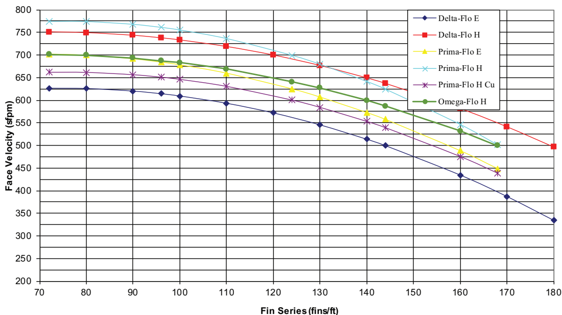
Figure 40. Face-velocity limits for moisture carryover with uncoated coils in unit size 12
