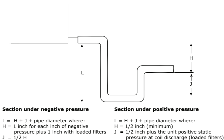
Figure 10. Drain pan trapping for positive and negative pressure applications
