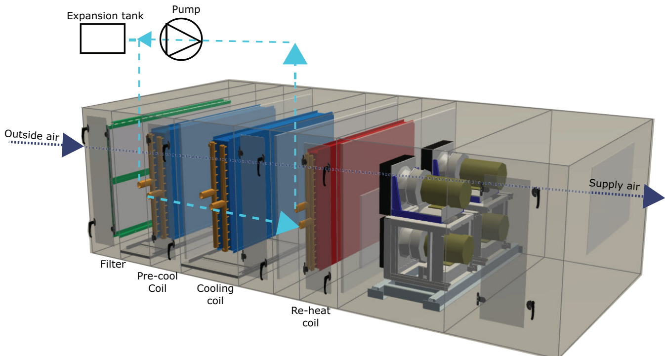
Figure 21. Series dehumidification with coil run-around loops
