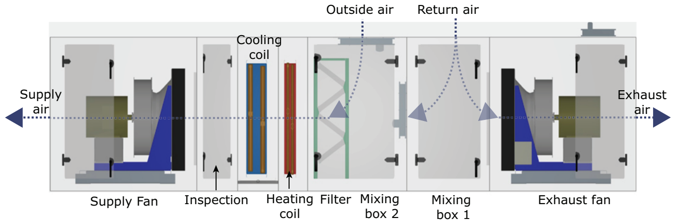
Figure 18. Exhaust fan and economizer arrangement
