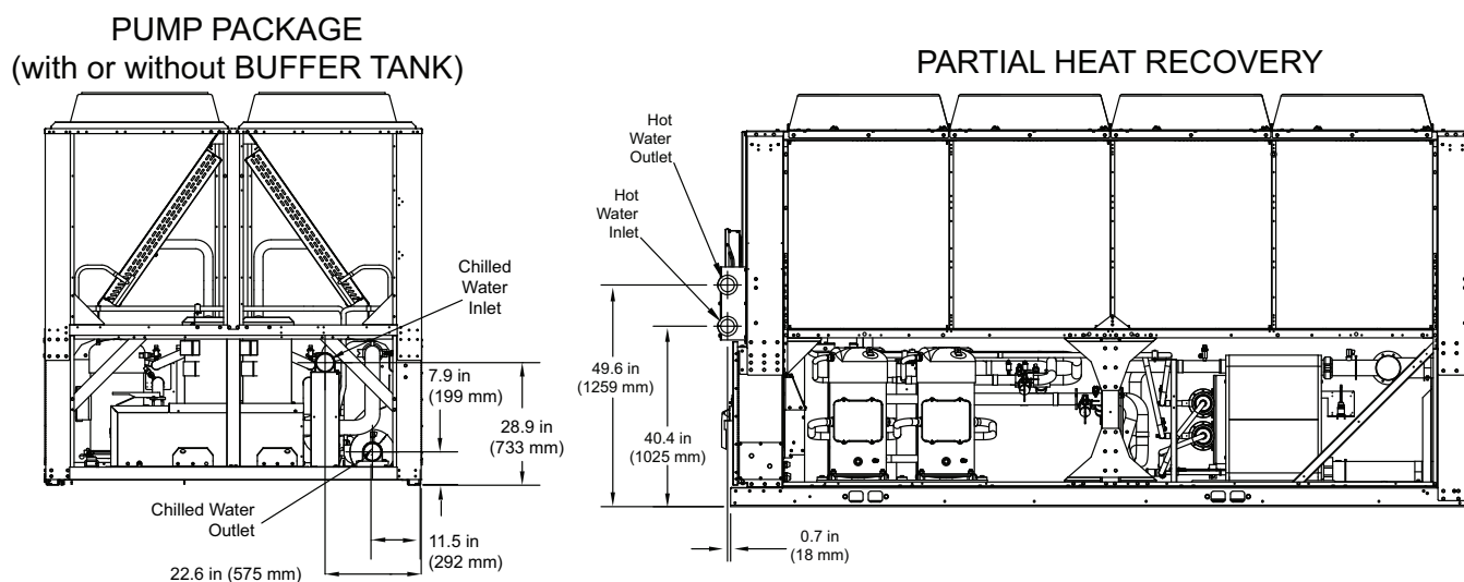
Figure 14. Water connection dimensions – 80 to 130 ton units with options
