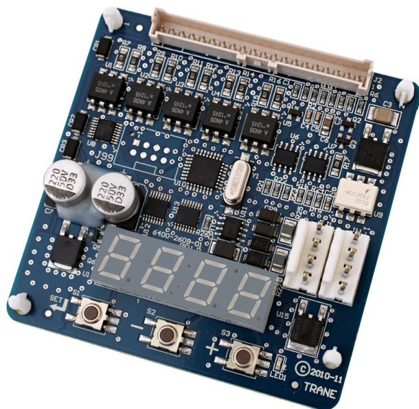
Figure 9. VelociTach motor control board
