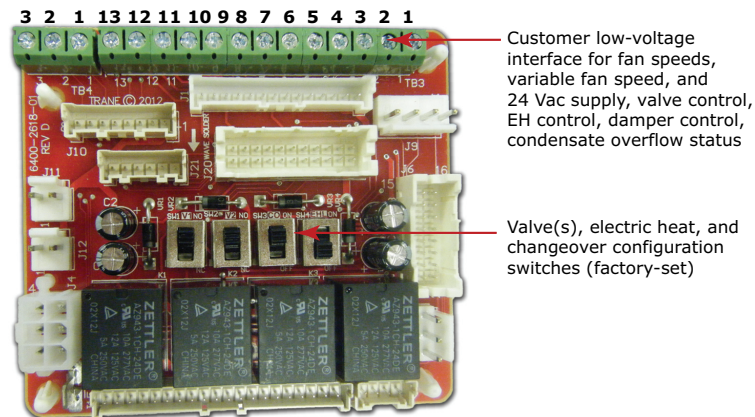
Figure 12. CSTI adapter board and field connections
