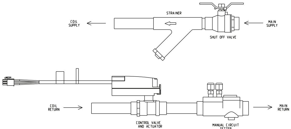
Figure 33. 2 way valve 2.3, 3.3, and 4.6 CV
