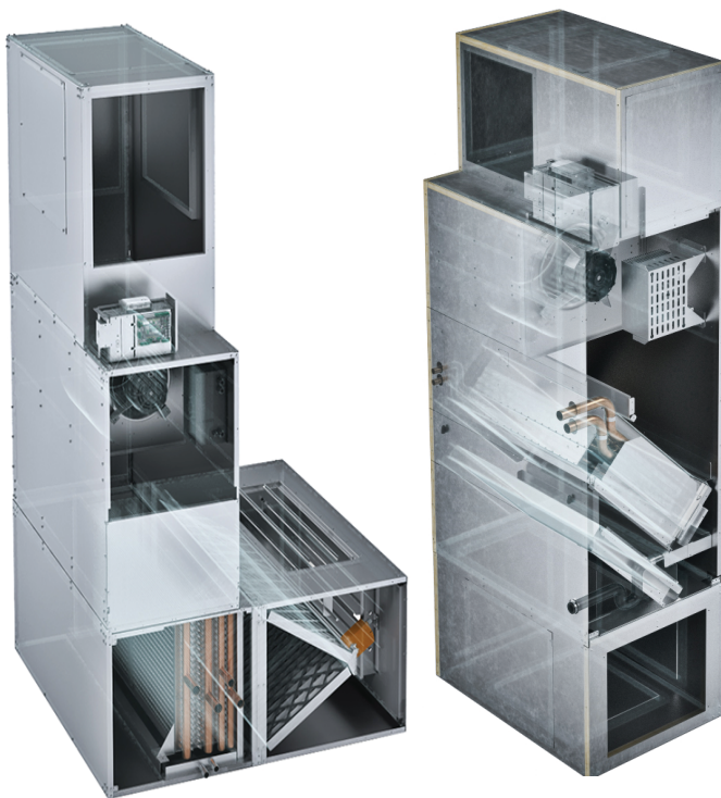
Figure 8. BCVE vertical arrangement
