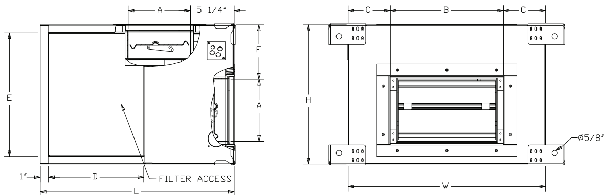
Figure 23. Mixing box dimension
