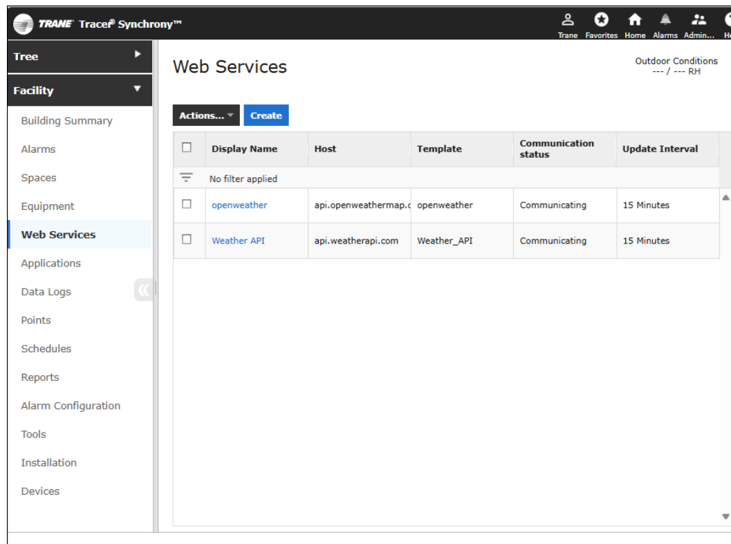
Figure 5. Web services
