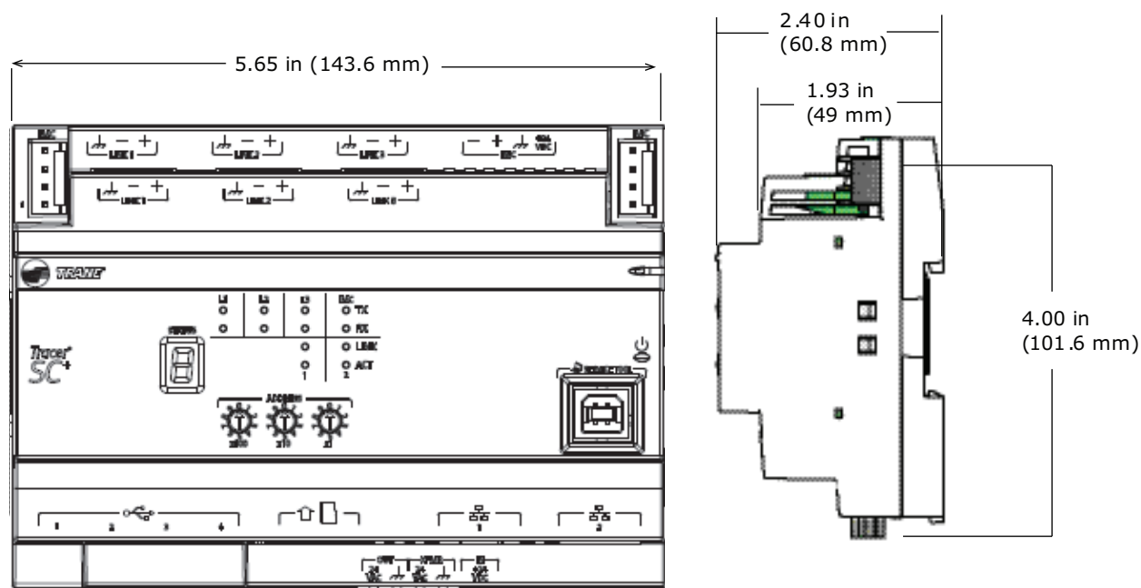
Figure 19. Tracer SC+ system controller dimensions
