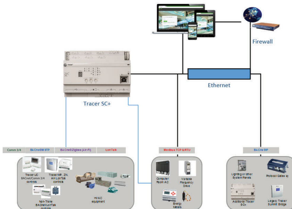
Figure 2. Example of a single SC+ facility configuration
