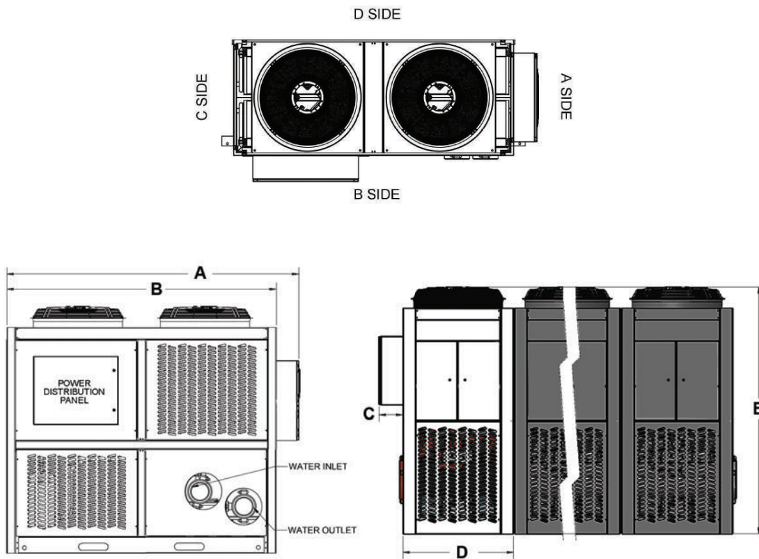
Figure 1. AMC air-cooled modulares - 15 to 40 tons
