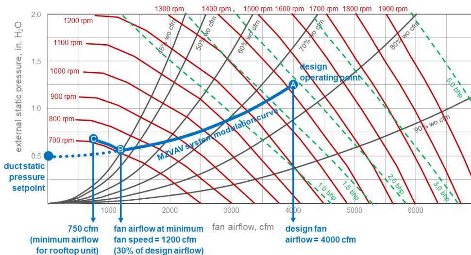
Supply fan turndown in a changeover hybrid, changeover VAV, or multiple-zone VAV system (fan only or cooling mode)
