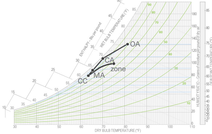
DOAS: 70°F supply air: Part load 0.611 SHR
