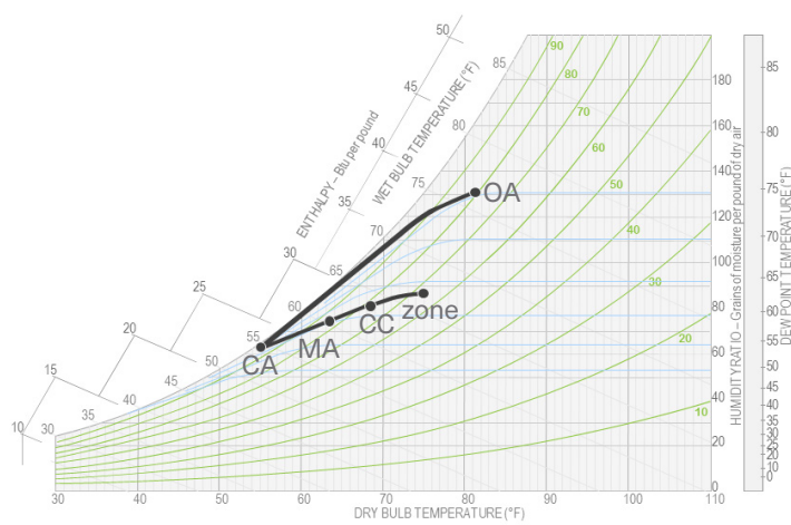
DOAS: 55°F supply air: Part load 0.611 SHR
