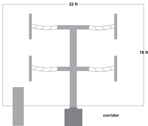
Acoustic model of an example classroom using the CoolSense system (plan)
