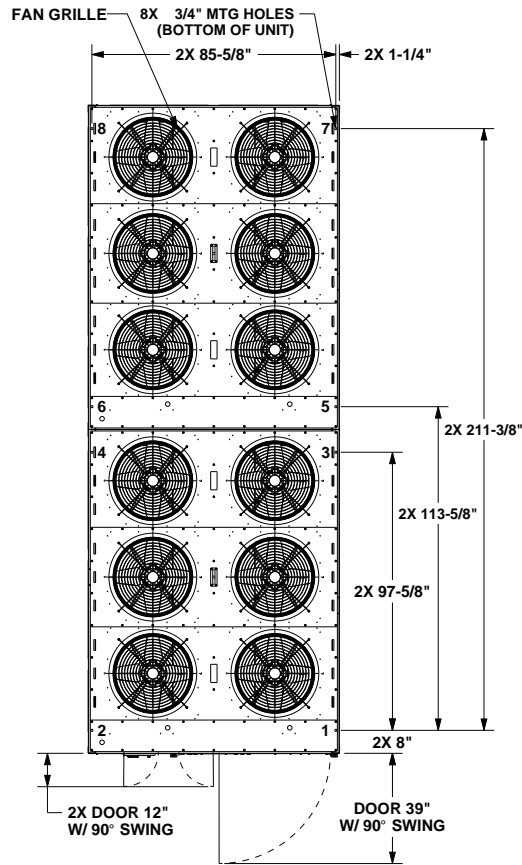
Figure 19. Air-cooled condenser — 100 and 120 tons
