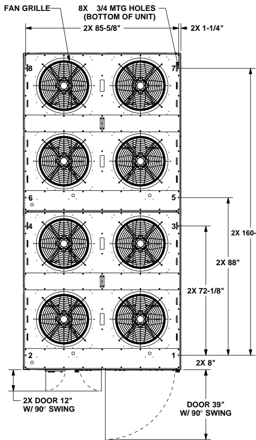
Figure 17. Air-cooled condenser — 80 ton
