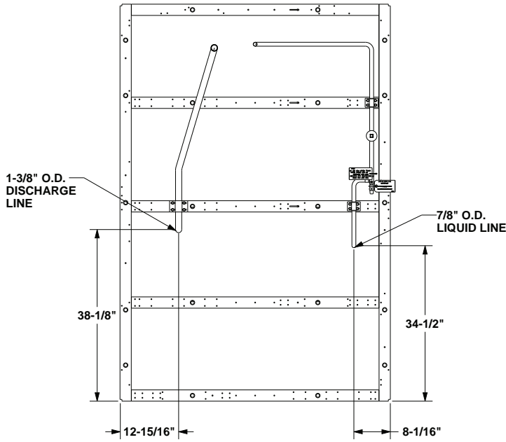
PLAN VIEW OF UNIT
