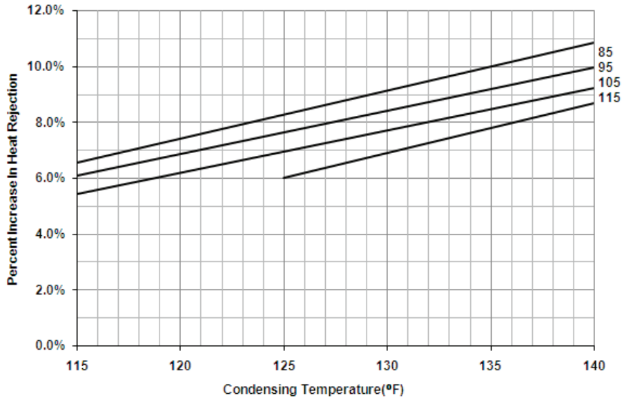
Figure 4. Condenser heat rejection increase due to subcooling (R-410A)
