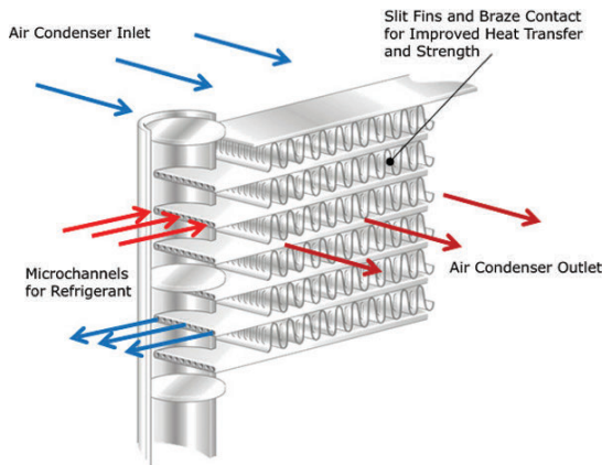
Figure 1. Microchannel condenser coil
