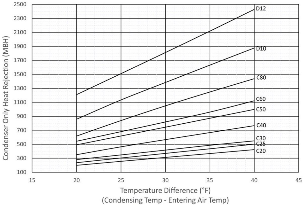
Figure 6. Condenser heat rejection (R-410A/R-454B) — 20 to 120 tons
