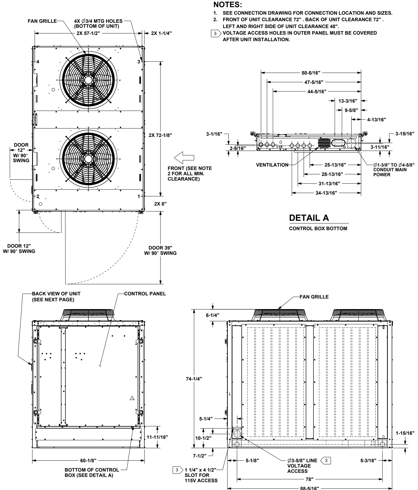
Figure 7. Air-cooled condenser — 20 ton
