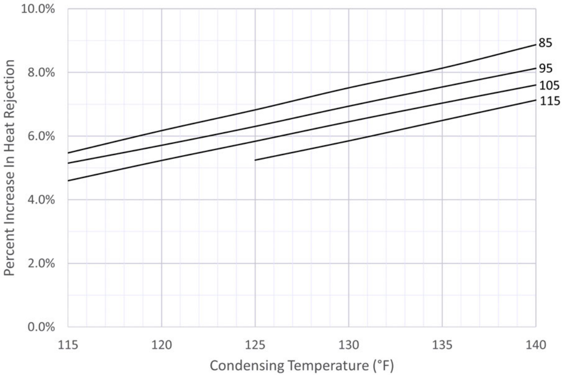
Figure 5. Condenser heat rejection increase due to subcooling (R-454B)
