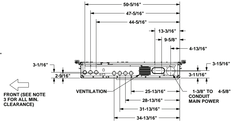
DETAIL A CONTROL BOX BOTTOM
