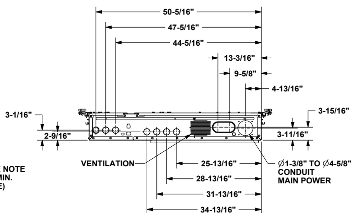
DETAIL A CONTROL BOX BOTTOM
