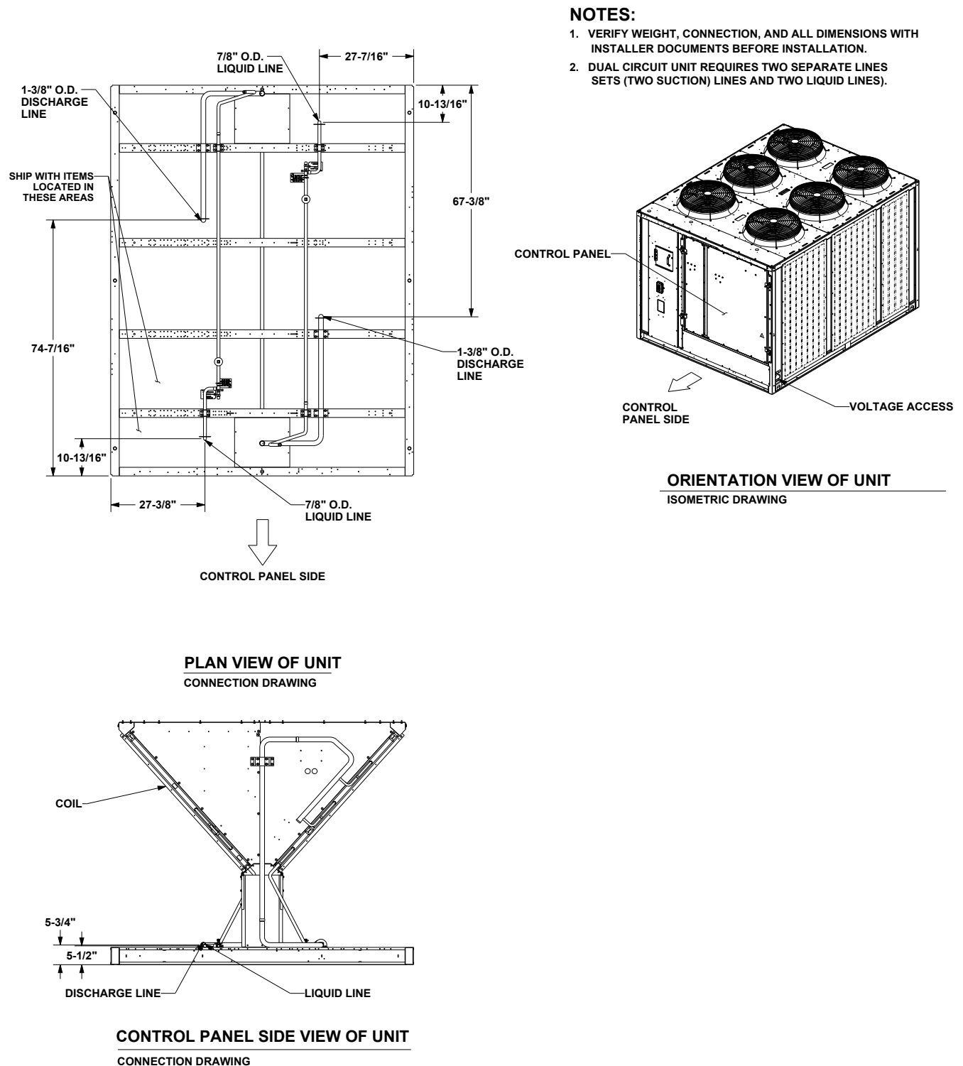
Figure 11. Air-cooled condenser connections — 50 ton
