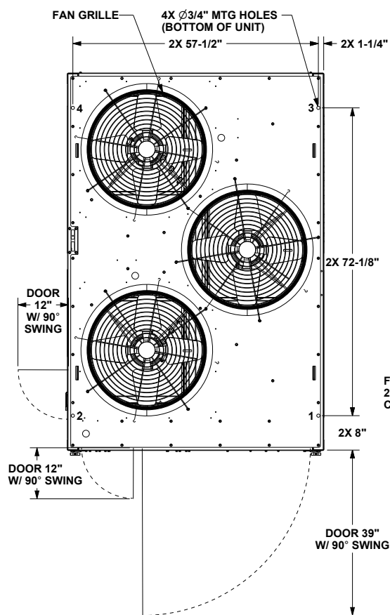
Figure 6. Air-cooled condenser — 25 and 30 tons
