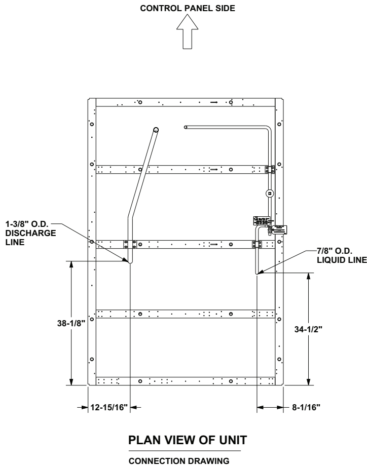
Figure 7. Air-cooled condenser connections — 25 and 30 tons
