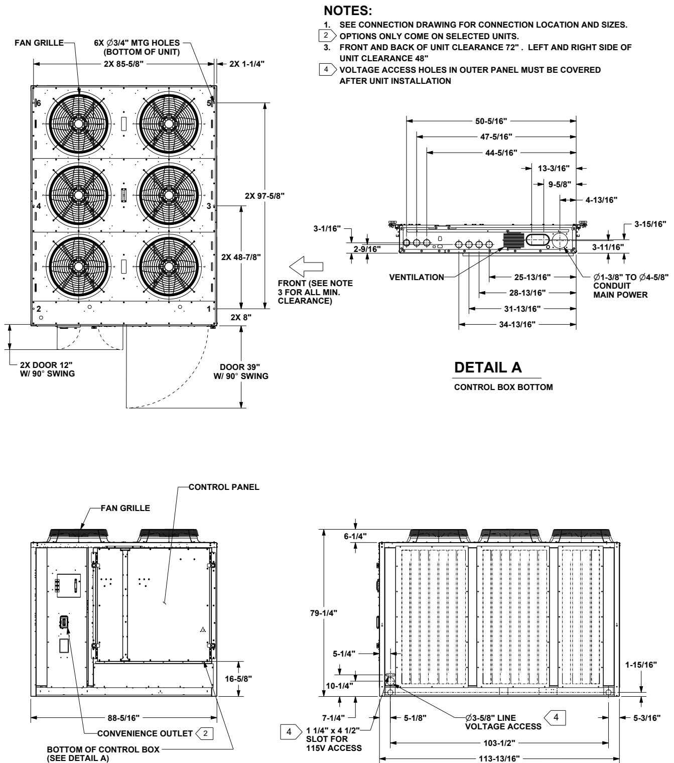
Figure 10. Air-cooled condenser — 50 ton
