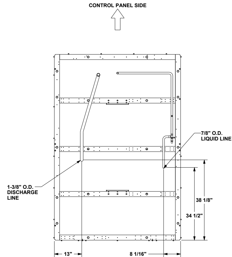
PLAN VIEW OF UNIT CONNECTION DRAWING
