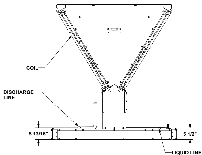
VIEW OPPOSITE OF CONTROL PANEL CONNECTION DRAWING
