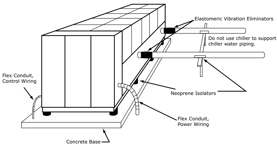
Figure 4. Installation example
