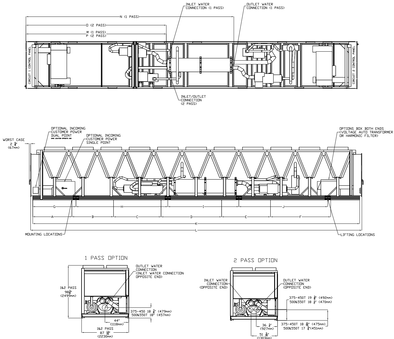
Figure 11. Dimensions — 375 to 550 ton units without direct-free cooling
