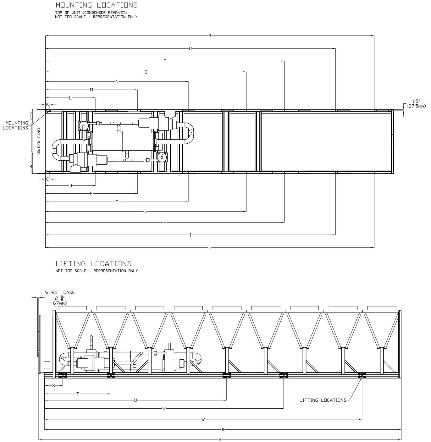
Figure 8. Dimensions — 150 to 330 ton units, standard length, mounting and lifting
