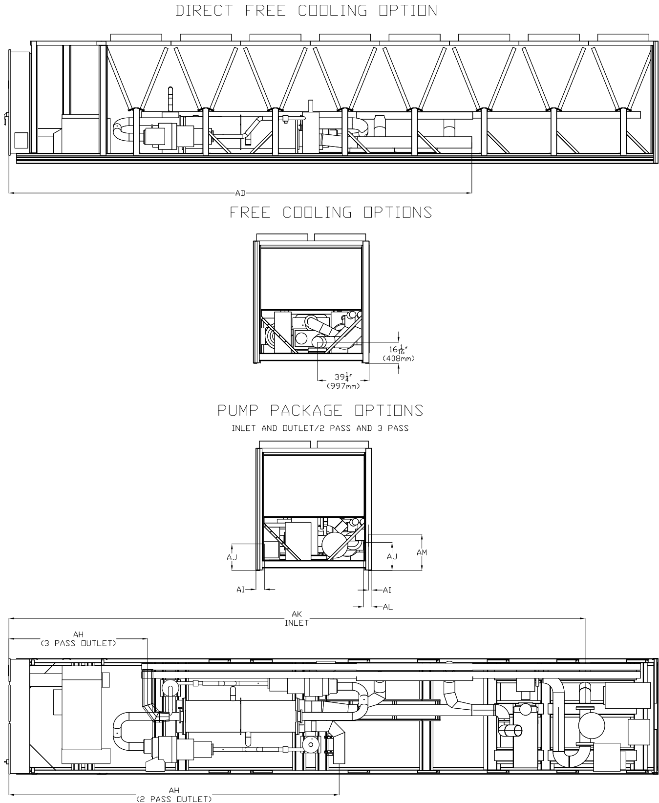
Figure 10. Water connection dimensions — 150 to 330 ton units with free-cooling or pump package option
