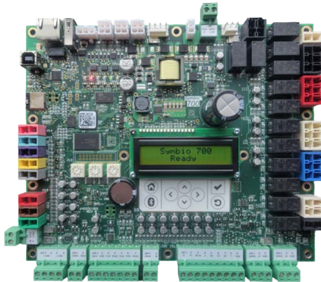
Figure 2. Symbio 700 controller
