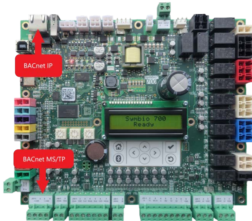
Figure 12. Communication wiring
