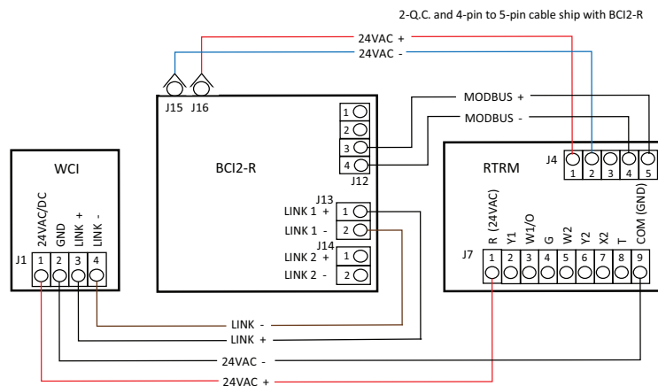
Figure 2. Wiring the Air-Fi Wireless Communication Interface (WCI)
