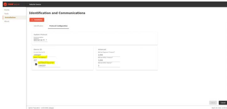
Figure 1. Setting the controller address with the embedded BC12 Service Tool
