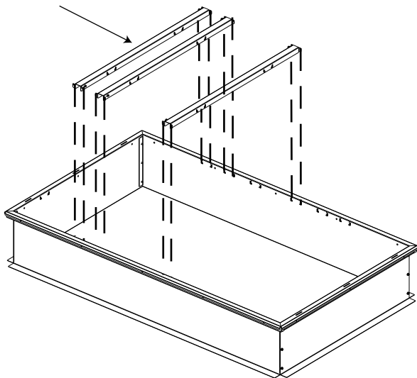
Long Duct Supports
