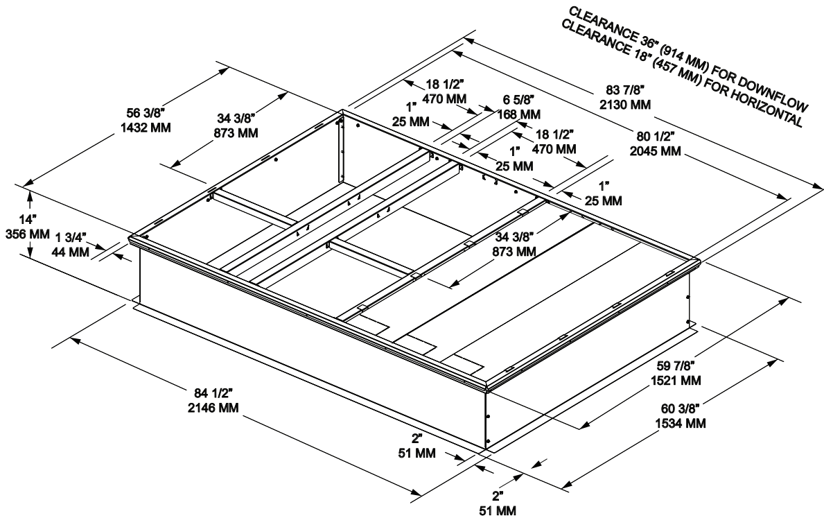
Figure 1. Curb dimensional data
