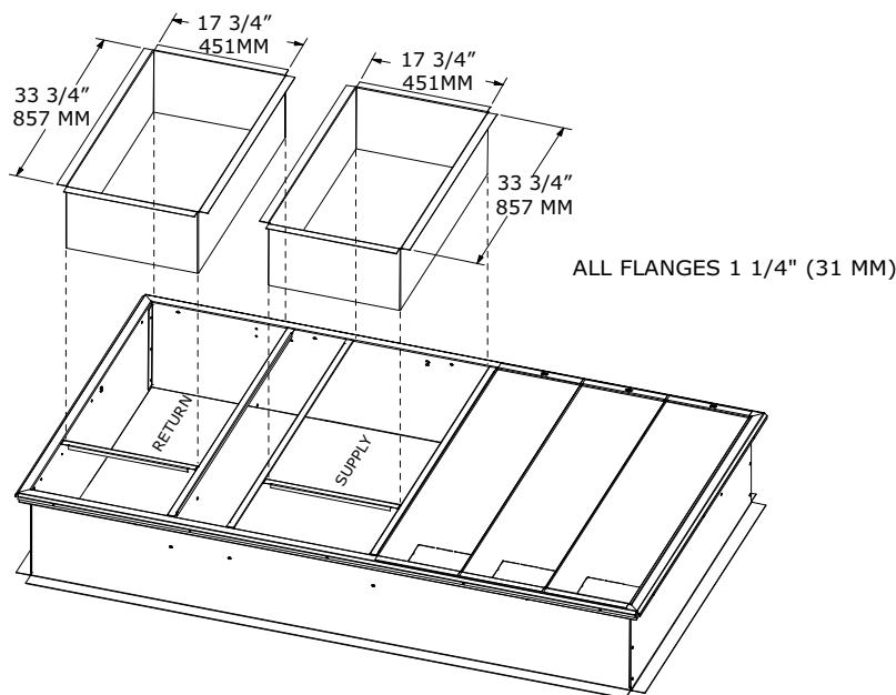
Figure 2. Curb dimensional data
