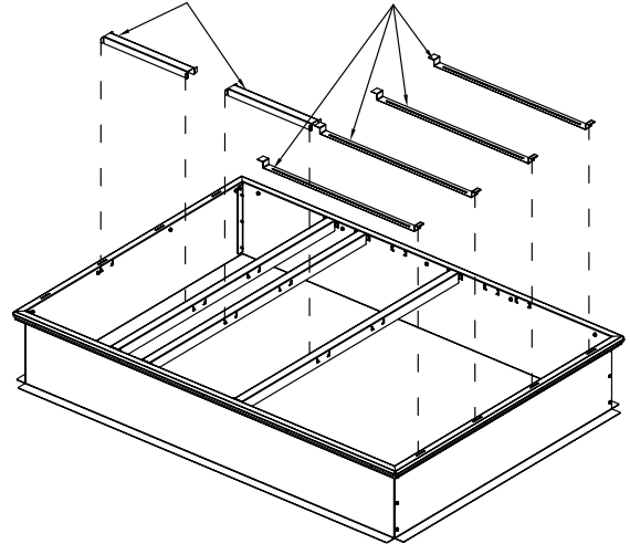
Short Duct Supports Insulation Supports
