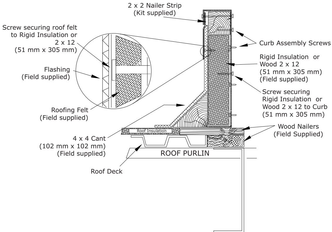
Figure 4. Existing roof construction
