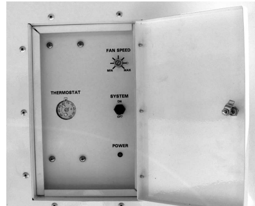
Figure 5. 150 kW (F0) Control Panel
