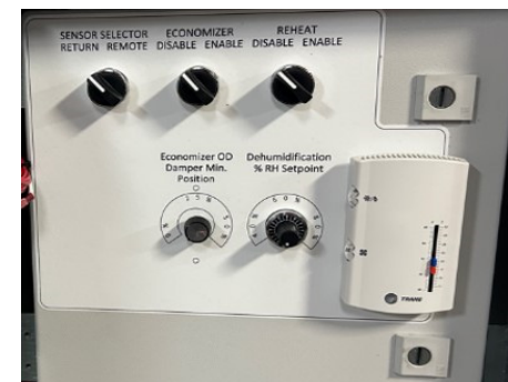
Figure 8. Control panel
