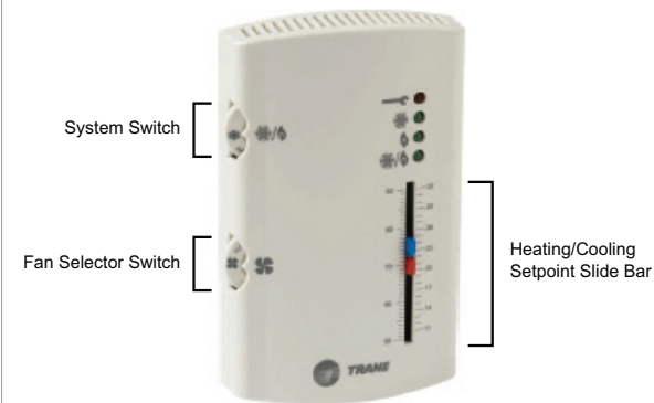
Figure 7. Sensor switch
