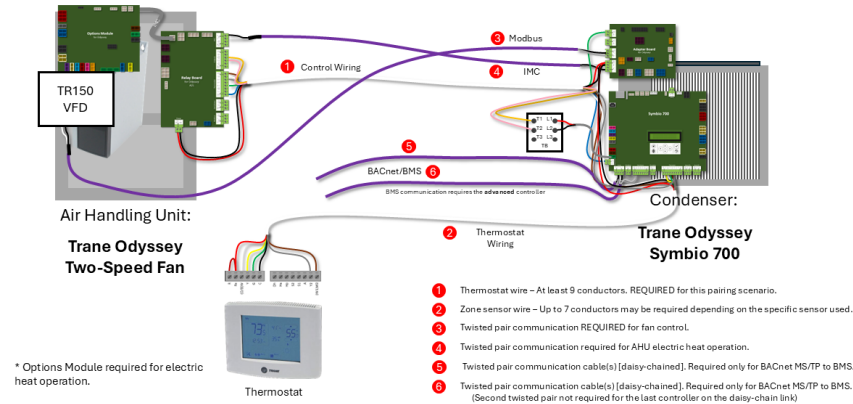
Figure 12. Pairing Y for condenser cooling or heat pump thermostat control applications
