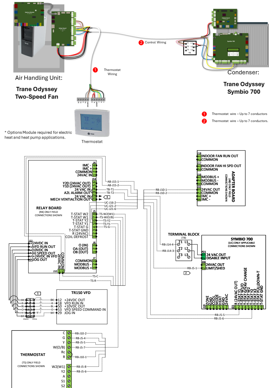
Figure 3. Pairing H for two speed condenser cooling thermostat control applications
