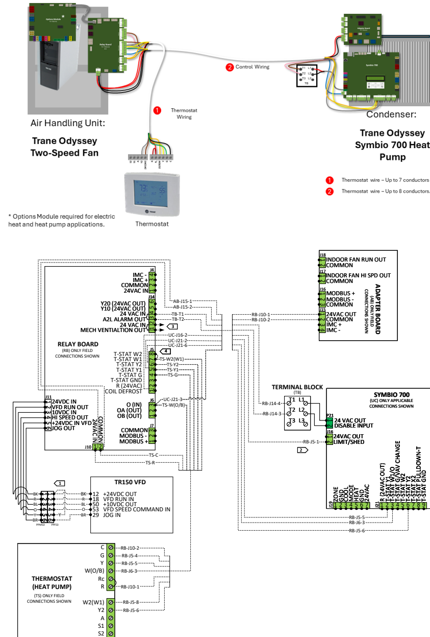
Figure 4. Pairing H for two speed heat pump thermostat control applications
