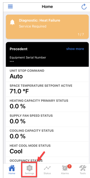
Figure 40. Home screen
