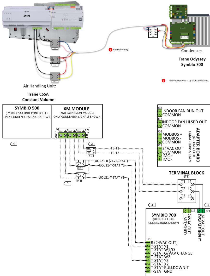
Figure 17. Pairing Alt3
