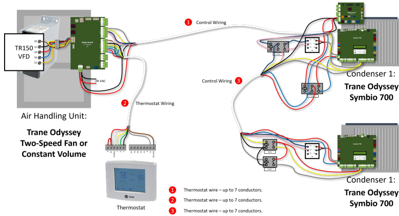
Figure 22. Pairing Alt 8
