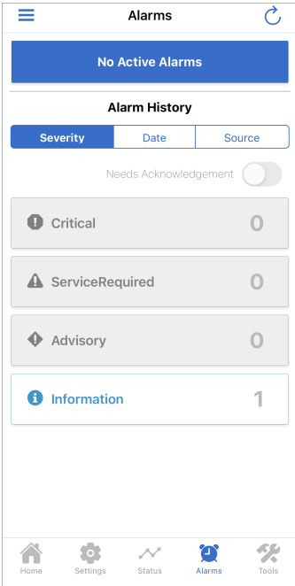
Figure 32. Alarms screen
