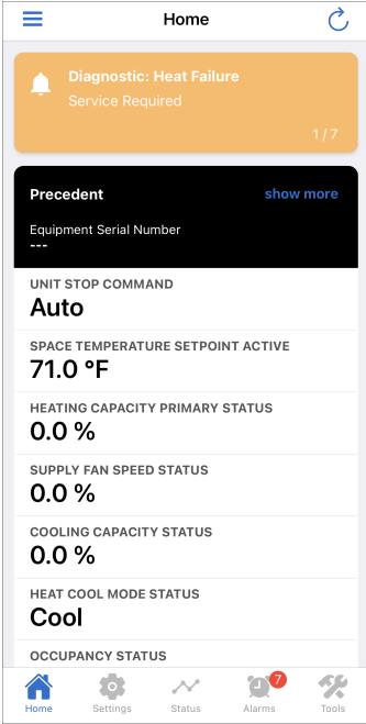
Figure 29. Home screen
