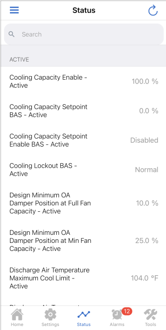
Figure 31. Status screen
