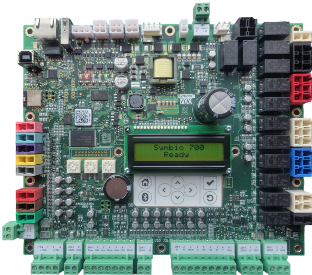
Figure 25. Symbio 700 controller
