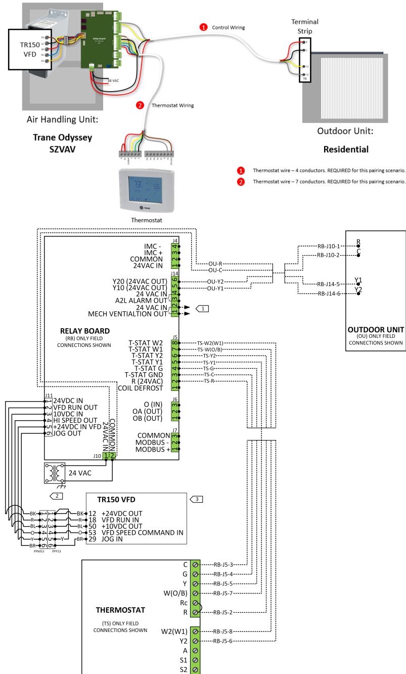
Figure 20. Pairing Alt6 for thermostat control applications
