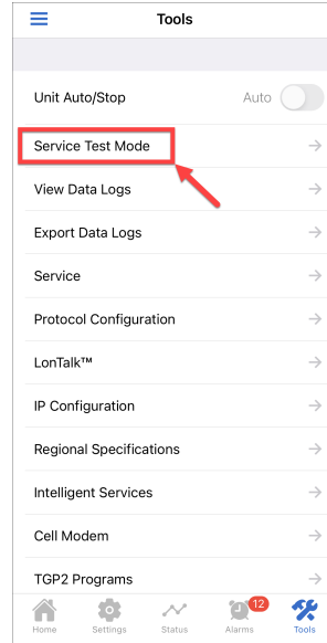
Figure 46. Tools screen
