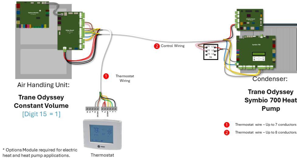
Figure 2. Pairing A for constant speed heat pump thermostat control applications
