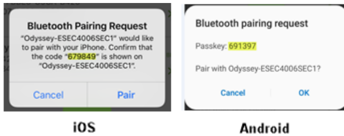
Figure 28. Bluetooth pairing
