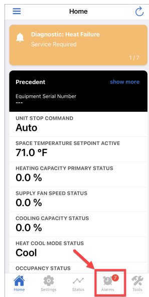
Figure 41. Home screen
