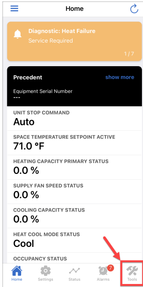
Figure 45. Home screen
