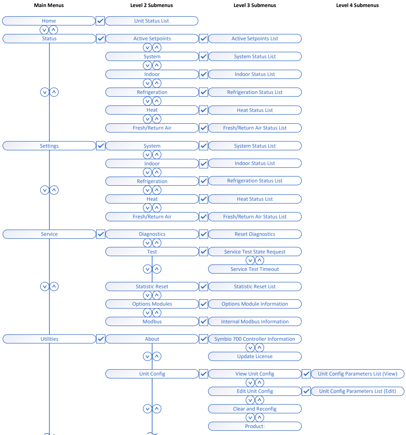
Figure 51. Symbio 700 menu
