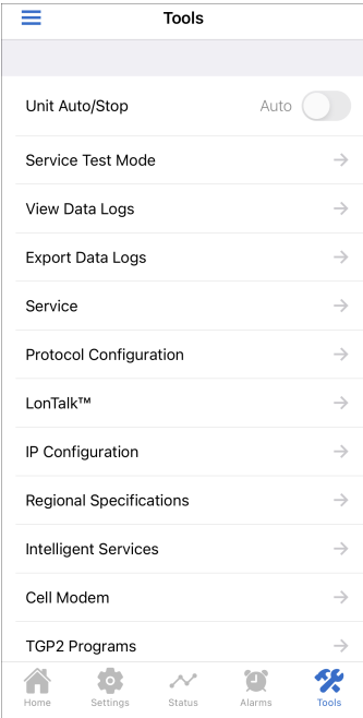
Figure 33. Tools screen
