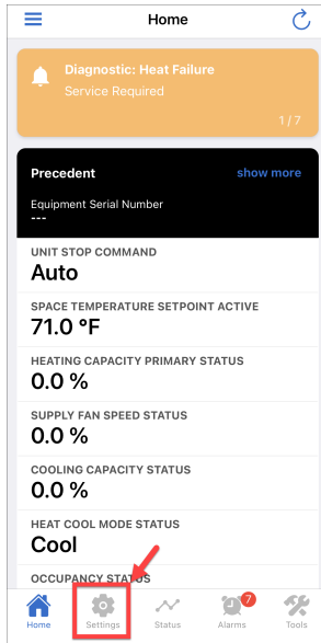
Figure 34. Home screen
