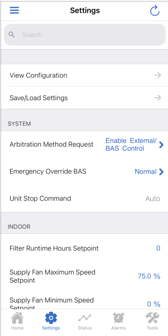
Figure 30. Settings screen
