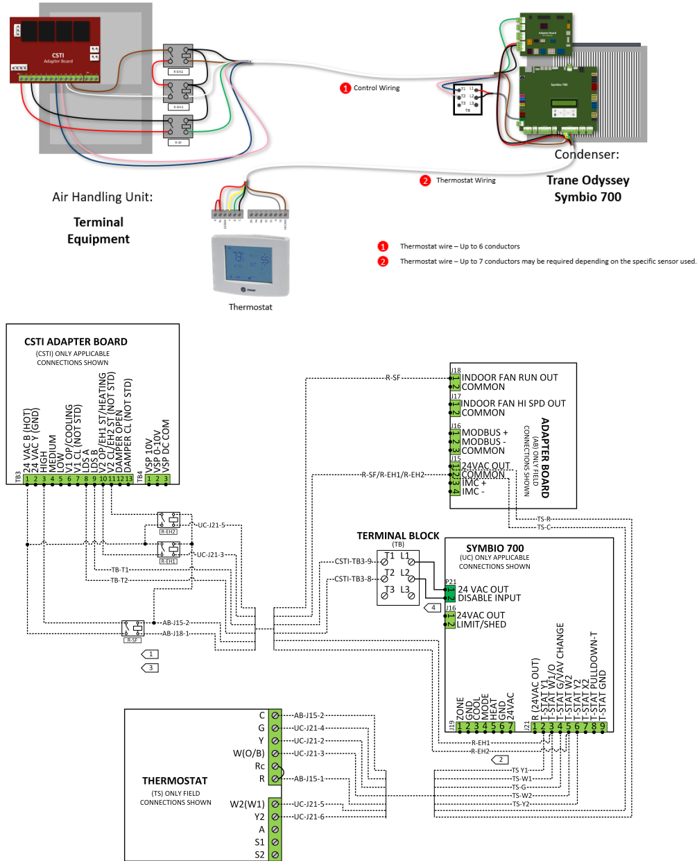
Figure 19. Pairing Alt5 for thermostat control applications
