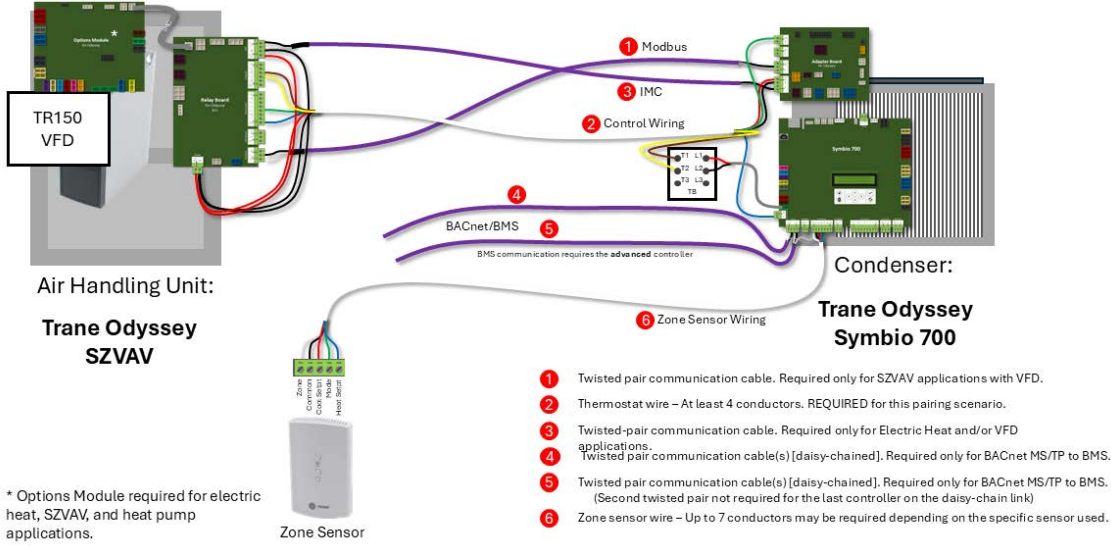
Figure 13. Pairing B for zone sensor control applications
