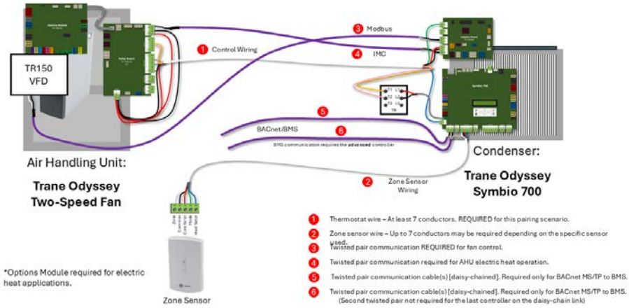
Figure 10. Pairing H for zone sensor control applications
