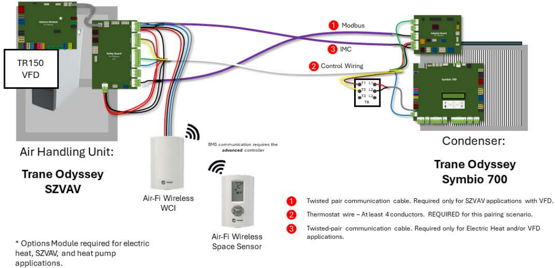
Figure 14. Pairing B for Air-Fi Wireless control applications
