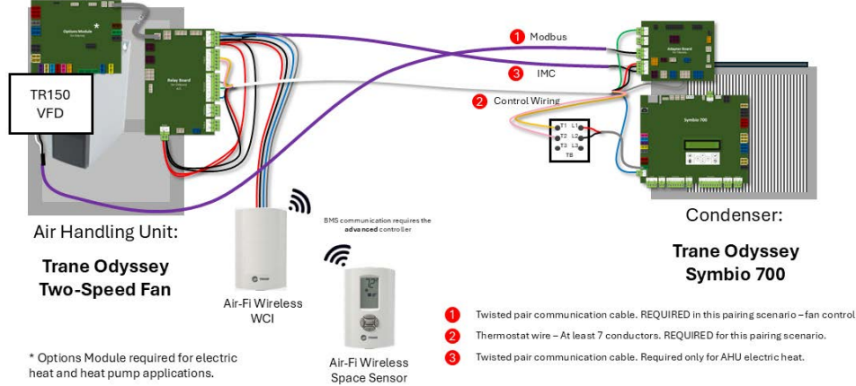
Figure 11. Pairing H for Air-Fi Wireless control applications
