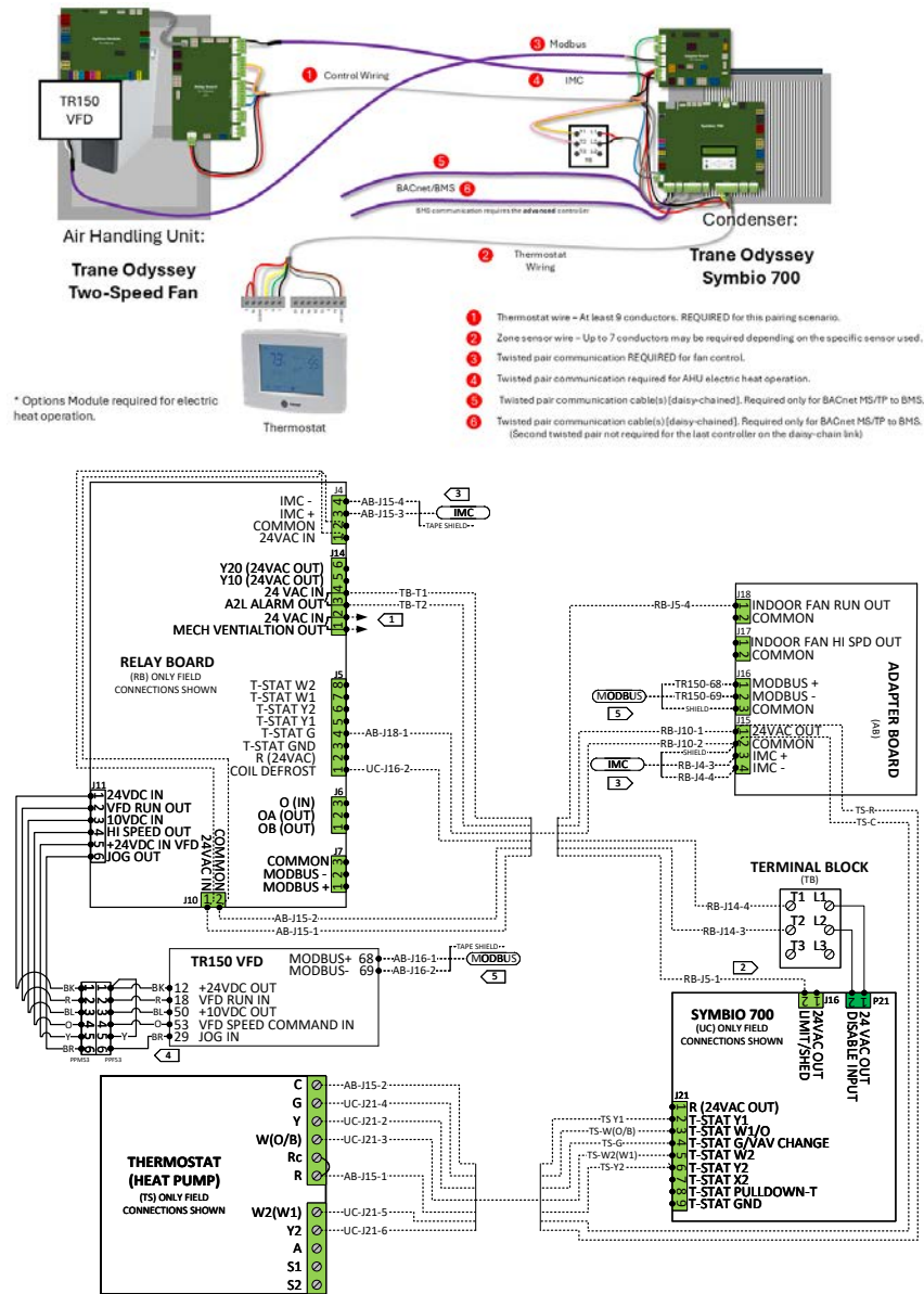
Figure 9. Pairing H for condenser cooling or heat pump thermostat control applications
