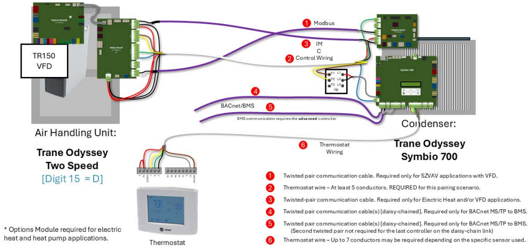
Figure 12. Pairing B for thermostat control applications
