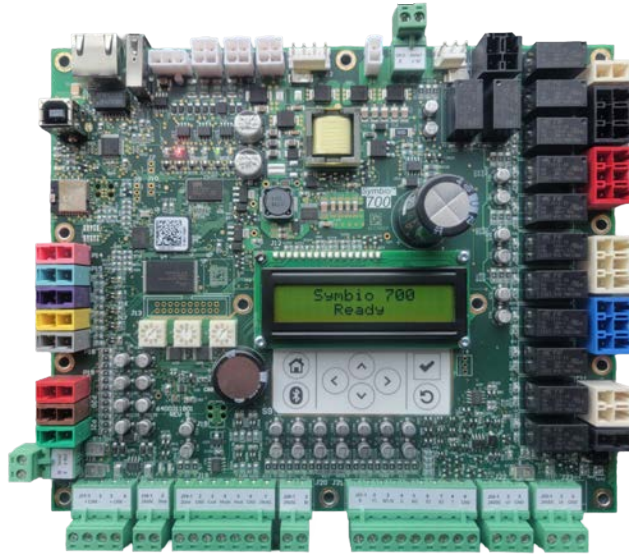
Figure 16. Symbio 700 controller
