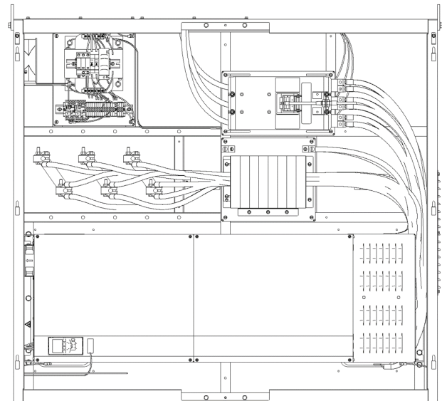
Figure 2. Open direct mount AFDH internal view
