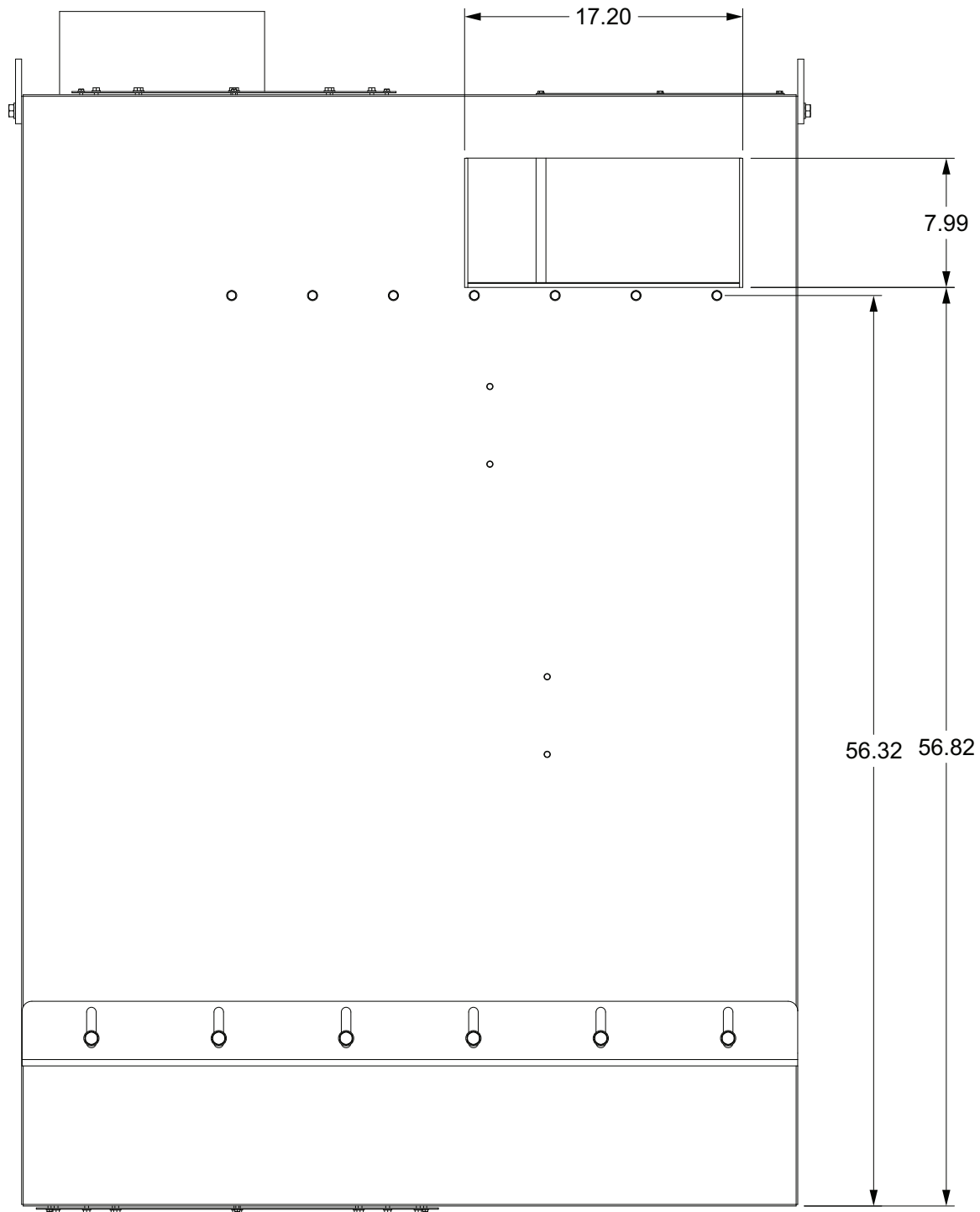
Figure 16. Rear view of E-Frame AFDH cabinet with dimensions - transition mount drive
