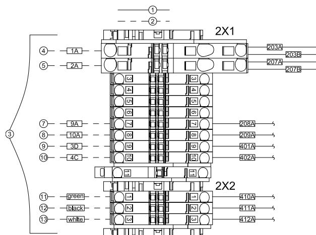
Figure 53. Wiring connections to 2X1 terminal strip in AFDH
