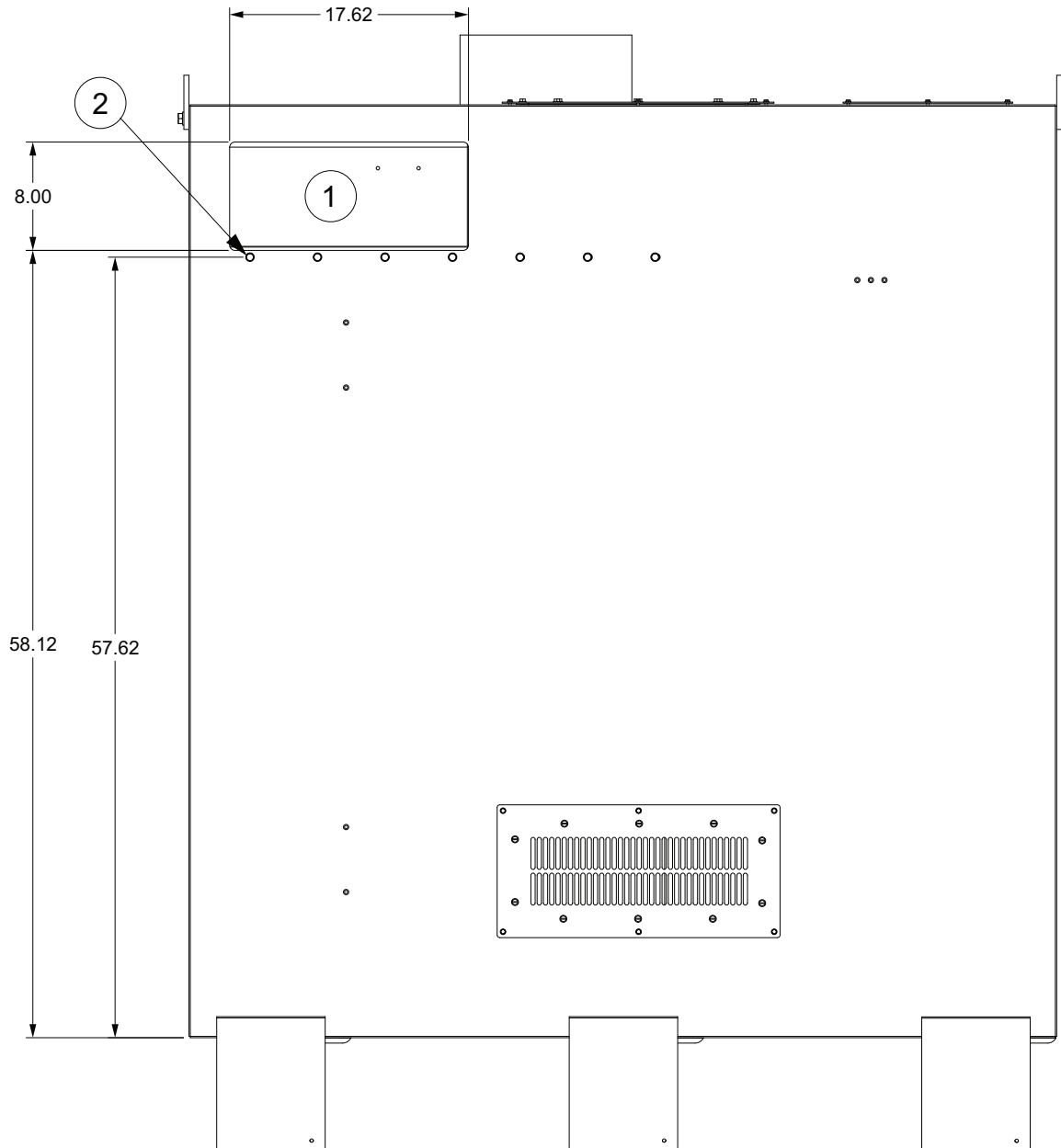
Figure 18. Rear view of LF 1/1.5 frame 4 E-Frame AFDH cabinet with dimensions - LiquiFlo drive
