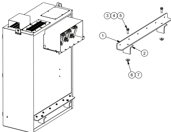
Figure 23. Transition mounting
