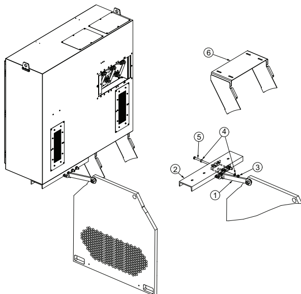
Figure 43. Fixing linkage under the C channel
