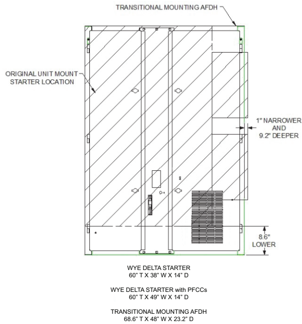
Figure 4. Open transition mount AFDH internal view
