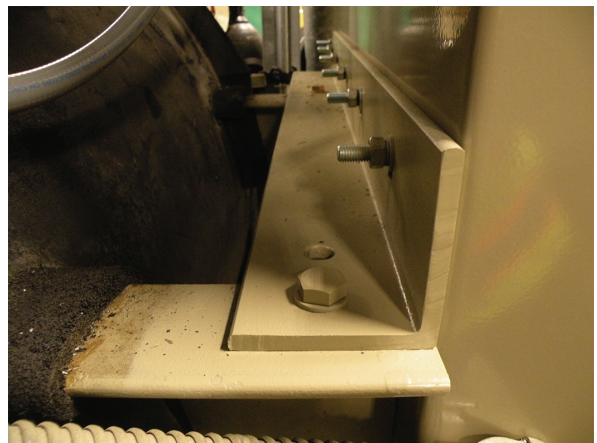
Figure 32. Cabinet angle bracket and evaporator support bracket in position
