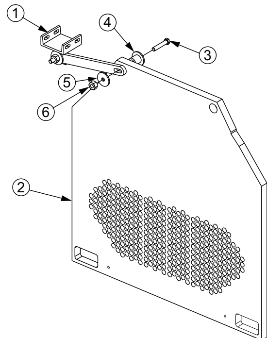
Figure 42. Install linkage subassembly into tube sheet
