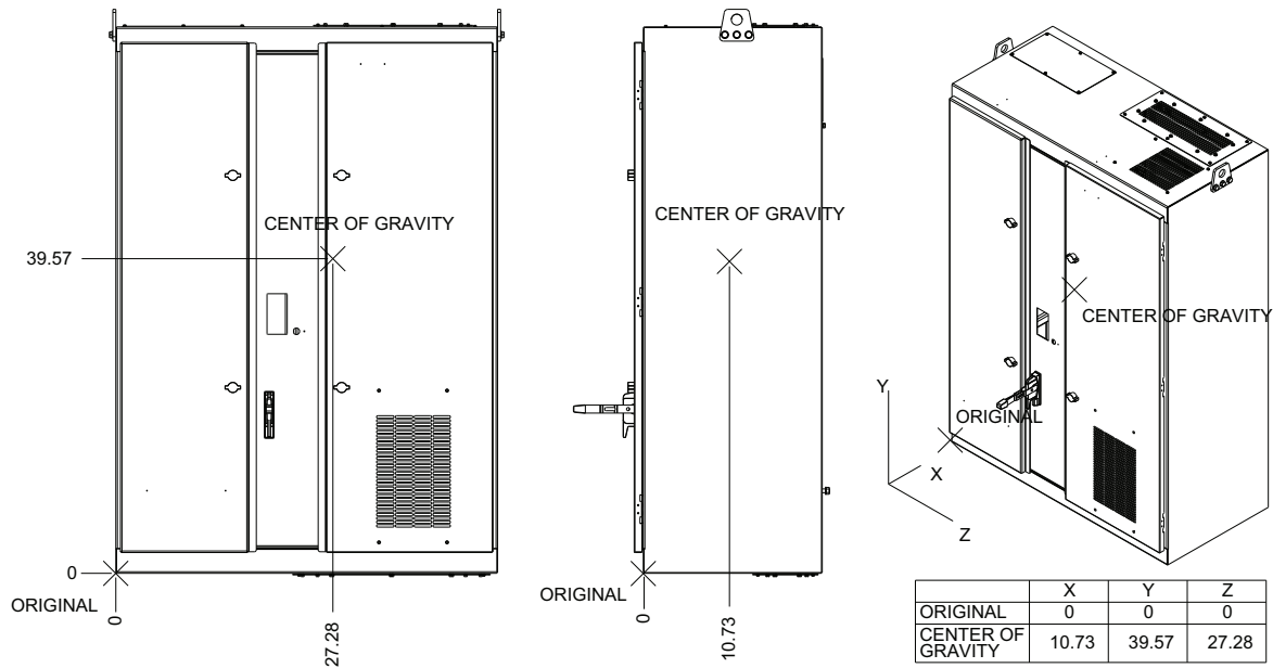
Figure 11. Transition mount and LiquiFlo 1.0/1.5 frame 3
