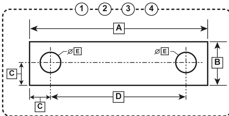
Figure 20. Buss bars specifications: Tracer AdaptiView hardware packages
