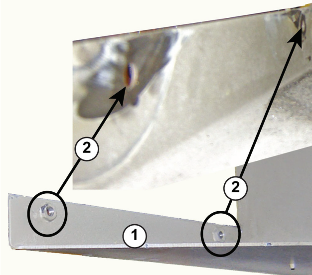
Figure 22. Removal of Z-bracket weldment nuts
