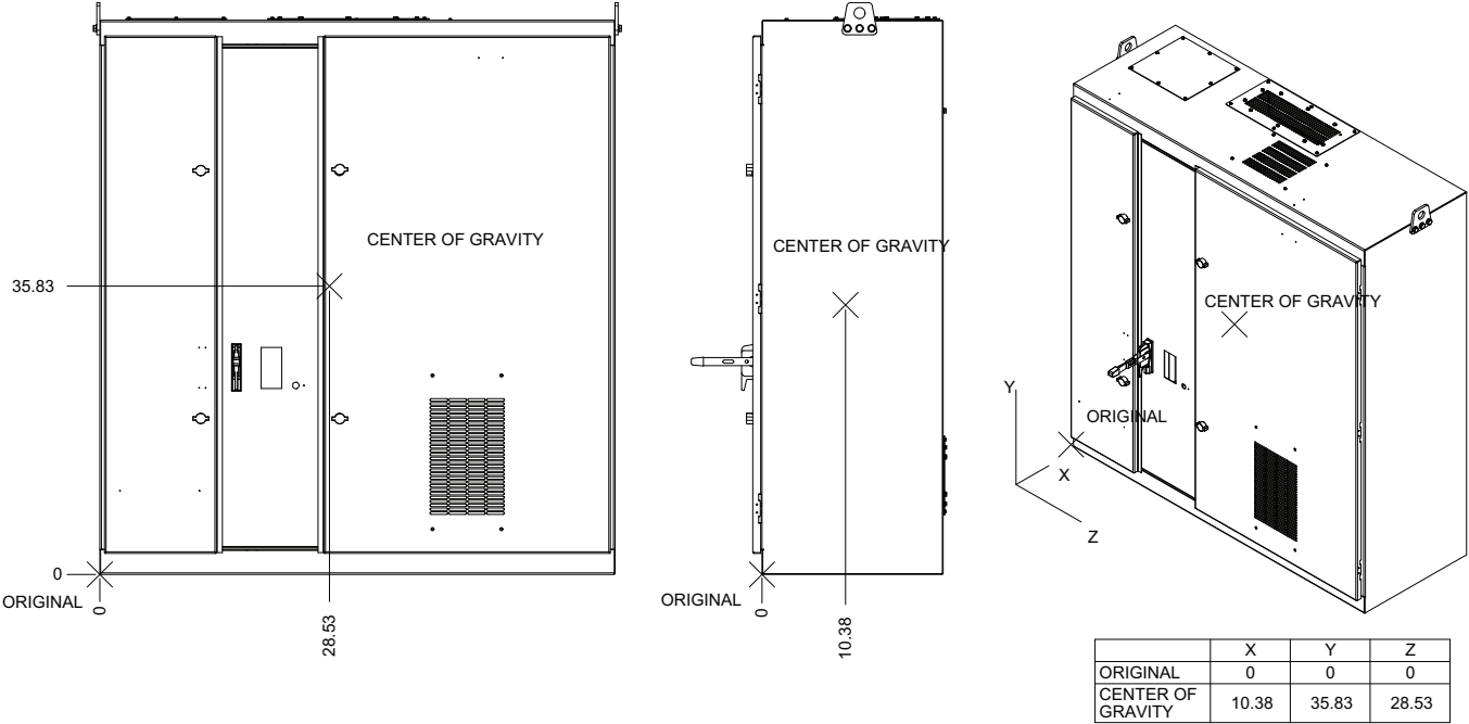
Figure 12. LiquiFlo 1.0/1.5 frame 4
