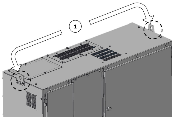
Figure 7. Unit lifting points and center of gravity
