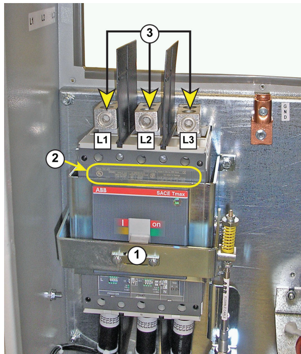
Figure 50. Factory installed input disconnect circuit breaker
