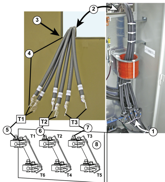
Figure 52. Output wiring from AFDH to CTV motor
