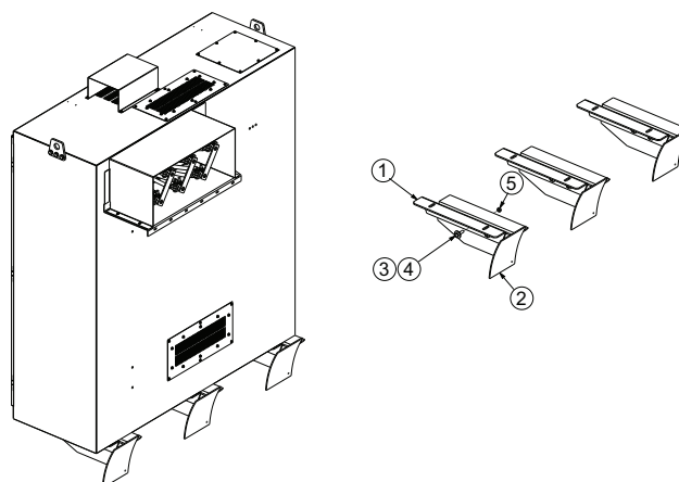
Figure 46. LiquiFlo 1.0/1.5 frame 4 mounting installation
