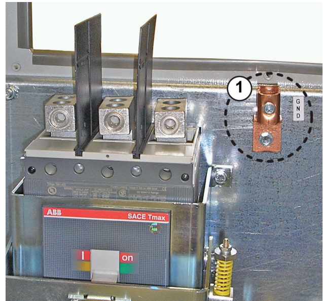
Figure 51. Location of AFDH cabinet ground terminal
