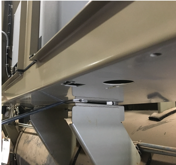
Figure 37. Secure cabinet to evaporator support brackets
