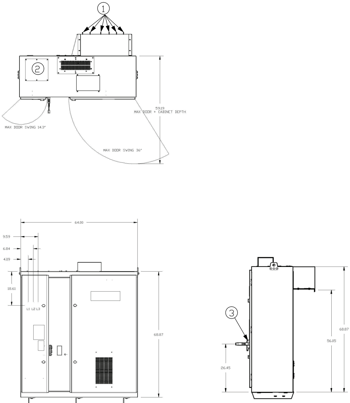
Figure 17. Top, front, and side view of LF 1/1.5 frame 4 E-Frame AFDH cabinet with dimensions - LiquiFlo drive
