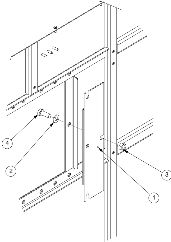
Figure 34. Adapter plate
