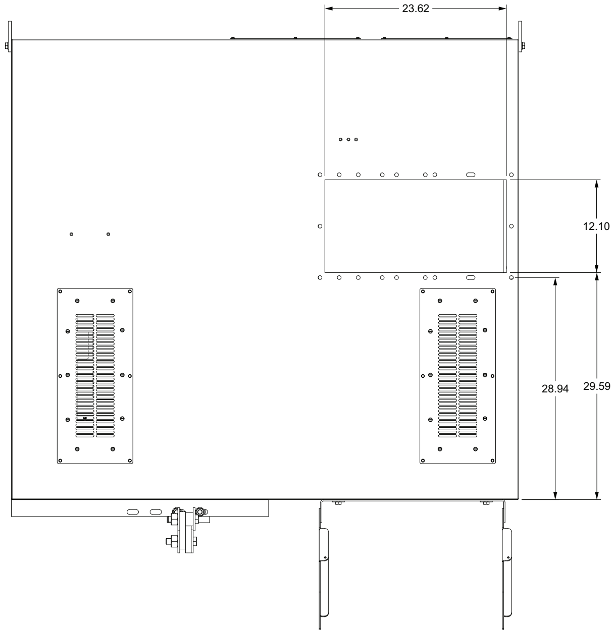
Figure 14. Rear view of E-Frame AFDH cabinet with dimensions - direct mount drive
