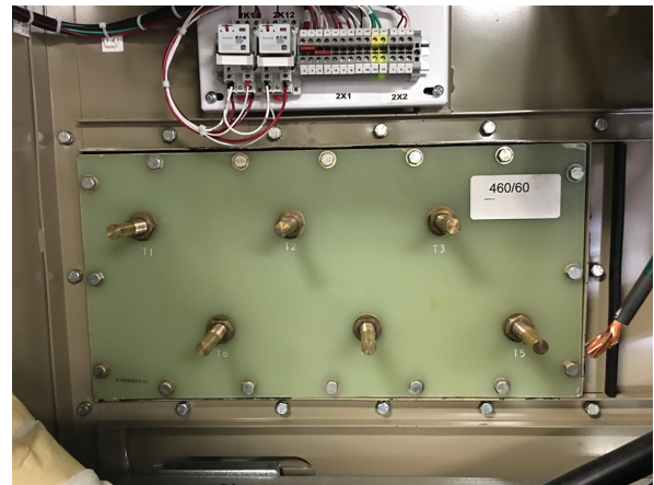
Figure 33. Bolt cabinet to motor
