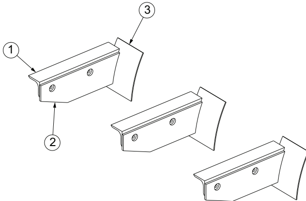
Figure 47. Evaporator mounting bracket
