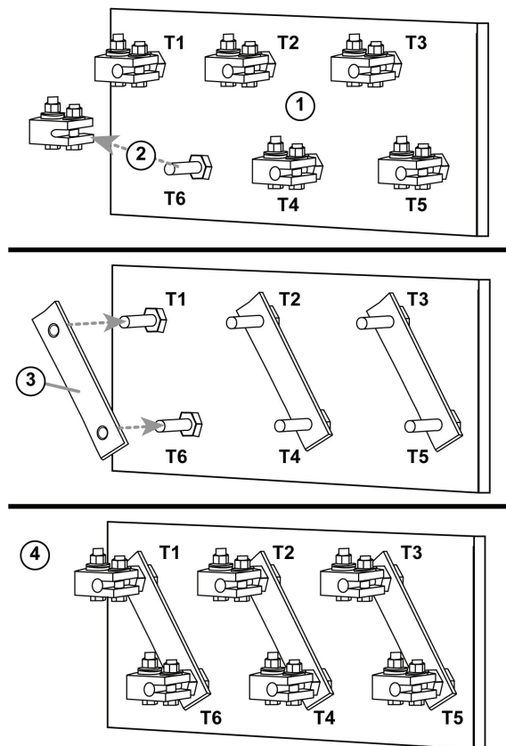
Figure 48. Buss bar installation on compressor motor terminal board
