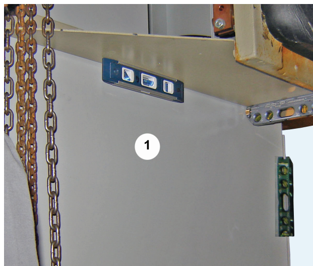
Figure 25. Leveling the AFDH drive cabinet against the Z-bracket
