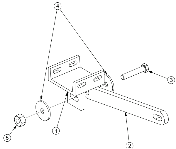
Figure 38. Linkage subassembly installation
