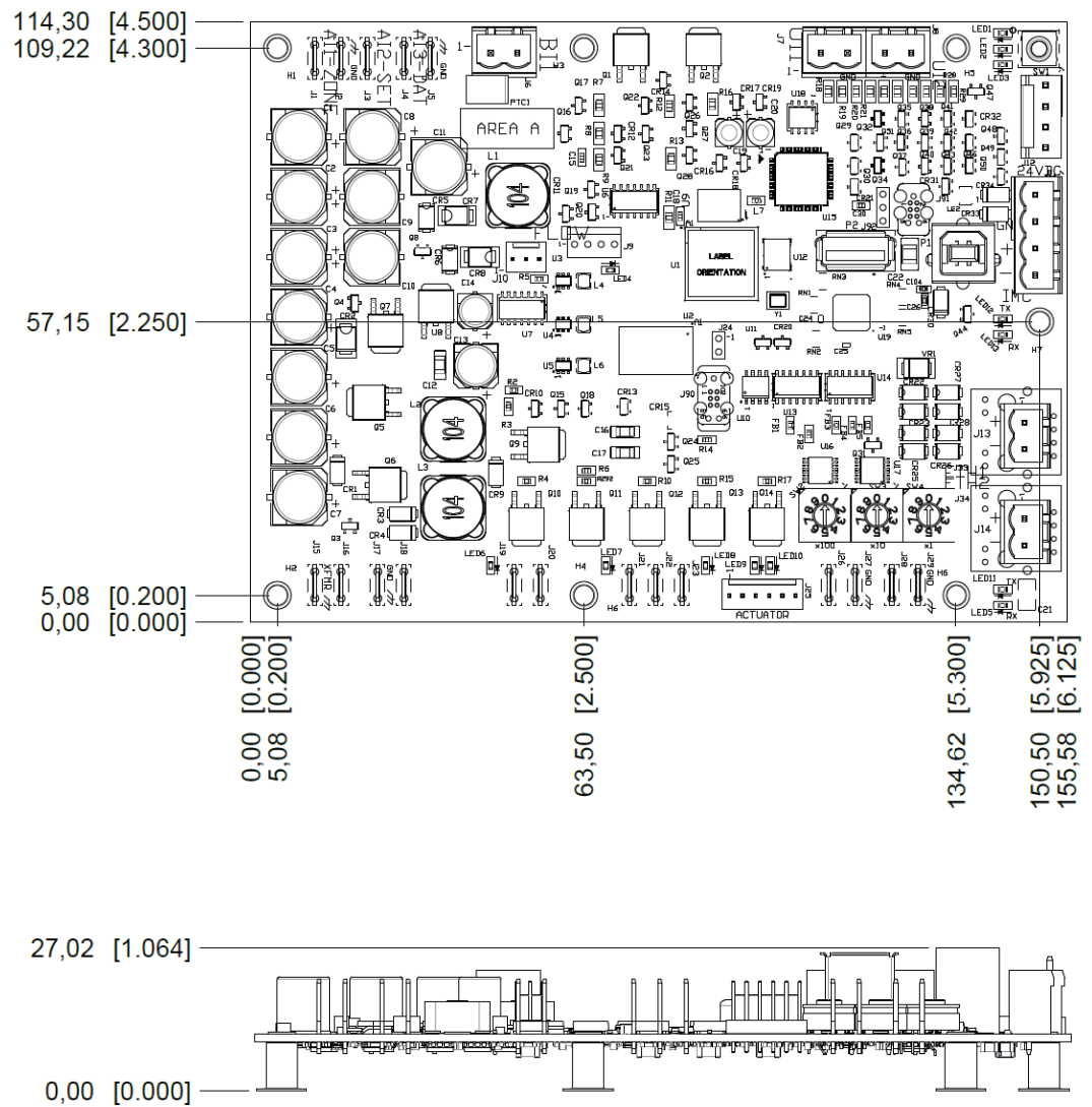
Figure 1. Controller dimension
