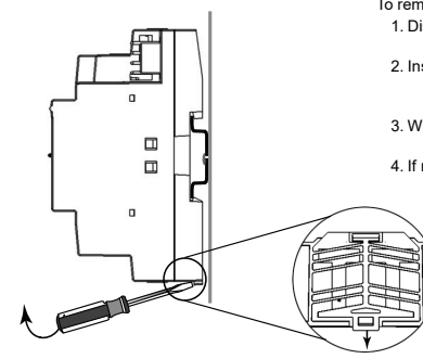
Slotted release clip shown from back side
