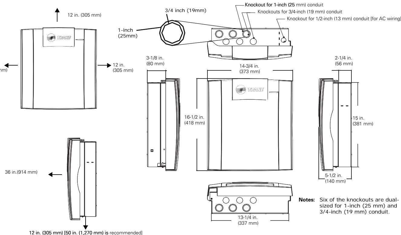
Figure 1. Minimum clearances and enclosure dimensions
